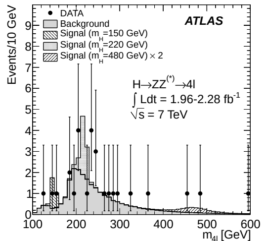
Figure 2: m_{4\ell} distribution of the selected candidates, compared to the background expectation. Error bars represent 68.3% central confidence intervals. The signal expectation for three m_H hypotheses is also shown.
