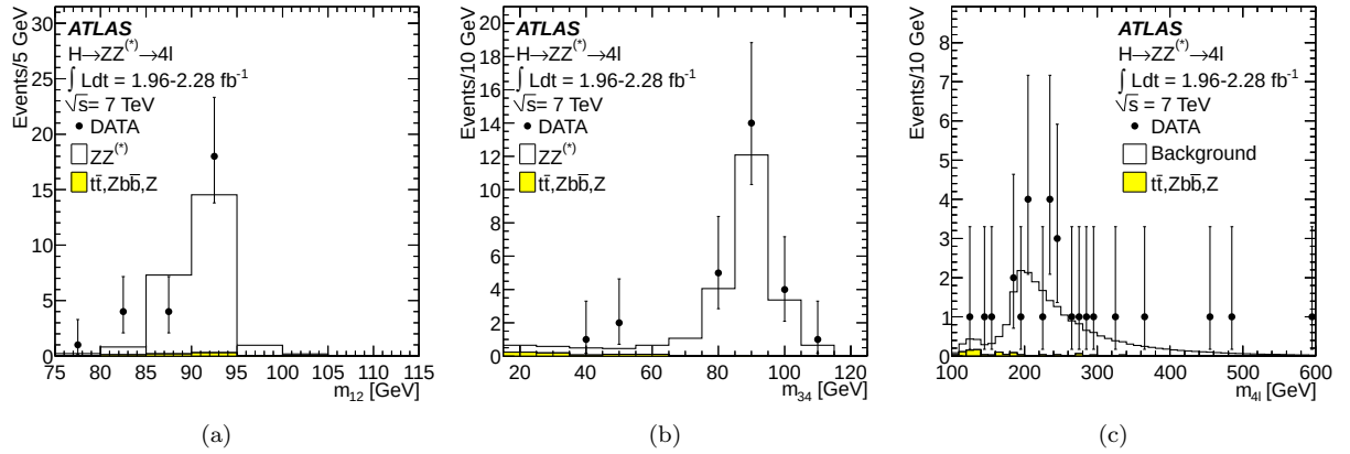
Figure 1: Invariant mass distributions (a) m_{12} , (b) m_{34} , and (c) m_{4\ell} for the selected candidates. The data (dots) are compared to the background expectations from the dominant ZZ^{(*)} process and the sum of t\bar{t} , Zb\bar{b} and Z +light flavour jets processes. Error bars represent 68.3% central confidence intervals.
