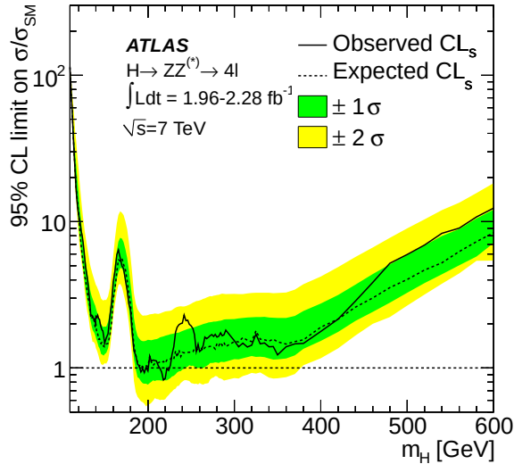
Figure 3: The expected (dashed) and observed (full line) 95% CL upper limits on the Higgs boson production cross section as a function of the Higgs boson mass, divided by the expected SM Higgs boson cross section. The green and yellow bands indicate the expected sensitivity with \pm 1\sigma and \pm 2\sigma fluctuations, respectively.
