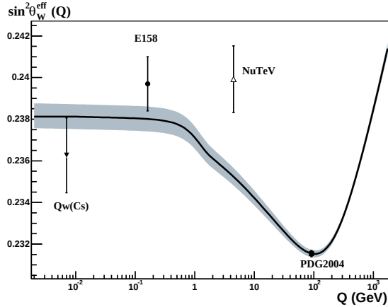
FIG. 2: Predicted variation [18] of \sin^2 \theta_W^{\text{eff}}(Q) as a function of momentum transfer Q (solid line) and its estimated theoretical uncertainty (shaded area). Results of prior low energy experiments [6, 16] (closed triangle, shown at an arbitrarily higher Q ) and [7] (open triangle) are overlaid together with the Z^0 pole value [16] (square) and this measurement (circle).
