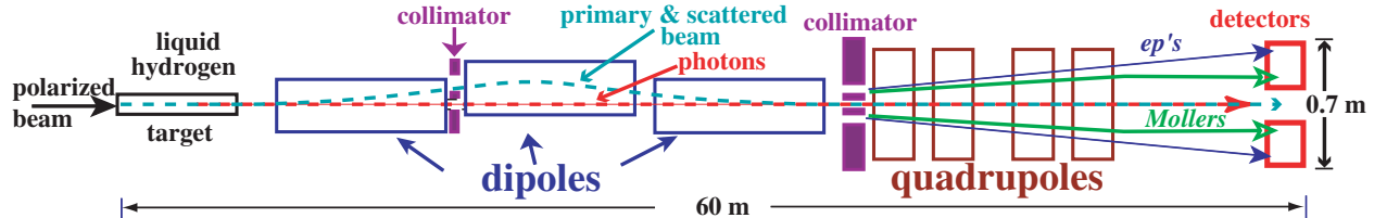
FIG. 1: Schematic plan view of the experimental configuration in SLAC End Station A.
