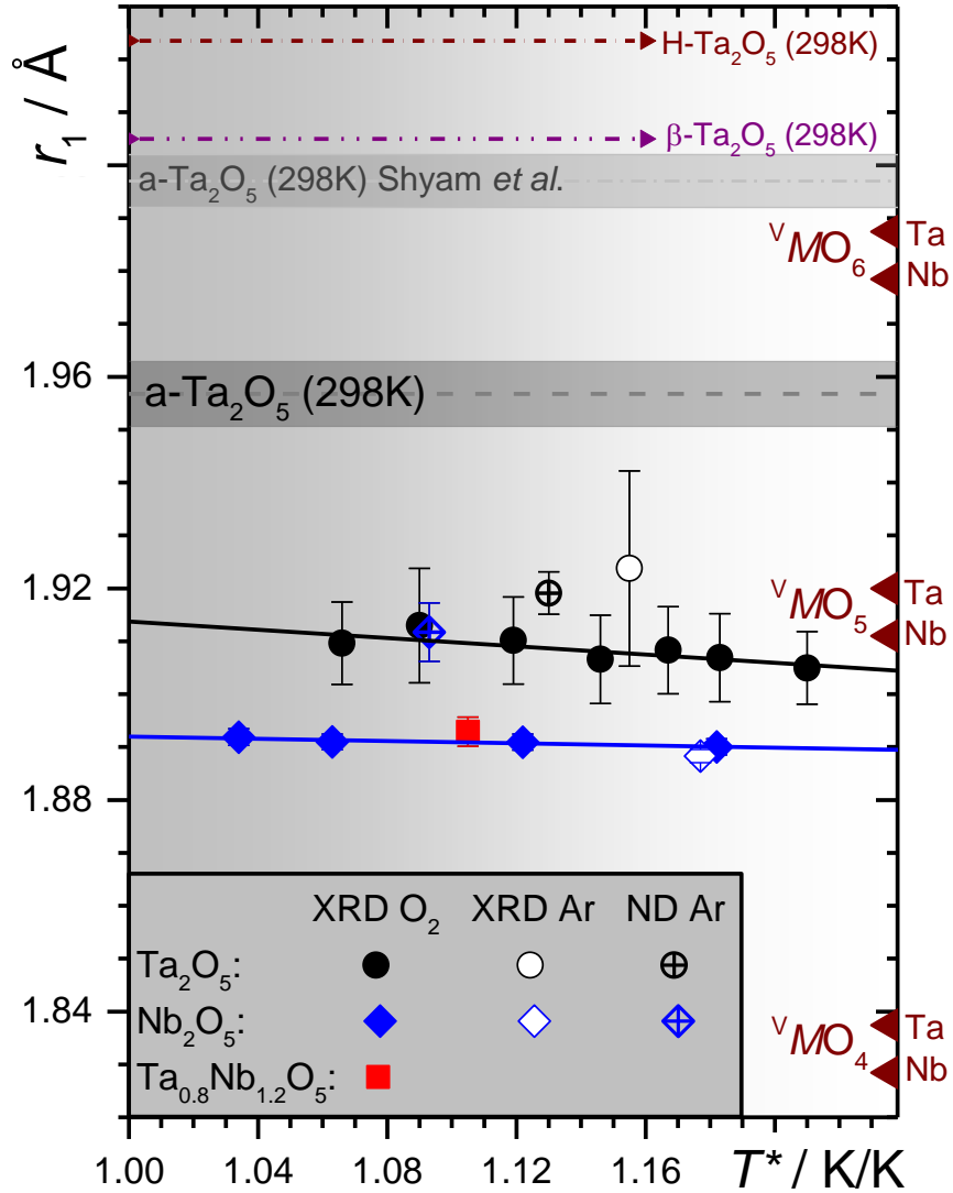
Figure 3: Peak (modal) bond lengths for a-Ta 2 O 5 IBS film and molten Ta 2 O 5 and Nb 2 O 5 liquids, as a function of T^* = T/T_{\text{melt}} . Solid lines are linear regressions of the XRD data collected in O 2 gas. Crystallographic mean bond lengths for H-Ta 2 O 5 [43] and \beta -Ta 2 O 5 [40] are shown for comparison. Also shown to the right-hand side are bond-valence derived bond-lengths for 4-, 5- and 6-fold pentavalent cations, relevant to ambient temperature and calculated assuming equivalency of all bonds within the polyhedron. Note that this equivalency of bonds does not exist in the liquids or the amorphous film, where the mean and modal bond lengths differ significantly. Nonetheless, the bond-valence derived values serve as a useful reference point.
