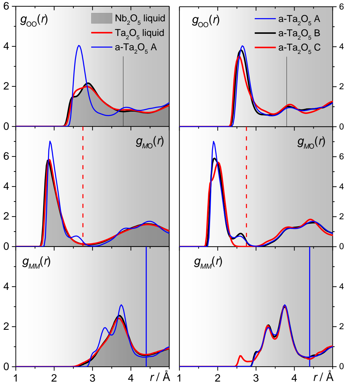
Figure 5: Partial pair distribution functions derived by EPSR for the \text{a-Ta}_2\text{O}_5 IBS film and molten \text{Ta}_2\text{O}_5 and \text{Nb}_2\text{O}_5 liquids. Vertical lines correspond to cutoff radii for which coordination number and bond-angle distributions were calculated.
