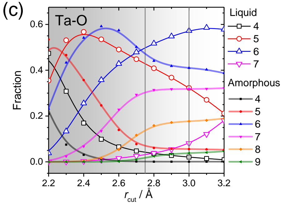
Figure 6: Coordination number distributions for a-Ta 2 O 5 IBS film and molten Ta 2 O 5 and Nb 2 O 5 liquids a) O–M and M–O distributions for a fixed cutoff radius of 2.75Å. Results from the MD study of Damart, et al. [9] are also shown. b) As a function of cutoff radius for the two liquids. c) As a function of cutoff radius for liquid and solid-amorphous tantalum.
