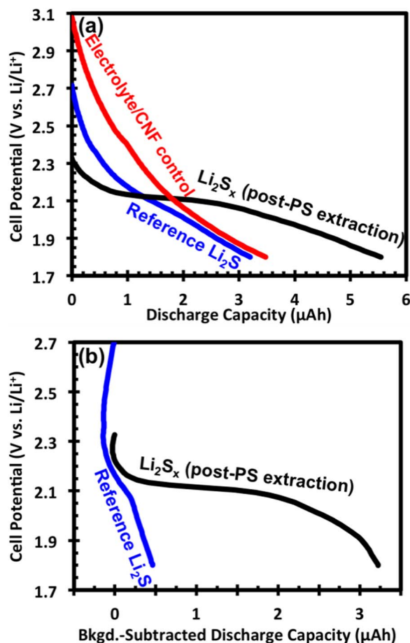
Figure 8. (a) Raw and (b) background-subtracted galvanostatic discharge curves at 100 \mu\text{A cm}^{-2} to 1.8 V vs. \text{Li/Li}^+ for CNF paper control (red line), commercial \text{Li}_2\text{S} (blue line), and synthesized \text{Li}_2\text{S}_x after complete extraction of soluble polysulfides (black line).
