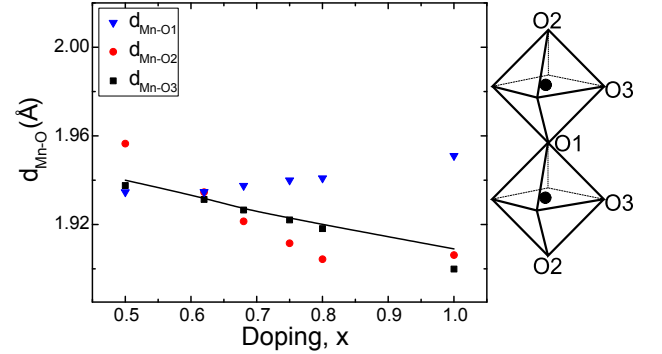
FIG. 2. (Color online) Mn-O bond lengths d_{\text{Mn-O}} in \text{MnO}_6 octahedra and the average Mn-O distance \langle d_{\text{Mn-O}} \rangle (black solid line) of \text{La}_{2-2x}\text{Sr}_{1+2x}\text{Mn}_2\text{O}_7 as a function of doping, x obtained from neutron diffraction 16 .
