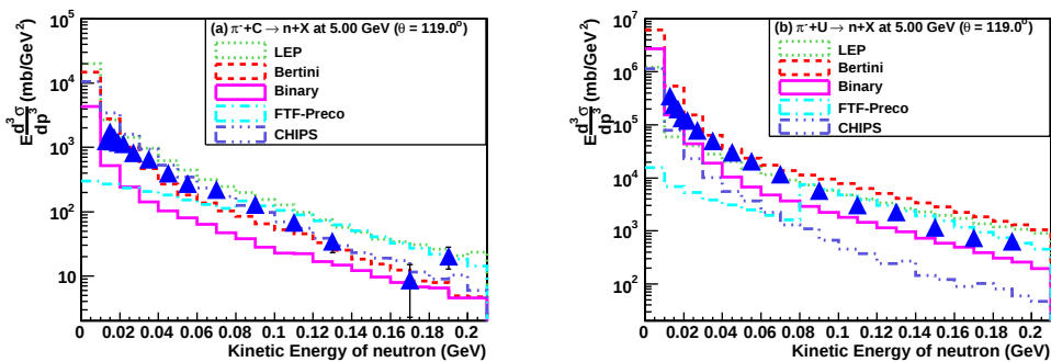
Figure 4. Lorentz invariant cross section for inclusive neutron production at 119.0^\circ in \pi^- -nucleus collisions at 5.0 GeV/c as a function of neutron kinetic energy for (a) Carbon and (b) Uranium targets being compared with predictions of GEANT4 hadronic models.
