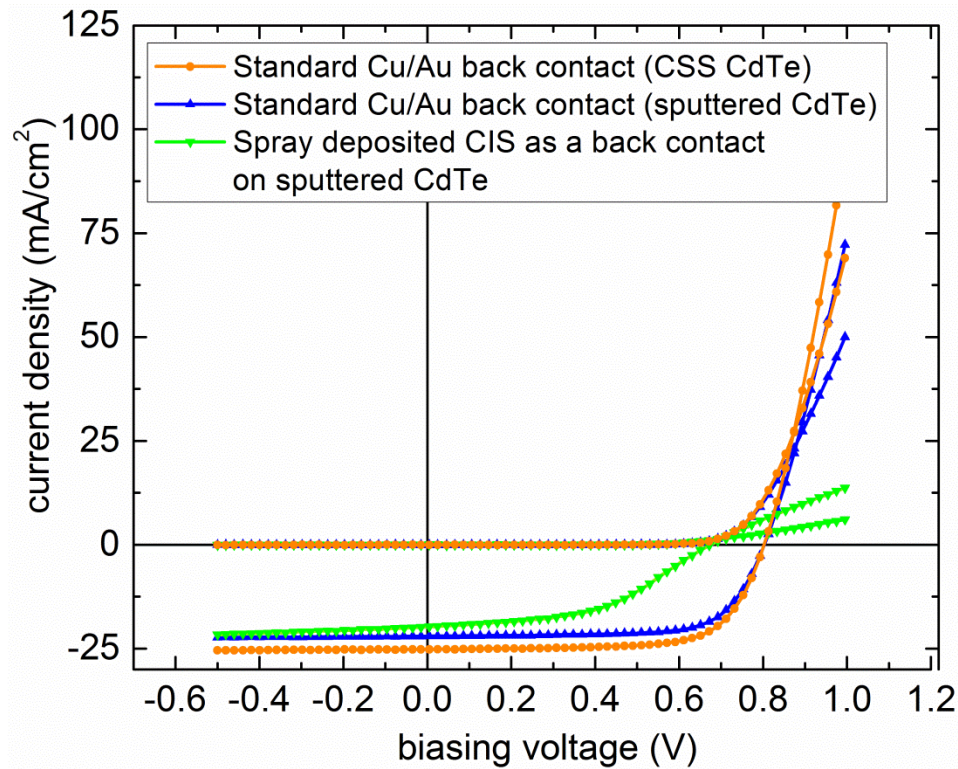
Figure 15. Light and dark J - V curves are compared for CdTe solar cells with the best CIS back contact with standard Cu/Au back contacts. The curves with circular symbols (orange) and upright triangles (blue) are for cells with CSS CdTe and sputtered CdTe absorbers respectively, both with Cu/Au back contacts. The curves with inverted triangles (green) are for the best cell with a CIS back contact, which was deposited by wet process.
