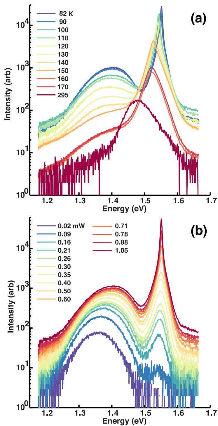
Figure 39: PL spectra for Sample A measured through the glass (front junction) side at (a) \sim 0.9 mW laser excitation power over a range of temperatures and (b) at 82 K as a function of laser power.
