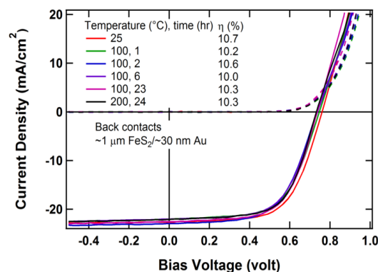
Figure 37. Stability of a CdTe solar cell with a sputtered absorber layer and a 1 \mu\text{m} \text{FeS}_2 back contact as measured under \text{N}_2 at 100°C for 23 hours, and at 200°C for one additional hour.
