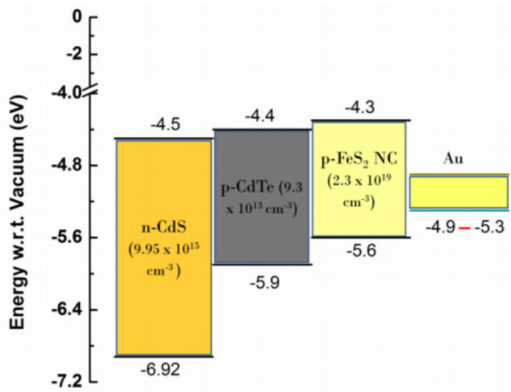
Figure 23. Non-interacting band diagram for the component layers of a CdTe solar cell structure with an FeS 2 back contact. The energy scale is plotted relative to the vacuum level indicated by 0 eV at the top.
