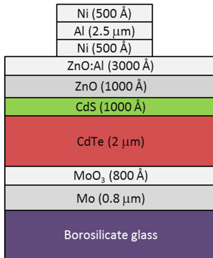
Figure 28. Layer stack for the CdTe thin film solar cell in the substrate configuration. All the layers other than \text{MoO}_3 and Ni/Al/Ni were deposited by sputtering. An 800 \text{\AA} layer of \text{MoO}_3 was deposited by atomic layer deposition (ALD) on Mo coated borosilicate glass and final metal contact layers (Ni/Al/Ni) were deposited by e-beam evaporation.
