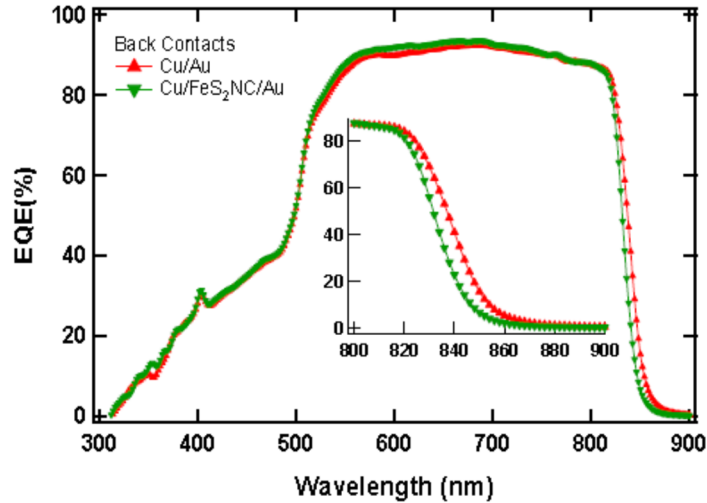
Figure 35. Typical external quantum efficiency (EQE) of cells before and after incorporation of FeS 2 NC as an interface layer for CSS deposited CdTe devices. The inset provides an expanded view in the CdTe bandgap region.
