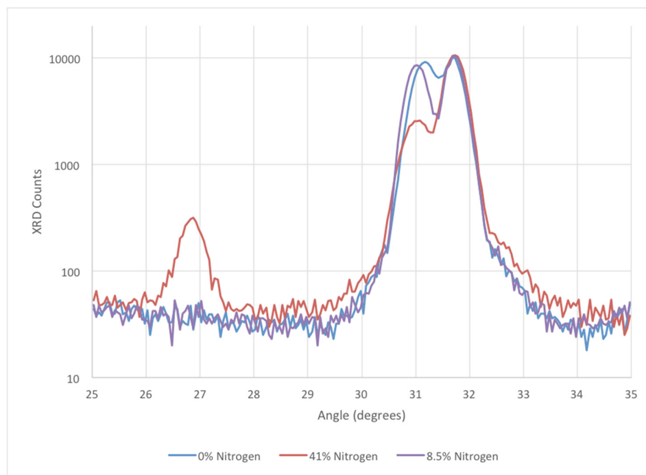
Figure 3: XRD scans for films grown on GaAs (100). The peak at 31.675^\circ is due to the GaAs (001) planes. The peak to the left at \sim 30.975^\circ is due to GaAs. The CIS film peak is located at 31.125^\circ for the film sputtered in pure Ar. There is probably not a true peak shift as N_2 is added. Rather the peak width is probably changing, resulting in more overlap. For higher N_2 partial pressures (eg: 41% in the sputtering gas) a secondary peak due to grains of different orientations begins to appear, indicating a partial transformation to polycrystalline material.
