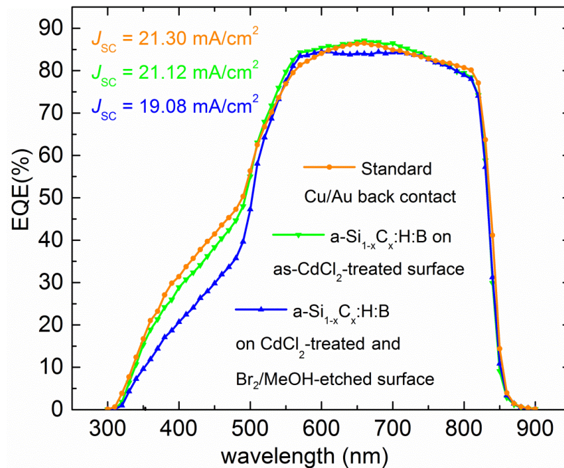
Figure 18. Quantum efficiency spectra are shown in the figure for two devices with a\text{-Si}_{1-x}\text{C}_x\text{:H:B/Cr} back contacts, with and without an etching step between the \text{CdCl}_2 treatment and back contact deposition (upright triangles, blue line; and inverted triangles green line, respectively). These measurements were performed one week after back contact deposition. These results are compared with a standard device having a \text{Cu/Au} back contact (circular points, orange line). The short circuit current values shown in the figure were calculated based on QE integrations.
