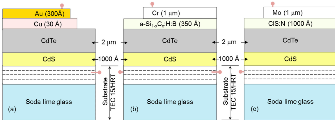
Figure 1. The schematic of device configuration is shown for (a) the standard CdTe solar cell with a Cu/Au back contact, (b) a CdTe cell with a novel p -type a-Si 1-x C x :H:B back contact and Cr as the final metal contact to define the cell area and (c) a CdTe cell with a novel p -type CIS:N back contact and Mo as the final metal contact to define the cell area. The layers beneath the CdS are the coatings of the TEC-15/HRT superstrate.
