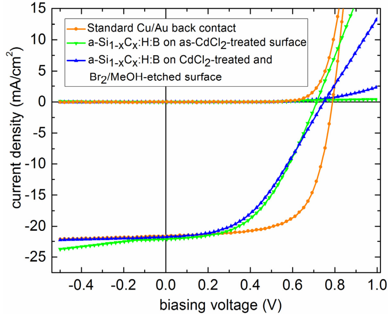
Figure 17. Light and dark J - V curves have been compared for CdTe solar cells with a-Si 1-x C x :H:B/Cr back contacts and standard Cu/Au back contacts. The curves with inverted (green) and upright (blue) triangles are for cells with a-Si 1-x C x :H:B/Cr back contacts on as-CdCl 2 -treated and CdCl 2 -treated + Br 2 /methanol etched surfaces, respectively. The curve with the circular symbols (orange) describes a standard device. Devices with the novel back contacts show comparable V_{oc} and J_{sc} but reduced fill factor relative to standard devices.
