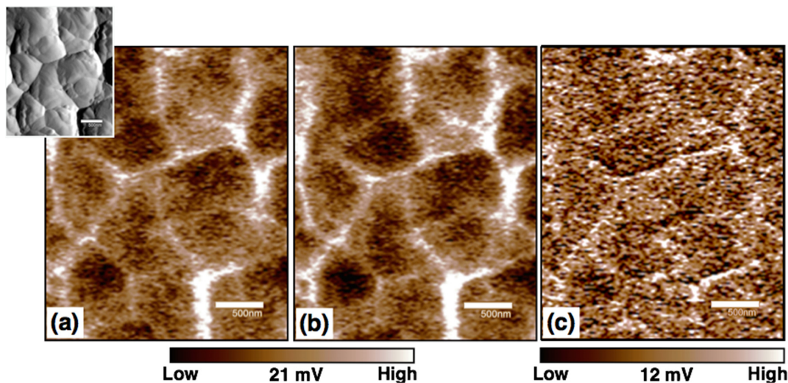
Figure 44: dC/dV data for a CdTe device sample measured with the illuminator (a) off and (b) on and (c) the difference in the two scans. The sample topography is shown in the insert.
