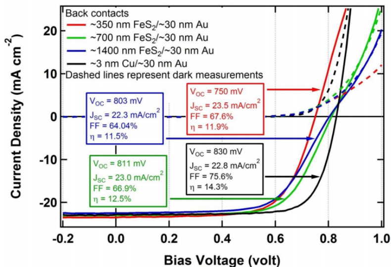
Figure 27. J-V characteristics -- light (solid lines) and dark (dotted lines) -- for devices with FeS 2 layer thicknesses ranging from 0.3 \mu m to 1.5 \mu m. Also shown in the diagram are the corresponding characteristics for a device with a standard Cu/Au back contact. These solar cells were fabricated with a CSS absorber layer.
