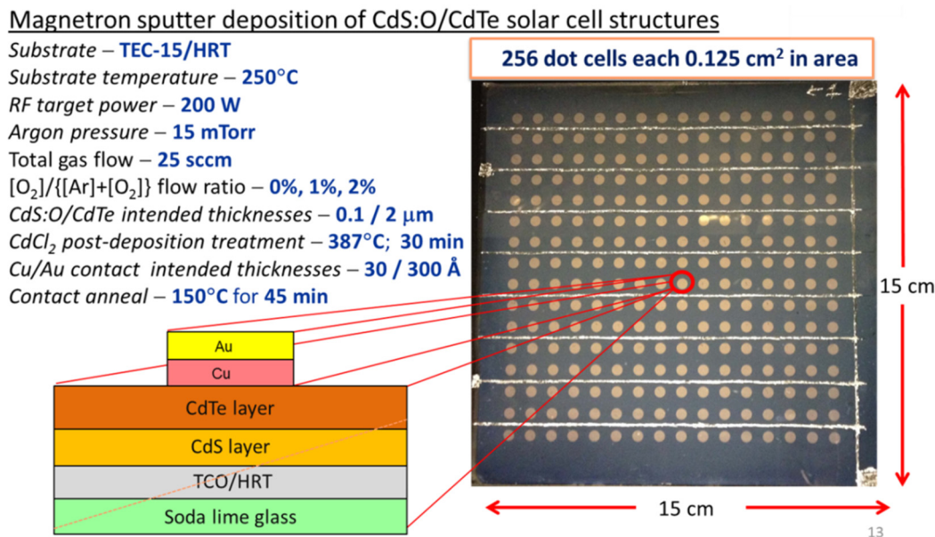
Figure 8. Fabrication conditions and standard layer structure for CdTe solar cells incorporating CdS 1-x O x for different flow ratios of [O_2]/\{[O_2] + [Ar]\} during reactive sputtering.
