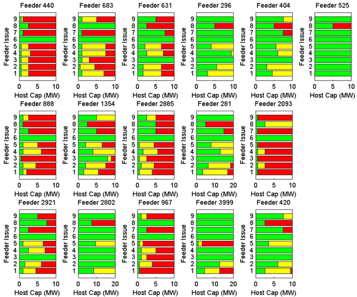
Figure 2-3 Detailed Hosting Capacity Assessment of 16 Feeders from CSI3 17,18
