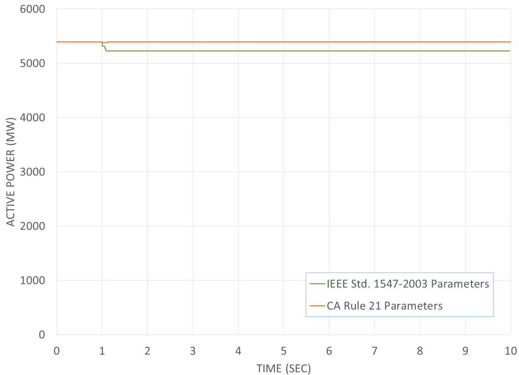
Figure 5-14 Active power output from DER PV in California.
