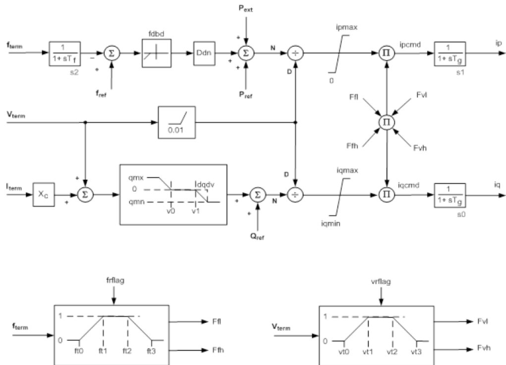
Figure 5-2 The block diagram for the PVD1 model. Source: GE PSLF User Manual.
