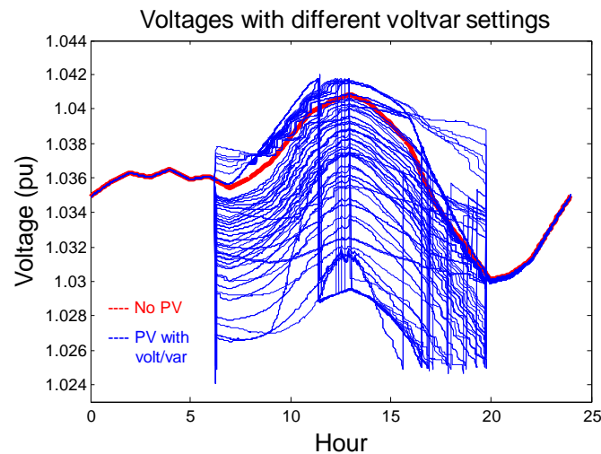
Figure 3-15 Sample Illustration of Sudden Change In Voltage with Onset of PV Connection 25
