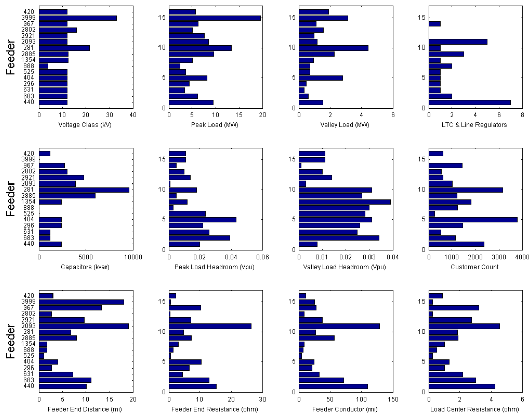
Figure 2-2. Characteristics of Analyzed Feeders in Previous CSI Project
