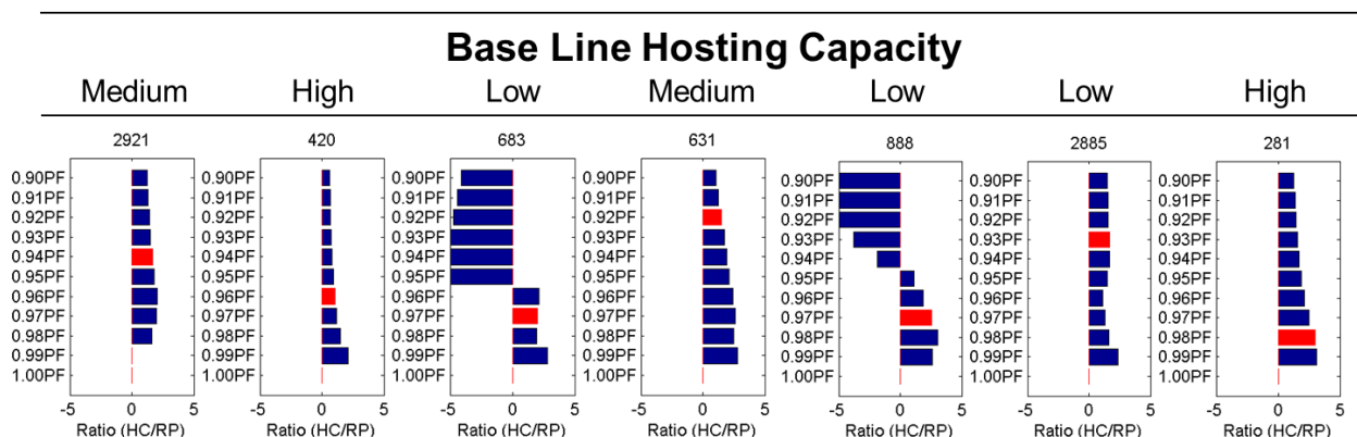
Figure 4-10 Ratio of Change in Hosting Capacity to Change in Reactive Power for Power Factor Brute Force Analysis (Level 1 Power Factor Settings are Highlighted in Red)
