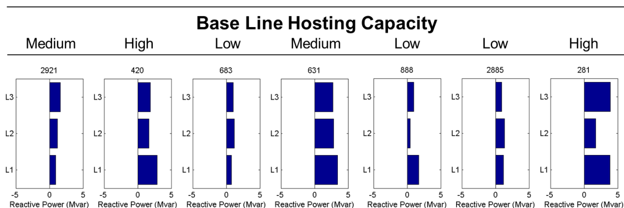
Figure 4-7 Change in Reactive Power – Power Factor
