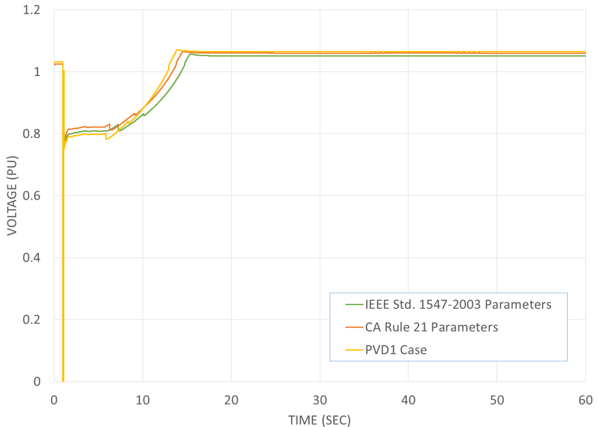
Figure 5-26 Voltage at the 115 kV sub-transmission bus for the three DER PV cases.
