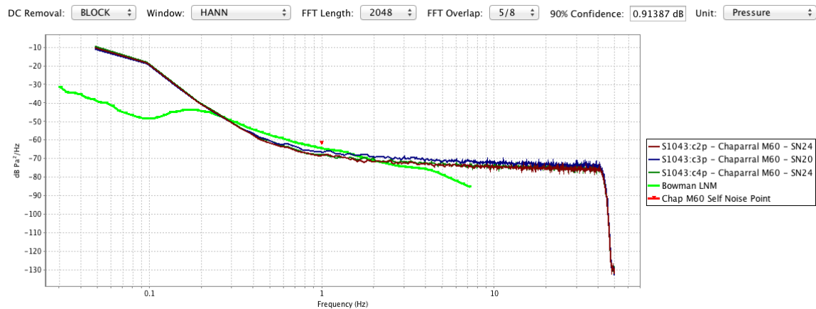
Figure 19 Pressure power spectra due to ground motion during seismic excitation
