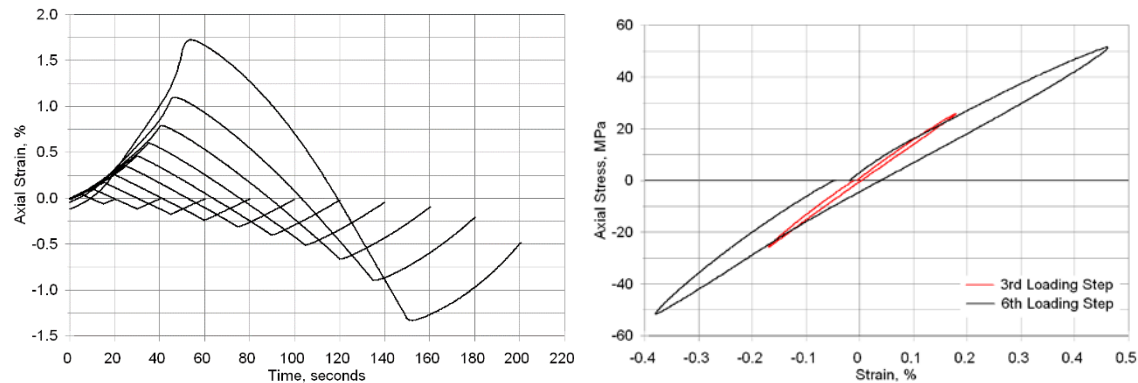
Figure 31. Reversed loading LUR results; left: strain vs. time at each loading step; right: stress-strain loops at the third ( \pm 25.8 MPa) and sixth ( \pm 51.6 MPa) steps.
