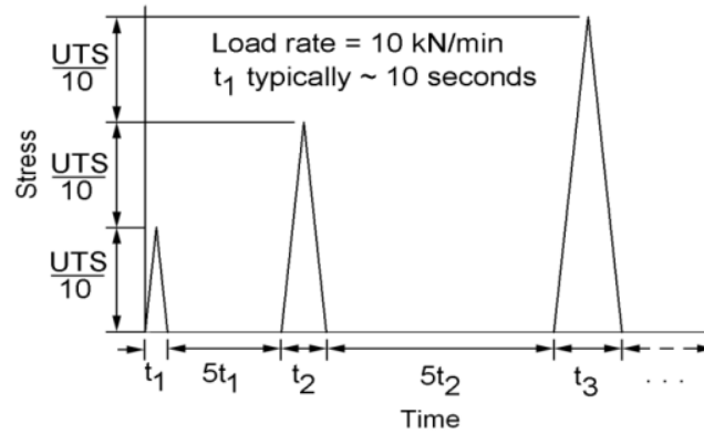
Figure 16. LUR tension test sequence with loading to successively higher loads.
