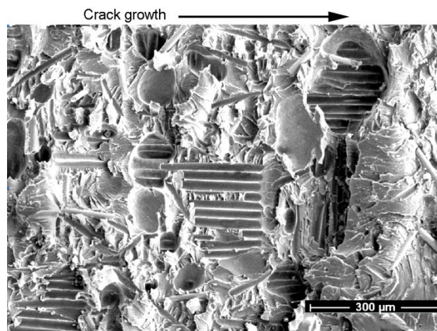
Figure 80. Path B showing fracture through pores over peel ply and through adhesive, ADH-1, static test, looking toward laminate side.
