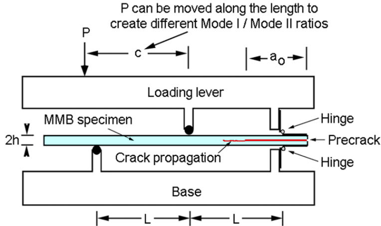
Figure 21. Mixed mode bending apparatus (MMB).
