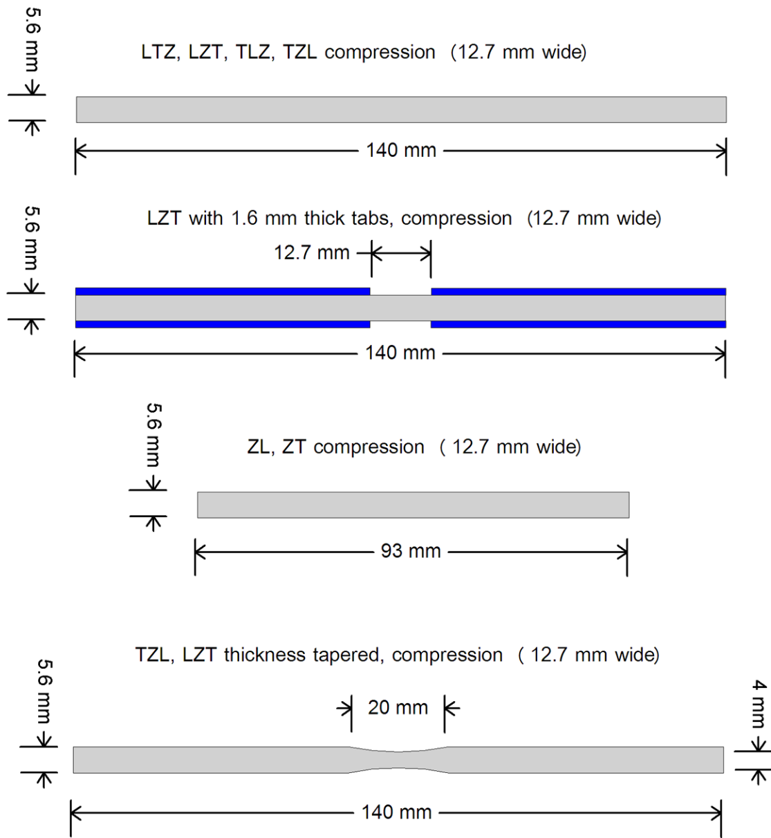
Figure 15(b). Compression coupon geometries (ASTM D6641)
