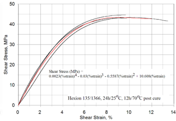
(28u) Neat resin shear
