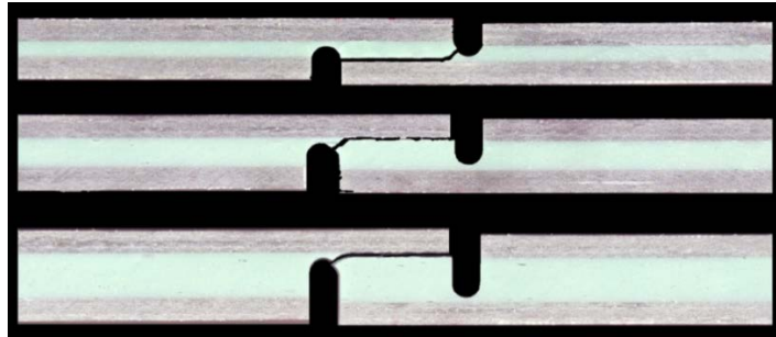
Figure 72. Failed coupons with 3.25, 6.50 and 9.75 mm thick adhesive layers, ADH-1, 25.4 mm overlap length [2].
