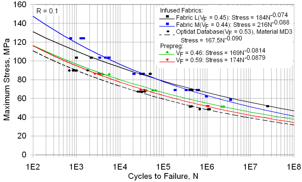
Figure 8. Comparison of literature data [1, 22] for DB glass/epoxy infused and prepreg blade laminates in tensile fatigue, R = 0.1.
