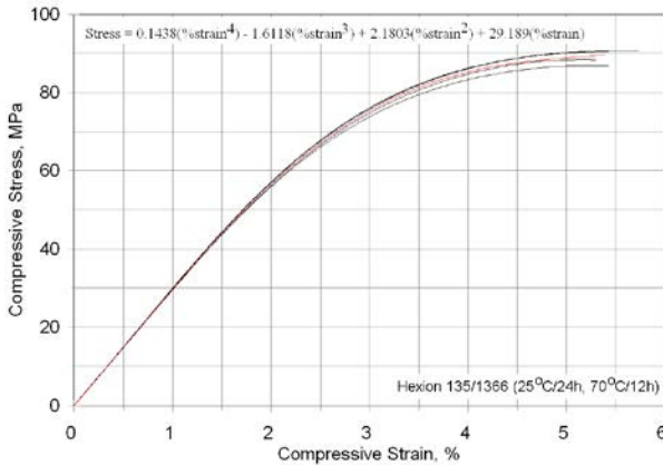
(28t) Neat resin compression
