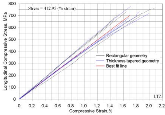
(28g) Long. compression, LTZ orientation
