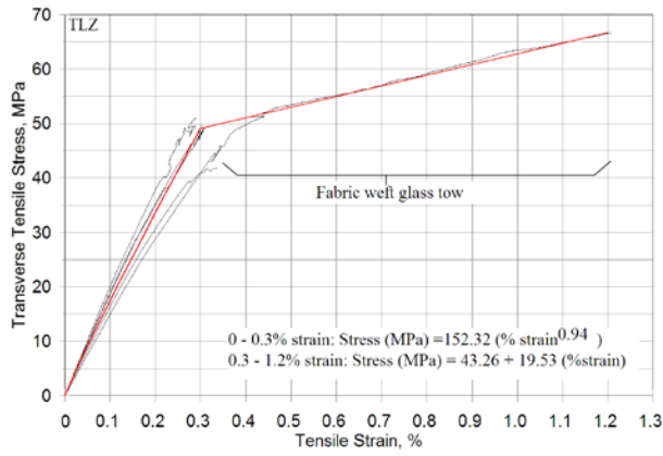
(28c) Transverse tension, TLZ orientation
