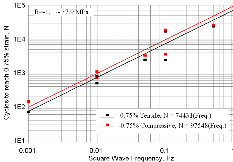
Figure 67. From Figure 66, plot of cycles to reach a strain of 0.75% (where damage becomes prevalent) vs. square wave frequency.
