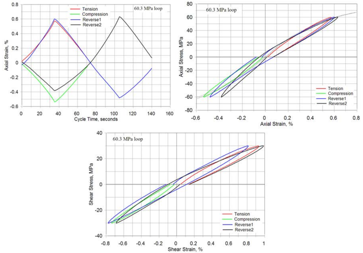
Figure 35(g). 60.3 MPa
