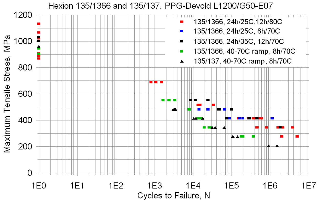
Figure 44. Tensile fatigue data for UD laminates, fabric H with 135/1366 or 135/137 epoxies with different cure and post-cure conditions shown, R = 0.1
