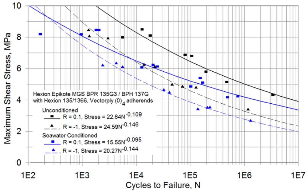
Figure 104. Notched lap shear adhesive joint coupons (Fig. 23), dry control and seawater conditioned tensile and reversed loading fatigue data.
