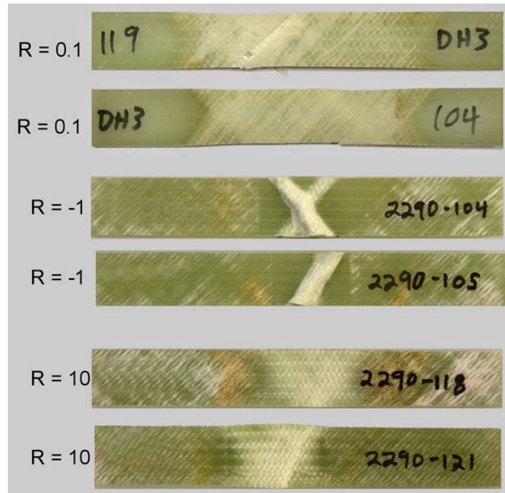
Figure 49. Failed fatigue coupons at indicated R-values, fabric P laminates.
