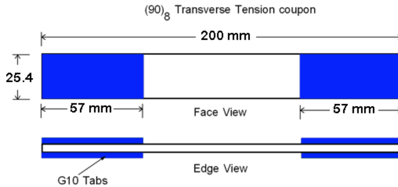
Transverse Tension Coupon Construction
