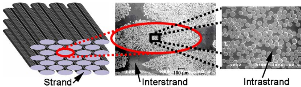
Figure 2. Exploded view of low density fabric A composite showing strand packing, inter-strand channels and intra-strand structure with individual glass fiber packing evident [2].
