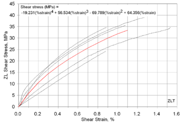
(28q) ZL shear direction, ZLT orientation
