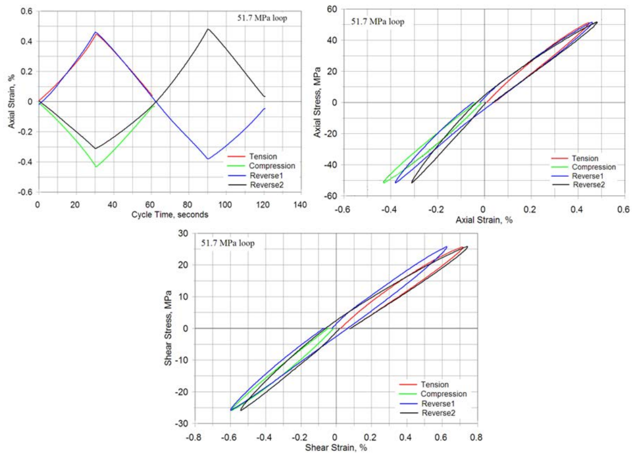
Figure 35(f). 51.7 MPa
