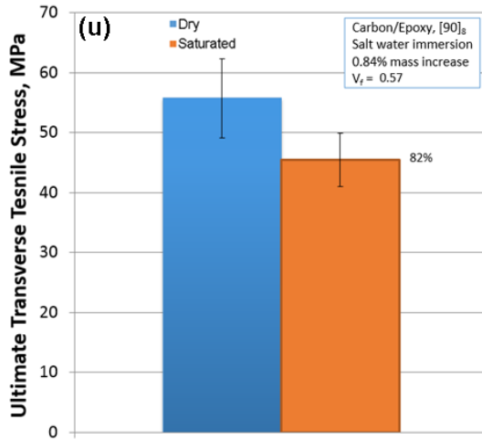
Figure 97 (s)-(v). Static environmental test data
