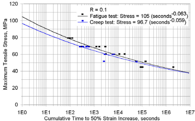
Figure 62. Cumulative test time to reach 50% increase in max strain at different max stresses for tensile creep loading, compared with sine-wave fatigue at R = 0.1 .
