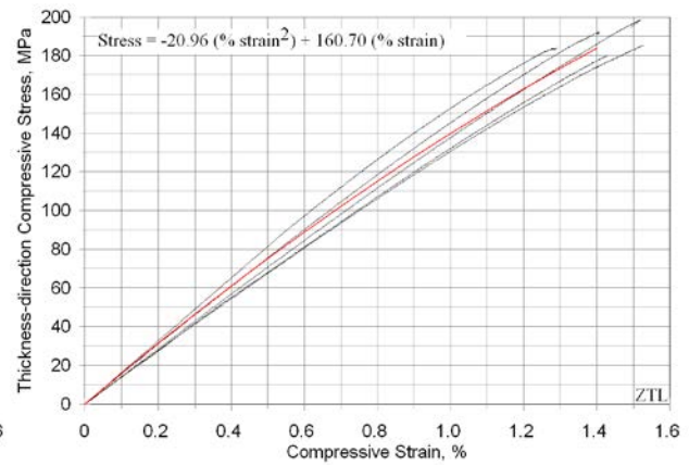
(28l) Thick dir. compression, ZTL orientation
