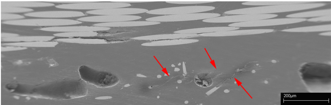
Figure 76. SEM micrographs of crack tip area, static CLS specimens with adhesive ADH-1, crack path B, crack growth left to right: fully cracked, partial shear displacement (top, crack 1a); mostly cracked (middle, crack 1b); and local micro-cracking at arrows ahead of tip at fibers and pores (bottom, crack 1a).
