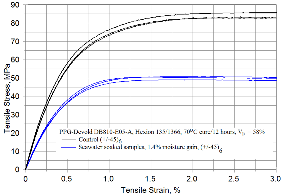
Figure 100. Tensile stress-strain curves for control and seawater saturated \pm 45^\circ DB coupons from Fig. 97(b).
