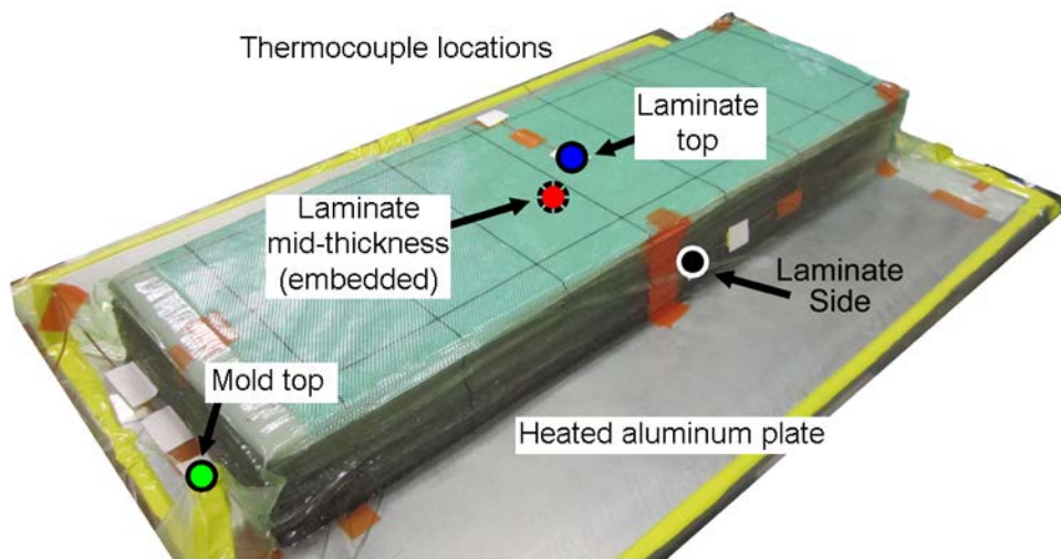
Figure 11. Laminate infusion photograph and temperature traces during cure and post-cure from thermocouples at the indicated positions for the 80-ply laminate.
