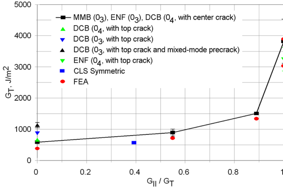
Figure 86. Mixed mode bending static test results for crack growth resistance of 2.4 mm thick ADH-1 adhesive joints: modified beam theory calculations (Eq. 2-7), comparison to FEA calculations from VCCT. Legend indicates laminate adherend thickness: (0) 3 , three plies, (0) 4 , four plies, starter crack at the top interface in Fig. 1, or center of adhesive (DCB); or MMB starter crack for DCB case.
