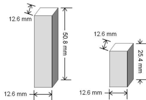
ASTM D695 Compression test geometries
