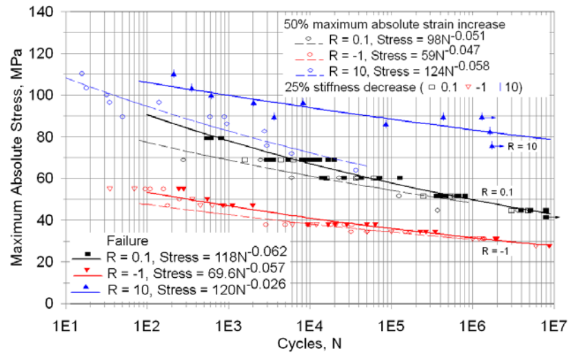
Figure 56. Data for 25% stiffness decrease and 50% max absolute strain increase plotted with failure S-N curves.
