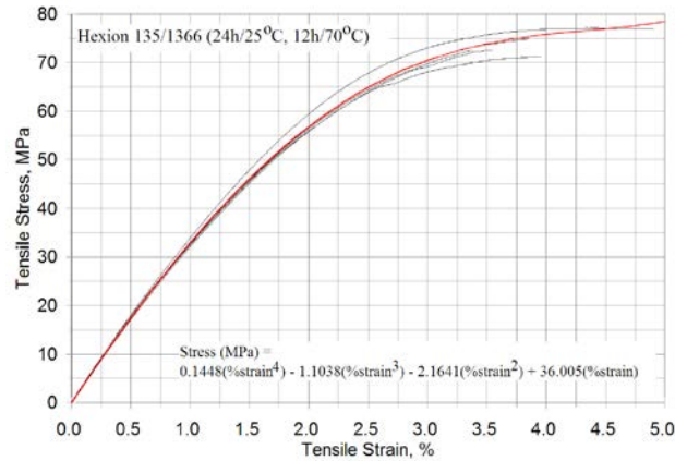
(28s) Neat resin tension
