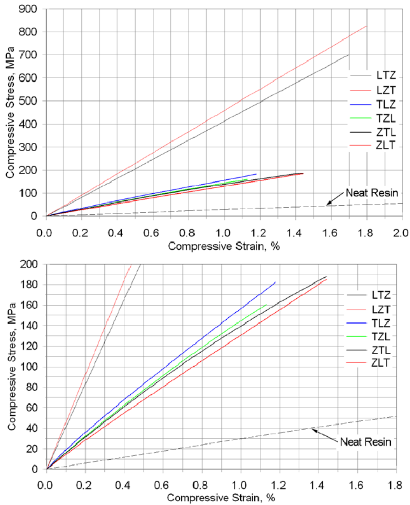
Figure 26b. Compression Best Fit Stress-Strain Curves (Two Scales)
