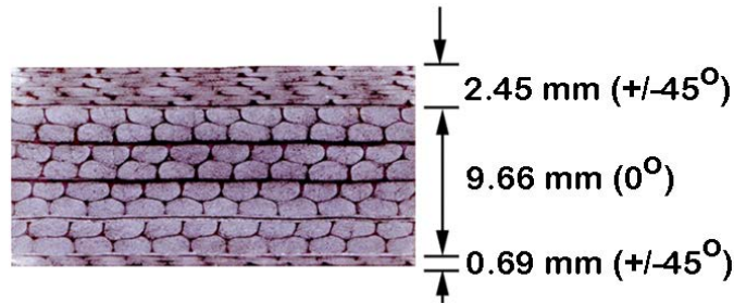
Figure 3. Infusion processed laminate with outer \pm 45^\circ ply stacks sandwiching eight 0^\circ UD plies (high fiber density fabric D [1]), where individual unidirectional (UD) plies are stacked back-to-back in pairs, and showing in-situ nesting of strands.
