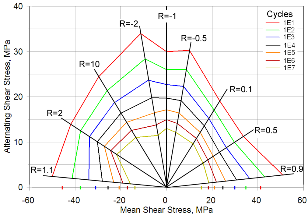
Figure 59(b). Shear Stress
