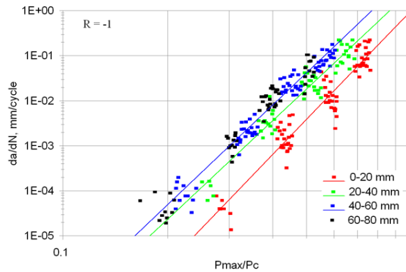
(c) Long CLS with steel, R = -1
