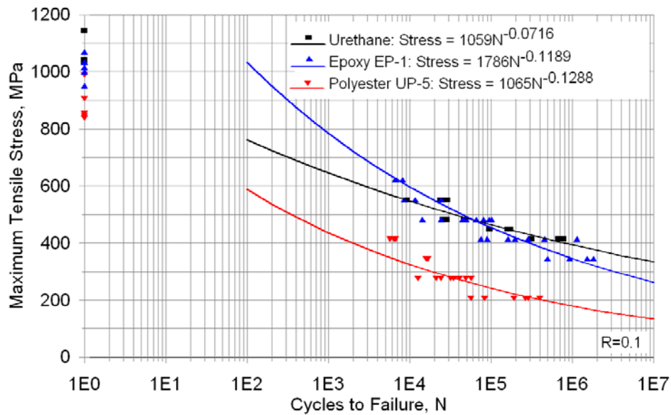
Figure 39. Comparison of tensile fatigue (R = 0.1) S-N trends for fiber dominated unidirectional ( 0^\circ ) urethane, epoxy (EP-1) and polyester (UP-5) resin laminates.
