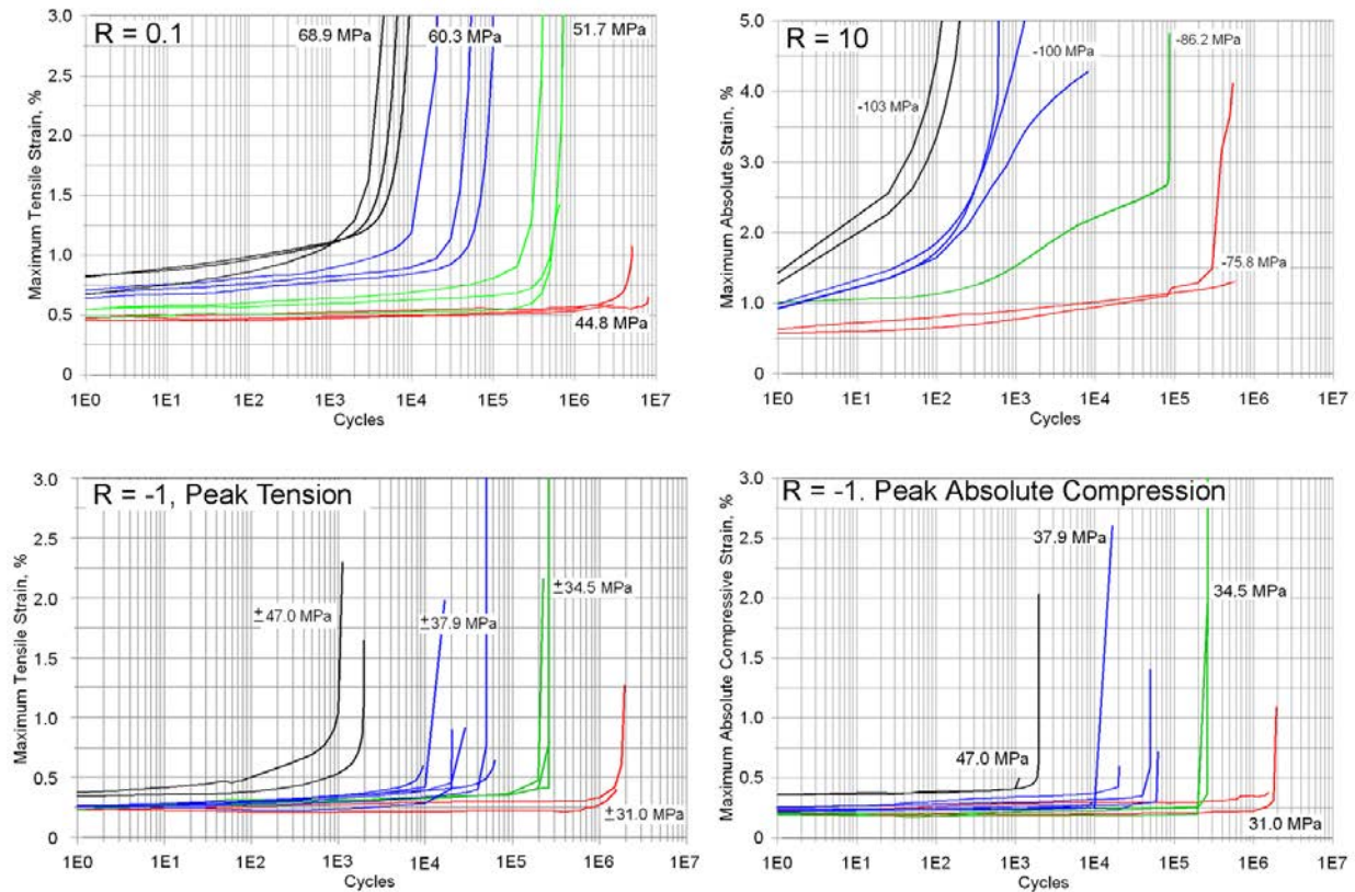
Figure 54. Maximum running strain over lifetime at different max loads: R = 0.1 (top left), 10 (top right) and -1 (bottom: left, tension part of cycle; right, compression part).
