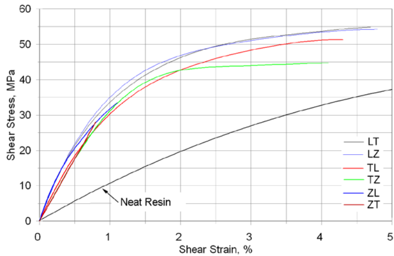
Figure 26c. Shear Best Fit Stress-Strain Curves
