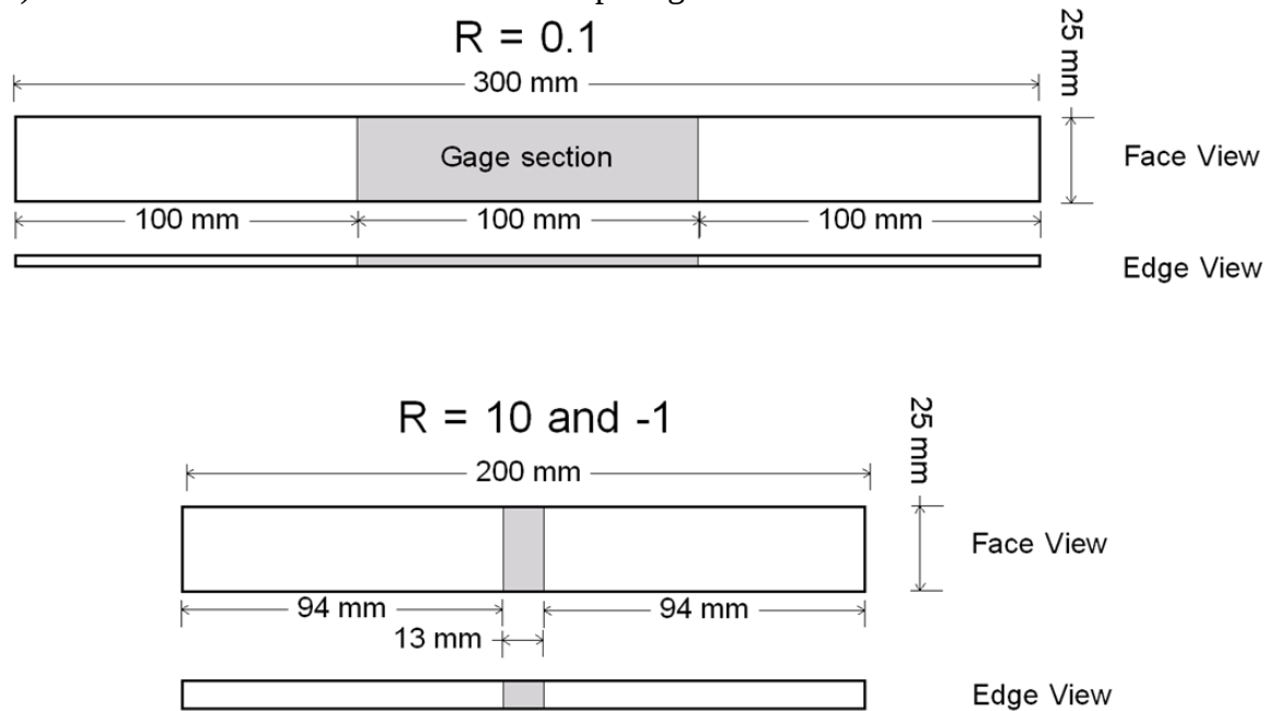
Figure 17. Standard tension static and fatigue (top, 1.7-mm thickness) and static compression and R = 10 and -1 fatigue coupons ( [0]_6 , 5.2-mm thickness) for UD laminates (fabric H/epoxy EP-1).
