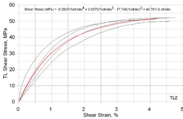
(28o) TL shear direction, TLZ orientation
