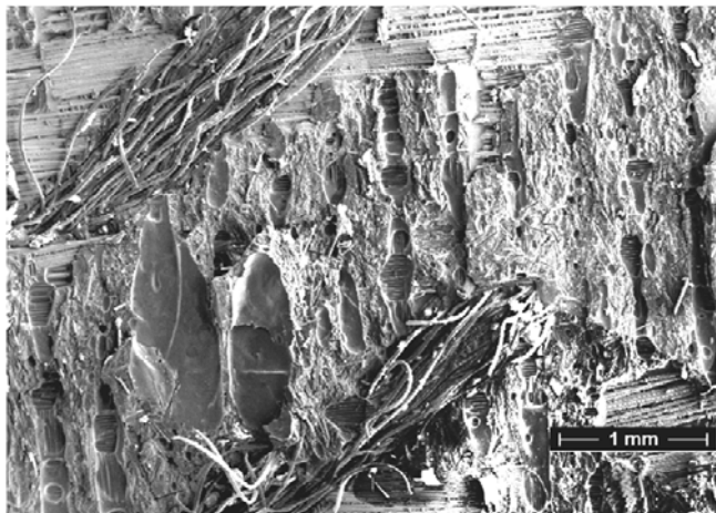
Figure 84. Low magnification reversed loading fracture surface looking toward laminate side, showing transitional characteristics of crack paths B (patches of fractured adhesive) and C (growth along glass strand surface inside laminate, also showing polyester fabric stitching), crack growth left to right, ADH-1, R = 0.1 , CLS test.
