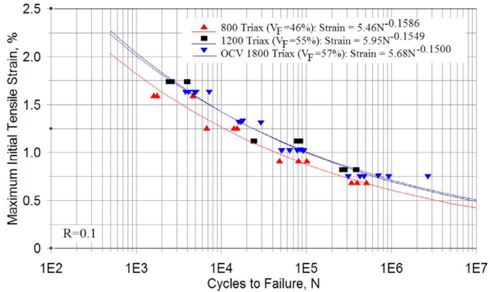
Figure 43. Strain vs. cycles to fail for triax fabric laminates with two Saertex fabrics (800 and 1200 gsm) and a heavier OCV™ fabric (1800 gsm), epoxy EP1, R = 0.1.
