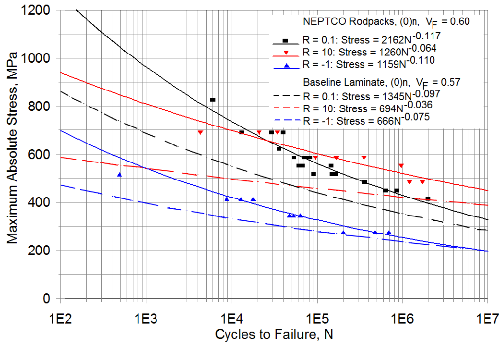
Figure 45. Maximum absolute stress versus cycles to failure, RodPack versus baseline laminates.
