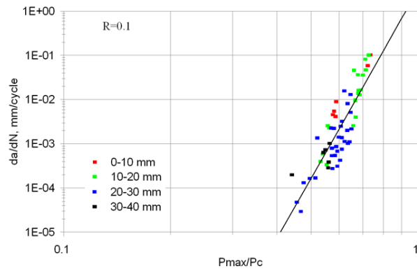
(b) Short CLS, no steel, R = 0.1
