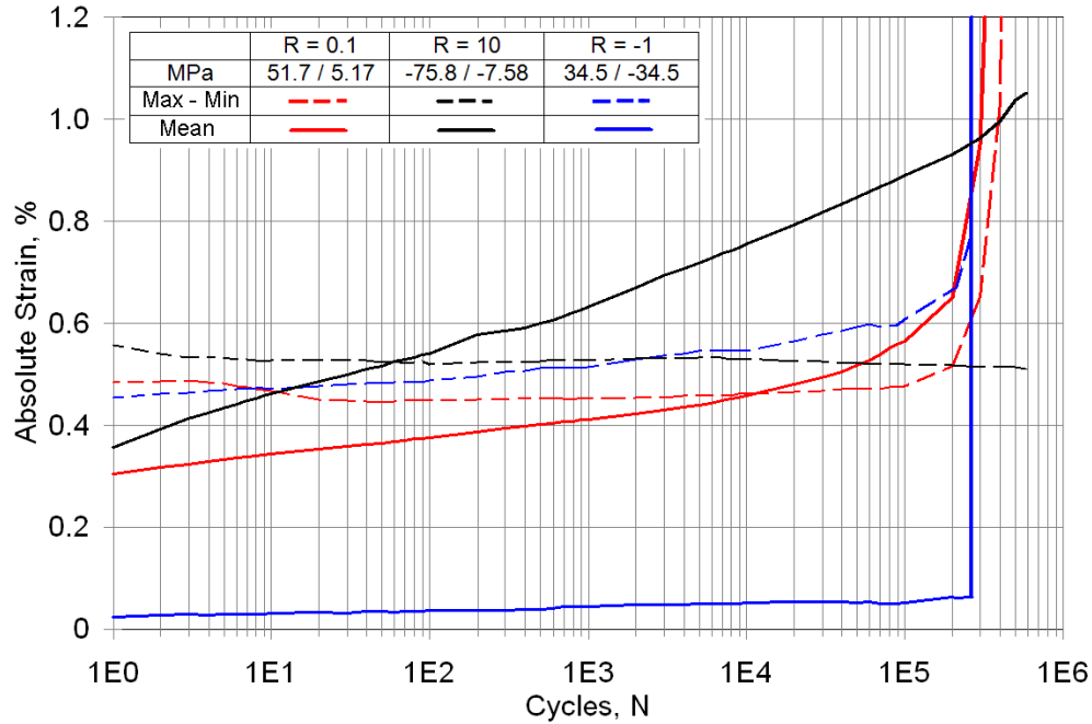
Figure 55. Typical individual test average strain, (\max + \min)/2 , and strain range (\max - \min) at each R-value.
