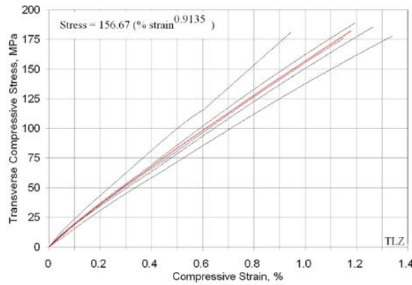
(28i) Transverse compression, TLZ orientation
