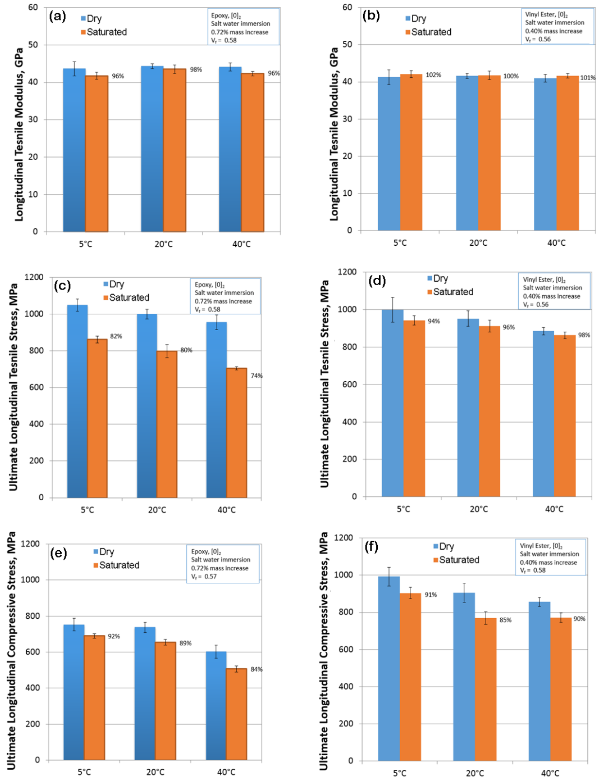
Figure 97 (a)-(f). Static environmental test data
