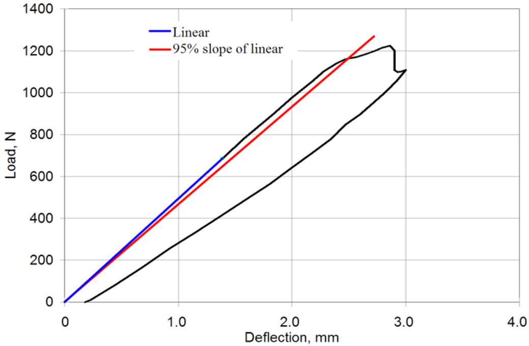
Figure 20. Typical load versus actuator displacement curve and critical load determination for an MMB specimen.
