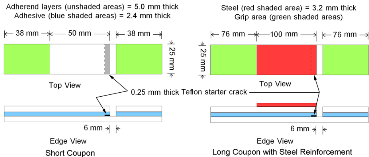
Figure 18(a). Coupon dimensions: left, short coupon with 50 mm gage length; right, 100 mm length specimen showing added steel reinforcement.
