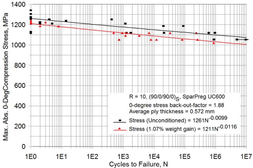
Figure 103. Compression fatigue data for SparPreg carbon/epoxy dry and seawater saturated UD laminates.
