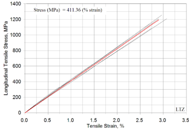
(28a) Longitudinal tension, LTZ orientation
