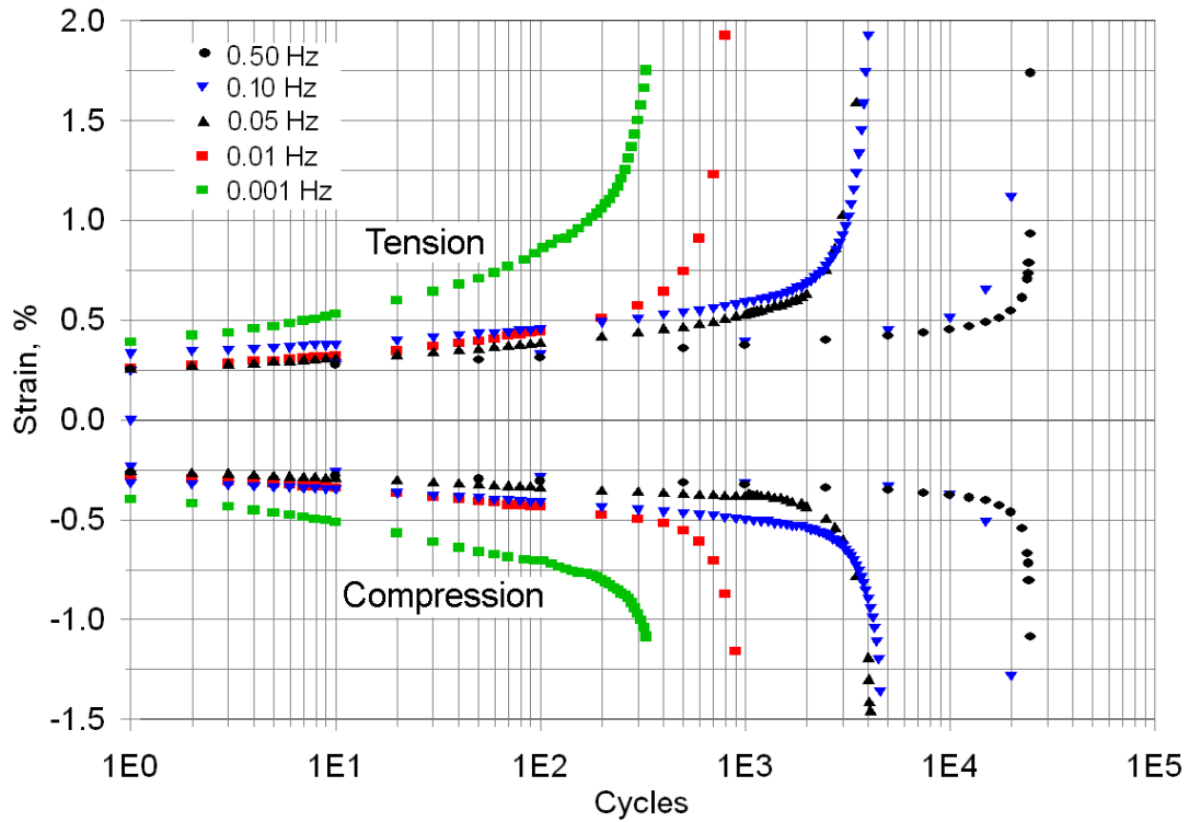
Figure 66. Data from Figure 65 plotted in terms of cycles rather than cumulative time.
