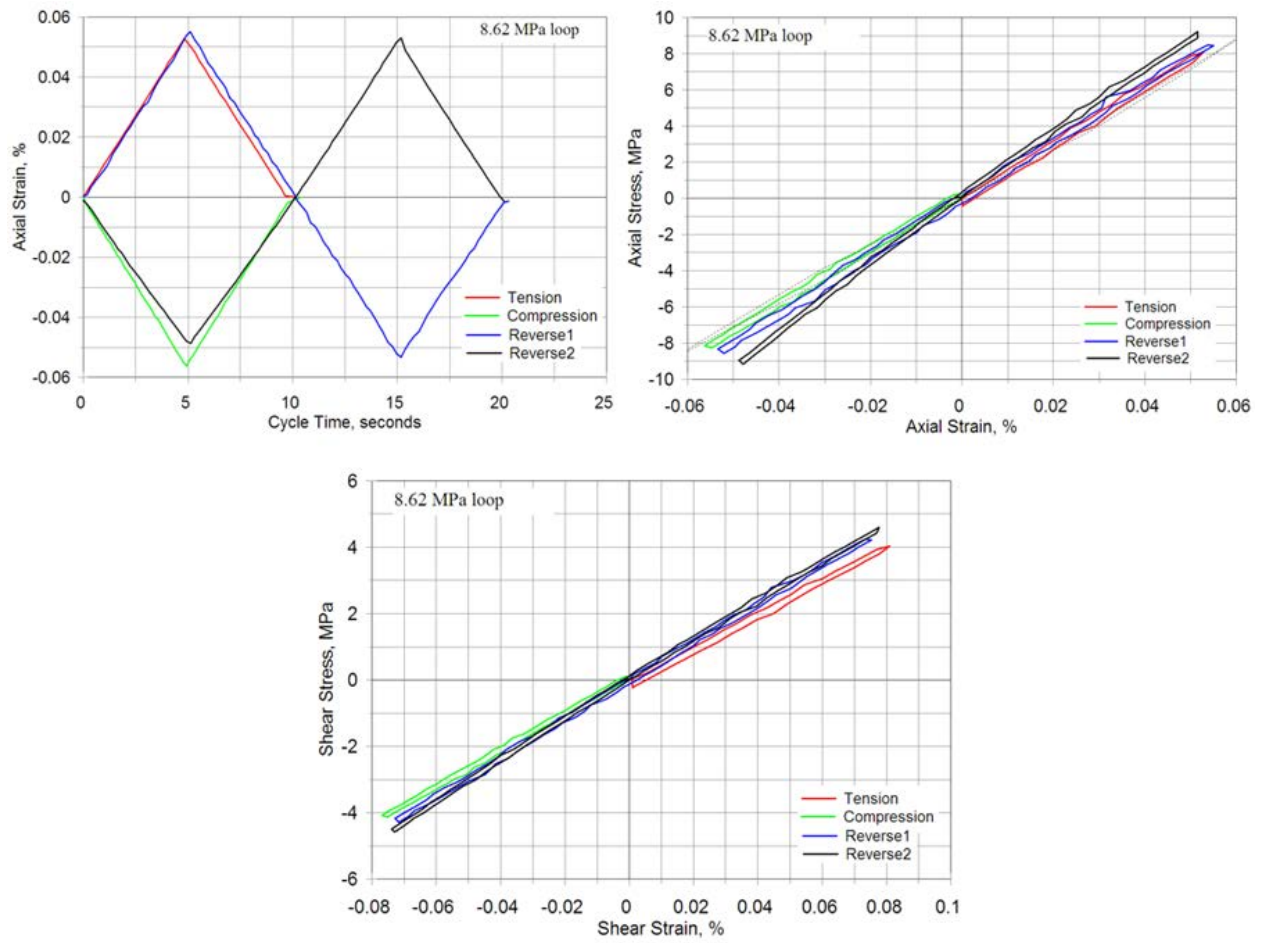
Figure 35(a). 8.62 MPa
