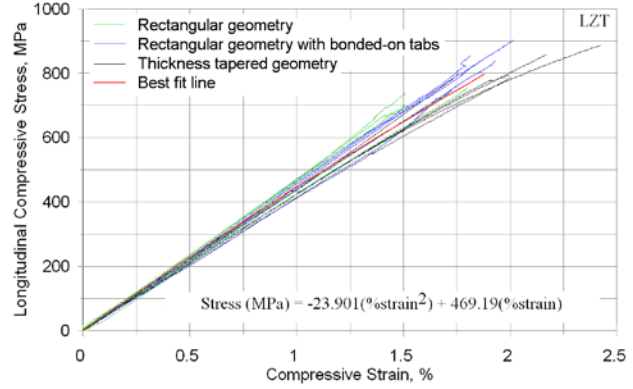
(28h) Long. compression, LZT orientation
