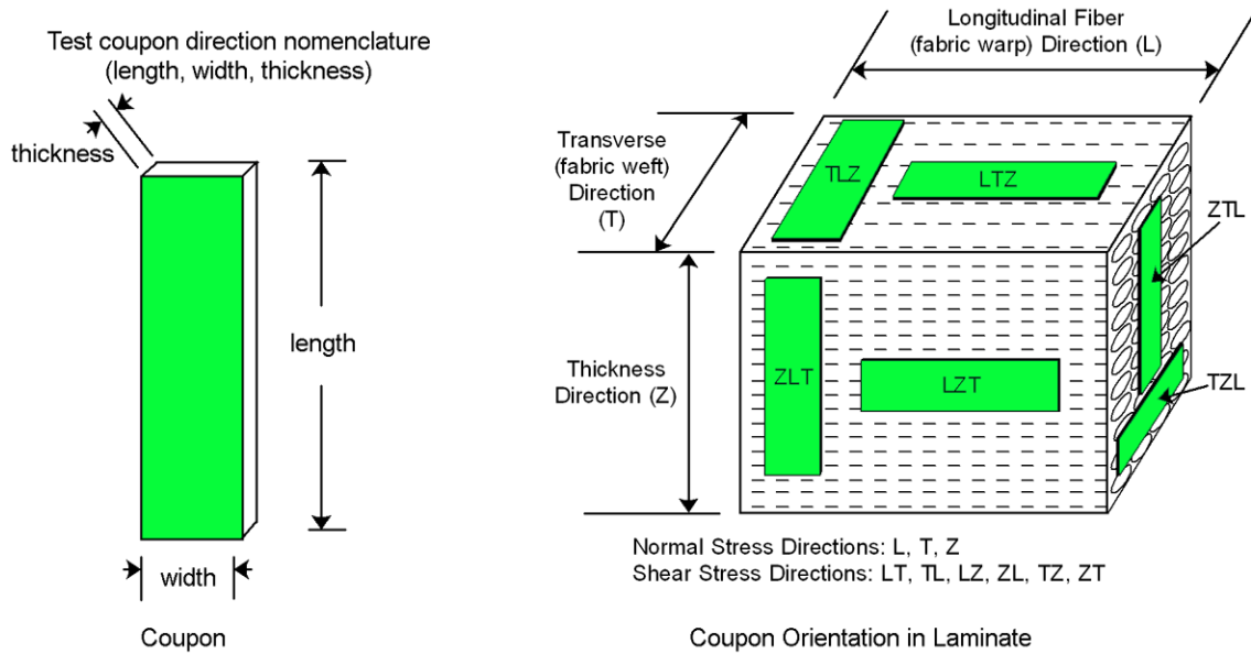
Figure 25. Coupon orientation indices and location in thick laminate.
