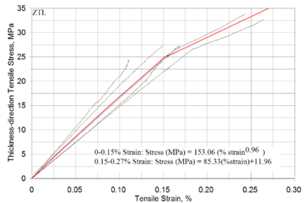
(28f) Thick dir. tension, ZTL orientation
