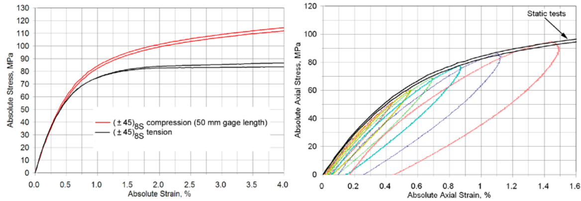
Figure 30. Comparison of typical \pm 45^\circ stress-strain curves in tension and compression (left); compression LUR results (right).
