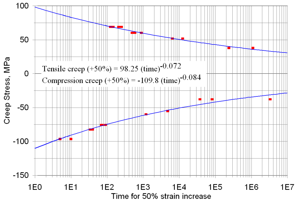
Figure 60. Creep trends from curve fits to tensile and compressive creep data for strain vs. time at various applied constant stress levels (0-stress amplitude), creep stress vs. cumulative time to 50% strain increase.
