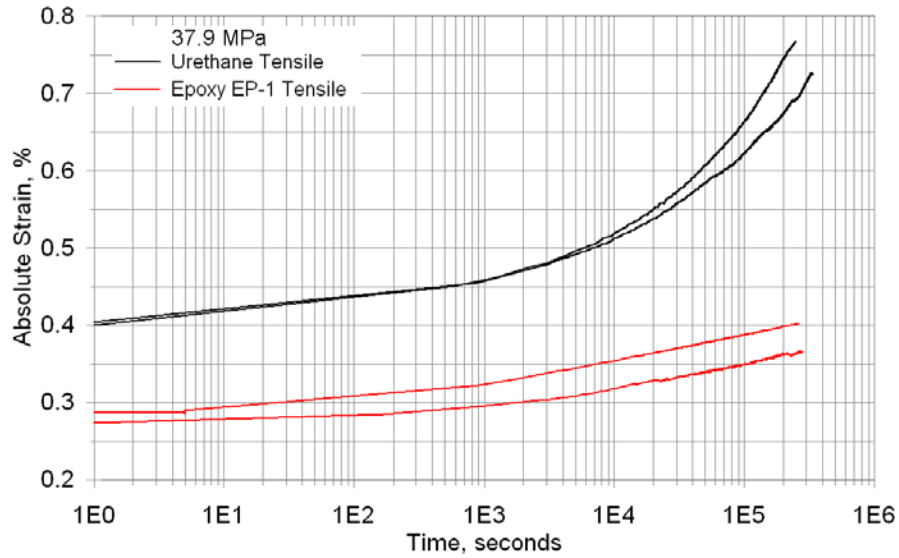
Figure 69. Comparison of creep strain vs. time curves for \pm 45^\circ laminates with urethane and epoxy EP-1 resins at 37.9 MPa constant applied tensile stress.
