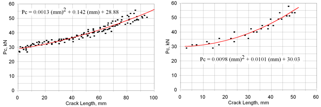
Figure 87. Static critical load vs. crack length, (a) 100 mm CLS with steel (left) and (b) 50 mm without steel, (right); adhesive ADH-1, crack growth from machined notch.
