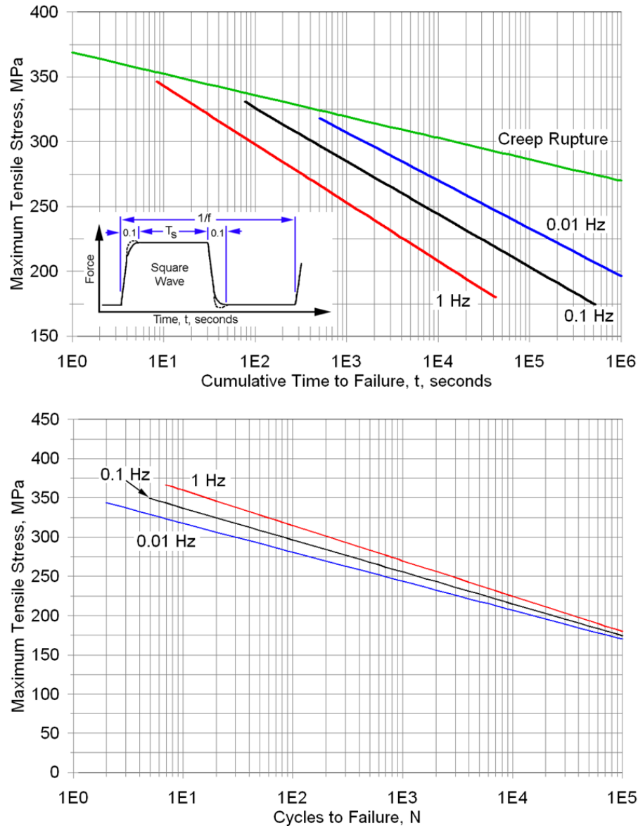
Figure 7. Creep rupture and tensile fatigue trends plotted in terms of cumulative time under load (top) and fatigue cycles (bottom); square wave loading at three frequencies, 0/90 glass/epoxy prepreg laminate (replotted from ref. [28]).
