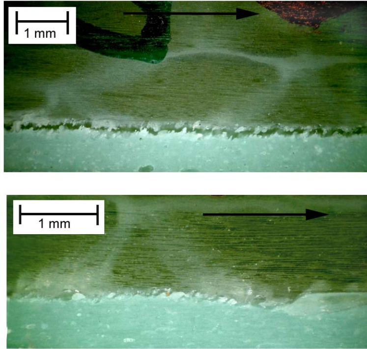
Figure 77. Optical micrographs of static crack paths with laminate strand and stitching visible on top, adhesive on bottom: ENF specimen, path B, crack growth left to right (top) and CLS specimen with steel showing transition from path B to path C on right end, crack growth left to right (bottom); adhesive ADH-1.
