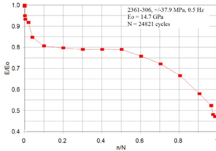
Figure 64. Decrease in modulus ( E/E_0 ) of the square wave loading vs. the cycles relative to total coupon lifetime ( n/N ) at \pm 37.9 MPa and 0.5 Hz.
