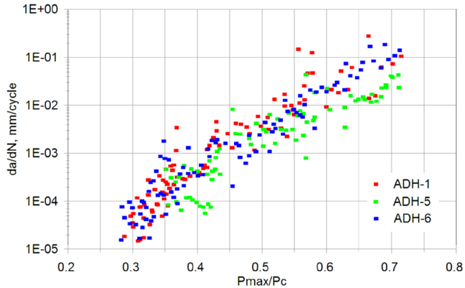
Figure 92. Comparison of reversed loading fatigue crack growth rates for three adhesives (short CLS specimen, no steel, 3.8 mm adhesive thickness).
