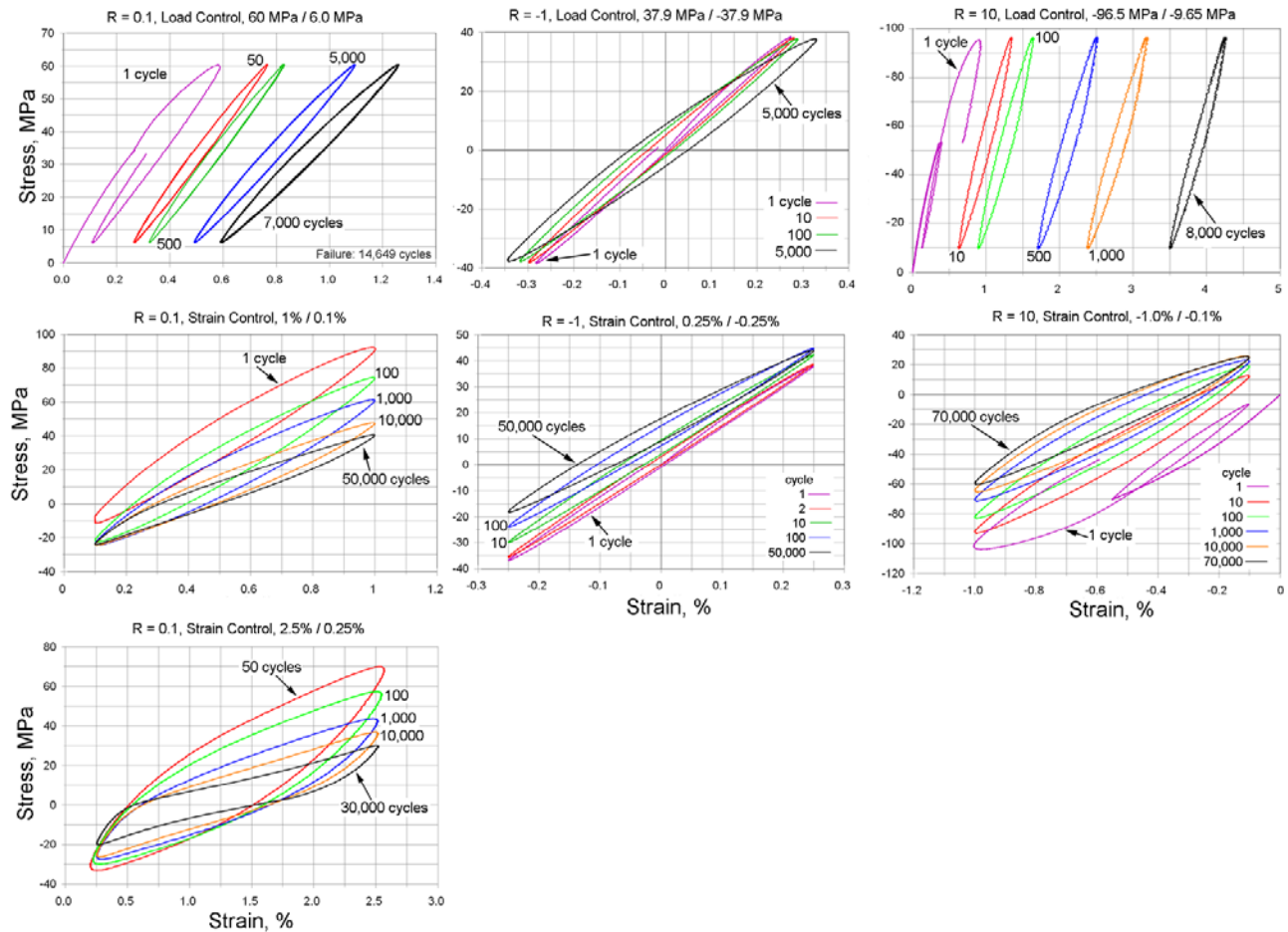
Figure 53. Typical cyclic stress-strain hysteresis loops for load control (top) and strain control (middle and bottom), fabric P, strain based R = 0.1 (left), -1 (center) and 10 (right).
