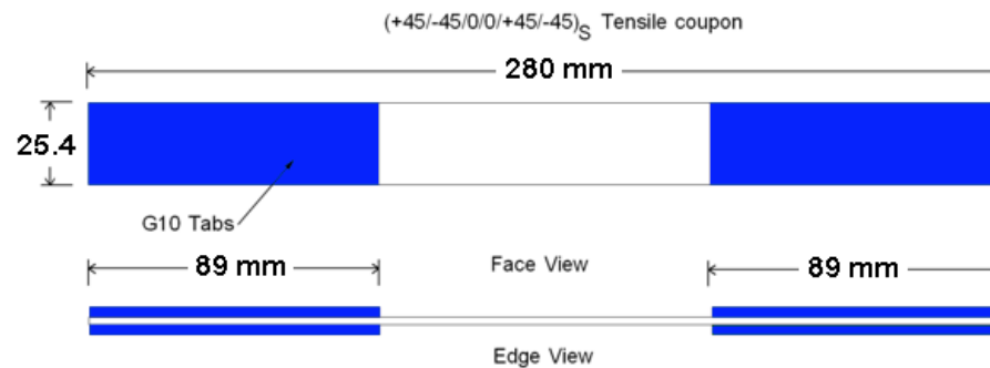
Spar Cap Tensile Coupon Construction
