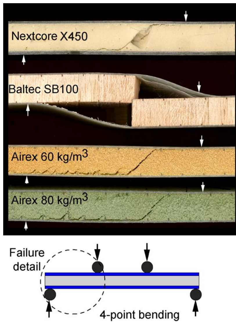
Figure 95. Failure modes for four core materials.
