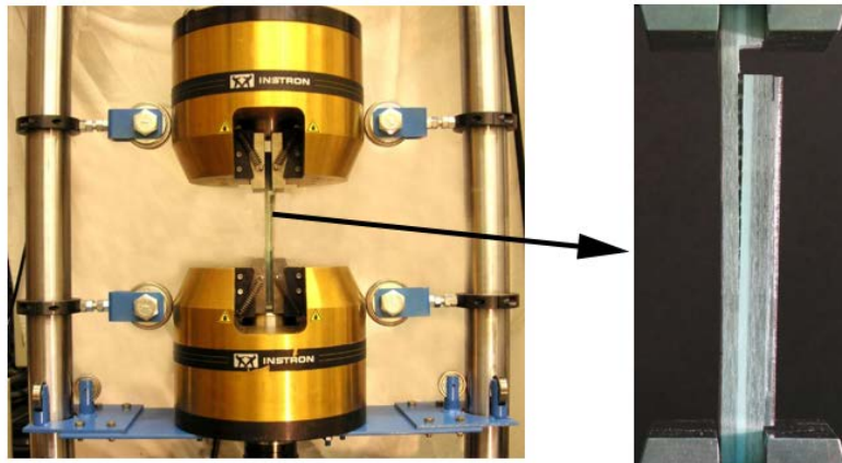
Figure 18(b). Test set-up with long specimen shown under load.
