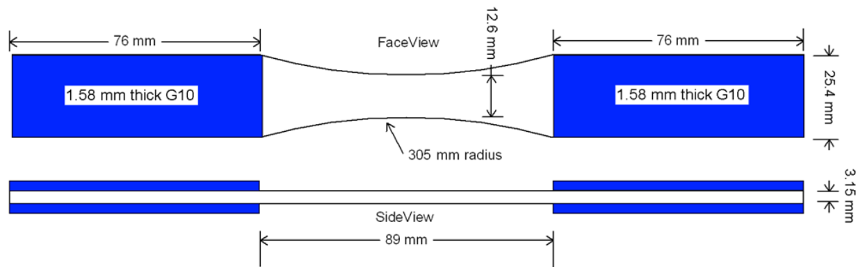
ASTM D638 Tensile test geometry (variation)
