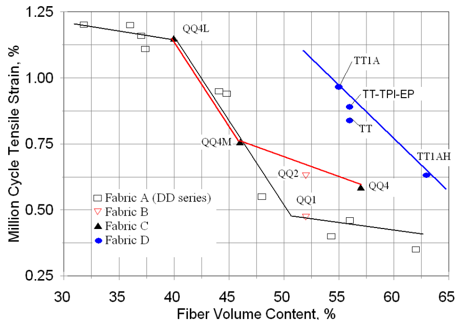
Figure 6. Million cycle strain vs. fiber volume content for various VARTM laminates and one SCRIMP laminate (TT-TPI-EP) showing transitions to reduced fatigue resistance as a function of 0^\circ fabric, R = 0.1 [1,2].
