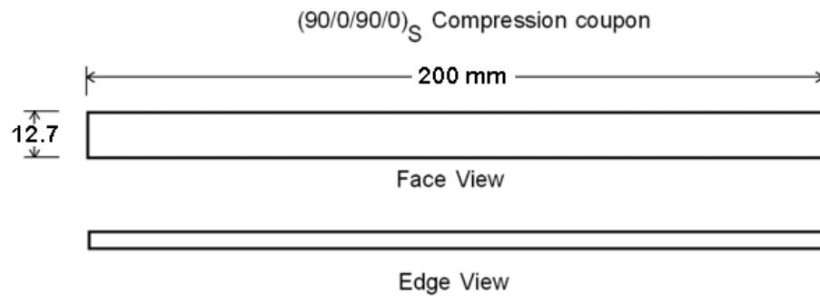
Compressive Coupon Construction
