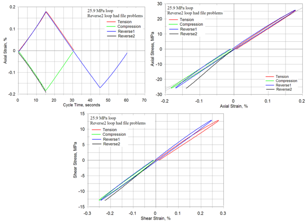
Figure35(c). 25.9 MPa
