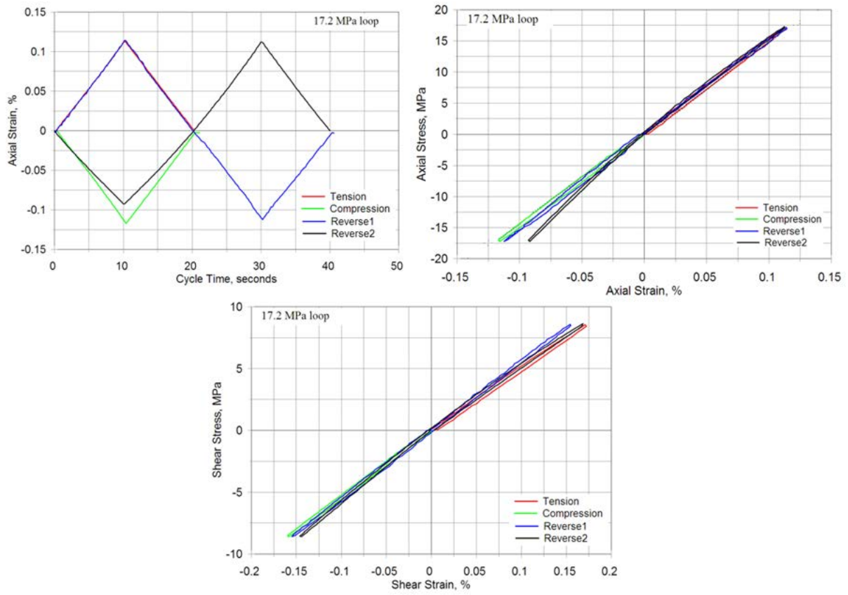
Figure 35(b). 17.2 MPa
