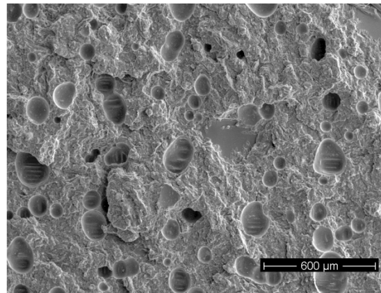
Figure 83. Crack Path A, cohesive near the interface, showing transition to path C (left), crack growth left to right, static CLS test with adhesive ADH-6.
