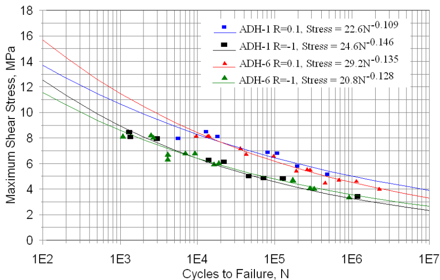
Figure 73. Tensile and Reversed Loading Fatigue S-N data for Two Blade Adhesives, Notched Lap Shear Coupon [2].
