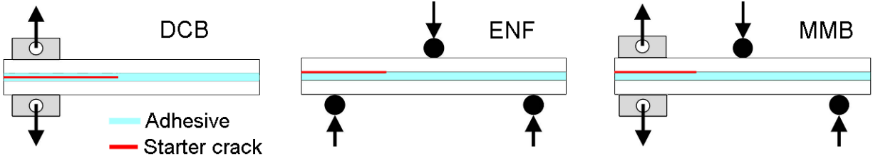
Figure 19. Flexural test geometries showing starter crack positions in adhesive: DCB, center or top; ENF, top; MMB, top.
