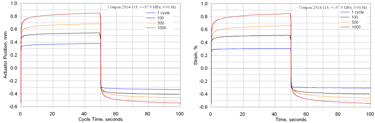
Figure 63. Typical square wave actuator position and extensometer axial strain for selected individual cycles; R = -1 , frequency 0.01 Hz.
