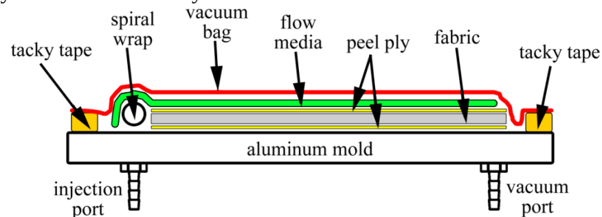
Figure 12. Schematic of the resin infusion process
