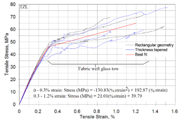
(28d) Transverse tension, TZL orientation
