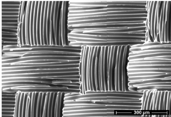
Figure 79. Laminate peel-ply surface as-molded.
