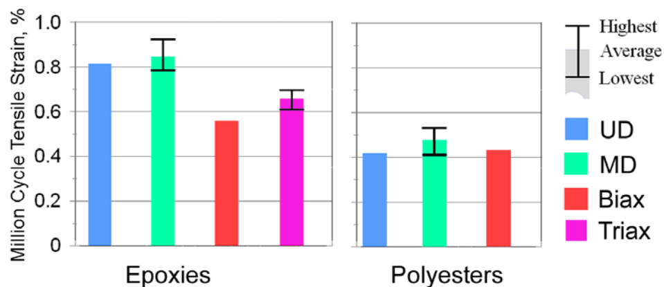
Figure 36. Comparison of million cycle fatigue strains for typical EP and UP resin laminates.
