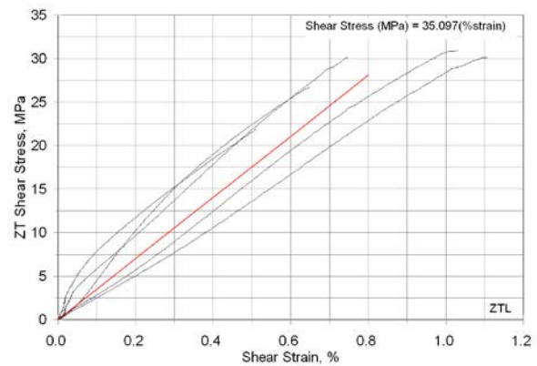
(28r) ZT shear direction, ZTL orientation
