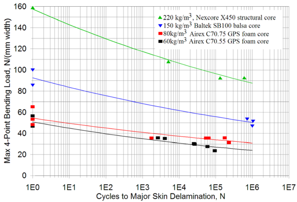
Figure 96. Flexural fatigue S-N data for sandwich panels with four core materials.
