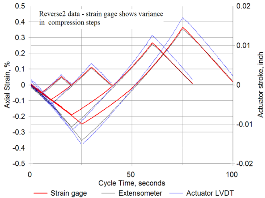
Figure 33. Reverse2 LUR results .
