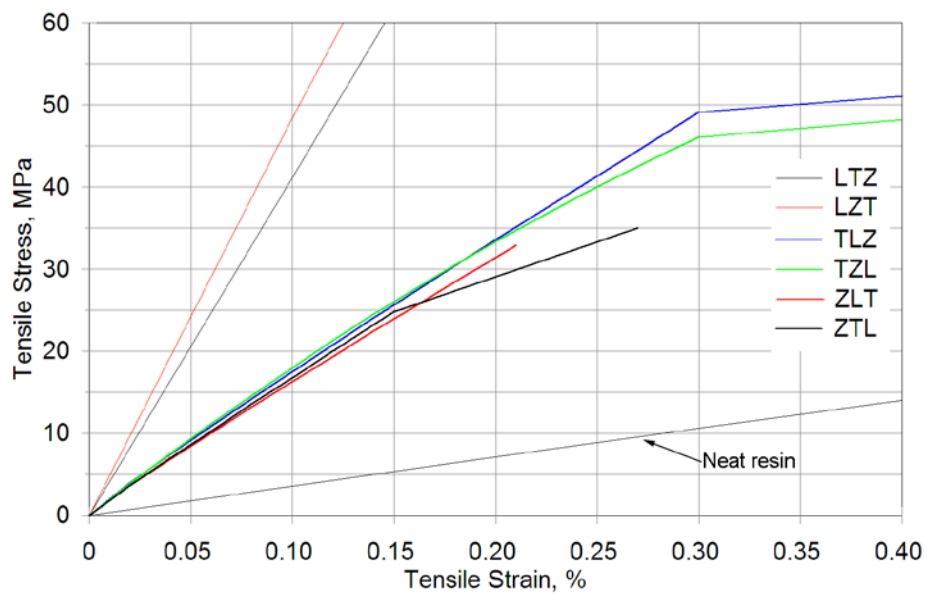
Figure 26a. Tensile Best Fit Stress-Strain Curves (Two Scales)
