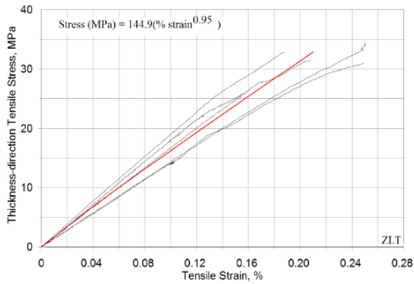
(28e) Thick dir. tension, ZLT orientation
