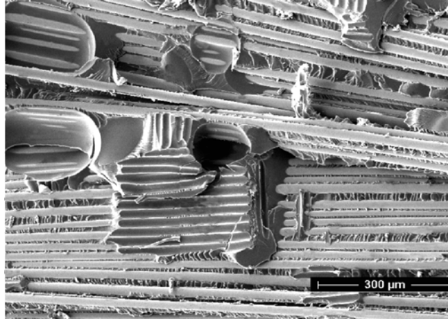
Figure 82. Crack path C, along reinforcement surface, with resin patch showing peel-ply imprint at pore (center), static CLS test, ADH-5, crack growth right to left.
