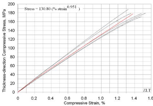
(28k) Thick dir. compression, ZLT orientation
