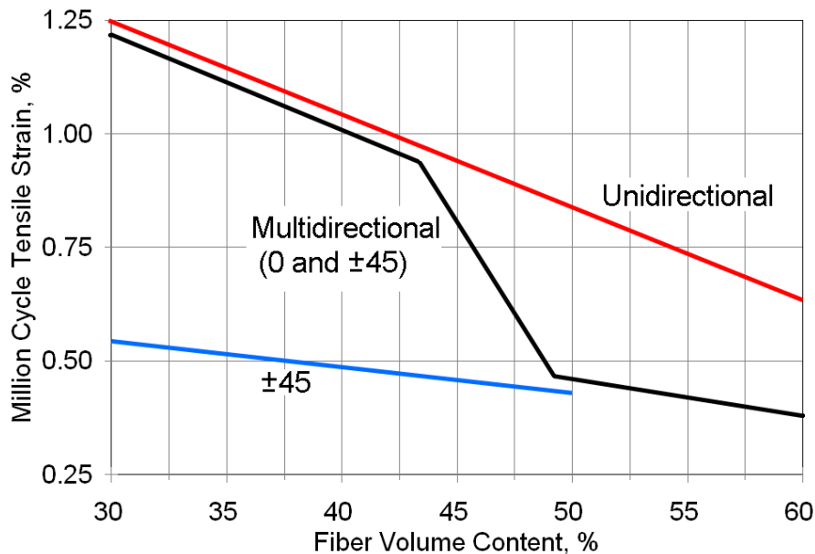
Figure 5. Fatigue trends vs. fiber content for unidirectional, multidirectional and biax laminates based on early [6, 9] low density weft unidirectional Owens Corning/Knytex fabrics D155 and D092, DB fabrics DB120 and DB240, with Interplastic Corp. Corezyn 63-AX-051 polyester resin (UP-2).
