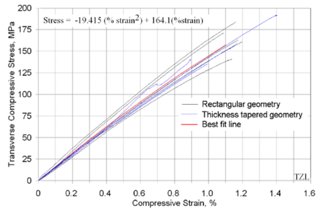
(28j) Transverse compression, TZL orientation
