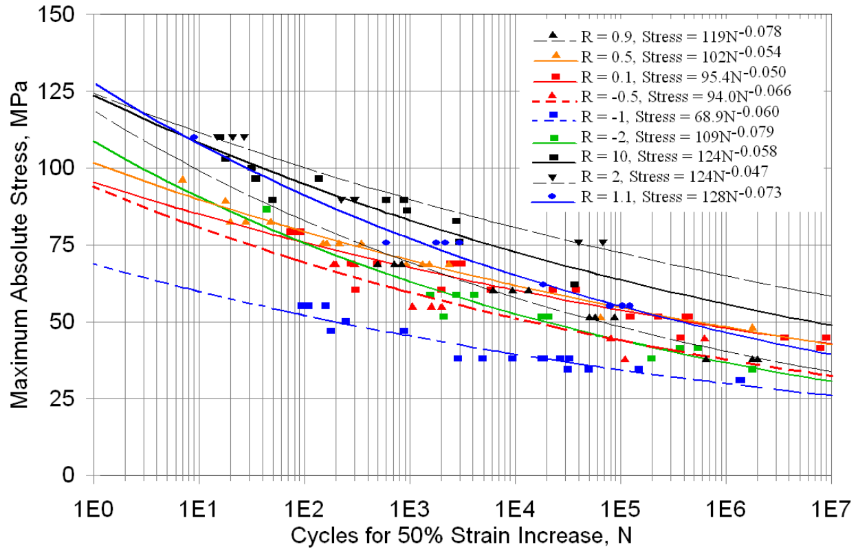
Figure 58. S-N data and trend lines for DB laminates tested at nine R-values.
