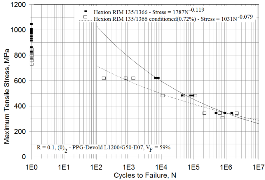
Figure 98. Tensile fatigue S-N data for UD fabric H/EP-1 laminates, comparing control conditioned and tested laminates with saturated seawater conditioned and tested laminates.
