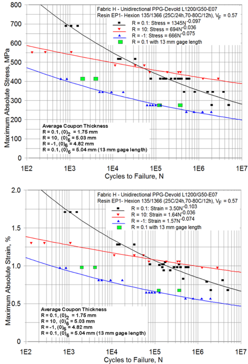
Figure 47. Fatigue S-N data for baseline UD laminates tested at three R-values, showing the influence of thickness and gage length on tensile fatigue results.
