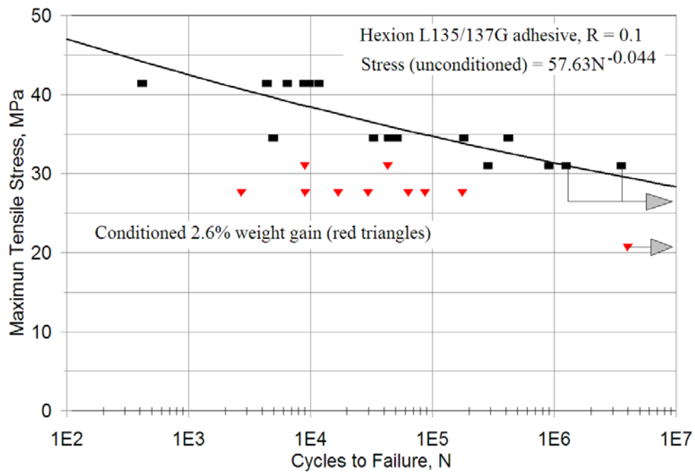
Figure 105. Neat adhesive dry control tensile fatigue behavior, with limited seawater saturated data shown for comparison.
