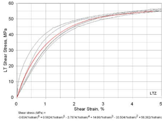
(28m) LT shear direction, LTZ orientation
