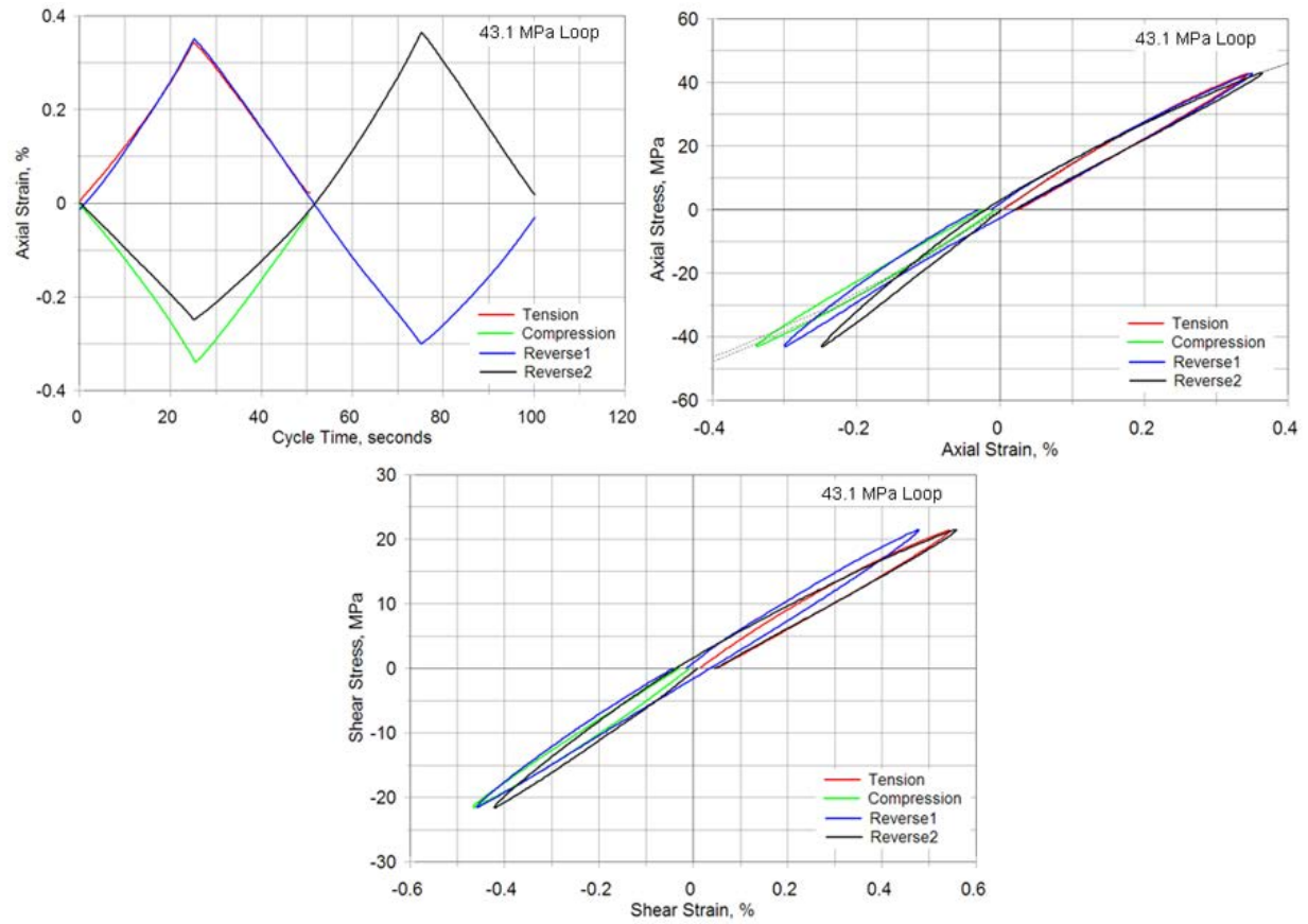
Figure 35 (e). 43.1 MPa
