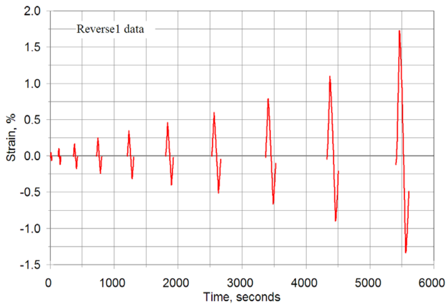
Figure 34. LUR strain-time response for each loading step for four reverse1 coupons.
