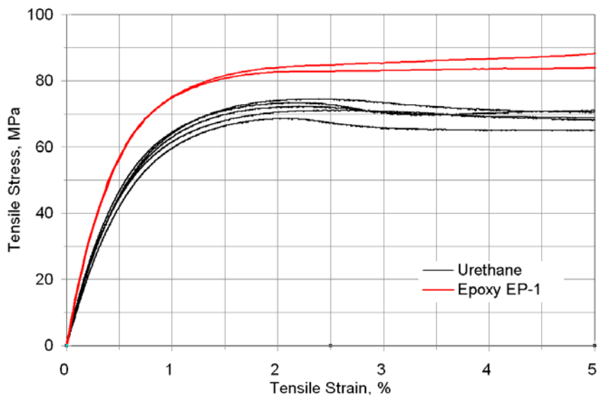
Figure 68. Comparison of tensile stress-strain curves for polyurethane and epoxy resin \pm 45^\circ laminates loaded at 0^\circ .
