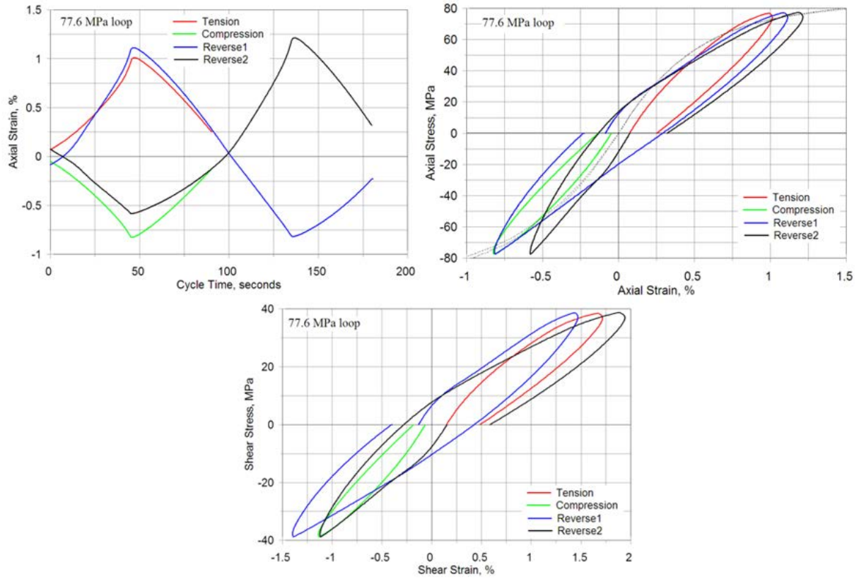
Figure 35(i). 77.6 MPa
