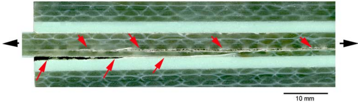
Figure 74. Photograph of crack transition from adhesive into laminate interior, symmetrical CLS geometry, 2.4 mm thick adhesive ADH-1, crack growth left to right.
