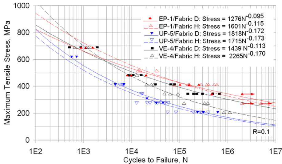
Figure 40. Effect of UD fabric D vs. fabric H, for EP, VE and UP resins, (0)_2 laminates.
