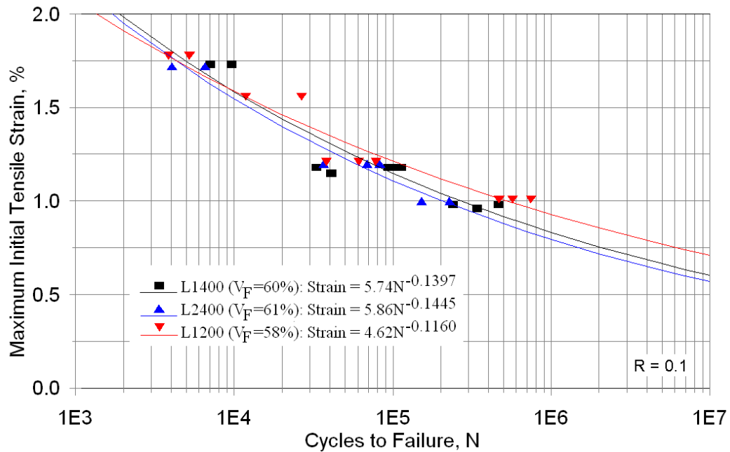
Figure 41. Strain vs. cycles for MD laminates fabricated with three different weight UD fabrics from Table 10, epoxy EP5, R = 0.1 .
