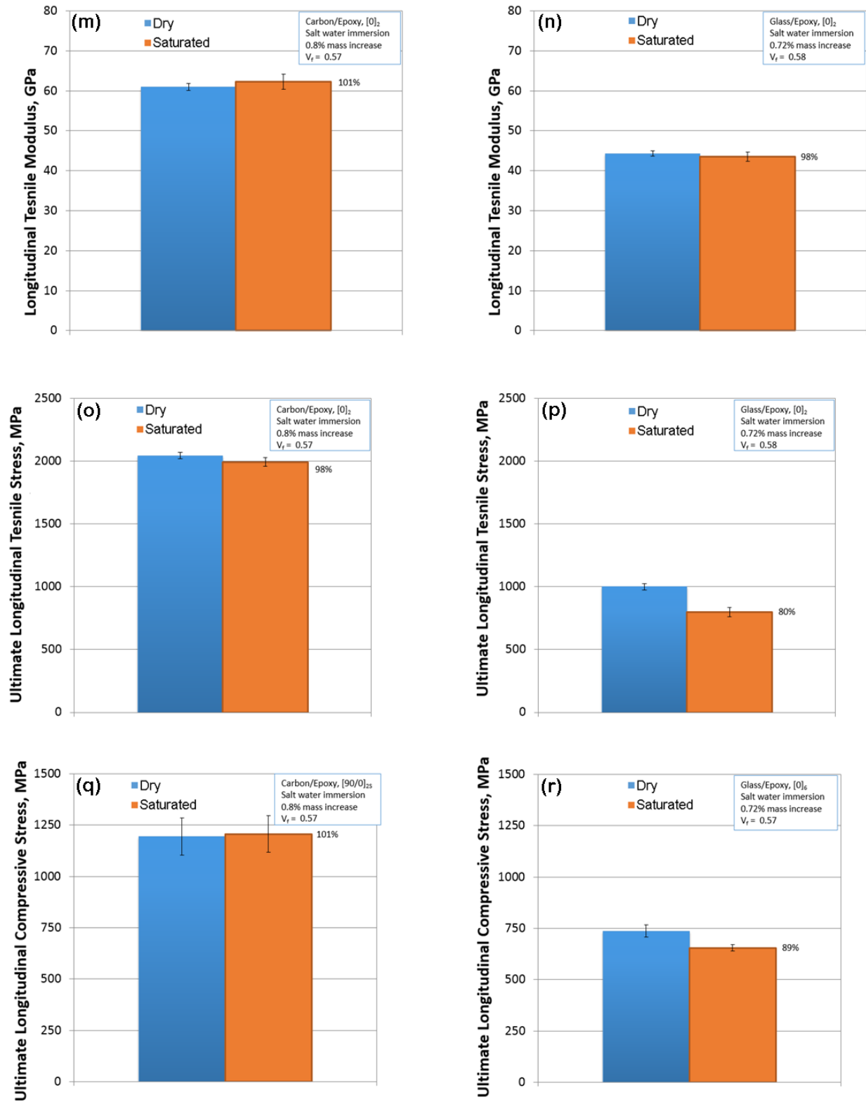
Figure 97 (m)-(r). Static environmental test data
