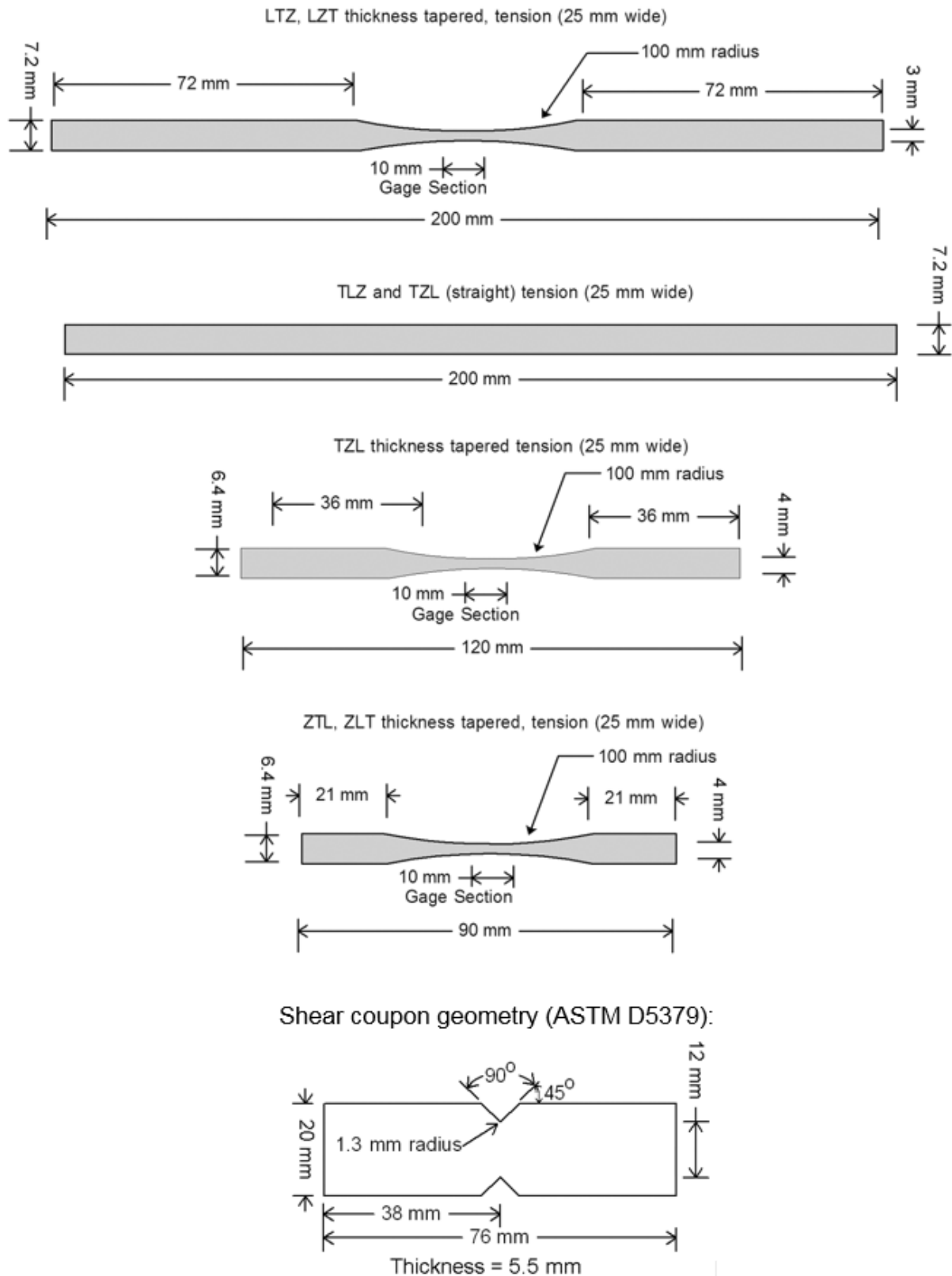
Figure 15(a). Tensile coupon geometries (ASTM D3039 and D638 with variations):
