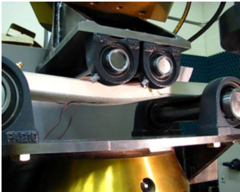
Figure 93. Sandwich panel fatigue test fixture (top) and with failed sandwich panel (bottom).
