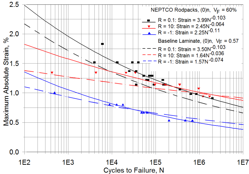
Figure 46. Maximum absolute strain versus cycles to failure, RodPack versus the baseline laminate.
