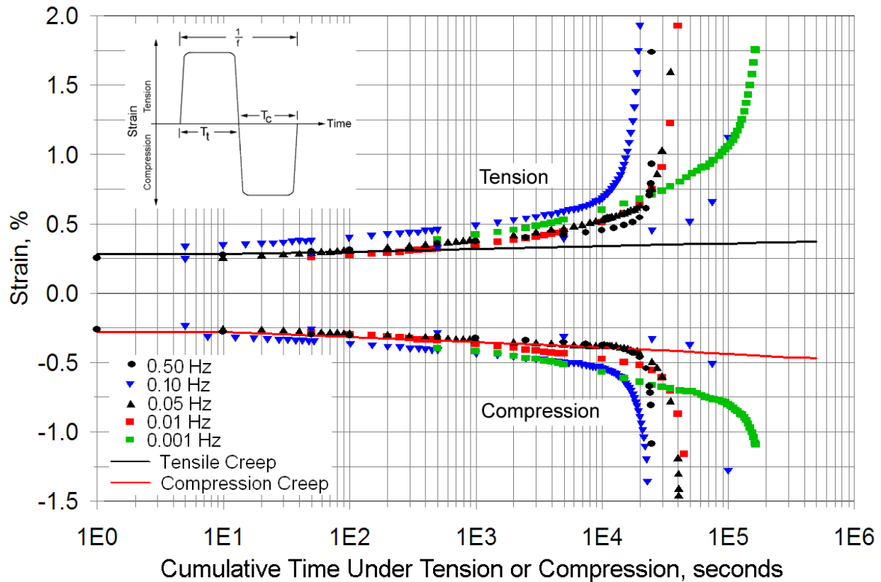
Figure 65 Strain accumulation vs. cumulative time under tension and compression parts of R = -1 square waveforms at different frequencies, compared to simple creep strains at the same stress of \pm 37.9 MPa, R = -1 .
