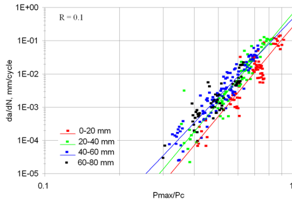
(a) Long CLS with steel, R = 0.1
