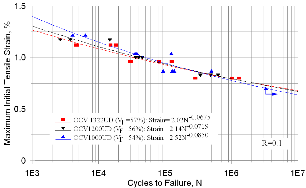
Figure 42. Strain vs. cycles for UD laminates with three different weight OCV™ fabrics, EP1 epoxy, R = 0.1 .
