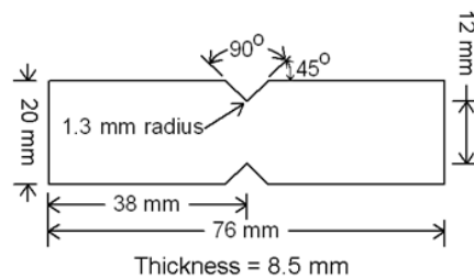
ASTM D5379 Shear test geometry
