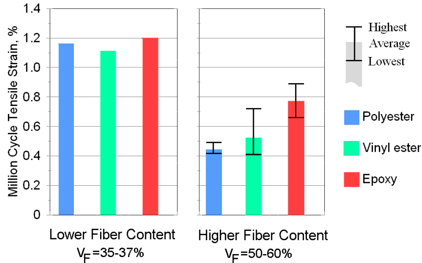
Figure 4. Comparison of polyester, vinyl ester and epoxy resin laminates at low (fabric A) and higher (fabrics D, G and H) fiber contents.
