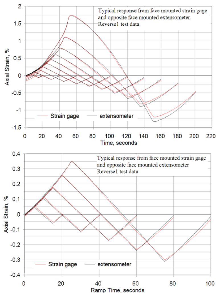
Figure 32. Strain-time traces for the reverse1 loading sequence comparing extensometer and strain gage readings for the same test; full loading range (top) and magnified range (bottom).
