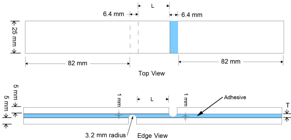
Figure 24. Notched lap shear adhesives test coupon [2].
