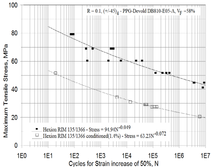
Figure 99. Tensile fatigue S-N data for DB fabric P/EP-1 laminates, comparing control conditioned and tested with saturated seawater conditioned and tested.
