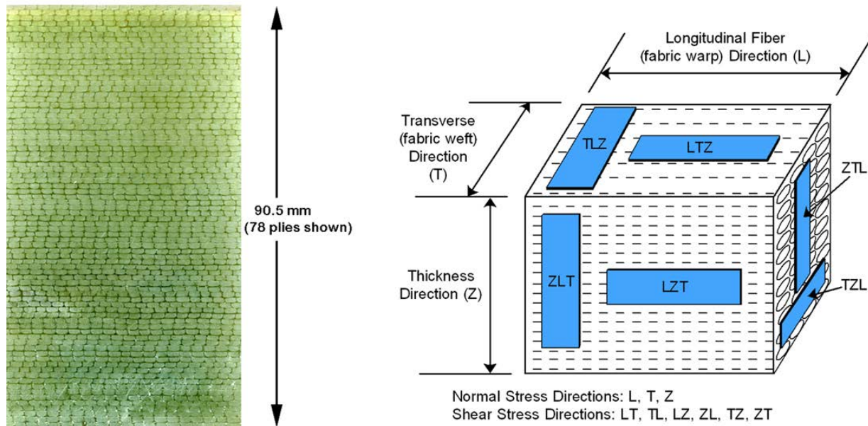
Figure 10. Through-thickness fabric strand stacking for infused 80 ply laminate (50 mm wide x 90.5 mm high slice) and laminate direction nomenclature.
