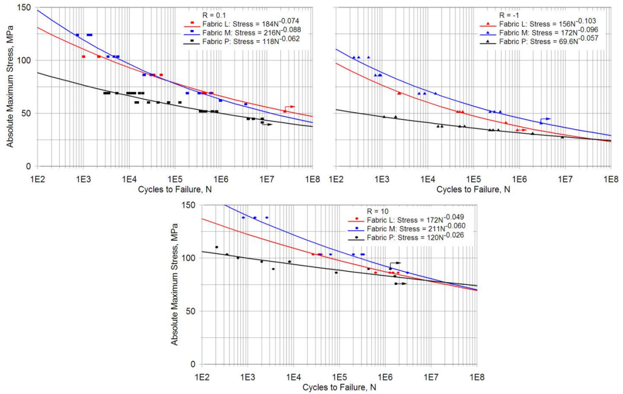
Figure 50. Maximum absolute stress vs. log cycles to failure for R = 0.1 (top left), -1.0 (top right) and 10 (bottom) for fabrics L, M and P, resin EP-1 (Tables 2 and 3).
