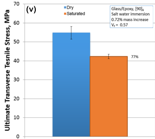
Figure 97 (s)-(v). Static environmental test data
