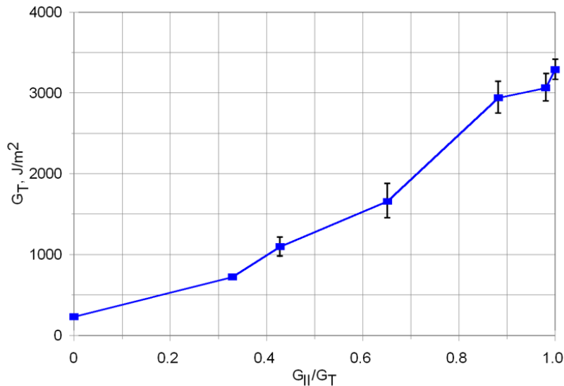
Figure 85. Mixed mode bending static test average results for laminate delamination resistance, unidirectional infused Vectorply ELT-5500 glass fabric with SP Systems Prime 20 LV epoxy, V_f = 0.51 [1].
