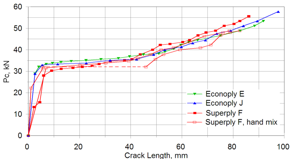
Figure 89. Effect of laminate peel-ply type and adhesive mixing method (machine mixed unless noted) on static crack growth resistance from machined notch; dashed line indicates unstable crack jump.
