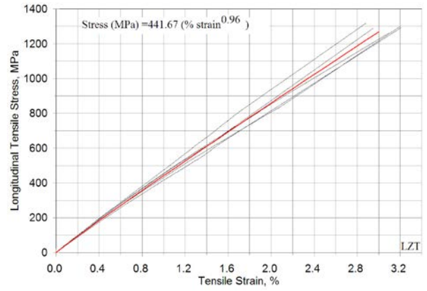
(28b) Longitudinal tension, LZT orientation
