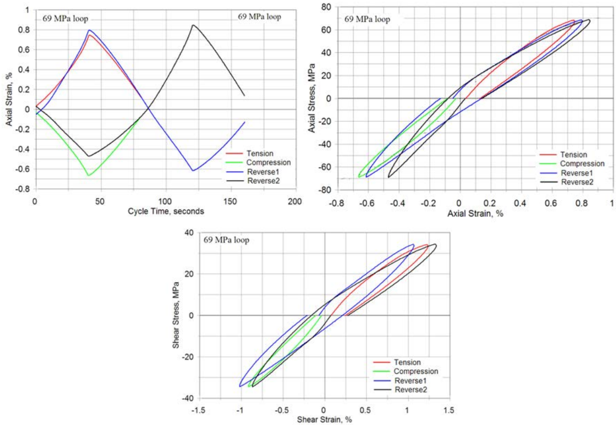
Figure 35(h). 69 MPa
