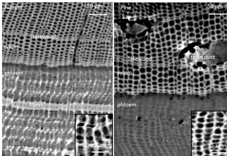
Figure 2: Axial views of irrigated one-seed juniper (left) and piñon pine (right) tissues at the xylem-phloem transition. In both images, xylem is the region of high contrast at the top of the image with less-structured phloem below. Two and three late-wood regions are clearly visible in one-seed juniper and piñon pine xylem, respectively. The newest growth ring (closest to the phloem boundary) is from 2012. In juniper, a ray from xylem to phloem is visible. In pine, two resin ducts are visible. Lighter areas are materials more interactive with X-rays (fibers, more lignified cell walls, clusters of sugars). In juniper phloem, rows of fibers are common, and conduit walls in the radial direction are very thin (insert). In pine phloem, the structure is more uniform, although there still is a clear difference in radial and tangential cell wall thickness between xylem and phloem (insert).
