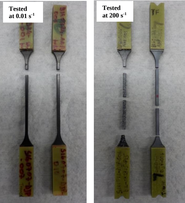
Figure 15. Failure modes for UD [90^\circ] CFRP specimens with longer gauge lengths.
