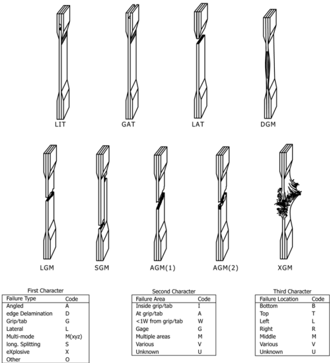
Figure 14. Tensile test failure codes and typical modes for polymer matrix composite materials [10].
