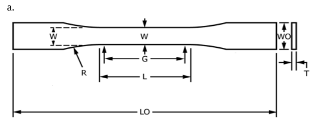
b. Figure 1. (a) Tensile specimen geometry for unidirectional (UD) material in the 0° and 90°. (b) specimen nomenclature.
