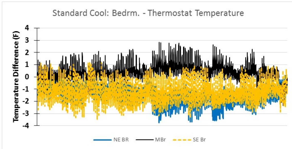
Figure 2-13. Hourly average room-to-thermostat temperature differentials during standard cooling
