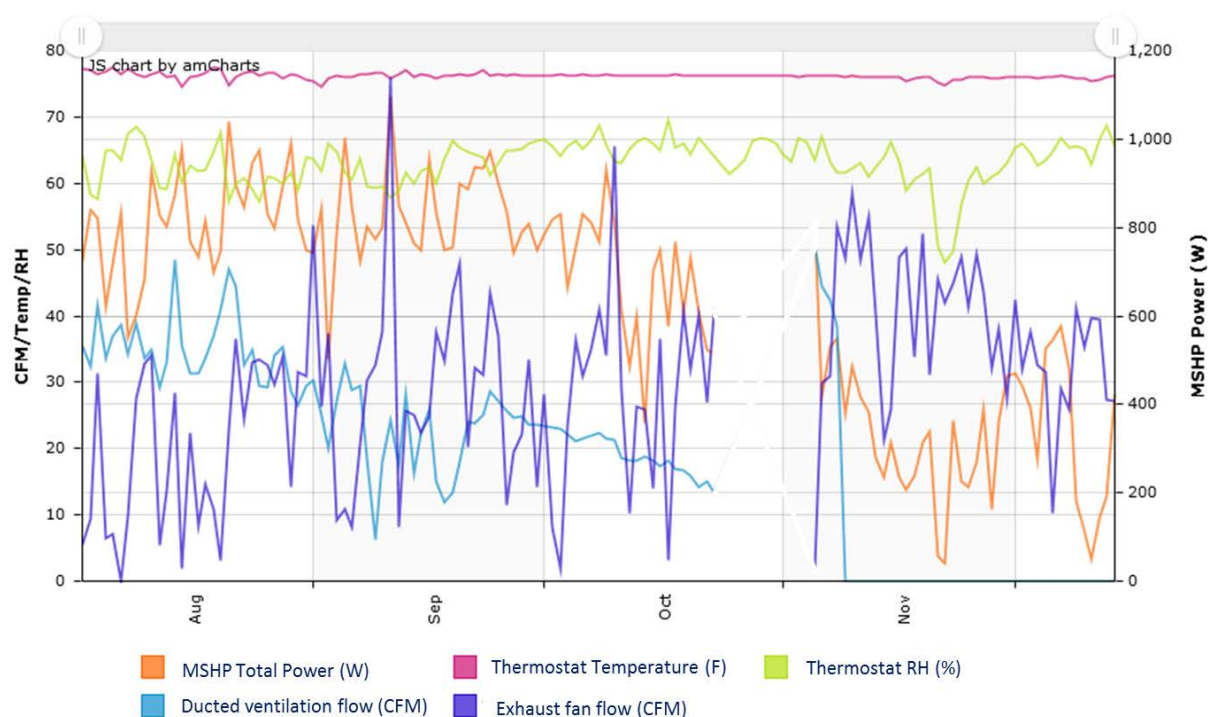
Figure 3-32. SS1 ventilation system performance post-occupancy, daily average values
