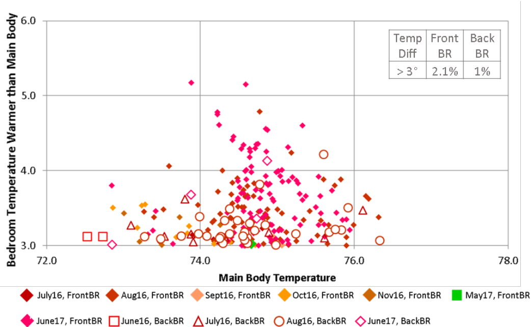
Figure 3-12. Periods when the SEV1 front (solid) and back (outline) bedroom temperatures were more than 3°F warmer than the main body
