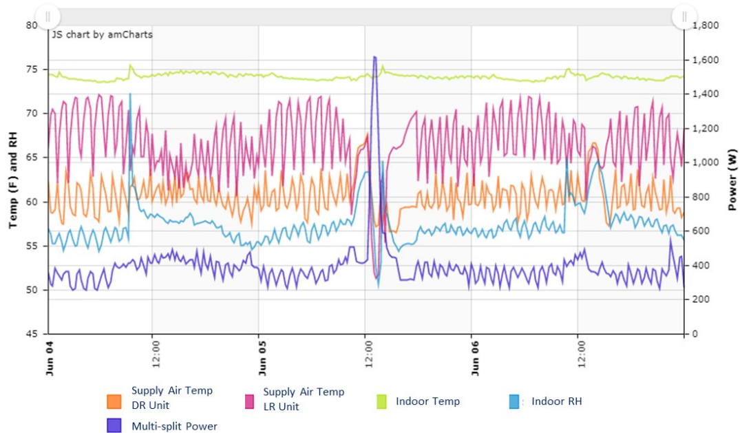
Figure 3-22. SEV1 indoor temperature and RH, along with SATs of the dining room (DR) and living room (LR) indoor fan coil units. The purple line shows the total power of the multisplit system.
