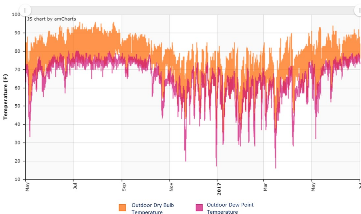
Figure 3-8. Outdoor temperature and dew point from Daytona Beach International Airport National Weather Service Station near the Southeast Volusia Habitat for Humanity Homes
