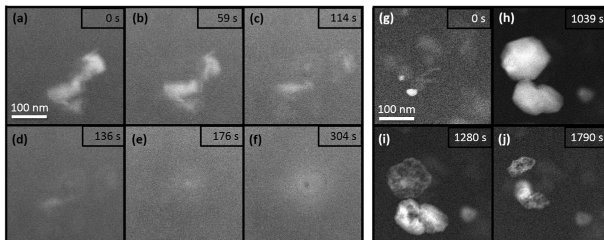
Figure 3. LCEM imaging in STEM mode of boehmite suspension in DI water. Images captured using (a–f) a 200 keV STEM probe and (g–j) a 300 keV STEM probe from Supplementary Movie 3.
