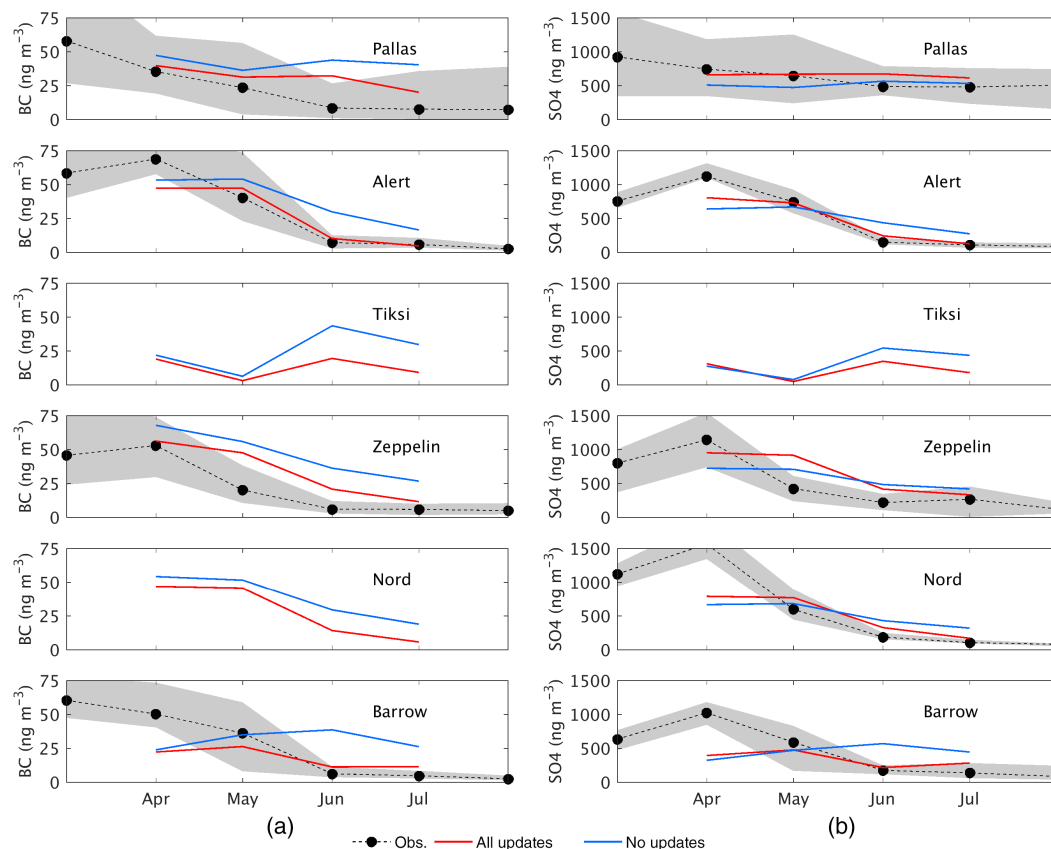
Figure 7. Monthly median BC (left) and SO 4 2- (right) observations at Arctic surface stations (gray shading indicates 25th and 75th percentile) and corresponding WRF-Chem results (red, ALL_UPDATES; blue, NO_UPDATES).
