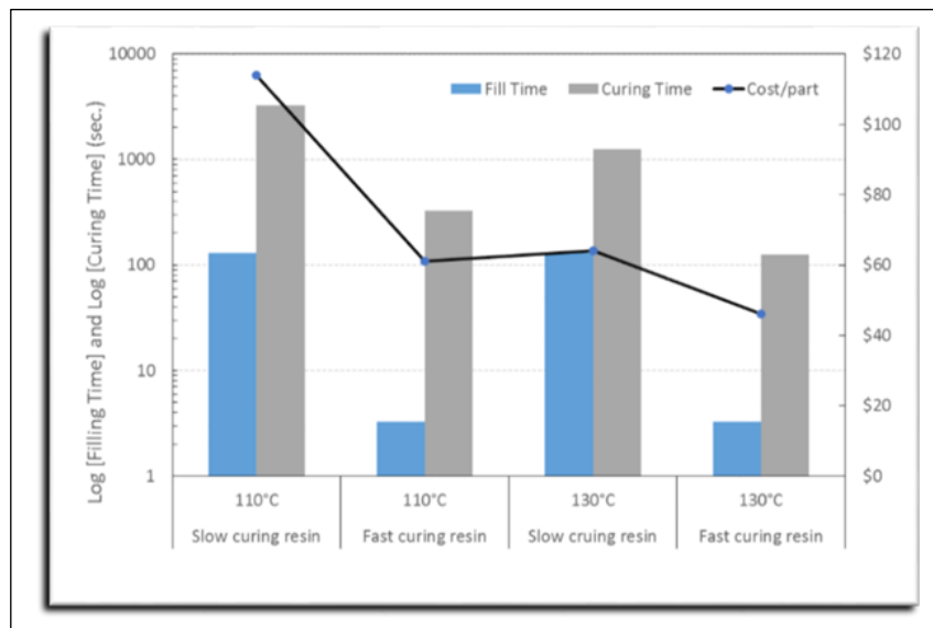
Figure 6. Curing time vs curing temperature and cost/part in CPF.
