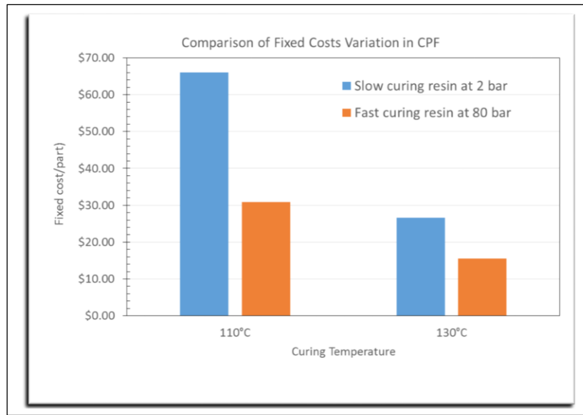
Figure 7. Comparison of the fixed costs variation in CPF.
