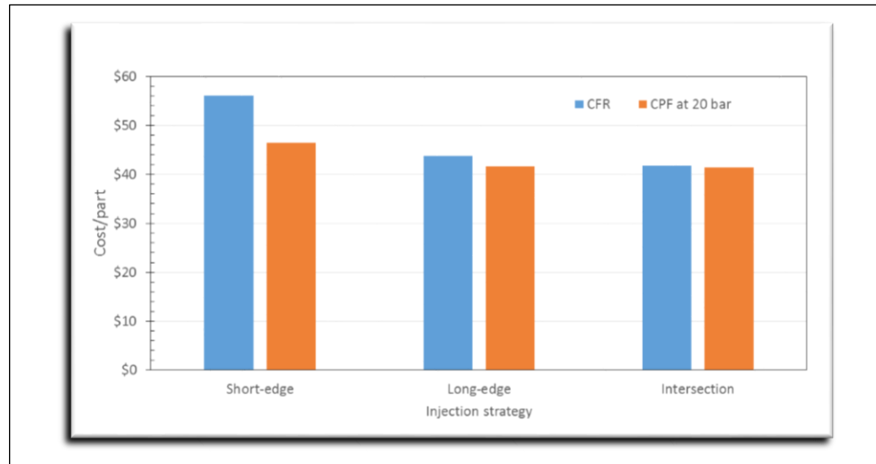
Figure 13. The cost variations of the three injection strategies in the representative automobile component.
