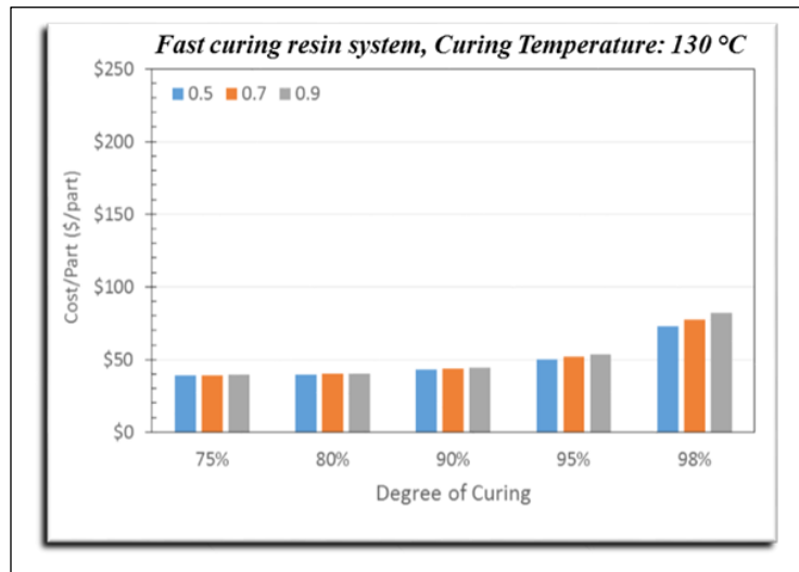
Figure 11. Cost/part vs the degree of curing at curing temperature 130°C in the fast curing resin system with the different ratios of the demolding time/curing time.
