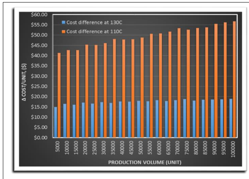
Figure 9. The difference in cost/unit vs production volume with the slow/fast curing resins systems in the mode of the CPF at different curing temperatures.
