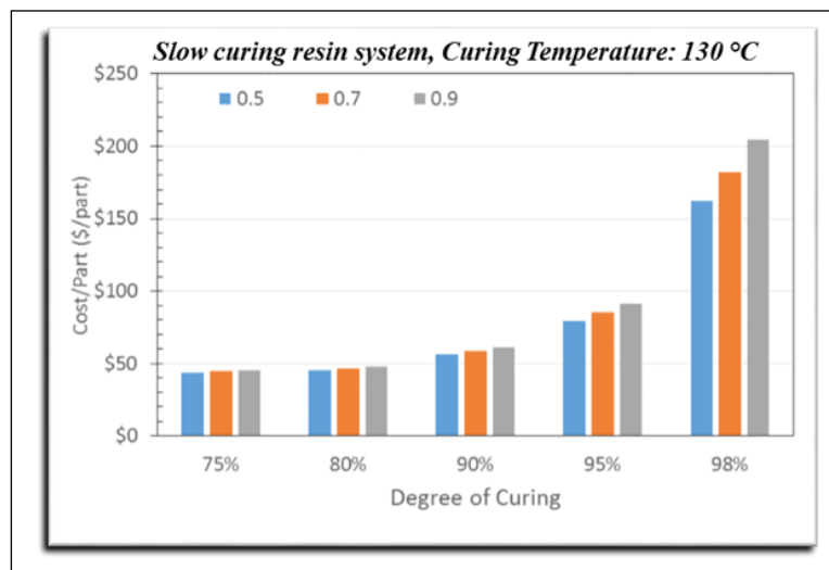
Figure 10. Cost/part vs the degree of curing at curing temperature 130°C in the slow curing resin system with the different ratios of the demolding time/curing time.
