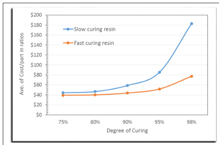
Figure 12. Average of cost/part vs the degree of curing at curing temperature 130°C for the two curing resins systems.
