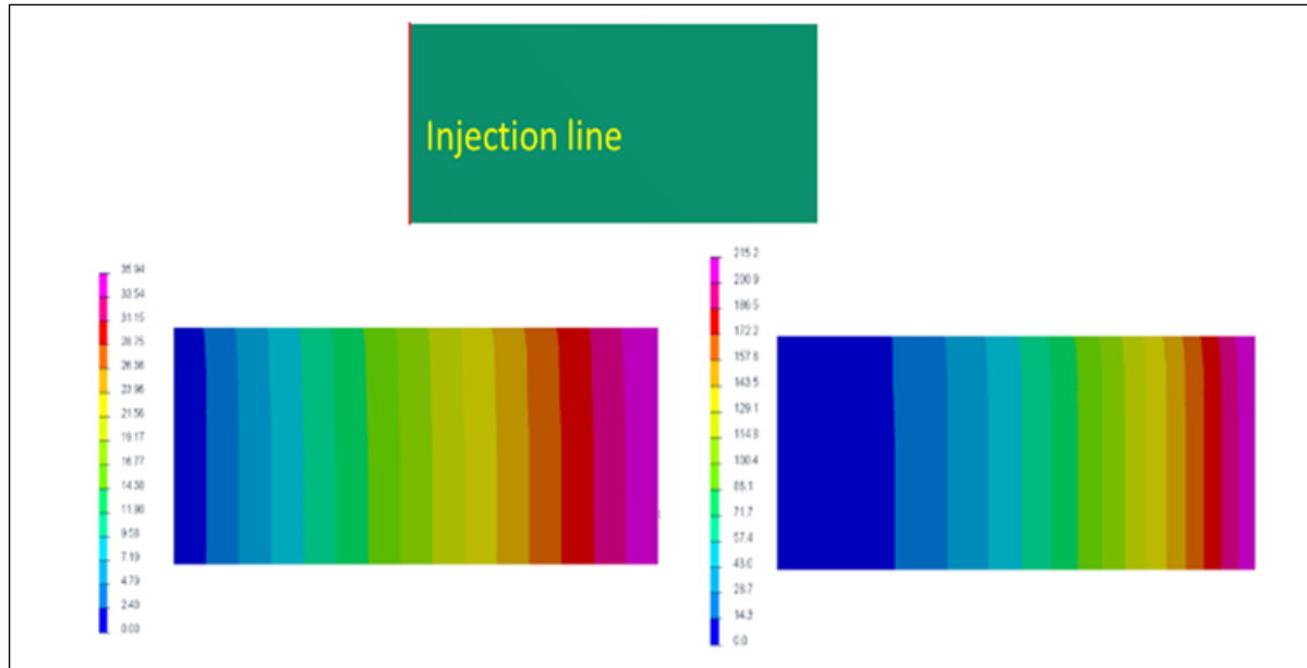
Figure 1. Injection line and the fill time contours of the panel with 237 bar and 20 bar (Injection design -1)
