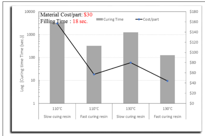
Figure 4. Curing time vs curing temperature and cost/part in CFR.
