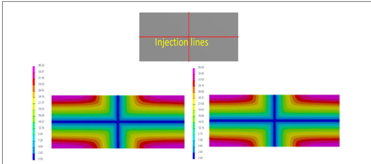
Figure 3. Injection line and the fill time contours of the panel without pressure limitation and limiting the pressure to 20 bar (Injection design -3)
