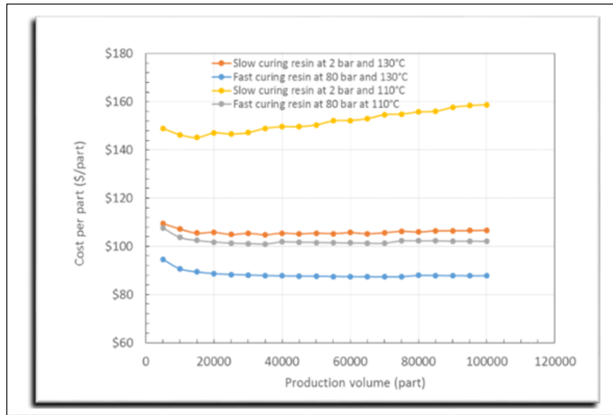
Figure 8. Cost/unit vs production volume with the slow/fast curing resins systems in the mode of the CPF at different curing temperatures.
