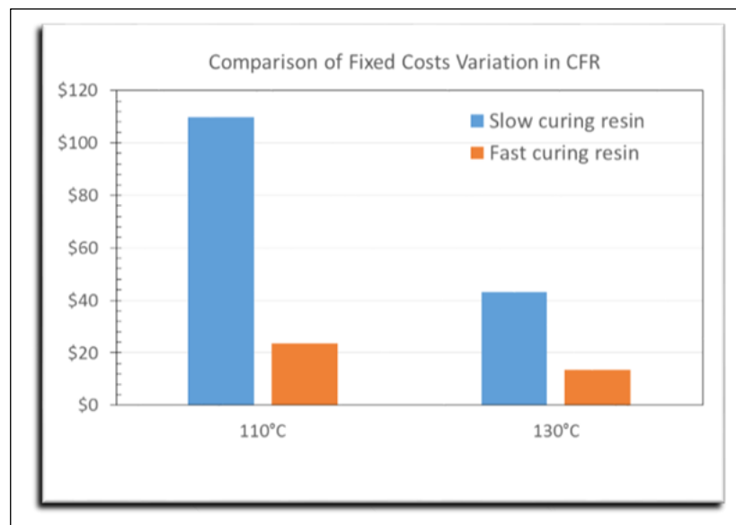
Figure 5. Comparison of fixed costs variation in CFR.
