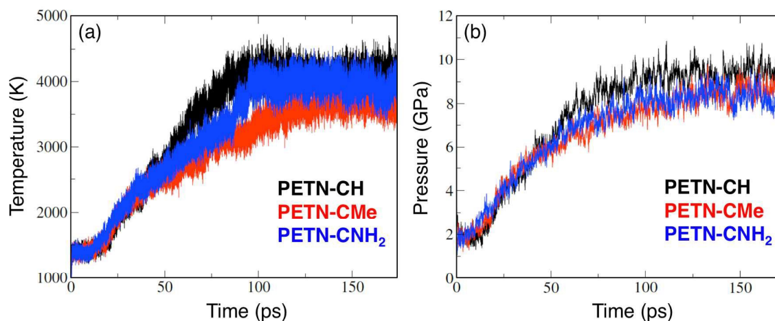
Figure 4. Evolution of the (a) temperature and (b) pressure in liquid PETN-CH, PETN-CMe, and PETN-CNH 2 initialized at a temperature of 1400 K. The pressure data were smoothed using a 50 point running average.
