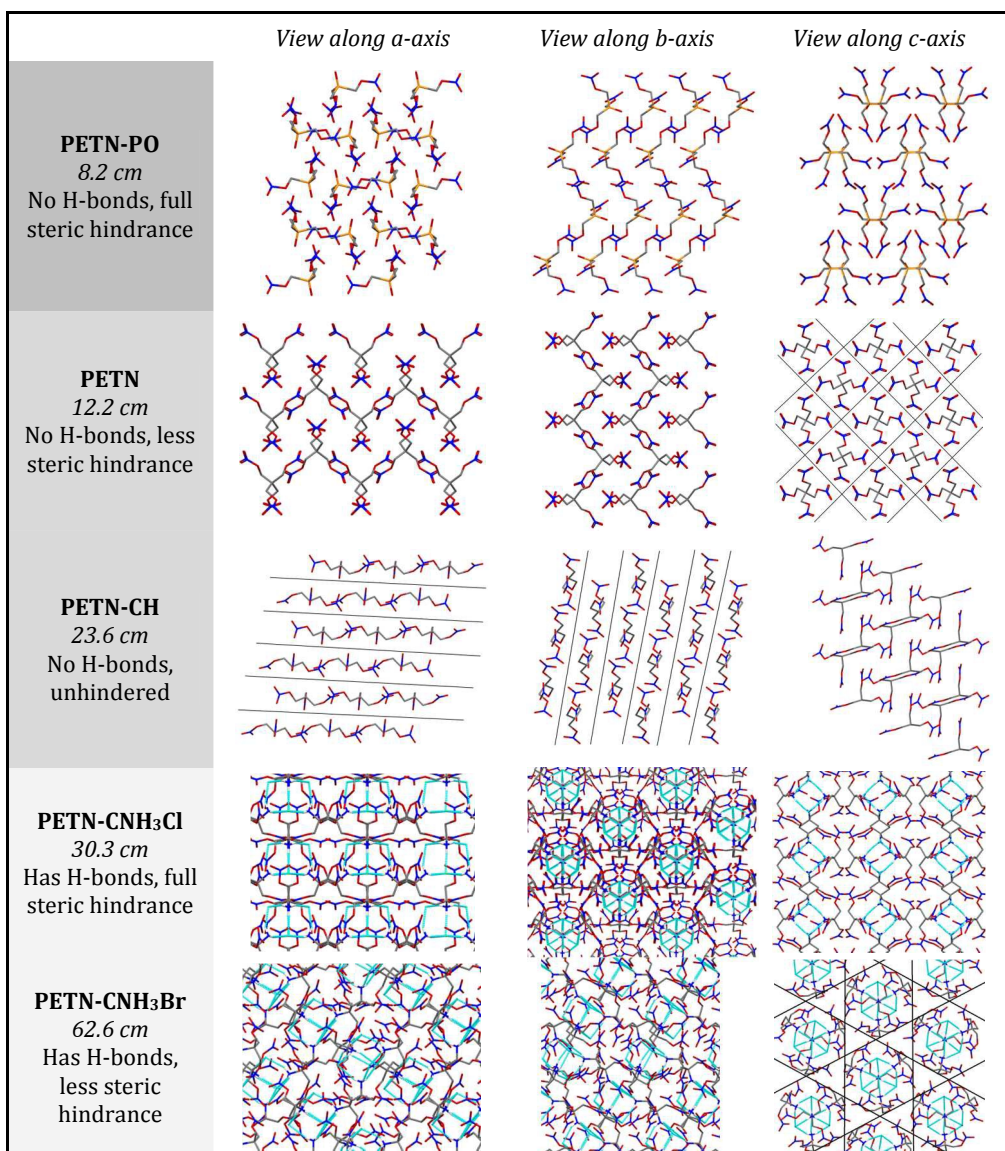
Figure 7. Solid state packing in PETN-PO, PETN, PETN-CH, PETN-CNH 3 Cl, and PETN-CNH 3 Br, viewed along the a, b, and c crystallographic axes. Each material has the impact sensitivity listed below it (in cm; decreases from top to bottom), with a summary of whether hydrogen bonding and planes exist.
