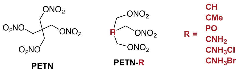
Figure 1. Structure of PETN and a list of the PETN-R derivatives examined in this study.
