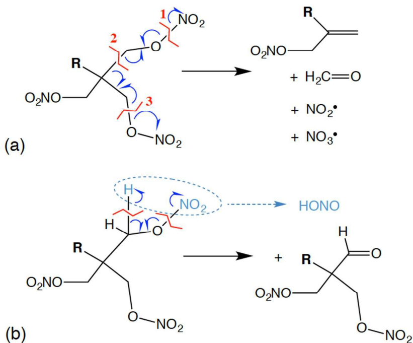
Figure 6. Proposed mechanisms for some of the likely first reactions for PETN derivatives including initial intermediate products, where R = \text{NH}_2 [ PETN-CNHR 2 ; mechanism (a)], H [ PETN-CH 2 R ; mechanism (b)], or \text{CH}_3 [ PETN-CMe 2 ; mechanisms (a) and (b)].
