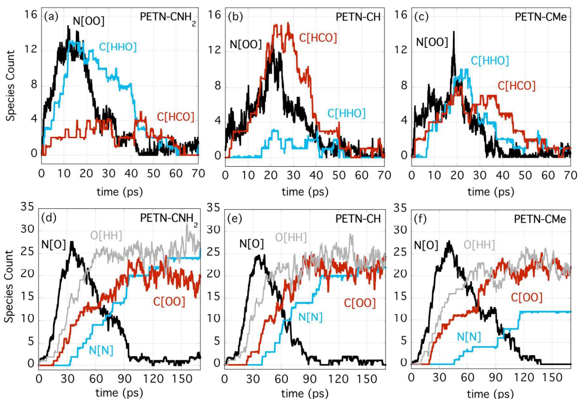
Figure 5. Species count for the three PETN derivatives, showing N[OO], C[HCO], and C[HHO] for (a) PETN-CNH 2 , (b) PETN-CH, (c) PETN-CMe, and N[O], O[HH], C[OO], and N[N] for (d) PETN-CNH 2 , (e) PETN-CH, and (f) PETN-CMe.
