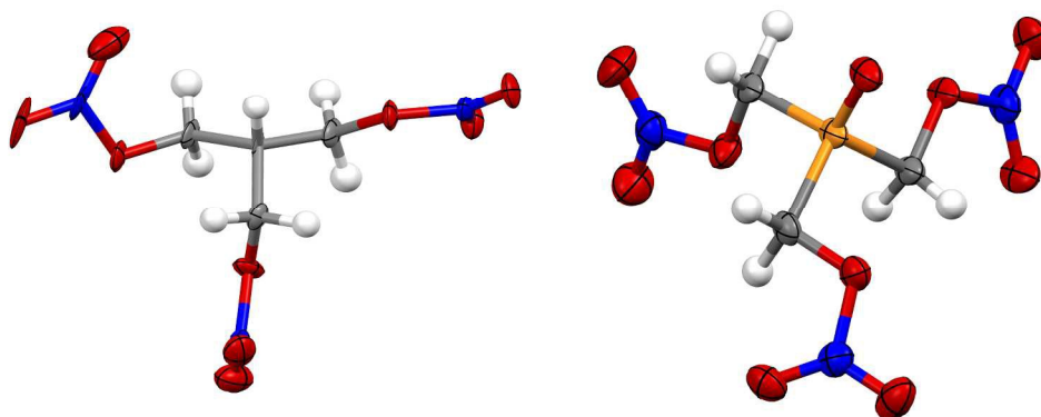
Figure 3. Solid state structure of PETN-CH (left) and PETN-PO (right). Orange, red, blue, grey and white ellipsoids represent P, O, N, C and H atoms respectively. Ellipsoids at 50% probability.
