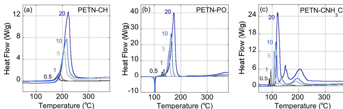
Figure 2. DSC kinetics plots, showing ramp rates at 0.5 °C, 1 °C, 5 °C, 10 °C, and 20 °C per minute, for (a) PETN-CH, (b) PETN-PO, and (c) PETN-CNH 3 Cl.
