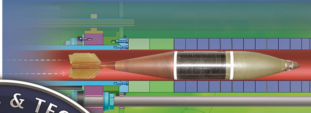
Sandia Pulsed Induction Coilgun
