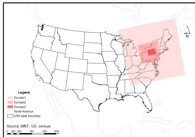
Figure 3. Map of study area shows three nested domains of WRF. The inner domain is located in the northeastern Pennsylvania and extends into southeastern New York.
