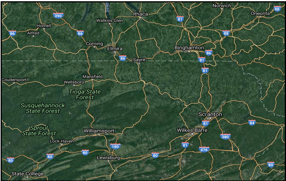
Figure 4. In domain 3, the latitude ranges from 40 to 42.67° N. The longitude ranges from −78 to −75.17° W. The figure shows the satellite view of the domain with major roads, cities and landmarks.
