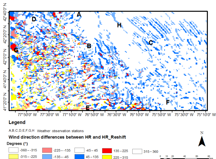
Figure 16. Wind direction difference between HR and HR_RESHIFT on 14 May 15:00 EST, 2015, showing a strip pattern in the right top corner where it is a valley region. The pattern indicates that the WRF model reacts differently on a small-area weather simulation when the GCS changes.
