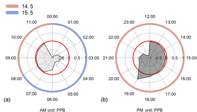
Figure 21. \text{CH}_4 mixing ratios difference between HR and HR_RESIFT in domain 3 for unconventional wells. Panel (a) shows the differences between 00:00 and 12:00 EST on 14 and 15 May. Panel (b) shows the differences between 12:00 and 24:00 EST on 14 May.
