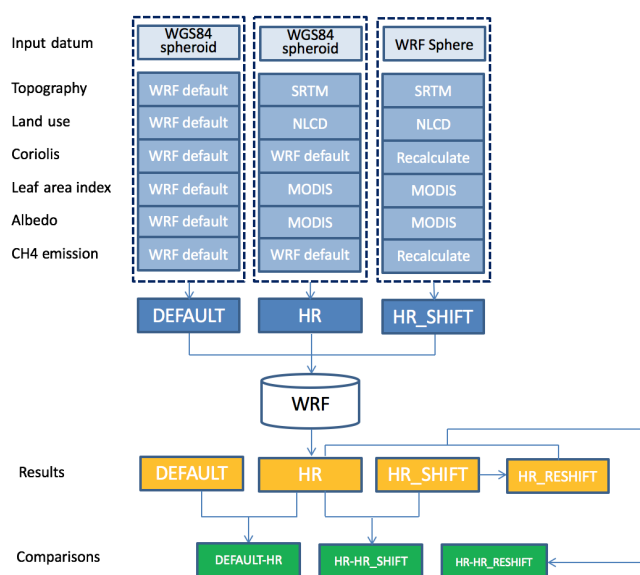
Figure 5. Workflow of the study showing the three scenarios: DEFAULT, HR and HR_SHIFT.
