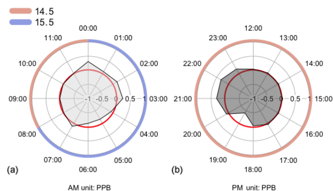
Figure 20. \text{CH}_4 mixing ratios difference between HR and HR_RESIFT in domain 3 for conventional wells. Panel (a) shows the differences between 00:00 and 12:00 EST on 14 and 15 May. Panel (b) shows the differences between 12:00 and 24:00 EST on 14 May.
