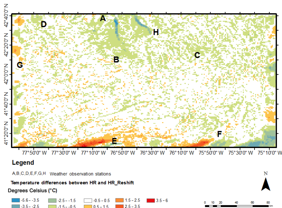
Figure 10. Temperature difference between HR and HR_RESIFT on 14 May 15:00 EST, 2015, showed that there is no significant spatial pattern.
