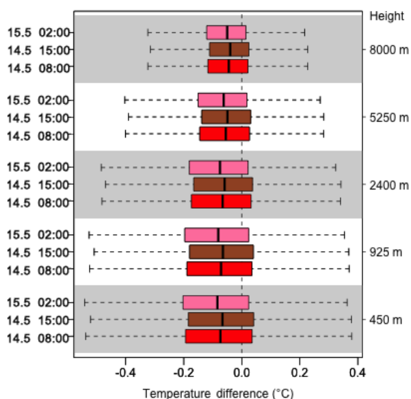
Figure 7. Temperature differences between HR and DEFAULT in domain 3.
