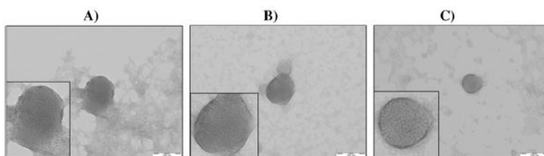
Figure 6. Morphology of cyclodextrin.siRNA structures visualized by transmission electron microscopy. (A) Cationic cyclodextrin (CCD) nanoparticle, (B) CD-M nanoparticle (M = methyl), (C) CD-F nanoparticle (F = folate). See text for full compositional details. All main structures shown at 200,000 \times magnification, with the scale bar indicating 100 nm. Insets show enlarged images at greater resolution. Figures reproduced with permission from [117]. Copyright Elsevier, 2016.
