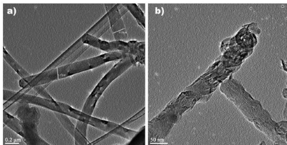
Figure 3. (a) Transmission electron micrographs of unmodified carbon nanotubes (CNTs) and (b) functionalized CNTs with activated carboxyl moieties. Scale bar equals 0.2 \mu\text{m} in (a); 50 nm in (b). Figures reproduced with permission from [64]. Copyright John Wiley & Sons, 2013.
