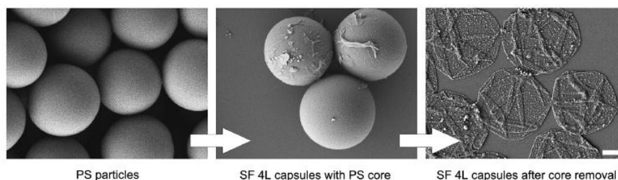
Figure 4. Representative scanning electron micrographs showing surface morphology of 4- \mu\text{m} polystyrene (PS) particles, after four layers (4L) of silk fibroin (SF) coating, and the dried microcapsules after core removal. Scale bar: 1 \mu\text{m} . Figures reproduced with permission from [78]. Copyright Elsevier, 2014.
