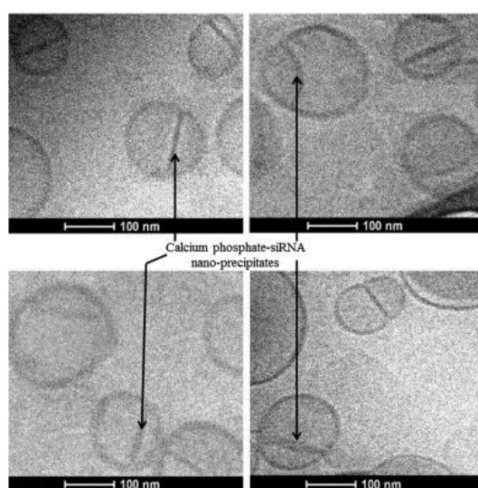
Figure 5. Transmission electron micrographs of cyclic arginine-glycine-aspartic acid (cRGD)—CPE liposomes (2%). CPE refers to calcium phosphate encapsulated siRNA. Arrows point to siRNA-calcium phosphate nano-precipitates inside the liposomes. Scale bar: 100 nm. Figure reproduced with permission from [92]. Copyright Elsevier, 2014.
