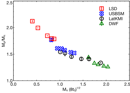
Figure 1. The ratio M_\rho/M_\pi shows indications of spontaneous chiral symmetry breaking in the massless fermion limit for QCD with N_f = 8 . The results from several lattice studies of different collaborations are shown as a function of the pion mass in units of the Wilson flow scale \sqrt{8t_0} , evaluated at each point. See text for references. Image from Ref. [3].
