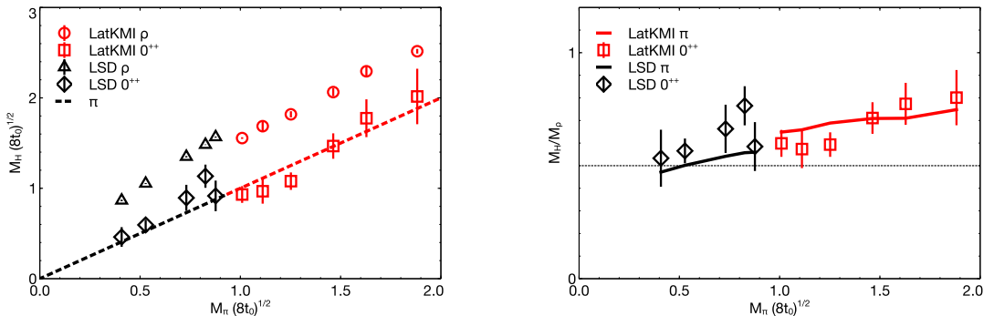
Figure 2. Combining LatKMI and LSD results for the flavor-singlet scalar state, a clear trend can be seen towards the massless fermion limit. The 0^{++} state remains degenerate with the pion (left) and much lighter than the vector meson (right), all the way to the lightest fermions studied by the LSD collaboration [11].
