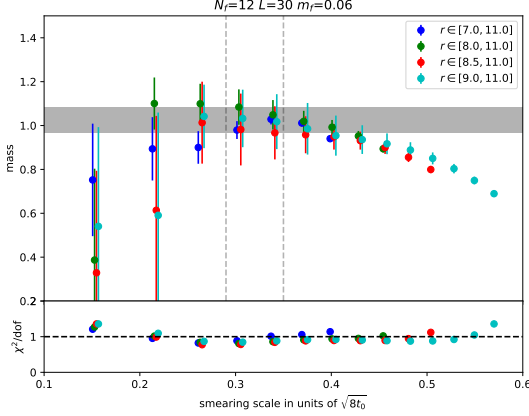
Figure 3. The \eta' mass fitted for different distance regions and smearings, for a specific ensemble of QCD with N_f = 12 . The main features are described in the text.
