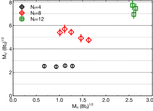
Figure 5. Comparison of the flavor-singlet pseudoscalar mass for N_f = 4, 8 and 12 as a function of the pion mass. The hadronic masses are in units of the Wilson flow scale \sqrt{8t_0} to partially remove discretization effects due to different gauge couplings for the various N_f theories. Different quark mass regions are explored for different N_f values.
