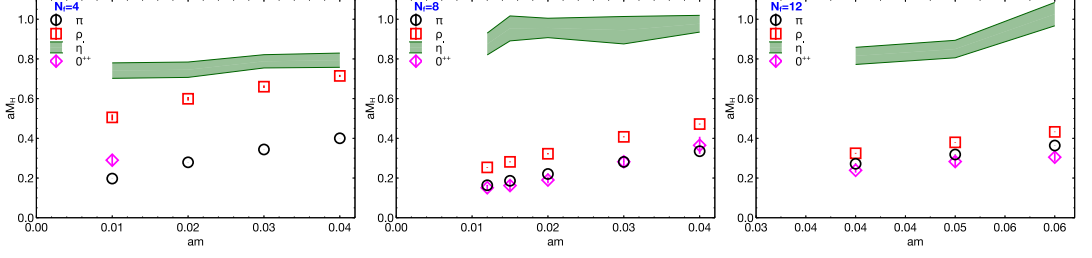
Figure 4. Flavor-singlet scalar and pseudoscalar spectrum compared to flavor-non-singlet pseudoscalar and vector spectrum for N_f = 4, 8 and 12 . The \eta' mass is shown with error bands that reflect a large systematic uncertainty. Only statistical errors are shown for the other states.
