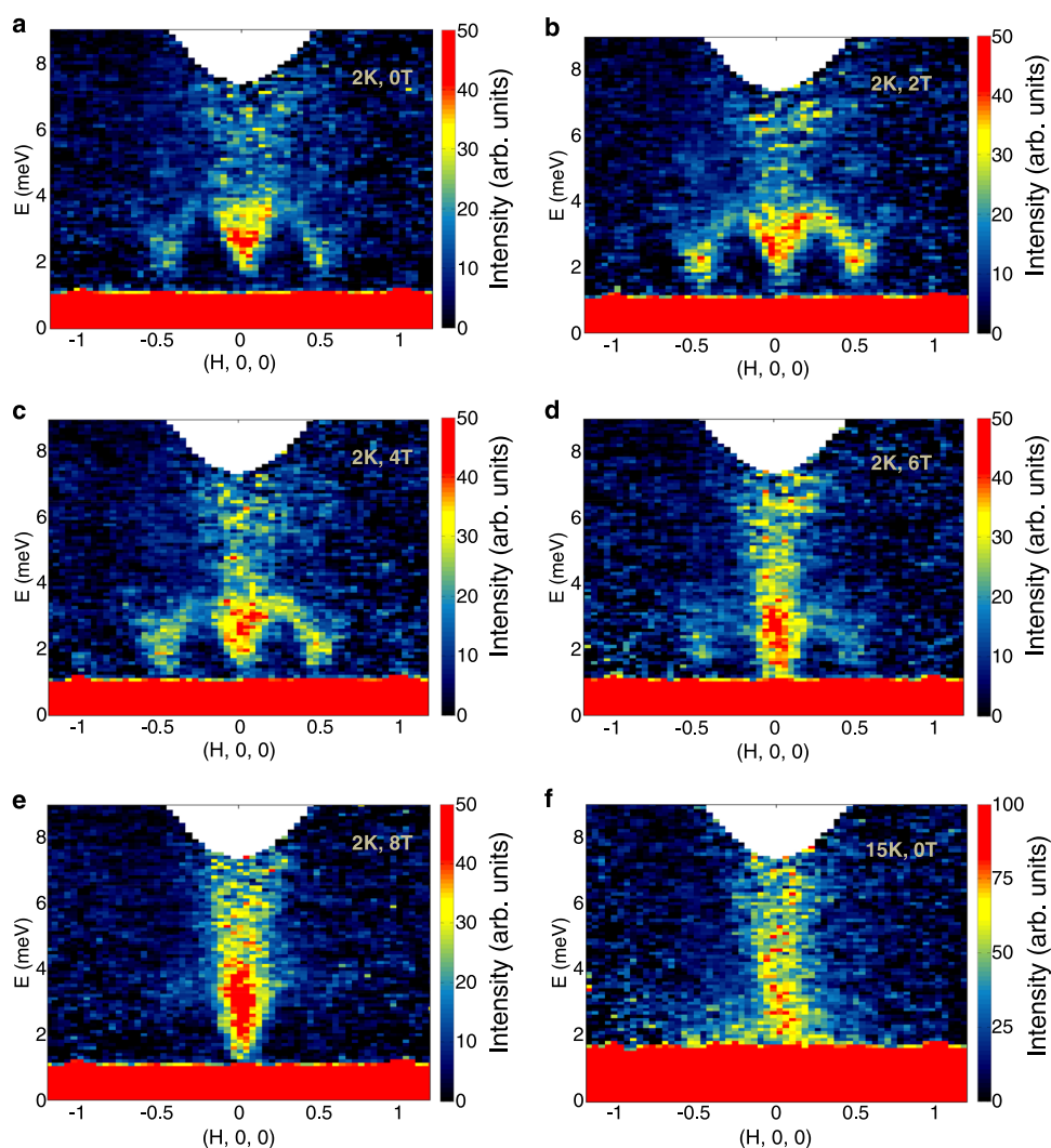
Fig. 2 Field and temperature dependence of INS along (H, 0, 0) : Data obtained on a 740 mg single crystal \alpha - \text{RuCl}_3 using the HYSPEC chopper spectrometer with E_i = 17 meV (see Methods). a–e Measurements at T = 2 K with an external field applied along the \zeta = (-1, 2, 0) direction (perpendicular to (H, 0, 0) ) using a Fermi chopper frequency of 240 Hz. The field strengths are a 0 T, b 2 T, c 4 T, d 6 T, and e 8 T. The slices shown are integrated over ranges \Delta\zeta = [-0.05, 0.05] (in units of 2.1 \text{ \AA}^{-1} , see Supplementary Fig. S1) and \Delta L = [-2, 2] (in units of 0.37 \text{ \AA}^{-1} ). The energy continuum at the \Gamma point is visible at all fields. The low-field data clearly shows the spin-wave spectrum along the (H, 0, 0) direction, with minima at the special points, Y-M- \Gamma -M-Y, of the 2D honeycomb BZ (see Fig. S1 for BZ definitions). f The zero-field spectrum at T = 15 K, using a Fermi chopper frequency of 120 Hz (see Methods)
