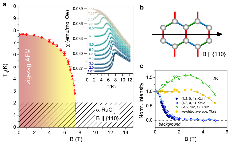
Fig. 1 Field-evolution of the zigzag order in \alpha -RuCl 3 : Bulk susceptibility and diffraction are shown as a function of magnetic field b applied along a reciprocal {110} direction. Note that the {110} is equivalently one of (1, 1, 0), (−1, 2, 0) or (2, −1, 0) directions. a Néel temperature vs. b determined from the local maximum in temperature-dependent magnetic susceptibility curves measured in fixed fields (i.e., where d\chi/dB = 0 ). Error bars are determined from the FWHM of a Gaussian fit to the peak in the derivative d^2\chi/dB^2 at the local maximum point (inset). For each field, \chi(T) was collected on warming after cooling in zero magnetic field. The region below the experimental base temperature is indicated by hash marks. b Schematic of the magnetic field direction in the honeycomb plane. c Magnetic Bragg peak intensity normalized to the zero-field value (i.e., I(B)/I(B=0) ). The field is applied in the (−1, 2, 0) direction perpendicular to the (H, 0, L) plane. Blue diamonds show the suppression of the in-plane (1/2, 0, 1) magnetic peaks in two different crystals, 'Xtal1' and 'Xtal2', measured at HYSPEC (solid symbols) and CORELLI (open symbols). The green circles show the out-of-plane magnetic peak at (−1/2, 1/2, 1) measured at CORELLI (See Methods for instrument parameters). The yellow symbols represent the weighted average intensity over magnetic peaks with L = 1 . In this average, the peaks within the (H, 0, L) plane contribute 1/3 of the intensity. Solid lines are a guide to the eye. Error bars represent one standard deviation assuming Poisson counting statistics
