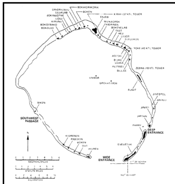
Figure 8: Enewetak Atoll.
