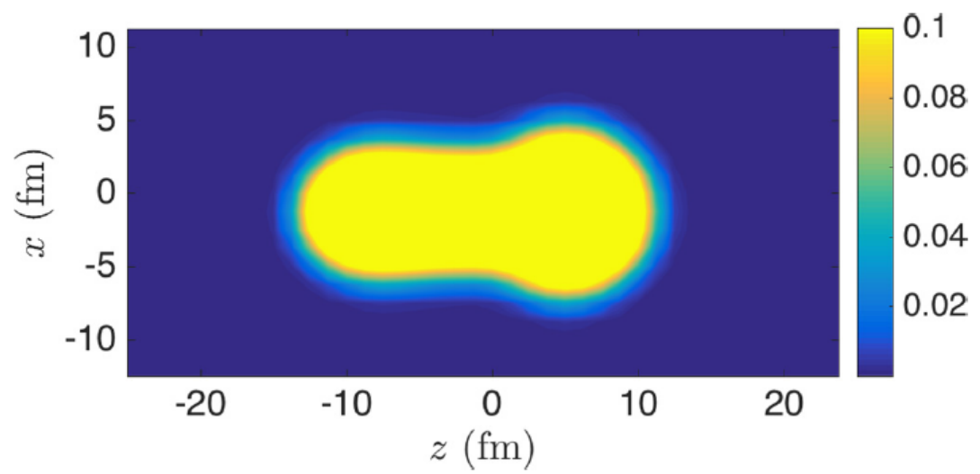
Initial condition for a ^{240}\text{Pu} calculation (will be used in fission) Jin et. al, Phys. Rev. C 95 , 044302 (2017)
