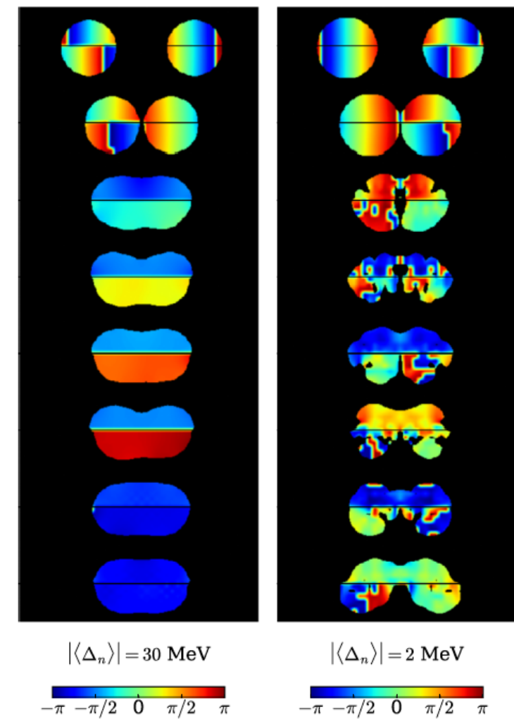
Initial condition for heavy-ion collisions Bulgac and Jin, Phys. Rev. Lett. 119 , 052501 (2017)
