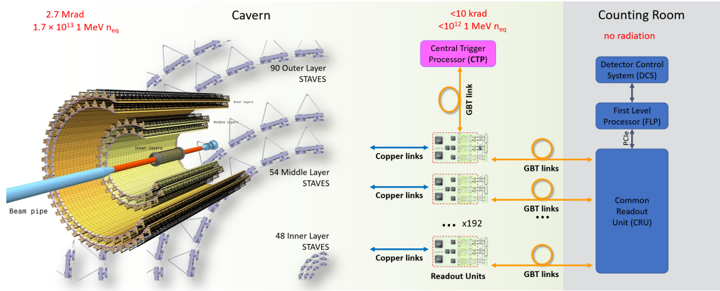
Figure 3. Architecture of the ITS Readout System.
