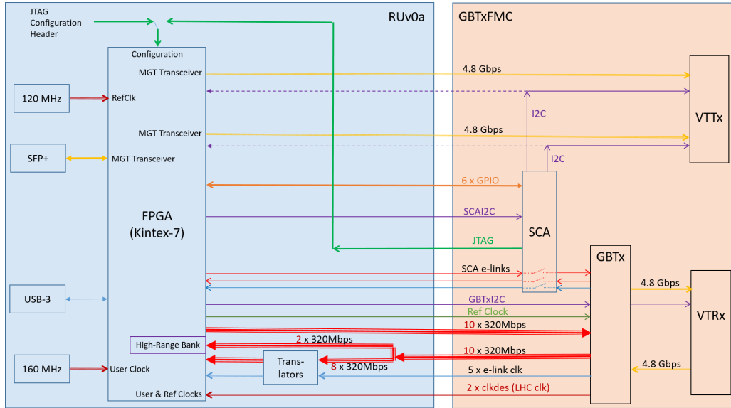
Figure 4. Prototype RU consisting of the Kintex-7 based carrier board and the FMC accommodating the GBT chipset.
