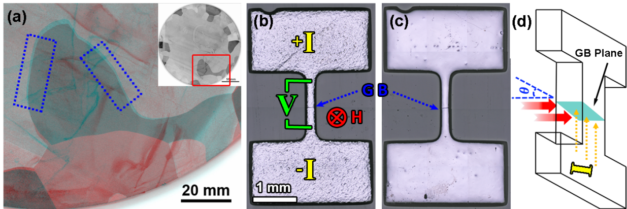
Figure. 1 (a) Overview of the large-grain (grain size > \sim 5\text{-}10 cm), high-purity ( \text{RRR} \geq 250 ) niobium ingot slice (2.5mm thickness), provided by TJNAF (Thomas Jefferson National Accelerator Facility) for this study. (b) The top and (c) bottom surface view of an I-shape (dog-bone) bi-crystal sample used for DC transport measurement after \sim 50 \mu\text{m} layer removal with BCP. The GB groove indicated by blue dotted arrows in (b) & (c) appeared after BCP. (d) Schematic diagram of the angular direction ( \theta ) between applied magnetic field (H) and the plane of GB and the direction of the transport current (I) on the I-shape sample. This bi-crystal sample was extracted from the regions indicated by the dotted blue rectangles in (a). The disorientation angle of the GB plane to the surface is \sim 5^\circ and the crystallographic misorientation across the GB is \sim 26^\circ .
