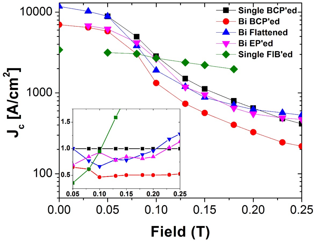
Figure 7. J_c(H) of all samples, in log-linear coordinates. The critical current density, J_c , was determined at, 0.1\mu\text{V}/\text{cm} , as shown in Figure. 2. The inset represents normalized J_c(H) characteristics compared to the BCP'ed single crystal (SC1). The anomalous behavior of the FIB'ed single crystal is clear.
