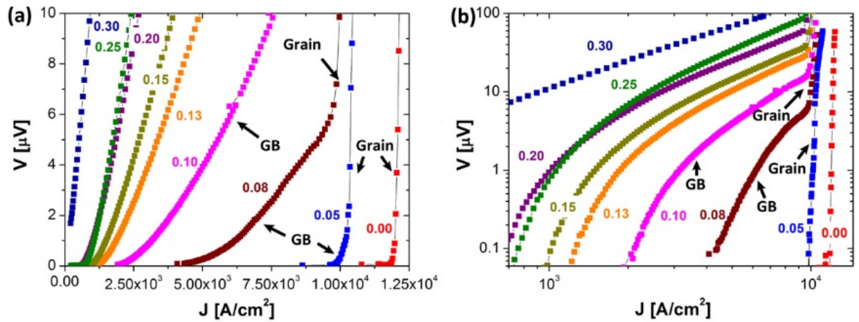
Figure 5. V - J characteristics of the mechanically smoothed bi-crystal (BC4) in (a) linear and (b) log-log scale at 4.2 K. The quasi-linearities in (a) are very similar to those of the BCP'ed bi-crystal (BC1) shown in Figure. 2b). The inset number represents external magnetic field (Tesla).
