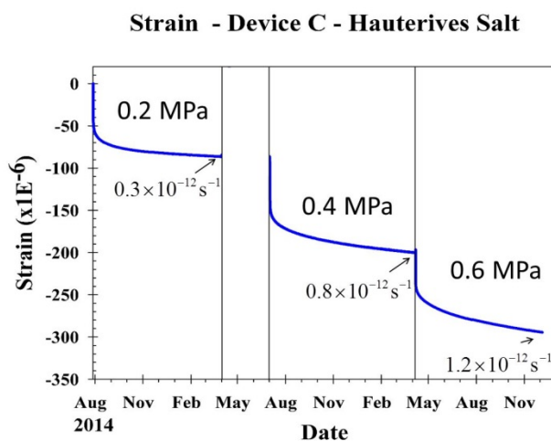
Figure 1. A three-stage, two-year long creep test on a Hauterives salt sample.
