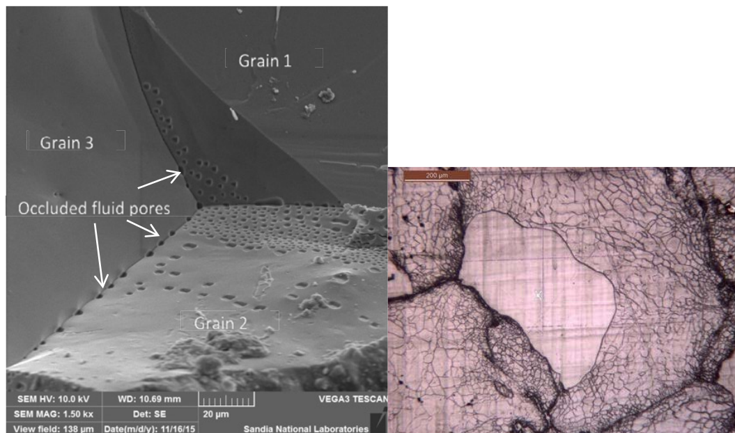
Figure 4-2. a. Occluded pore structure of reconsolidated salt (Stormont et al., 2017). b. Recrystallization.
