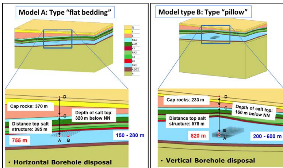
Figure 5-1. Generic sites (3D-models) of bedded salt formations with detail sections showing examples of repository design used for integrity analysis: left) model type A “flat-bedded salt,” right) model type B “salt pillow.”
