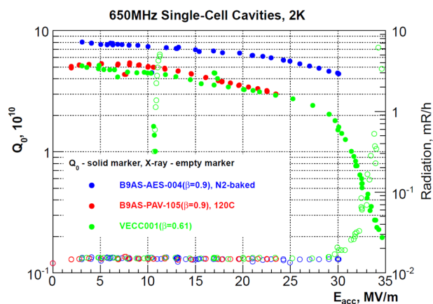
Figure 3: Single-cell 650 MHz cavity vertical test results.
