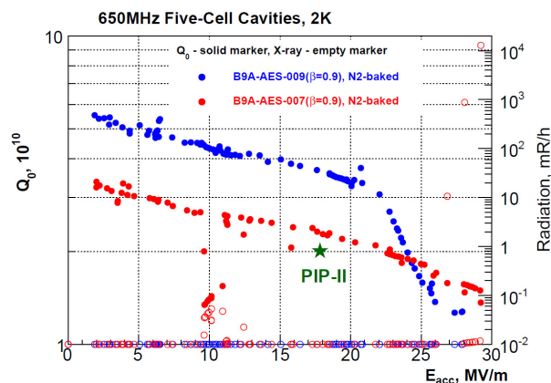
Figure 4: Five-cell B=0.90 650 MHz cavity test results.
