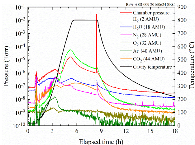
Figure 2: RGA plot of an 800^\circ\text{C} heat treatment with nitrogen doping of a 650 MHz 5-cell cavity.
