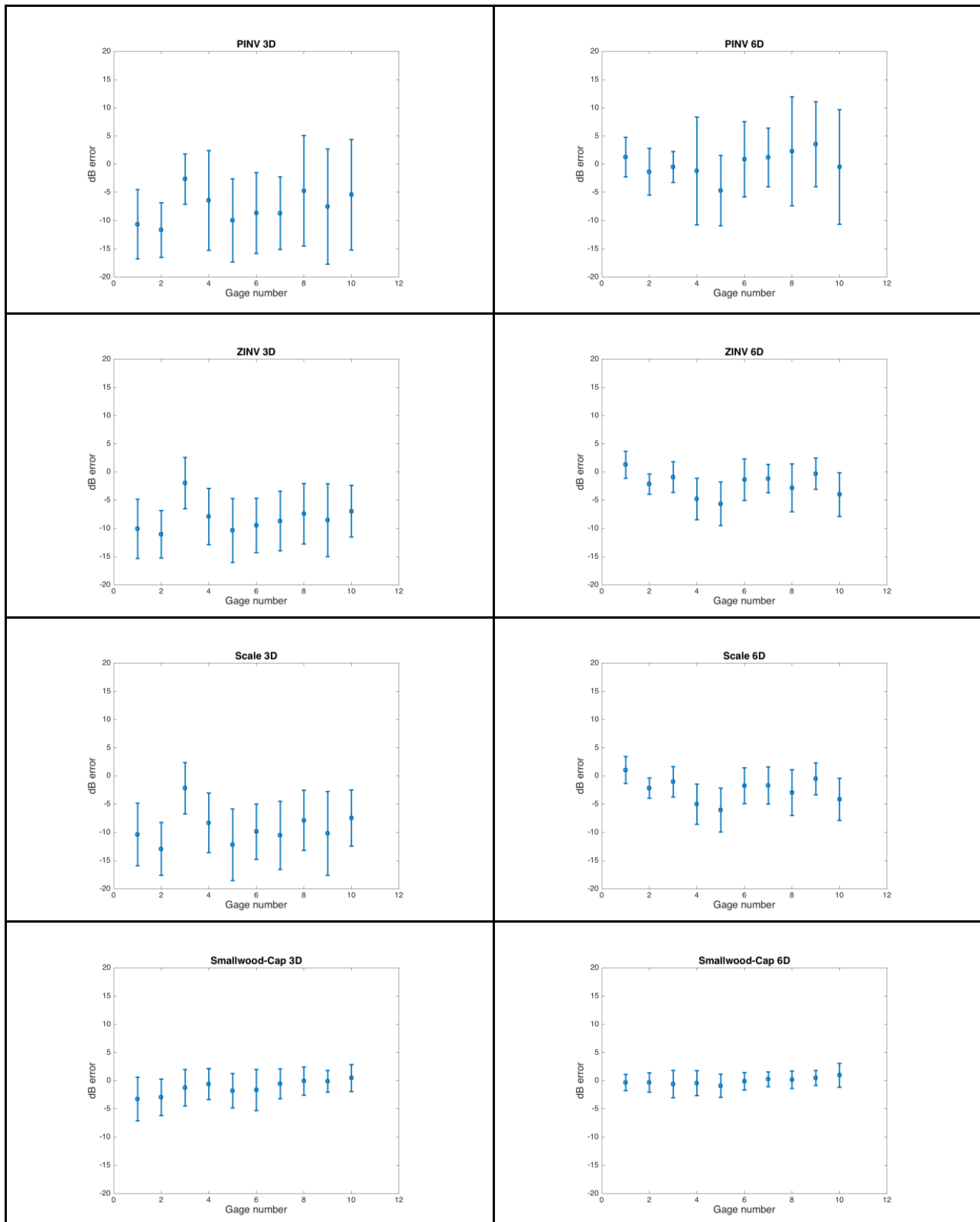
Fig. 6 Error comparisons in terms of decibels at each gage for each method
