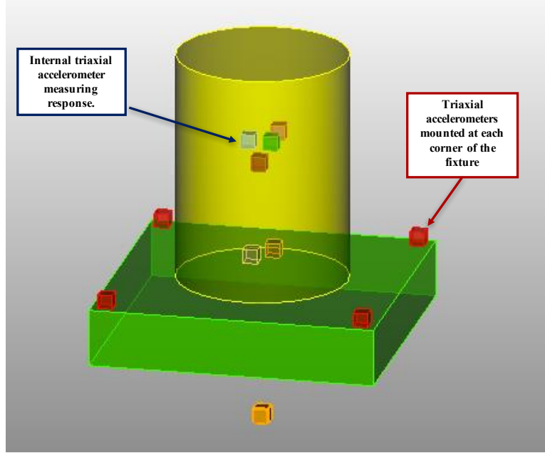
Fig. 2 Notional depiction of internal accelerometers
