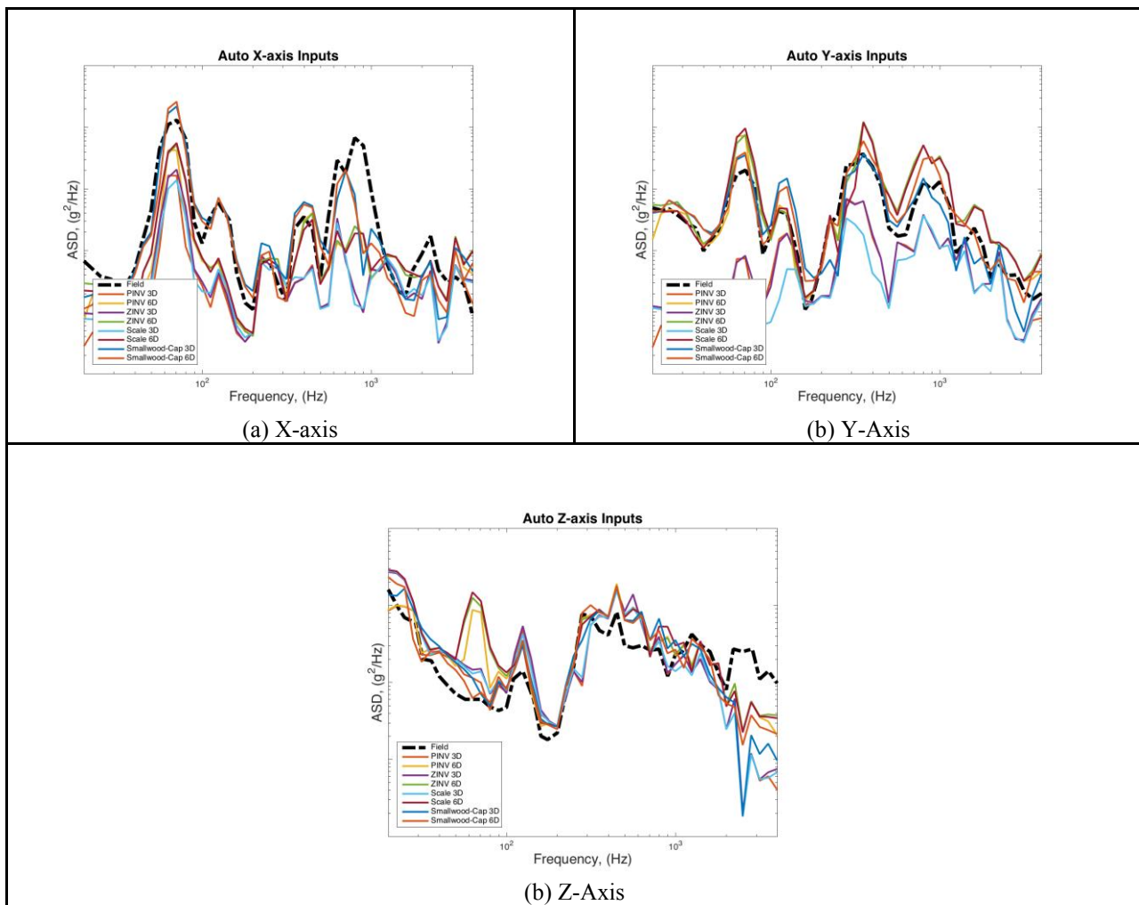
Fig. 3 Input comparisons of the different methods to the field data recommended input for translational values
