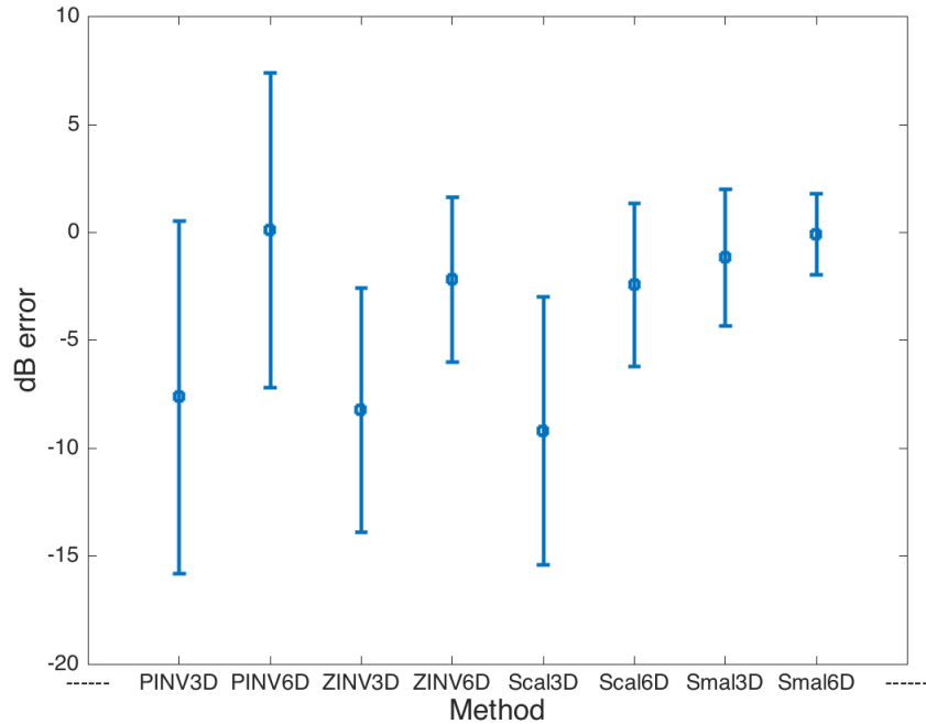
Fig. 7 Overall error comparisons among the different methods
