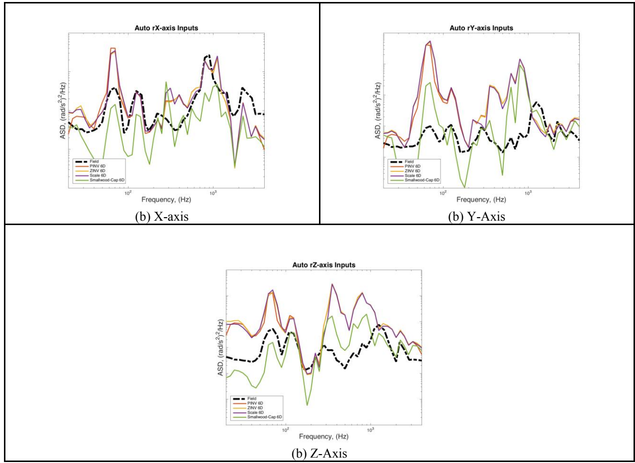
Fig. 4 Input comparisons of the different methods to the field data recommended input for rotational values
