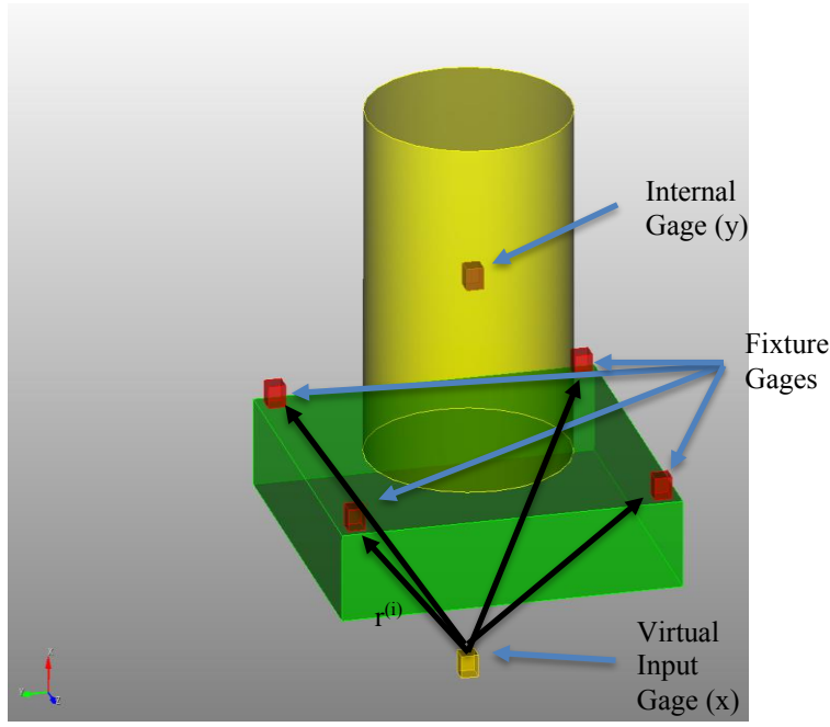
Fig. 1 Experimental set-up with fixture gages and a virtual input gage used to derive the transmissibility function
