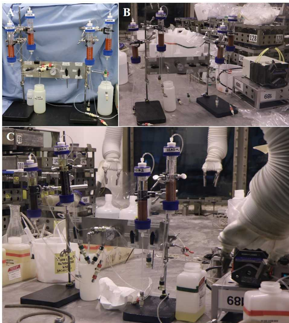
Figure 3-3. Ion Exchange Column and Manifold System.
