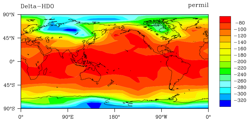
Figure 2: A map of water vapor \delta\text{D} at approximately 760 mb, as simulated by CAM5 with isotope-enabled cloud physics schemes and isotopic fractionation produced by oceanic evaporation.
