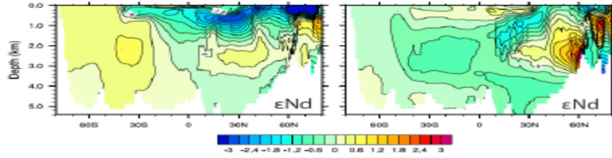
Figure 8: The difference of the simulated abiotic \epsilon\text{Nd} in the ocean wiso-TRACE21 simulation. The left column shows the difference between 16ka and 19ka, representing the H1 event, and the right column shows the difference between 14.35ka and 19ka, representing the BA transition from the LGM.
