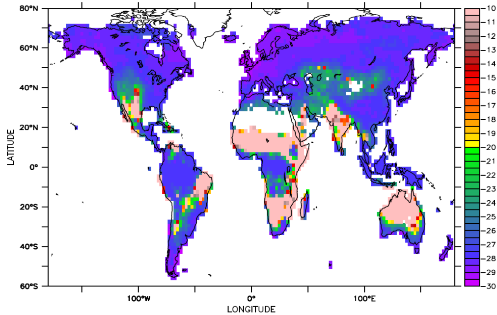
Figure 7: Global \delta^{13}\text{C} of the Total Vegetation at the end of the spin-up. This map shows a 25-year average over the end of the previous slide. The time frame to be averaged is selected to reflect the repetition loop of the applied climatology fields.
