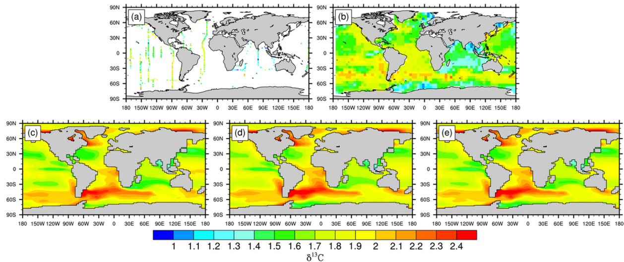
Figure 6. Surface values of \delta^{13}\text{C} for the 1990s from (a) cruise data compiled by Schmittner et al., (b) 5^\circ extrapolated gridded data from Gruber and Keeling (1999) and Gruber and Keeling (2001), and (c–e) the biotic model, using the biological fractionation from (c) Rau et al. (Nature, 1989), (d) Laws et al. (Geochem. Cosmochim. Ac., 1995), and (e) Keller and Morel (Mar. Ecol.-Prog.Ser., 1999).
