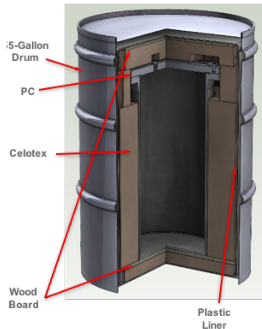
Figure 1: Components of the Pipe Overpack Container (POC). As shown, the inner metal container is called the Pipe Container (PC).
