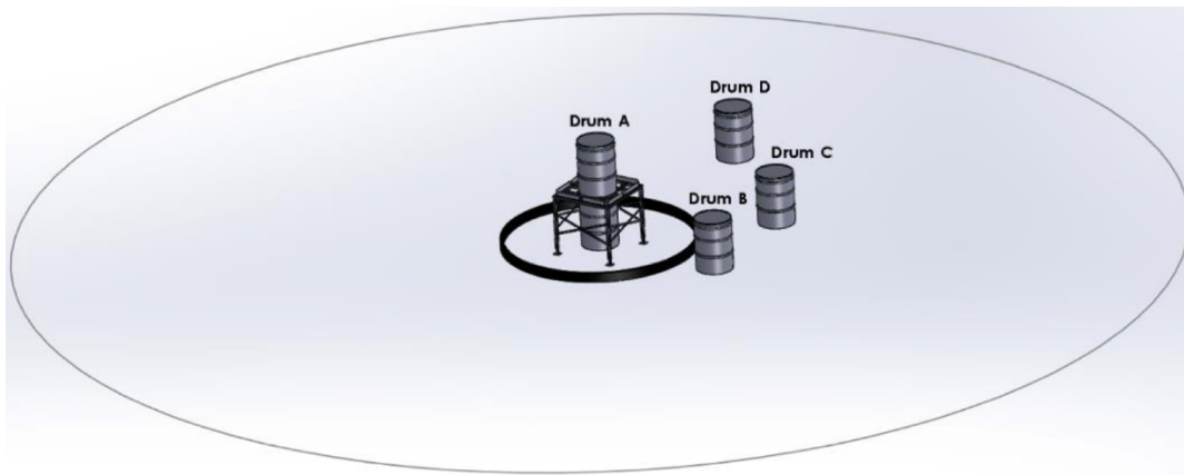
Figure 4. Layout of indoor POC tests in the FLAME facility. The inner circular wall marks the edge of the pool; the outer circular line marks the edge of the floor in the FLAME facility.
