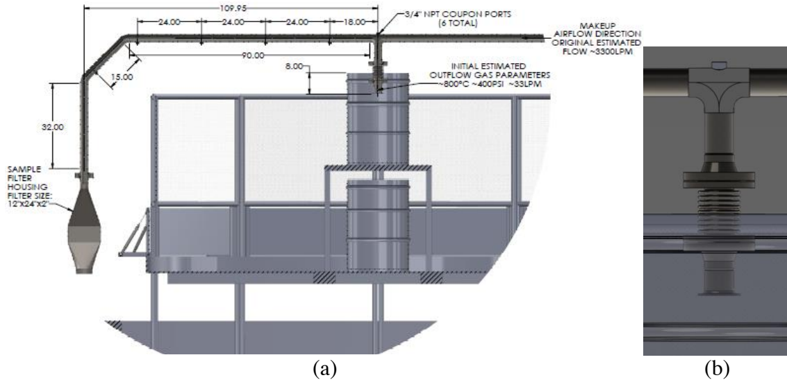
Figure 9. (a) Schematics of the aerosol system showing the outlet HEPA filter and the location of the coupons. Not shown is the inlet end of the U-shaped pipe which mirrors the outlet end shown. (b) Close-up of the vertical section of the pipe. Contents of the POC drum are not shown. All length units are in inches.
