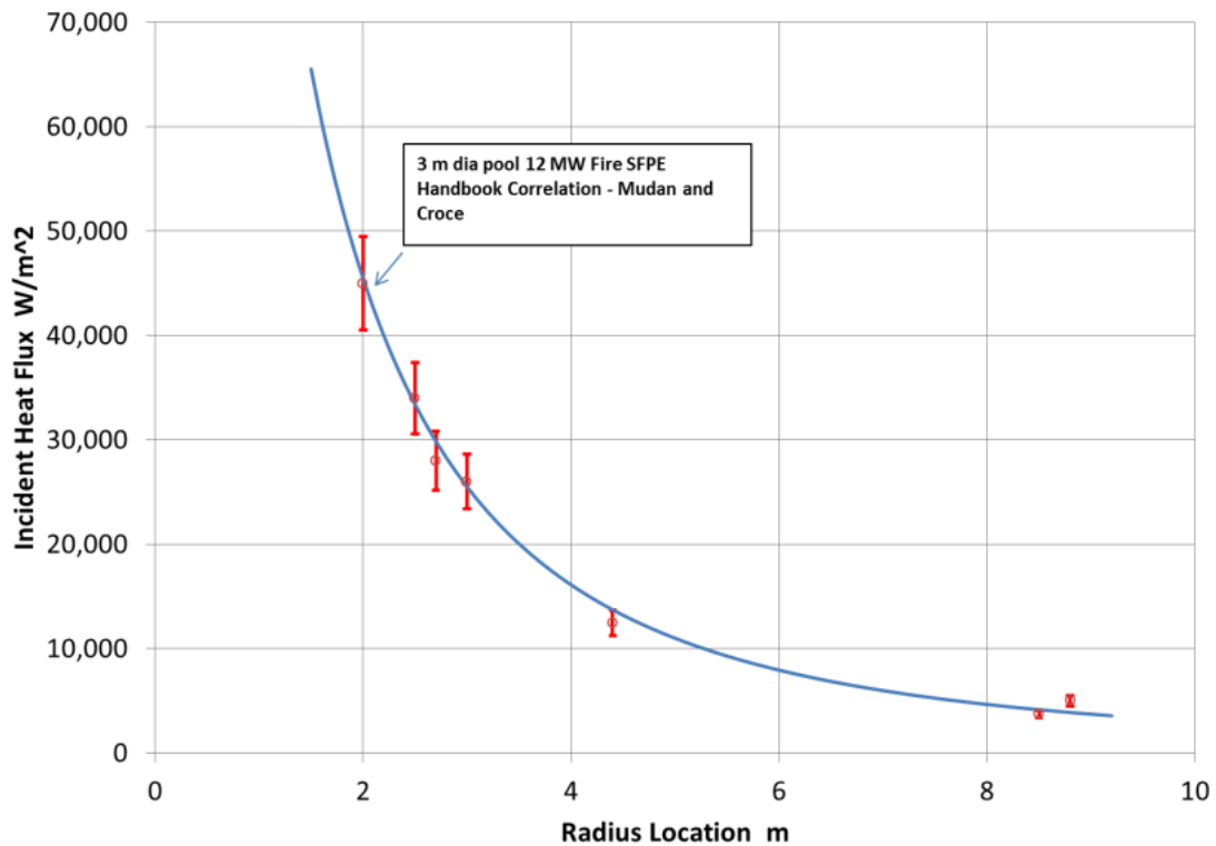
Figure 13. Incident heat fluxes (red) recorded with HFGs for various test and at various distances. Superimposed on the data are correlation results for typical incident radiation from a fire plume as a function of distance.
