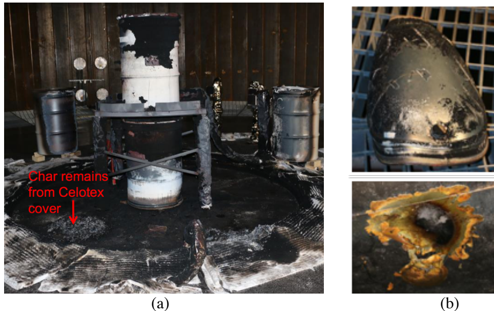
Figure 10. (a) View of center drum after the fire. Also showing are the remains of top Celotex cover ash remains inside the fuel pool. (b) Close-up view of the ejected lid (top) and the remains of the plastic liner cover (bottom) on the test cell floor.
