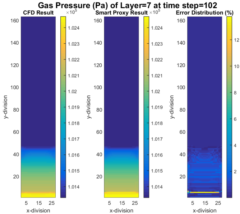
Figure 4-8 CFD and smart proxy results for gas pressure at K = 7 cross-sectional plane
