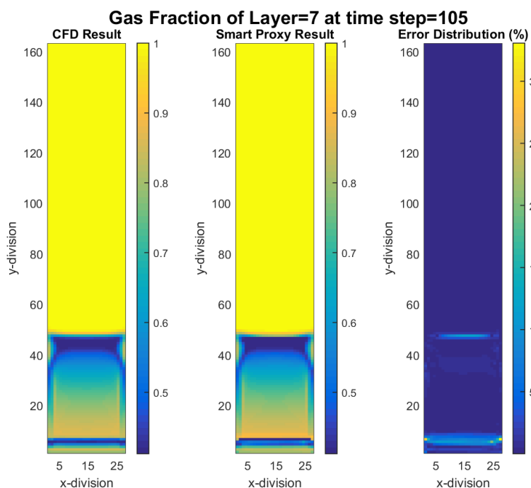
Figure 4-21 CFD and cascading smart proxy results for gas volume fraction at K = 7 cross-sectional plane and time step = 105
