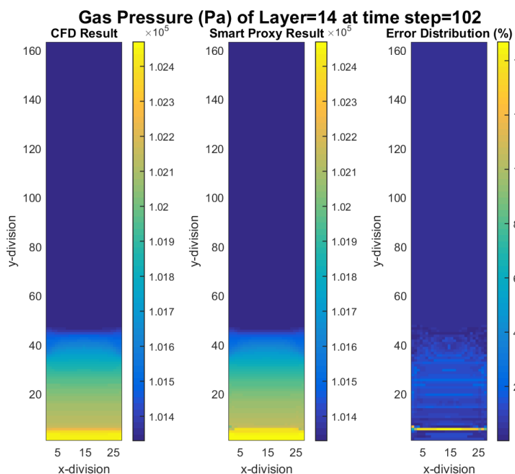
Figure 4-9 CFD and smart proxy results for gas pressure at K = 14 cross-sectional plane
