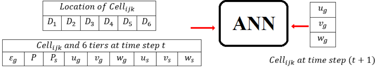
Figure 3-18 Training with multiple outputs (3 components of gas velocity)
