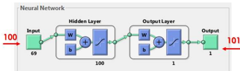
Figure 3-12 Input at time step 100 and CFD output at time step 101 used for training (early time, startup)
