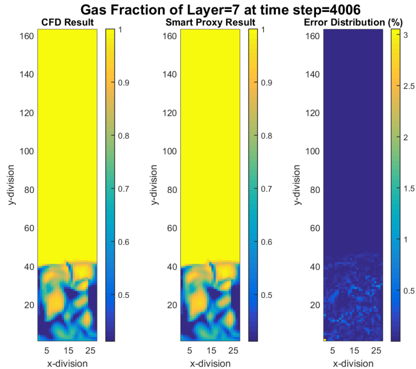
Figure 9-1 CFD and smart proxy results for gas volume fraction at K = 7 cross-sectional plane and time step = 4006
