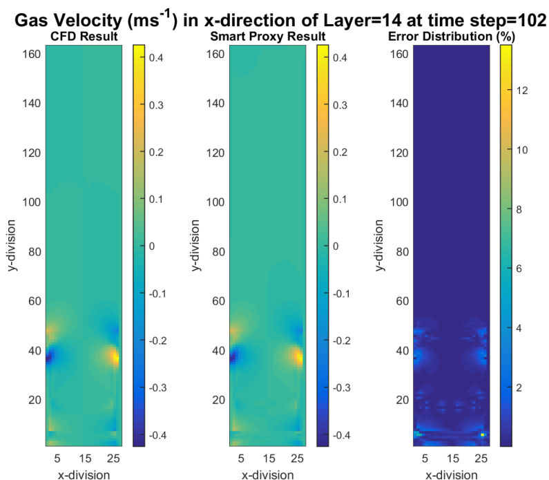
Figure 8-2 CFD and smart proxy results for x-component of gas velocity at K = 14 cross-sectional plane
