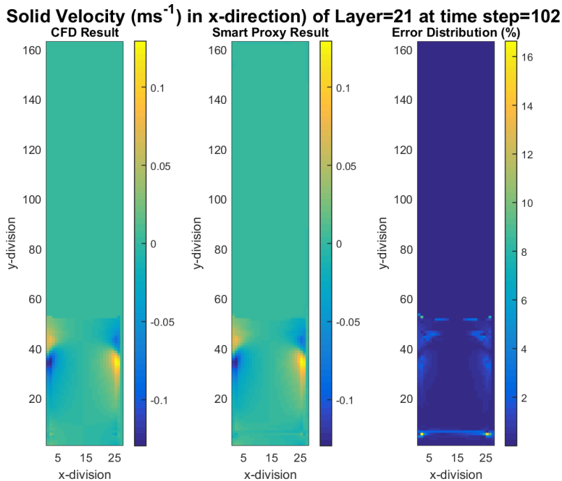
Figure 8-7 CFD and smart proxy results for x-component of solid velocity at K = 21 cross-sectional plane
