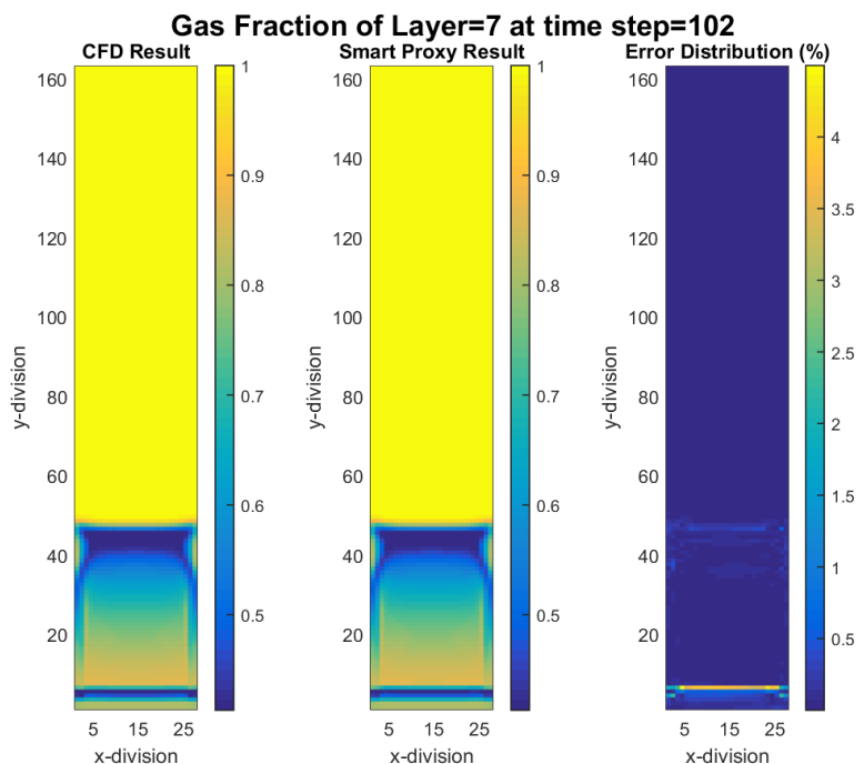
Figure 4-18 CFD and cascading smart proxy results for gas volume fraction at K = 7 cross-sectional plane and time step = 102
