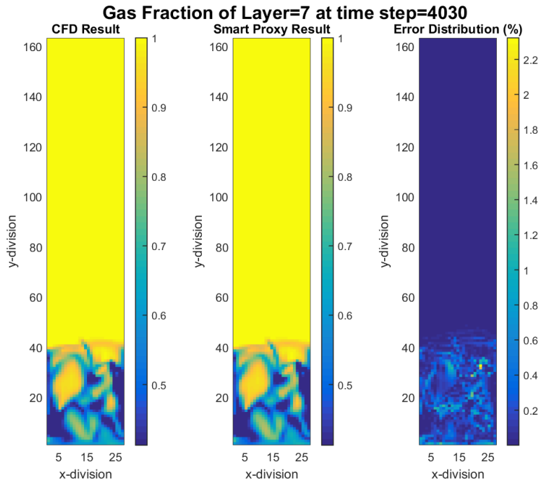
Figure 9-8 CFD and smart proxy results for gas volume fraction at K = 7 cross-sectional plane and time step = 4030
