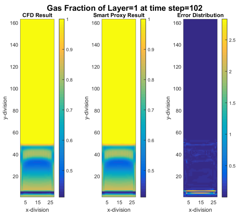
Figure 4-2 CFD and smart proxy results for gas volume fraction at K = 1 cross-sectional plane
