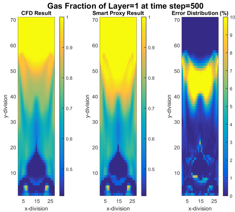
Figure 4-38 CFD and smart proxy results for gas volume fraction at K = 1 cross-sectional plane
