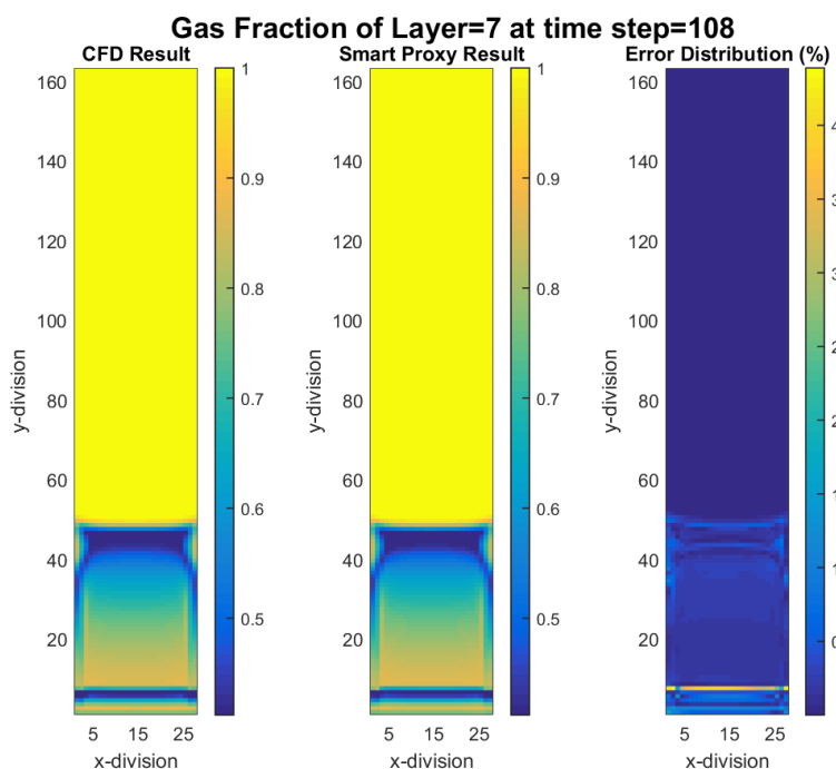
Figure 7-6 CFD and smart proxy results for gas volume fraction at K = 7 cross-sectional plane and time step = 108
