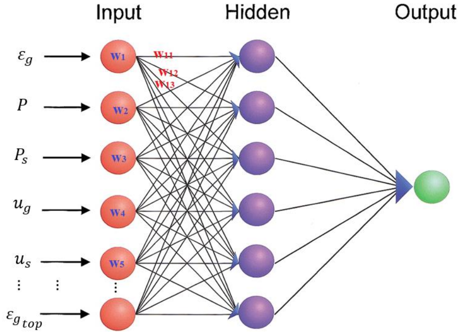
Figure 3-25 Network schematic with its weights
