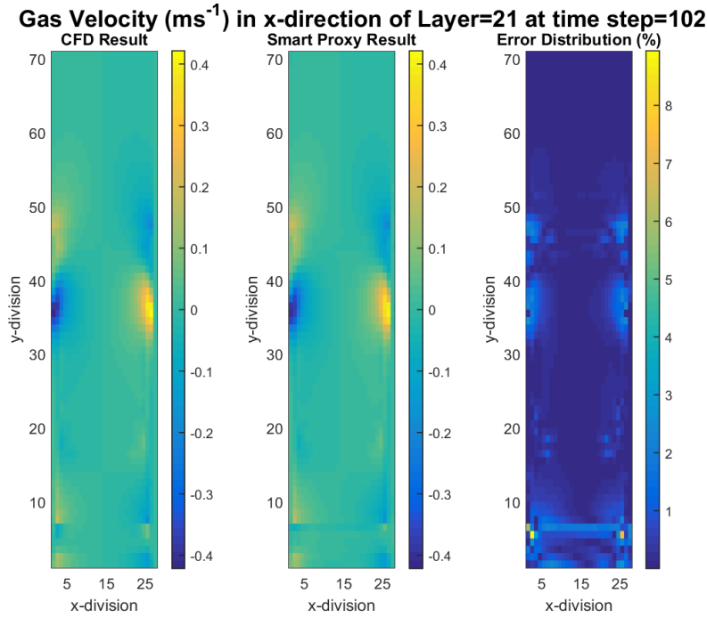
Figure 4-34 CFD and smart proxy results for x-component of gas velocity at K = 21 cross-sectional plane, based on implicitly constructed ANN
