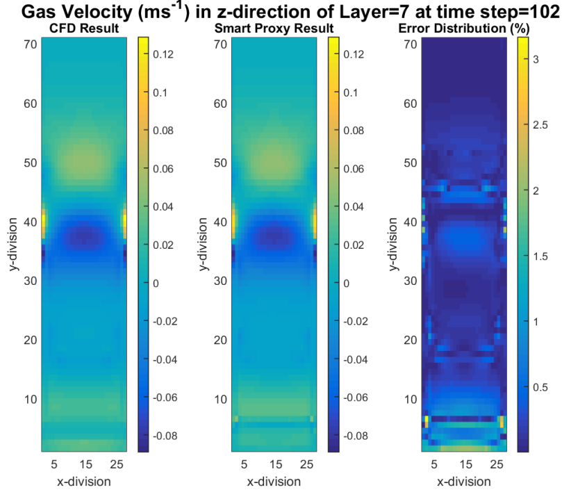
Figure 4-36 CFD and smart proxy results for z-component of gas velocity at K = 7 cross-sectional plane, based on implicitly constructed ANN
