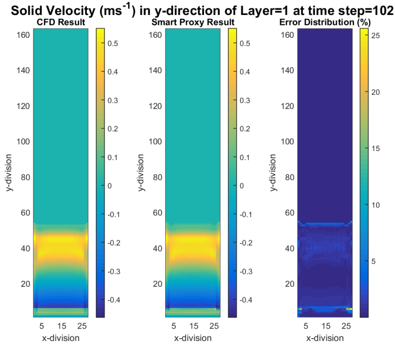
Figure 8-8 CFD and smart proxy results for y-component of solid velocity at K = 1 cross-sectional plane
