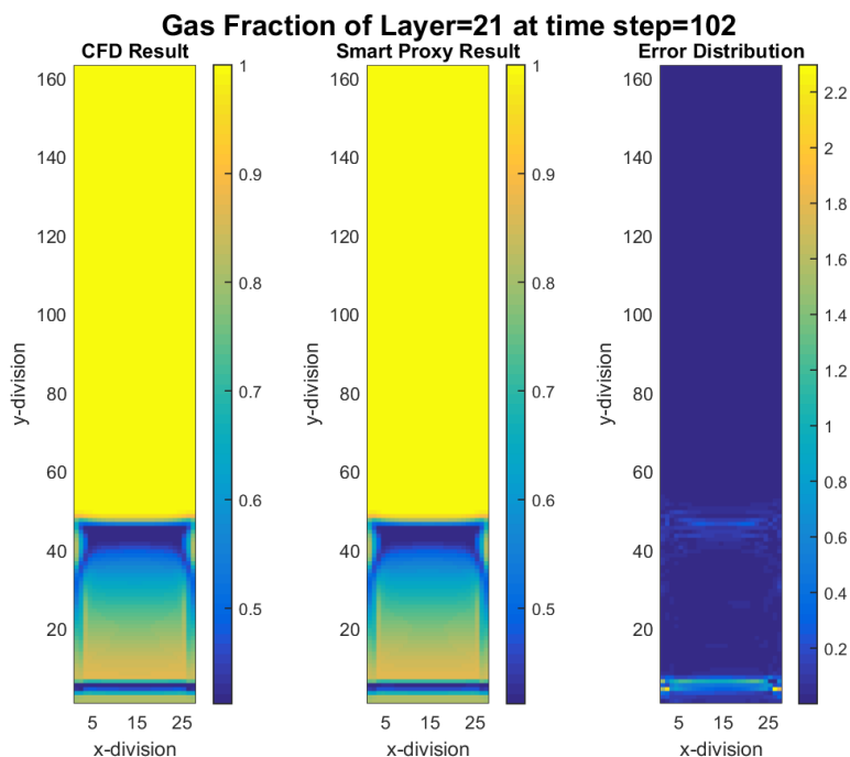
Figure 4-5 CFD and smart proxy results for gas volume fraction at K = 21 cross-sectional plane
