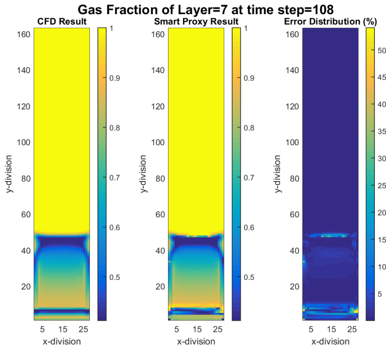
Figure 4-24 CFD and cascading smart proxy results for gas volume fraction at K = 7 cross-sectional plane and time step = 108
