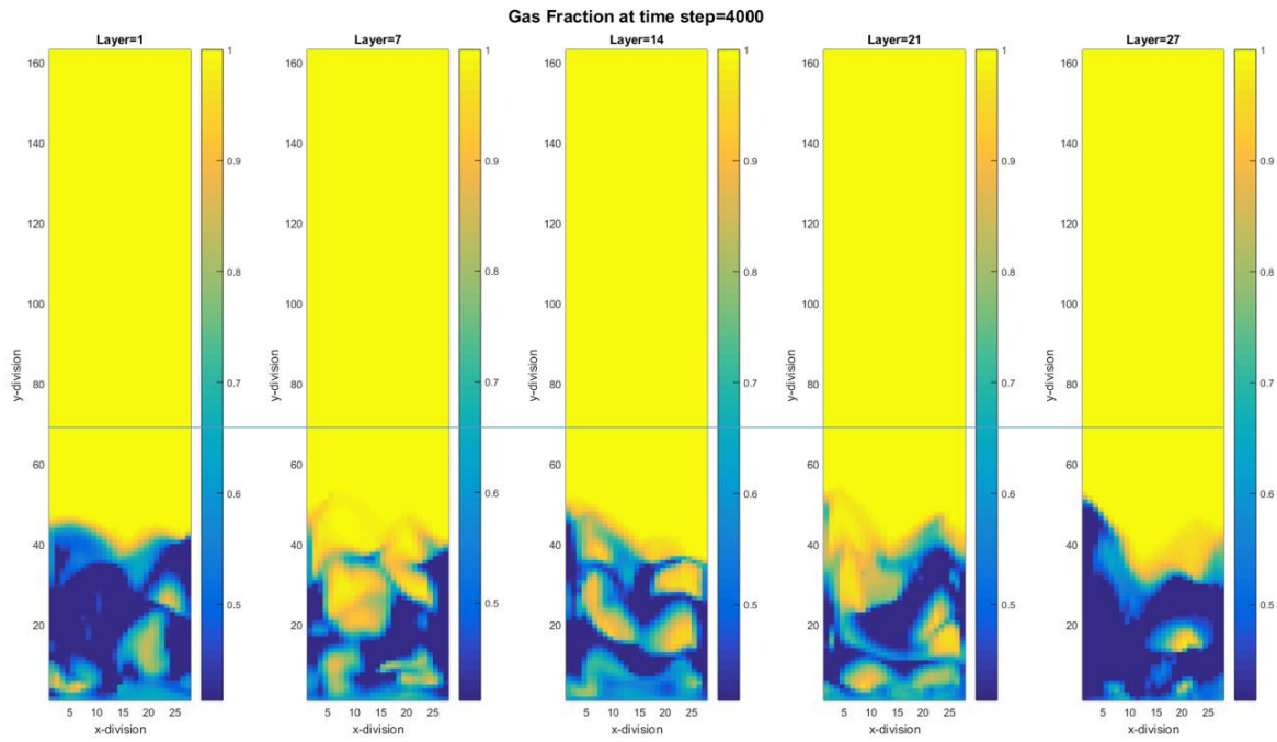
Figure 3-23 Gas volume fraction contours at time-step 4000
