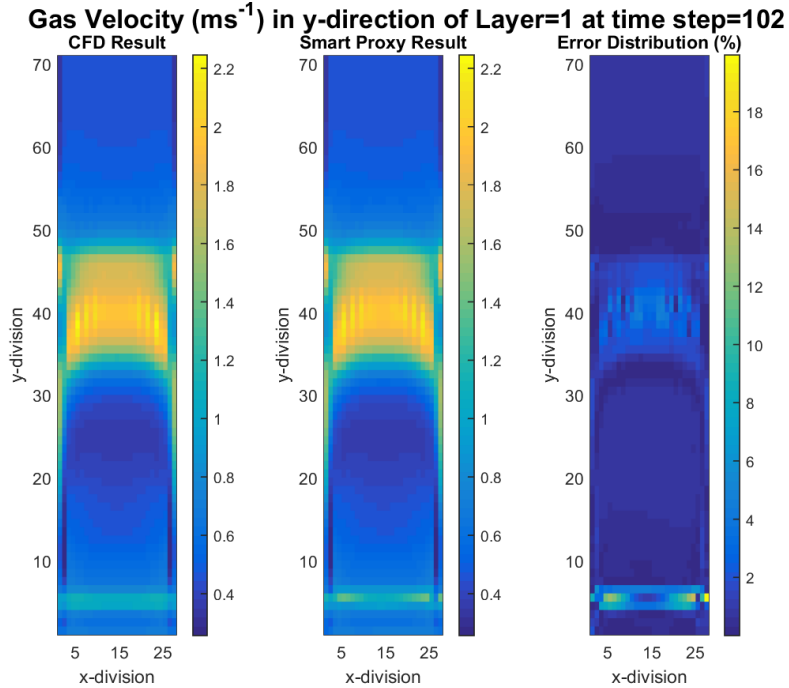
Figure 4-32 CFD and smart proxy results for y-component of gas velocity at K = 1 cross-sectional plane, based on explicitly constructed ANN
