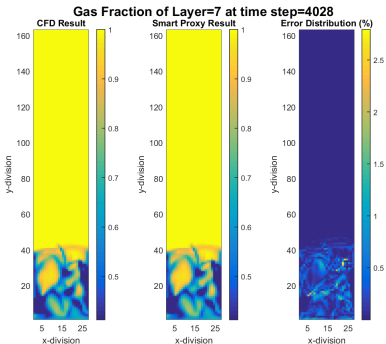
Figure 9-7 CFD and smart proxy results for gas volume fraction at K = 7 cross-sectional plane and time step = 4028
