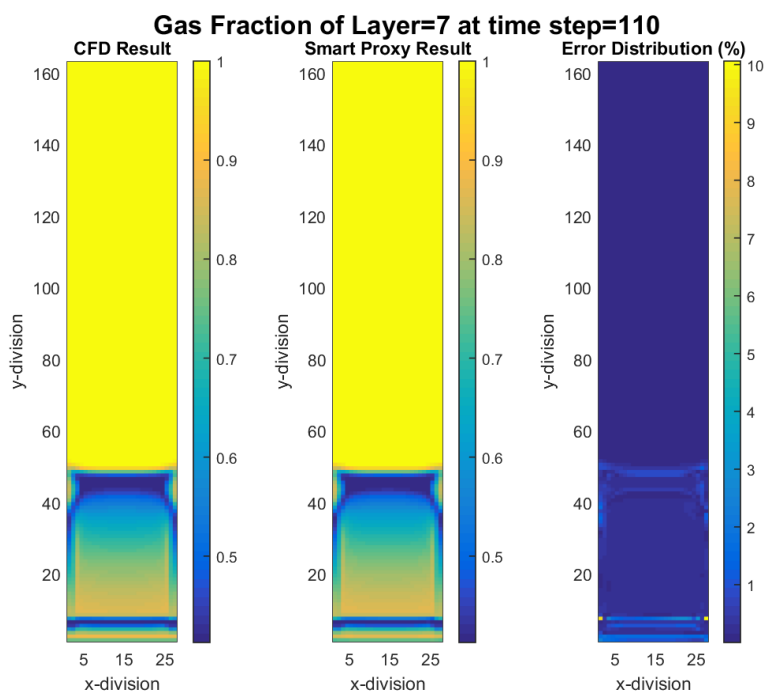
Figure 7-8 CFD and smart proxy results for gas volume fraction at K = 7 cross-sectional plane and time step = 110
