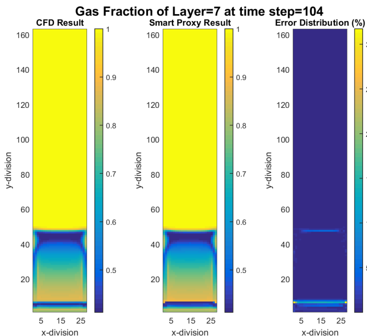
Figure 4-20 CFD and cascading smart proxy results for gas volume fraction at K = 7 cross-sectional plane and time step = 104
