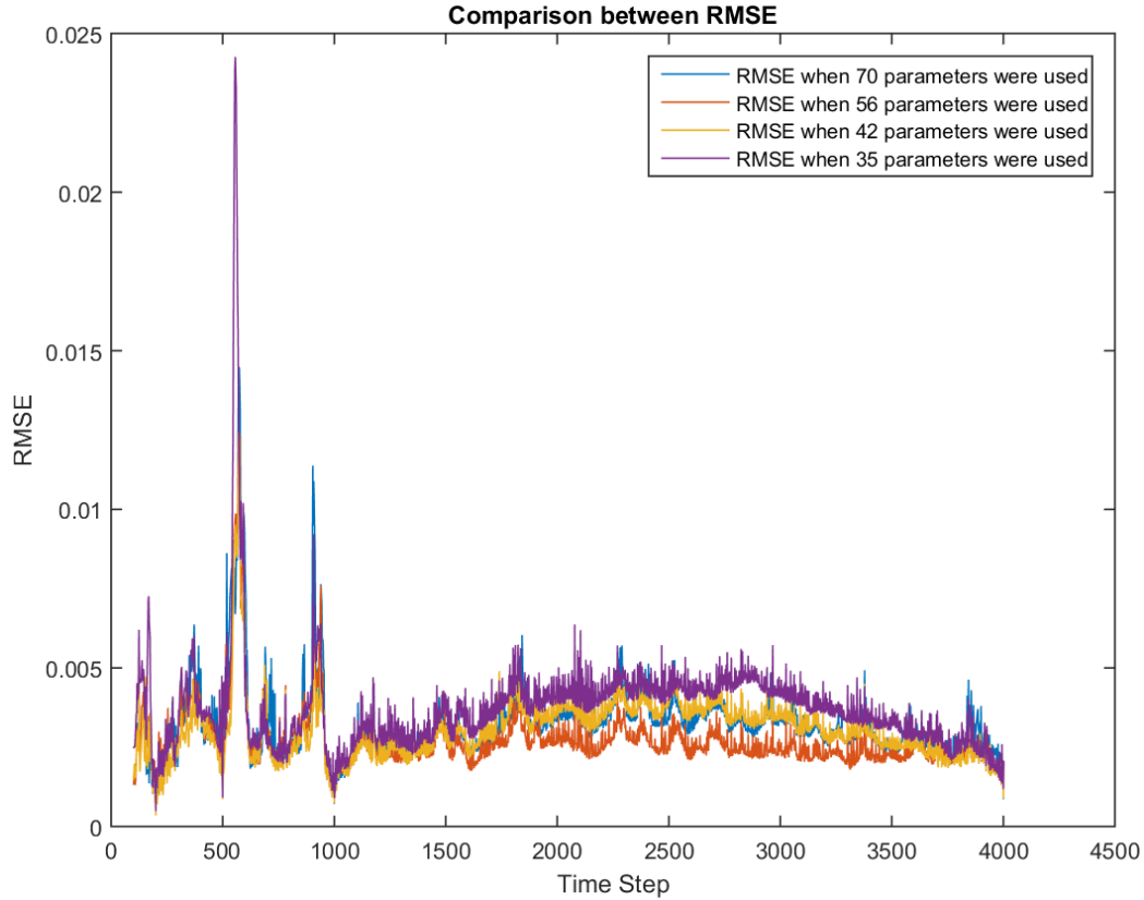
Figure 4-43 RMSE distribution with different parameters used for training
