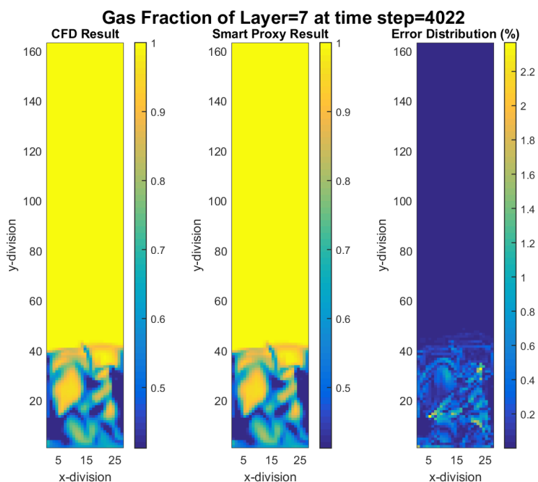
Figure 9-6 CFD and smart proxy results for gas volume fraction at K = 7 cross-sectional plane and time step = 4022
