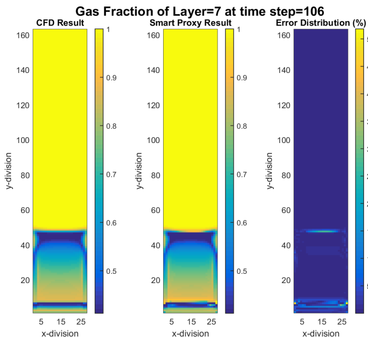
Figure 4-22 CFD and cascading smart proxy results for gas volume fraction at K = 7 cross-sectional plane and time step = 106
