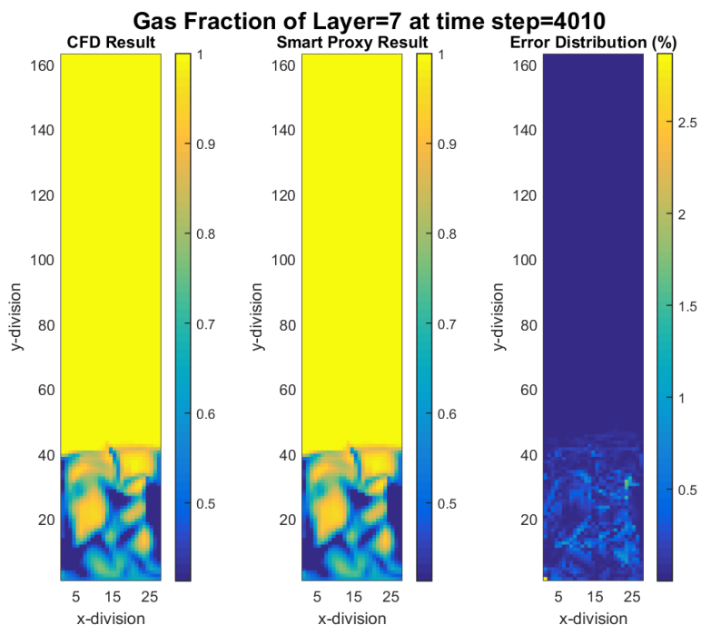
Figure 9-3 CFD and smart proxy results for gas volume fraction at K = 7 cross-sectional plane and time step = 4010
