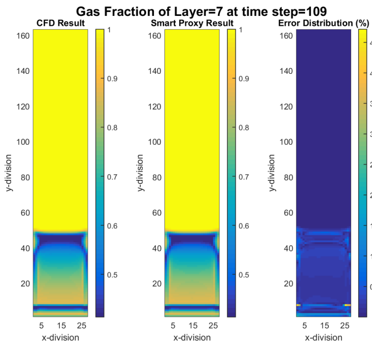
Figure 7-7 CFD and smart proxy results for gas volume fraction at K = 7 cross-sectional plane and time step = 109
