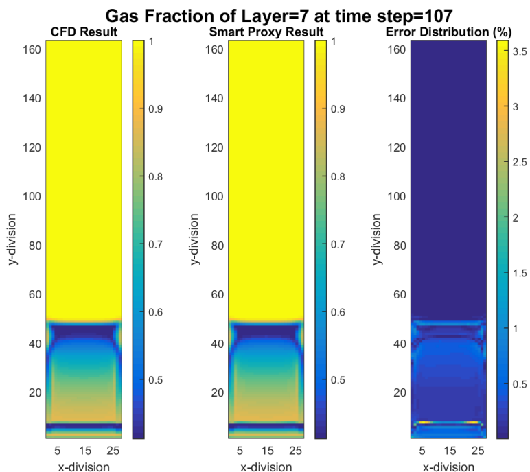
Figure 7-5 CFD and smart proxy results for gas volume fraction at K = 7 cross-sectional plane and time step = 107
