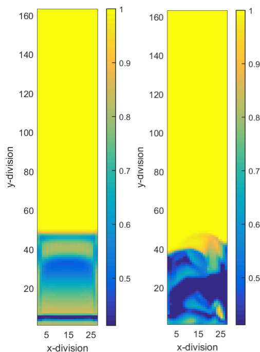
Figure 3-11 Gas volume fraction distribution initially in the bed (left) and later when it is fully fluidized (right)
