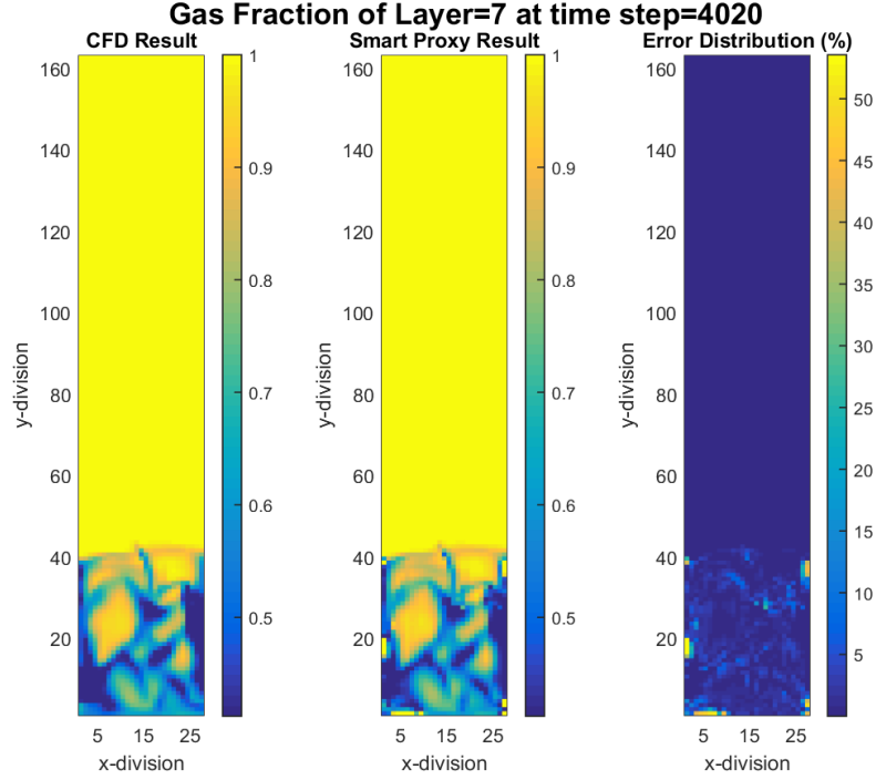
Figure 4-30 CFD and cascading smart proxy results for gas volume fraction at K = 7 cross-sectional plane and time step = 4020
