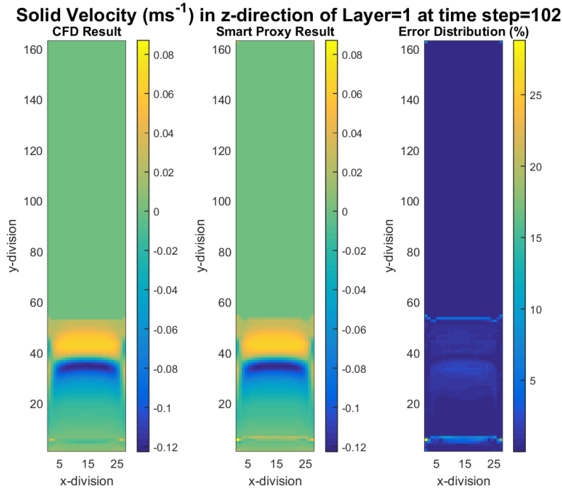
Figure 8-10 CFD and smart proxy results for z-component of solid velocity at K = 1 cross-sectional plane
