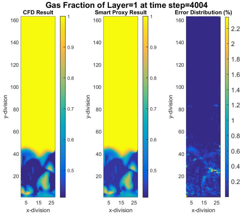
Figure 4-46 CFD and non-cascading smart proxy results for gas volume fraction at K = 1 cross-sectional plane with 60% of data used for training
