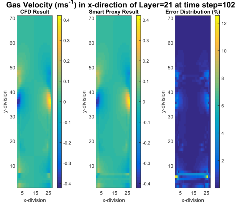
Figure 4-31 CFD and smart proxy results for x-component of gas velocity at K = 21 cross-sectional plane, based on explicitly constructed ANN
