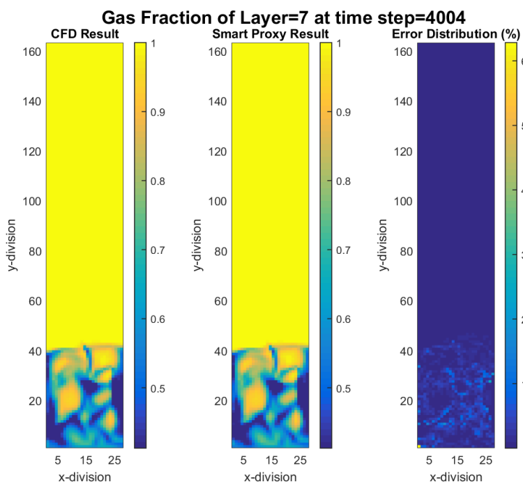
Figure 4-28 CFD and cascading smart proxy results for gas volume fraction at K = 7 cross-sectional plane and time step = 4004
