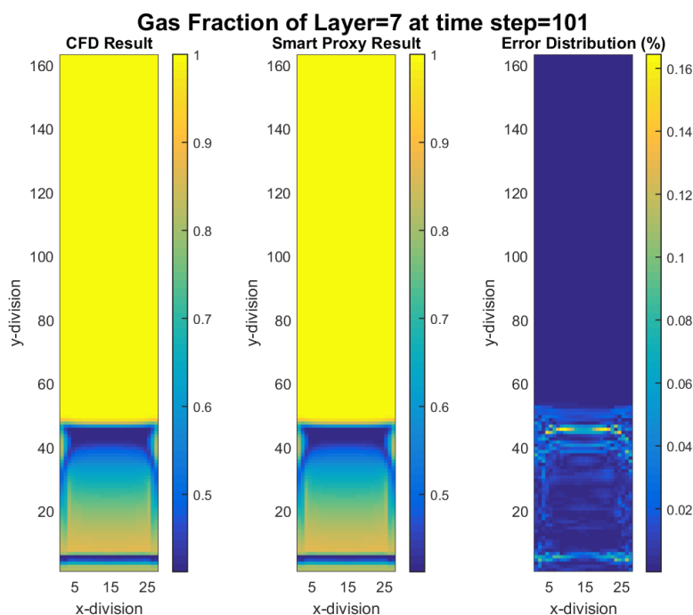
Figure 4-17 CFD and cascading smart proxy results for gas volume fraction at K = 7 cross-sectional plane and time step = 101
