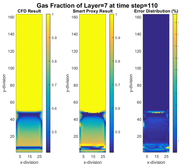
Figure 4-26 CFD and cascading smart proxy results for gas volume fraction at K = 7 cross-sectional plane and time step = 110
