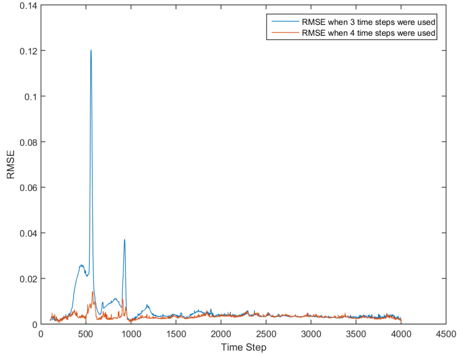
Figure 4-39 RMSE distribution over time, when four pairs of data are used for training
