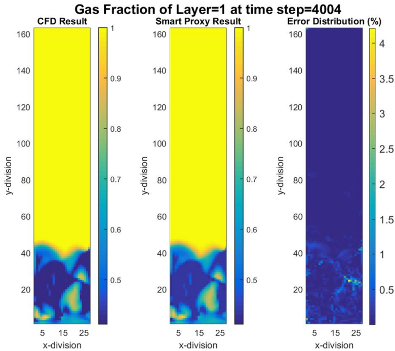
Figure 4-47 CFD and non-cascading smart proxy results for gas volume fraction at K = 1 cross-sectional plane with 40% of data used for training
