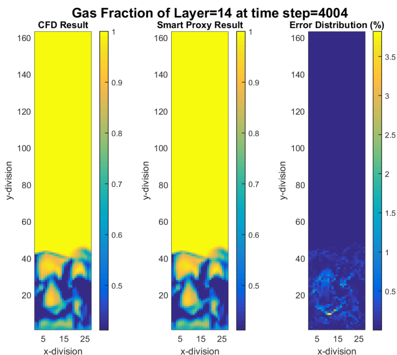
Figure 4-14 CFD and smart proxy results for gas volume fraction at K = 14 cross-sectional plane
