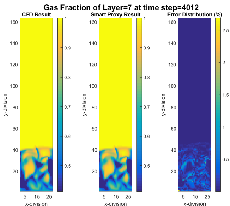
Figure 9-4 CFD and smart proxy results for gas volume fraction at K = 7 cross-sectional plane and time step = 4012
