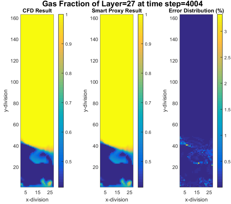
Figure 4-16 CFD and smart proxy results for gas volume fraction at K = 27 cross-sectional plane
