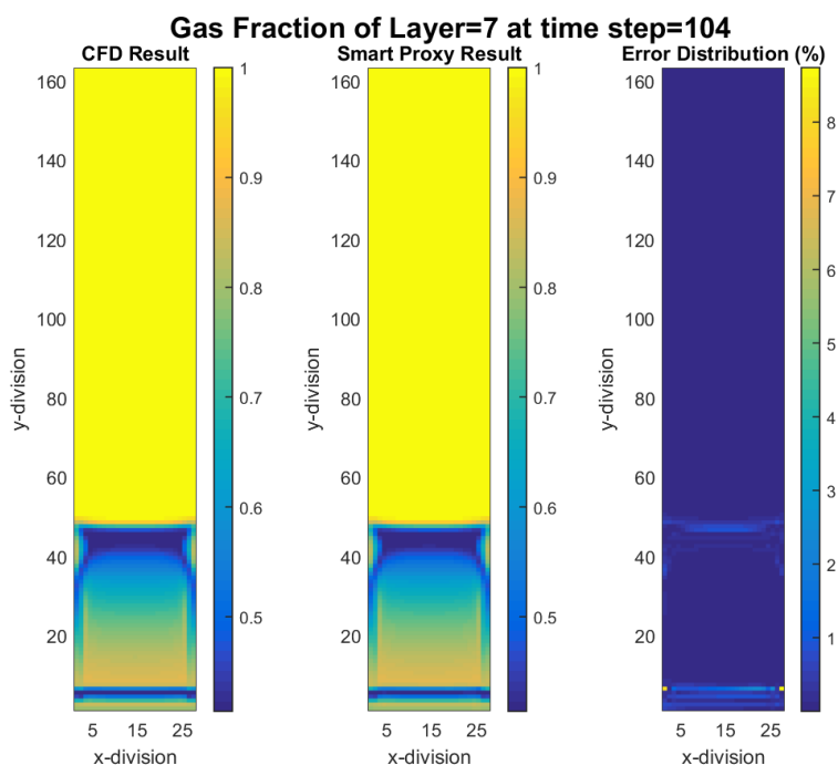
Figure 7-2 CFD and smart proxy results for gas volume fraction at K = 7 cross-sectional plane and time step = 104
