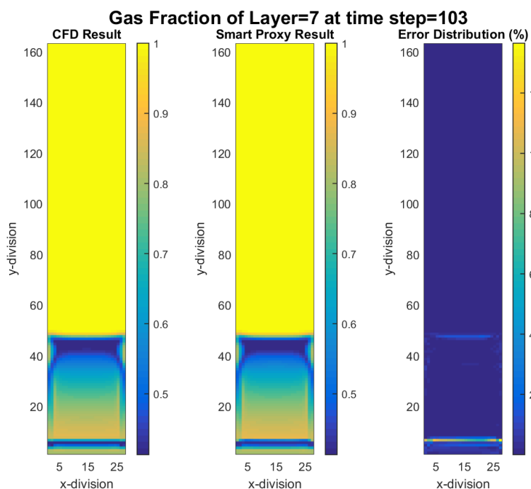
Figure 4-19 CFD and cascading smart proxy results for gas volume fraction at K = 7 cross-sectional plane and time step = 103
