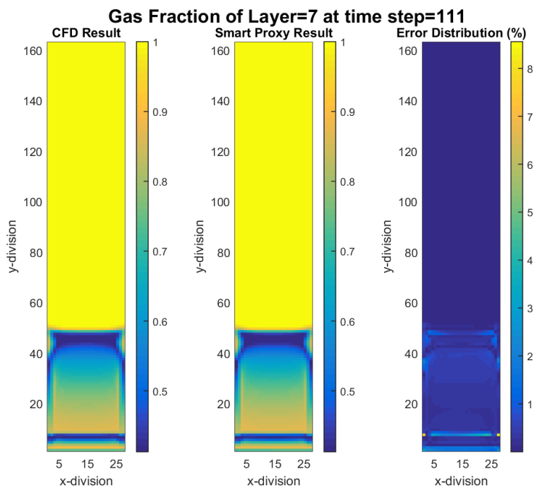
Figure 7-9 CFD and smart proxy results for gas volume fraction at K = 7 cross-sectional plane and time step = 111
