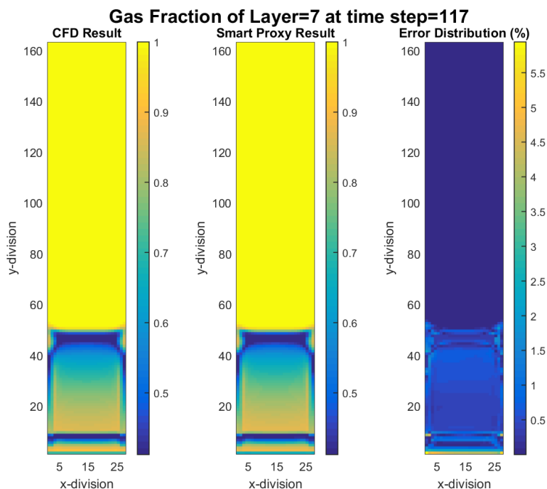
Figure 7-11 CFD and smart proxy results for gas volume fraction at K = 7 cross-sectional plane and time step = 117
