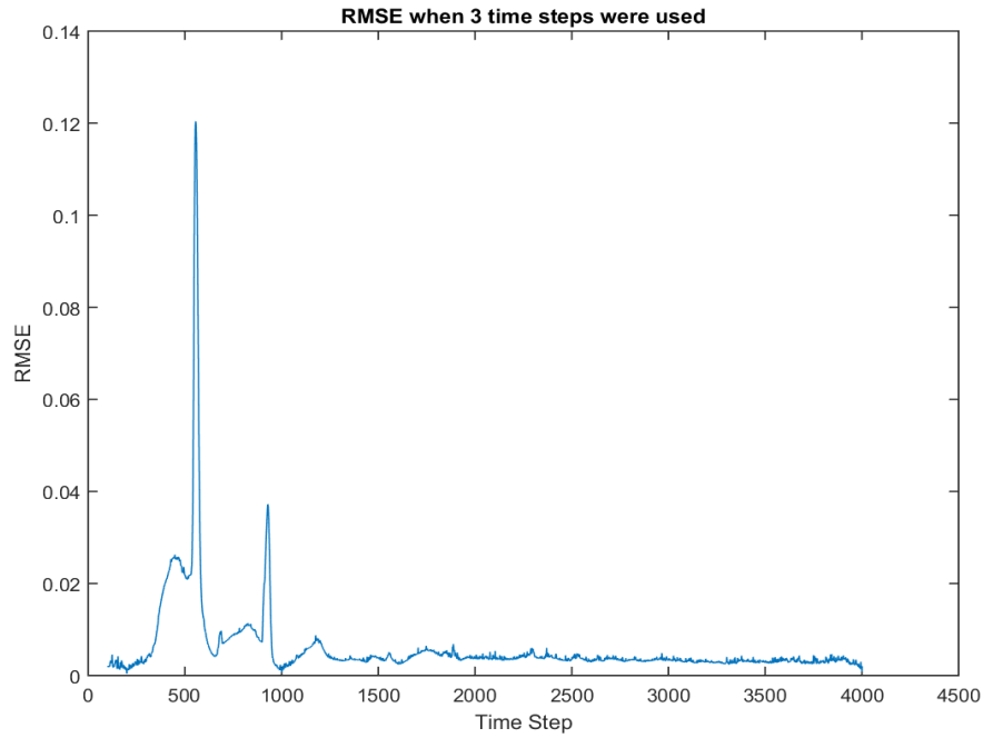
Figure 4-37 RMSE distribution over time, when three pairs of data are used for training
