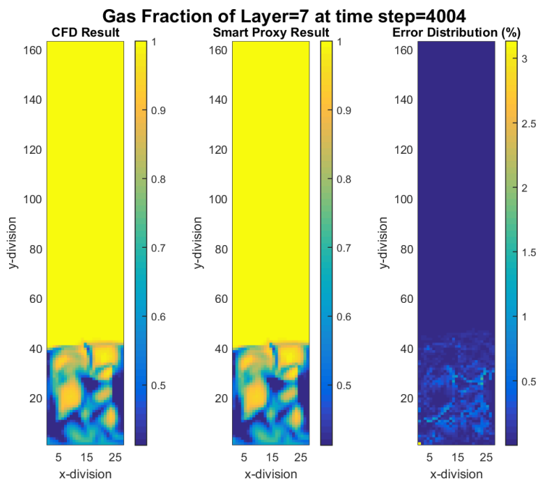
Figure 4-13 CFD and smart proxy results for gas volume fraction at K = 7 cross-sectional plane
