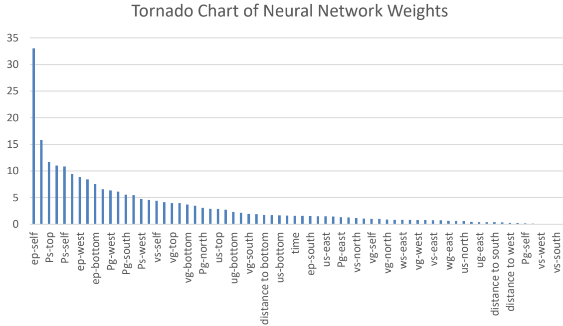
Figure 4-40 Parameters ranking for construction of gas volume fraction ANN, based on averaging all weights
