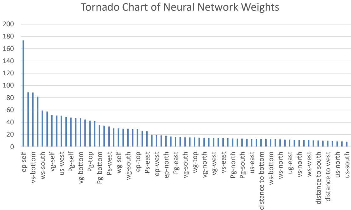
Figure 4-41 Parameters ranking for construction of gas volume fraction ANN, averaging of absolute value of all weights
