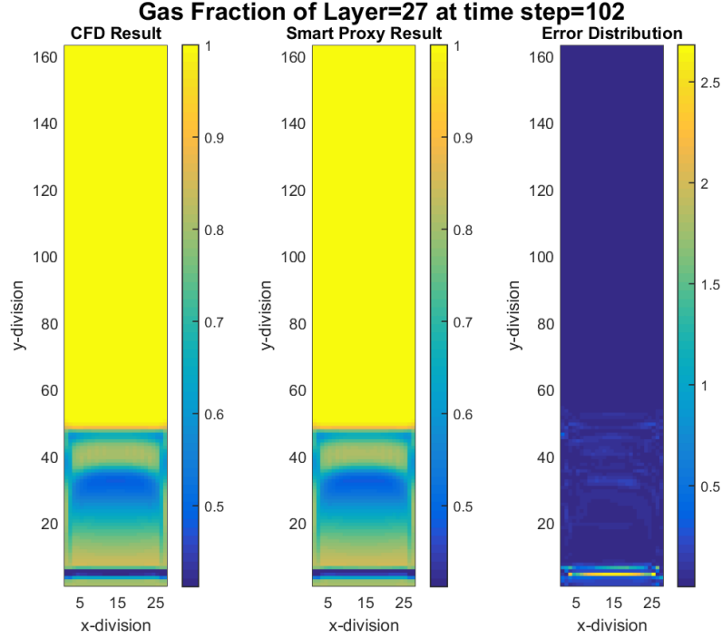
Figure 4-6 CFD and smart proxy results for gas volume fraction at K = 27 cross-sectional plane
