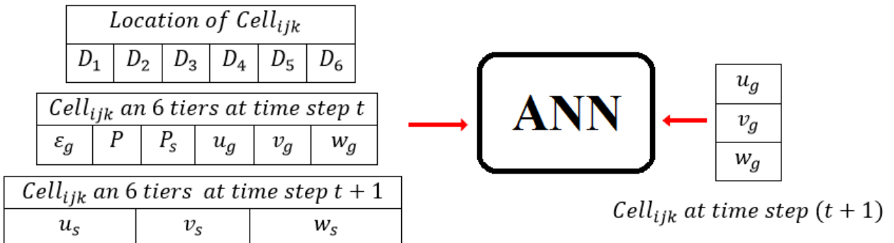
Figure 3-19 Training implicitly with multiple outputs
