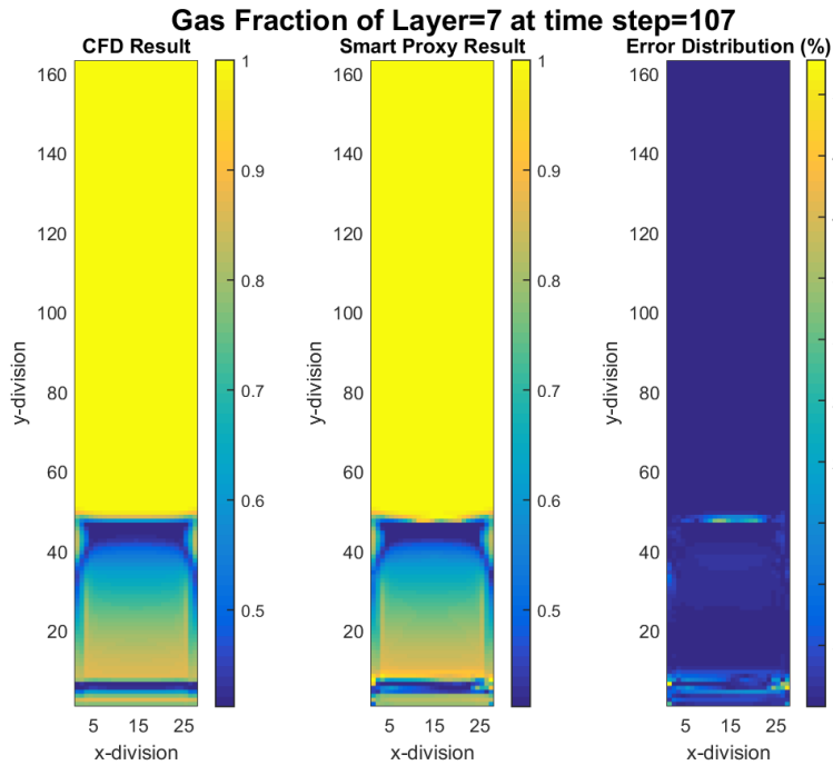
Figure 4-23 CFD and cascading smart proxy results for gas volume fraction at K = 7 cross-sectional plane and time step = 107
