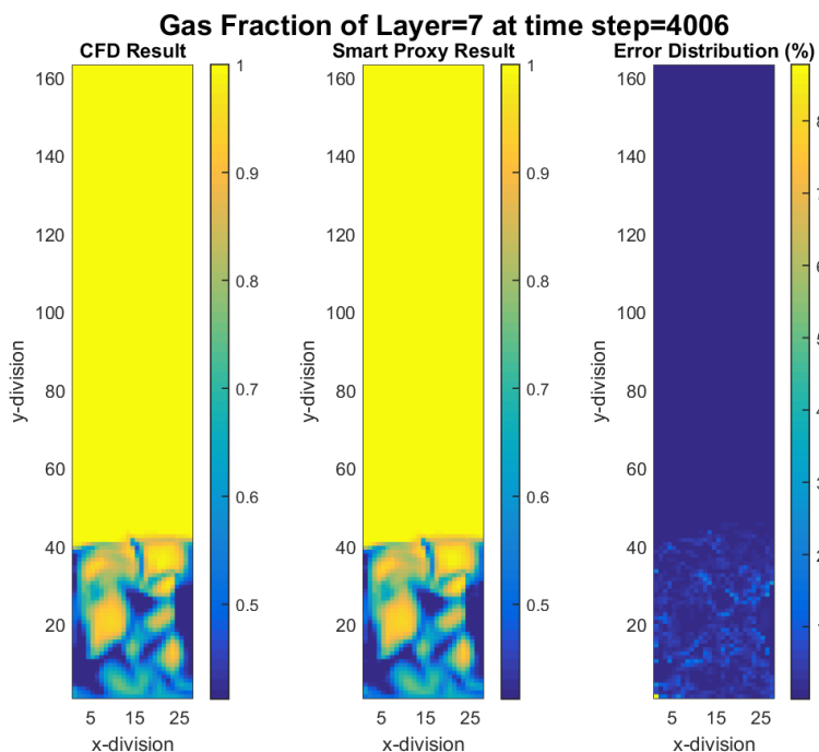
Figure 4-29 CFD and cascading smart proxy results for gas volume fraction at K = 7 cross-sectional plane and time step = 4006
