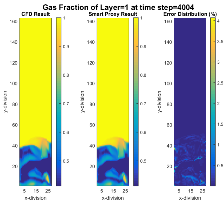
Figure 4-12 CFD and smart proxy results for gas volume fraction at K = 1 cross-sectional plane
