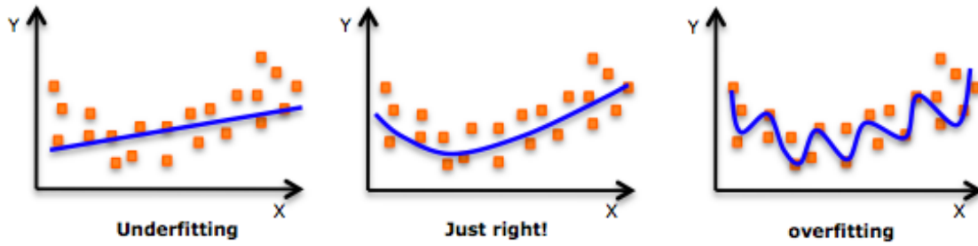
Figure 3-7 Underfitting and overfitting of the data
