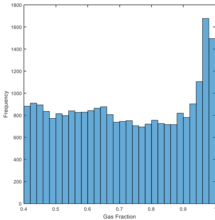
Figure 3-27 Distribution of gas volume fraction at time step 4000 after smart sampling
