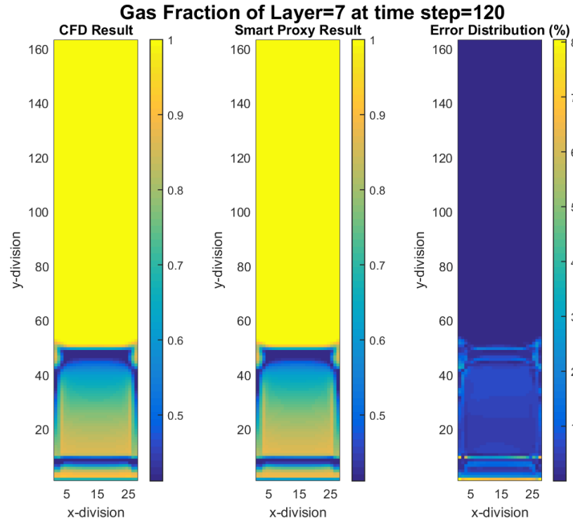
Figure 7-12 CFD and smart proxy results for gas volume fraction at K = 7 cross-sectional plane and time step = 120
