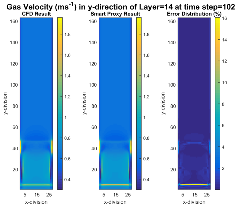
Figure 8-5 CFD and smart proxy results for y-component of gas velocity at K = 14 cross-sectional plane
