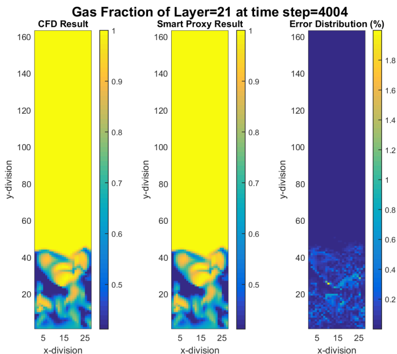
Figure 4-15 CFD and smart proxy results for gas volume fraction at K = 21 cross-sectional plane
