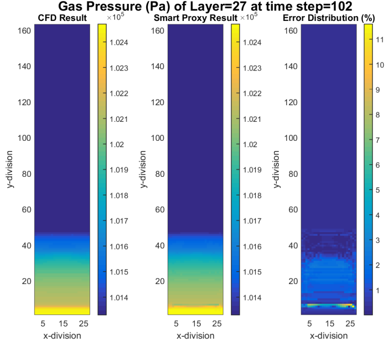
Figure 4-11 CFD and smart proxy results for gas pressure at K = 27 cross-sectional plane
