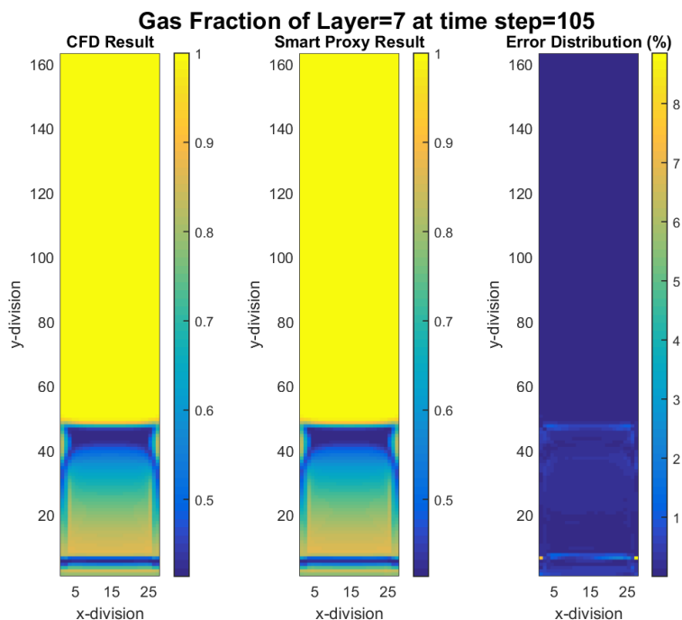
Figure 7-3 CFD and smart proxy results for gas volume fraction at K = 7 cross-sectional plane and time step = 105
