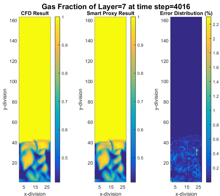
Figure 9-5 CFD and smart proxy results for gas volume fraction at K = 7 cross-sectional plane and time step = 4016
