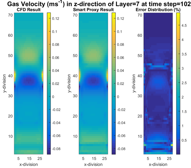
Figure 4-33 CFD and smart proxy results for z-component of gas velocity at K = 7 cross-sectional plane, based on explicitly constructed ANN
