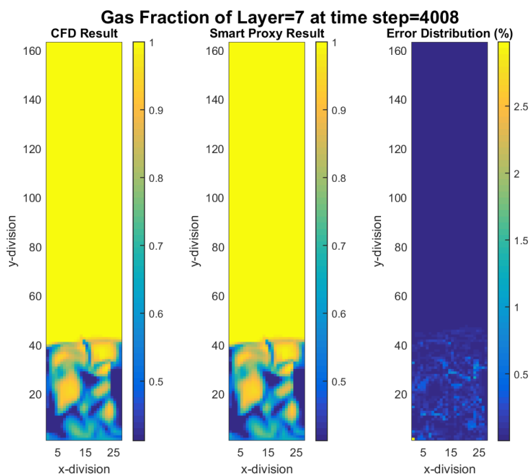
Figure 9-2 CFD and smart proxy results for gas volume fraction at K = 7 cross-sectional plane and time step = 4008
