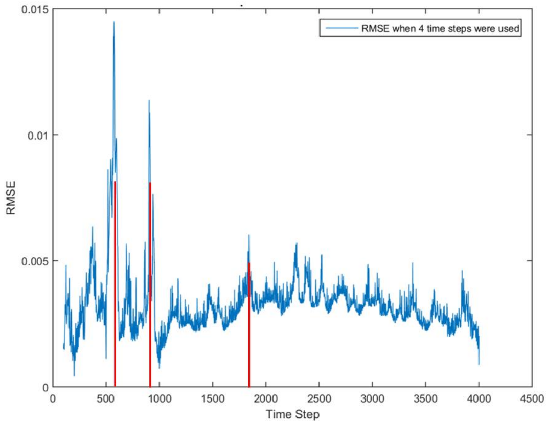
Figure 4-44 RMSE distribution in time, with three of the high RMSE values identified
