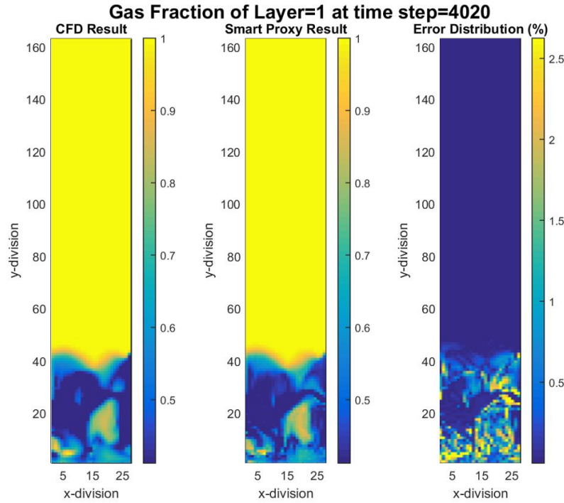
Figure 4-45 CFD and cascading smart proxy results for gas volume fraction at K = 1 cross-sectional plane
