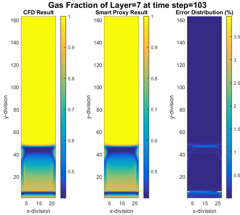
Figure 7-1 CFD and smart proxy results for gas volume fraction at K = 7 cross-sectional plane and time step = 103
