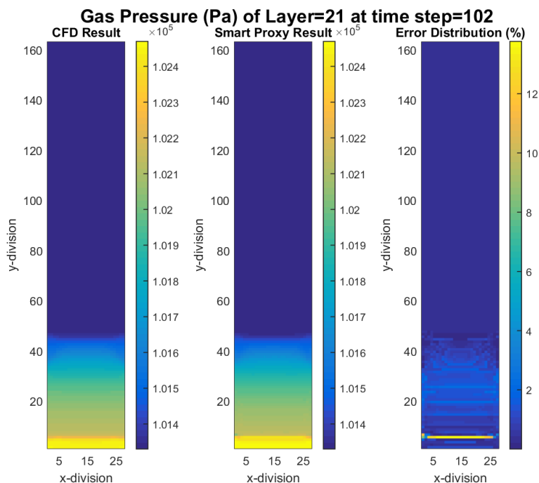
Figure 4-10 CFD and smart proxy results for gas pressure at K = 21 cross-sectional plane
