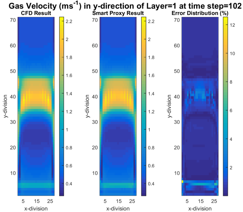
Figure 4-35 CFD and smart proxy results for y-component of gas velocity at K = 1 cross-sectional plane, based on implicitly constructed ANN
