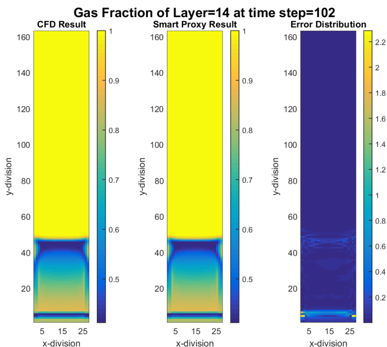
Figure 4-4 CFD and smart proxy results for gas volume fraction at K = 14 cross-sectional plane
