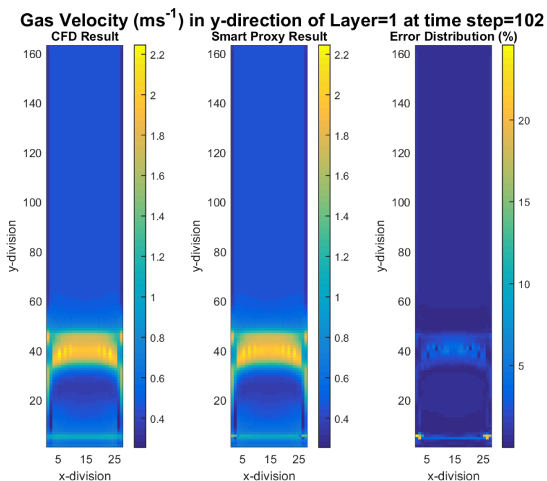
Figure 8-4 CFD and smart proxy results for y-component of gas velocity at K = 1 cross-sectional plane
