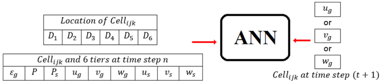
Figure 3-17 Training with one output (one component of gas velocity)
