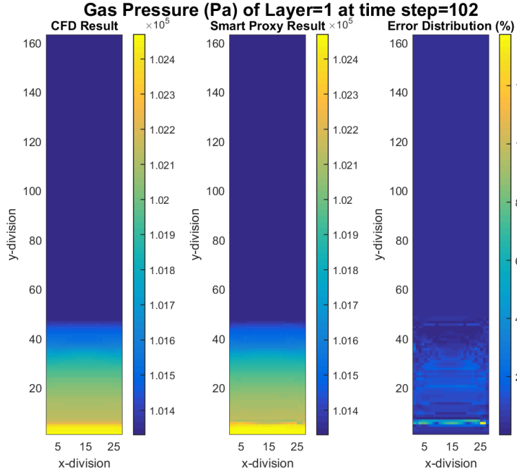
Figure 4-7 CFD and smart proxy results for gas pressure at K = 7 cross-sectional plane
