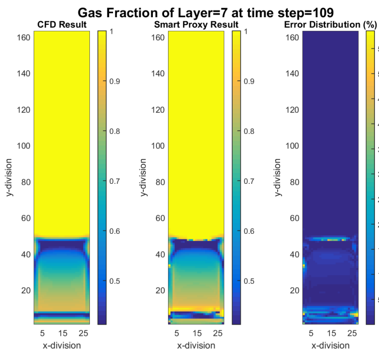
Figure 4-25 CFD and cascading smart proxy results for gas volume fraction at K = 7 cross-sectional plane and time step = 109
