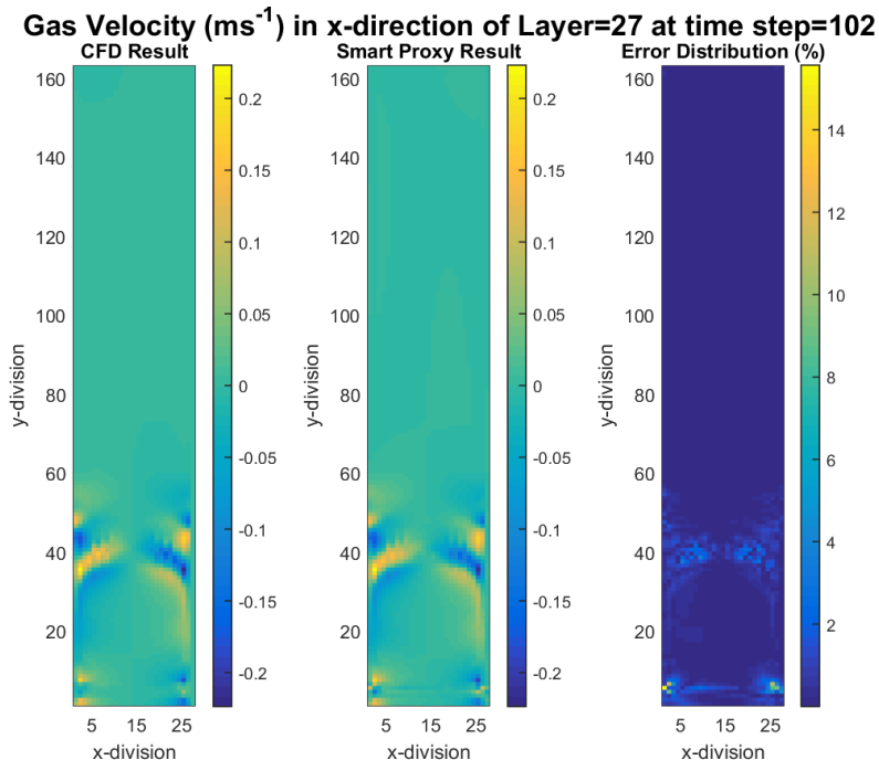
Figure 8-3 CFD and smart proxy results for x-component of gas velocity at K = 27 cross-sectional plane
