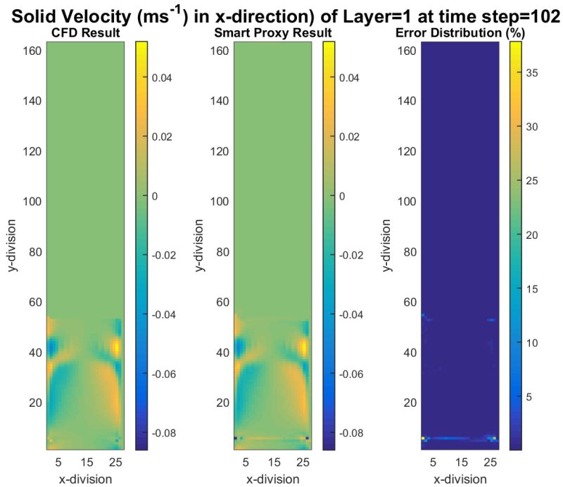
Figure 8-6 CFD and smart proxy results for x-component of solid velocity at K = 1 cross-sectional plane
