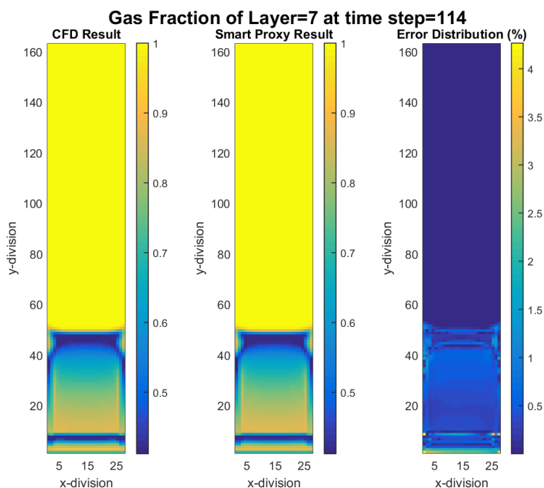
Figure 7-10 CFD and smart proxy results for gas volume fraction at K = 7 cross-sectional plane and time step = 114
