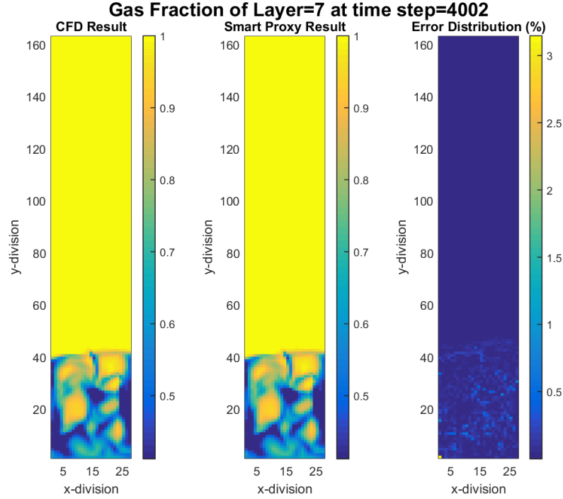
Figure 4-27 CFD and cascading smart proxy results for gas volume fraction at K = 7 cross-sectional plane and time step = 4002
