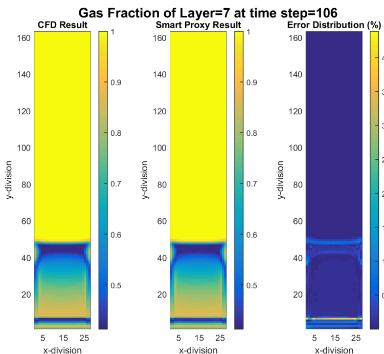
Figure 7-4 CFD and smart proxy results for gas volume fraction at K = 7 cross-sectional plane and time step = 106
