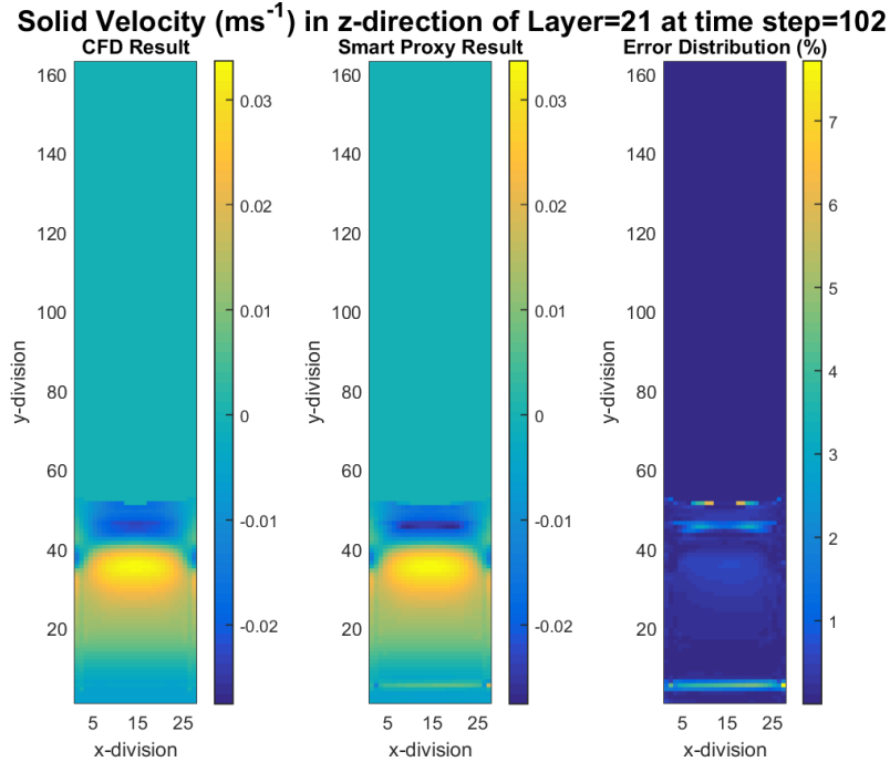
Figure 8-11 CFD and smart proxy results for z-component of solid velocity at K = 21 cross-sectional plane
