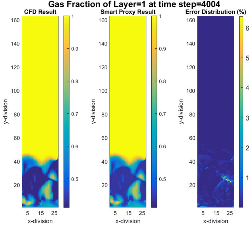
Figure 4-48 CFD and non-cascading smart proxy results for gas volume fraction at K = 1 cross-sectional plane with 30% of data used for training
