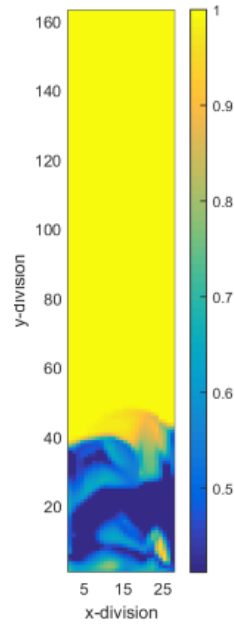
Figure 3-2 Snap shot of voidage contour predicted by MFiX
