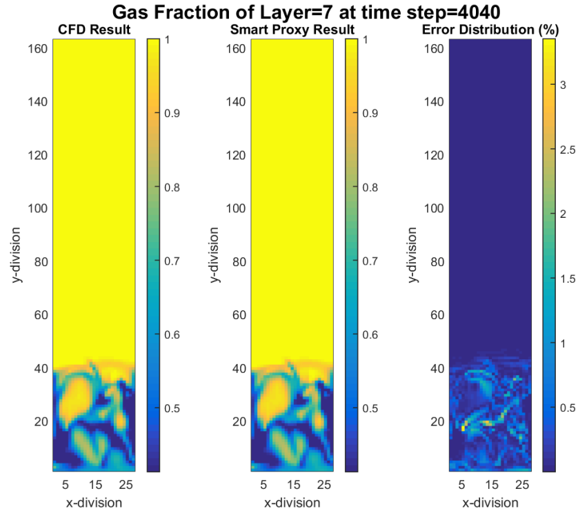
Figure 9-10 CFD and smart proxy results for gas volume fraction at K = 7 cross-sectional plane and time step = 4040
