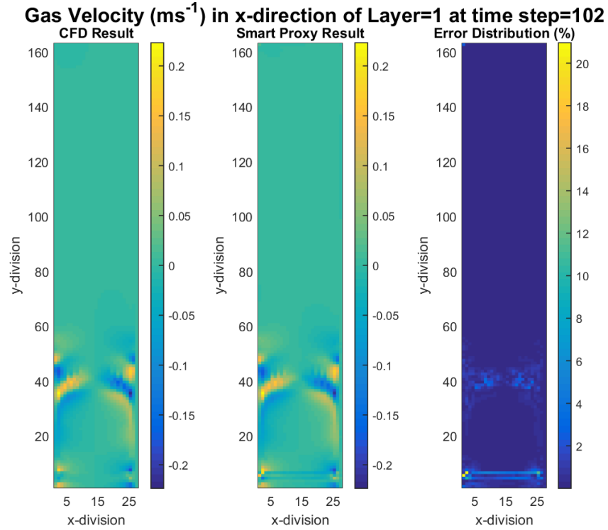
Figure 8-1 CFD and smart proxy results for x-component of gas velocity at K = 1 cross-sectional plane
