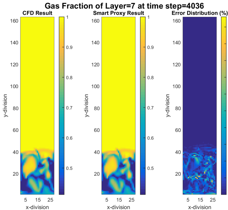
Figure 9-9 CFD and smart proxy results for gas volume fraction at K = 7 cross-sectional plane and time step = 4036
