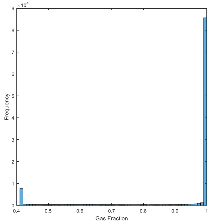
Figure 3-26 Distribution of gas volume fraction at time step 4000
