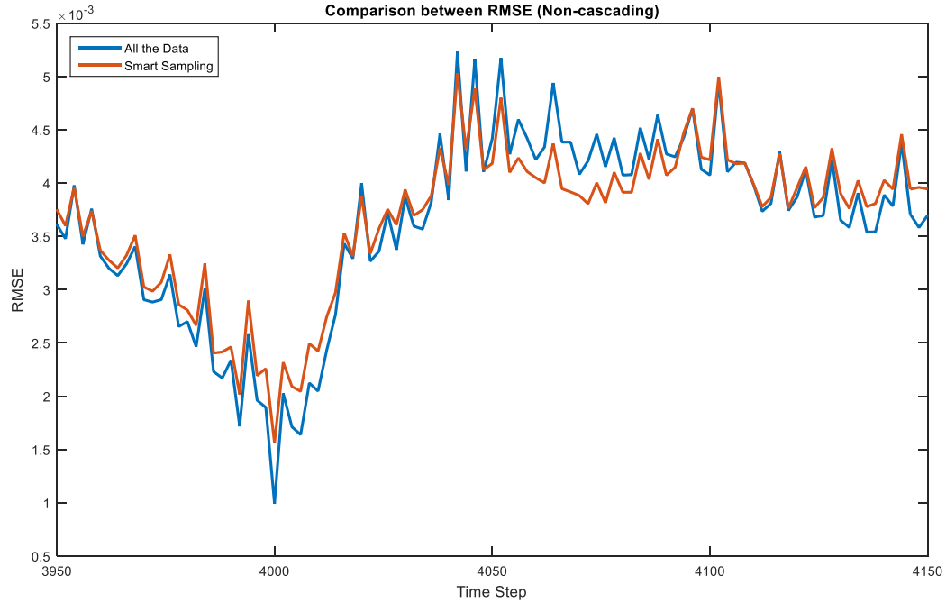
Figure 4-49 RMSE distribution in time with and without smart sampling
