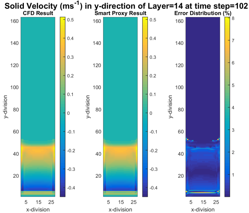
Figure 8-9 CFD and smart proxy results for x-component of solid velocity at K = 14 cross-sectional plane
