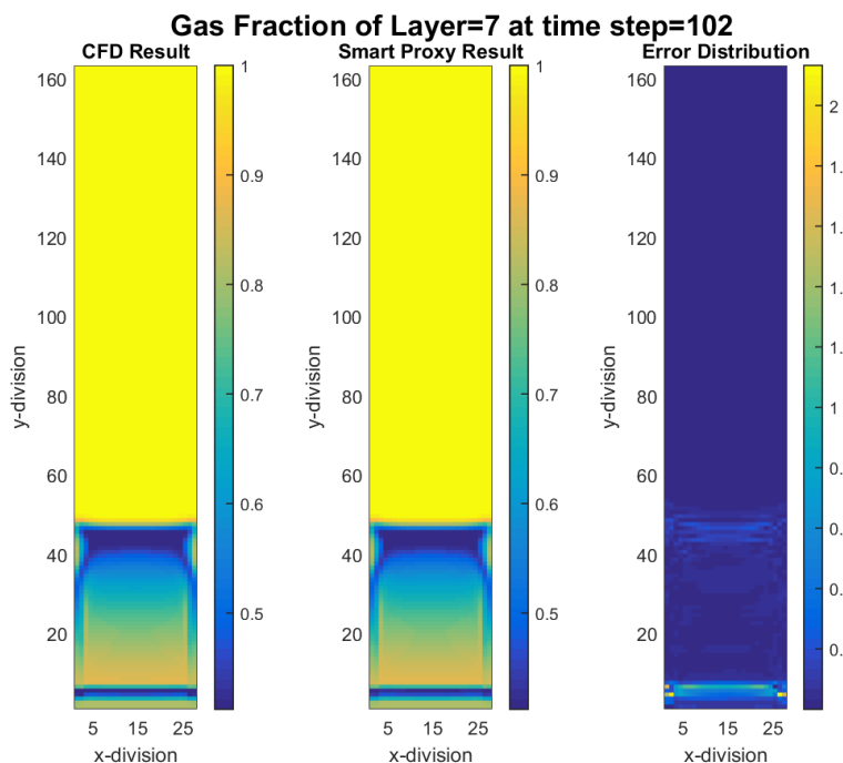
Figure 4-3 CFD and smart proxy results for gas volume fraction at K = 7 cross-sectional plane
