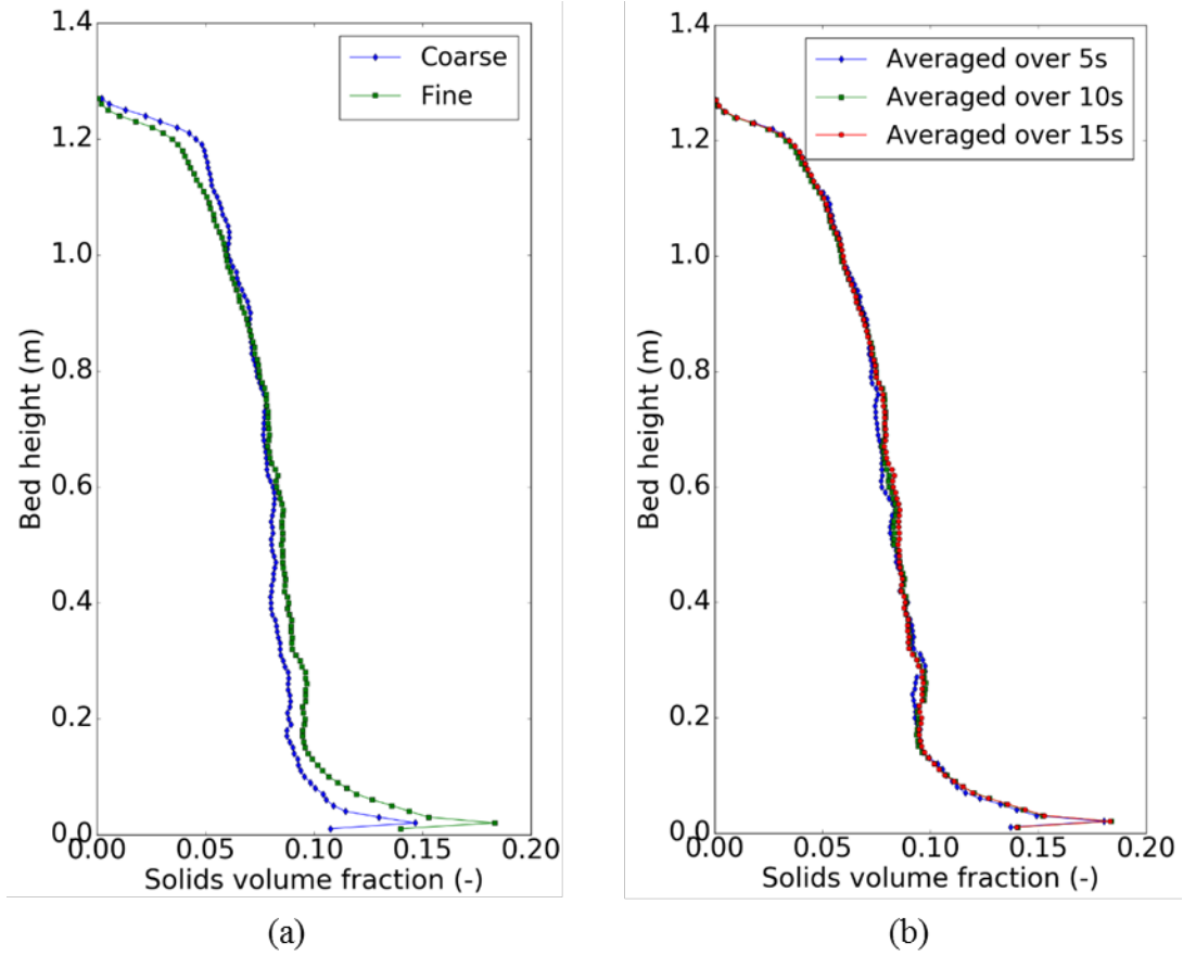
Figure 2: Average solids holdup along the riser (simulated data were taken from the center line across the riser) (a) Systems with different grid resolutions; (b) systems with different statistical time.
