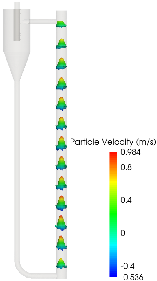
Figure 9: The typical core-annulus structure (the average vertical particle velocity) along the riser with the HKL drag correlation.
