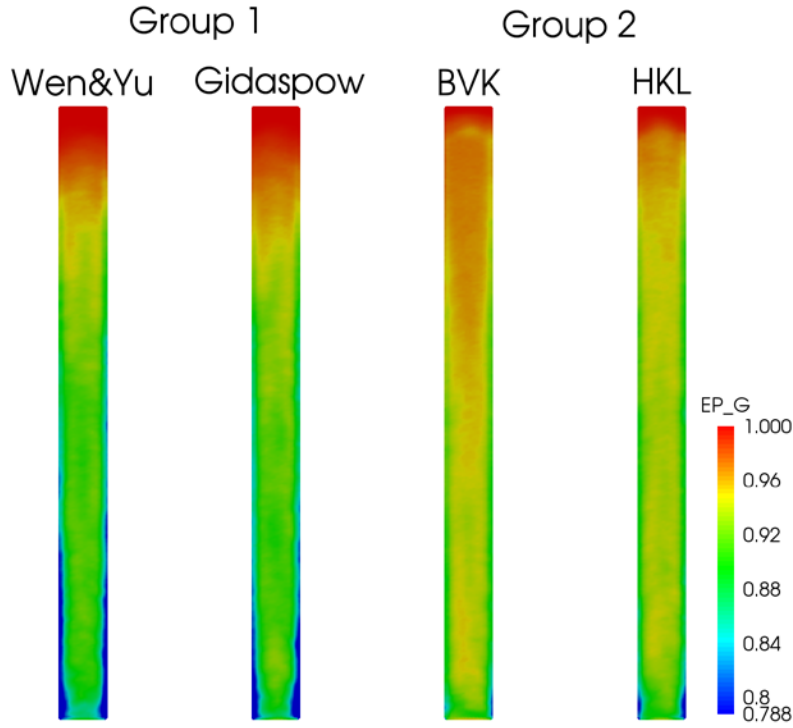
Figure 8: Time-averaged gas void fraction along longitudinal cross section of riser under different drag correlations as labeled (the height of riser is scaled down for better representation)
