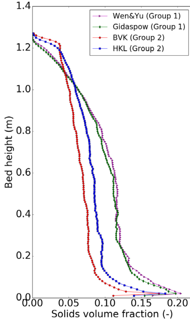
Figure 7: Predicted solids volume fraction in the riser of the CFB system.
