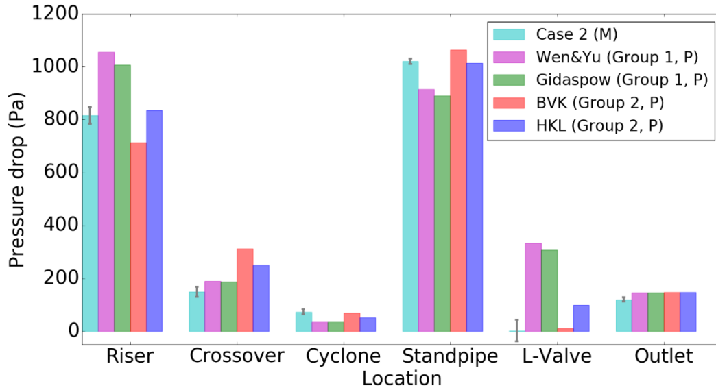
Figure 4: Comparison of measured and predicted time-averaged pressure drop across key system components, the error bars represent the standard deviation between different measurements (M: Measured, P: Predicted).
