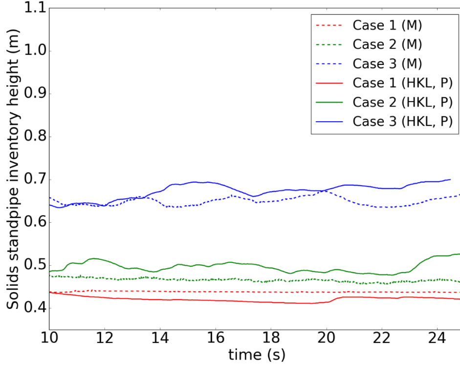
Figure 19: Direct comparison of the solids standpipe inventory height under different operation conditions (M: Measured, P: Predicted).
