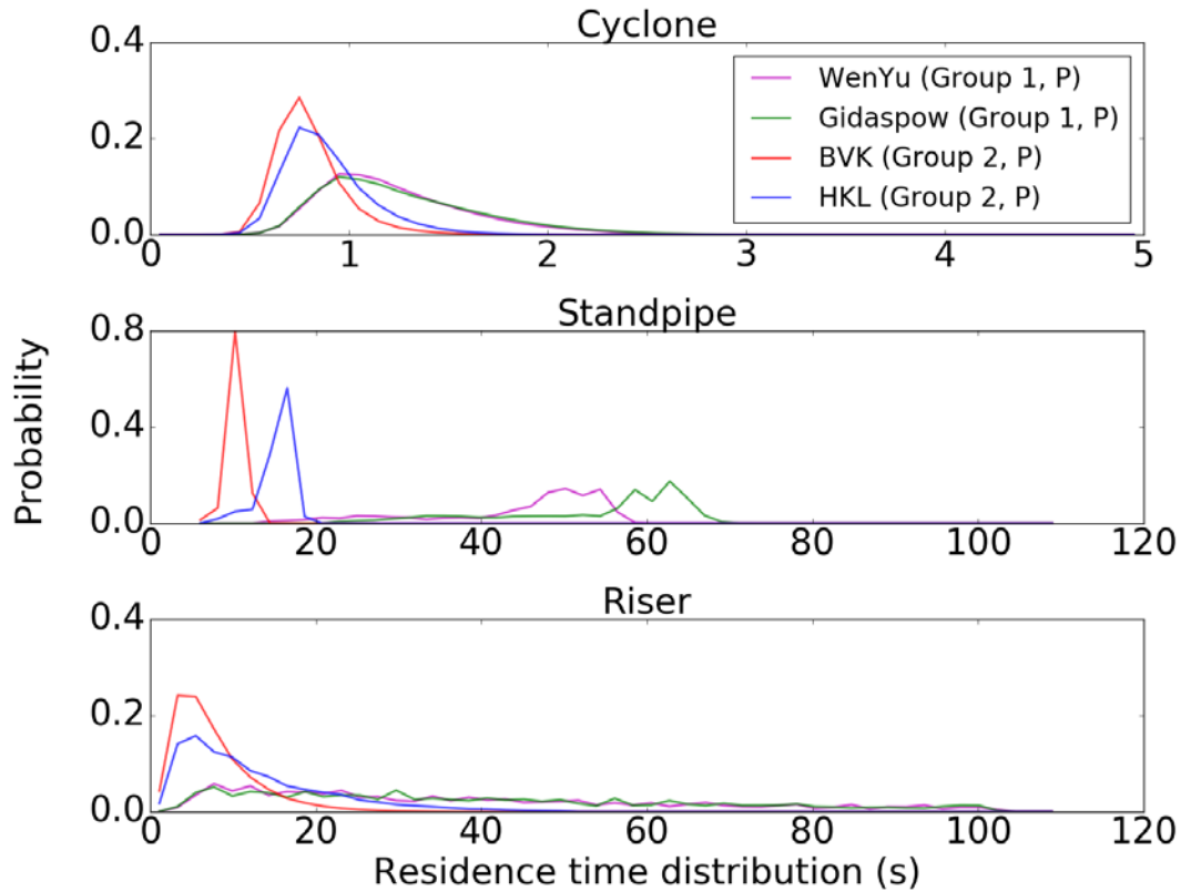
Figure 12: Residence time distribution in different components of the CFB under different drag correlations
