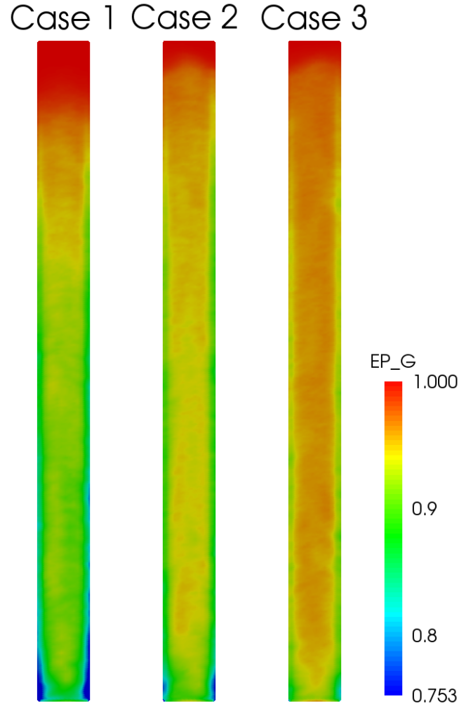
Figure 21: Time-averaged gas void fraction of the center surface inside the riser under different drag correlations.
