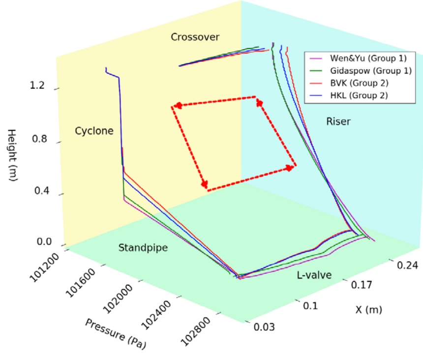
Figure 3: Predicted, time-averaged pressure profile around the CFB system, the red arrows indicate the flow direction inside the CFB.
