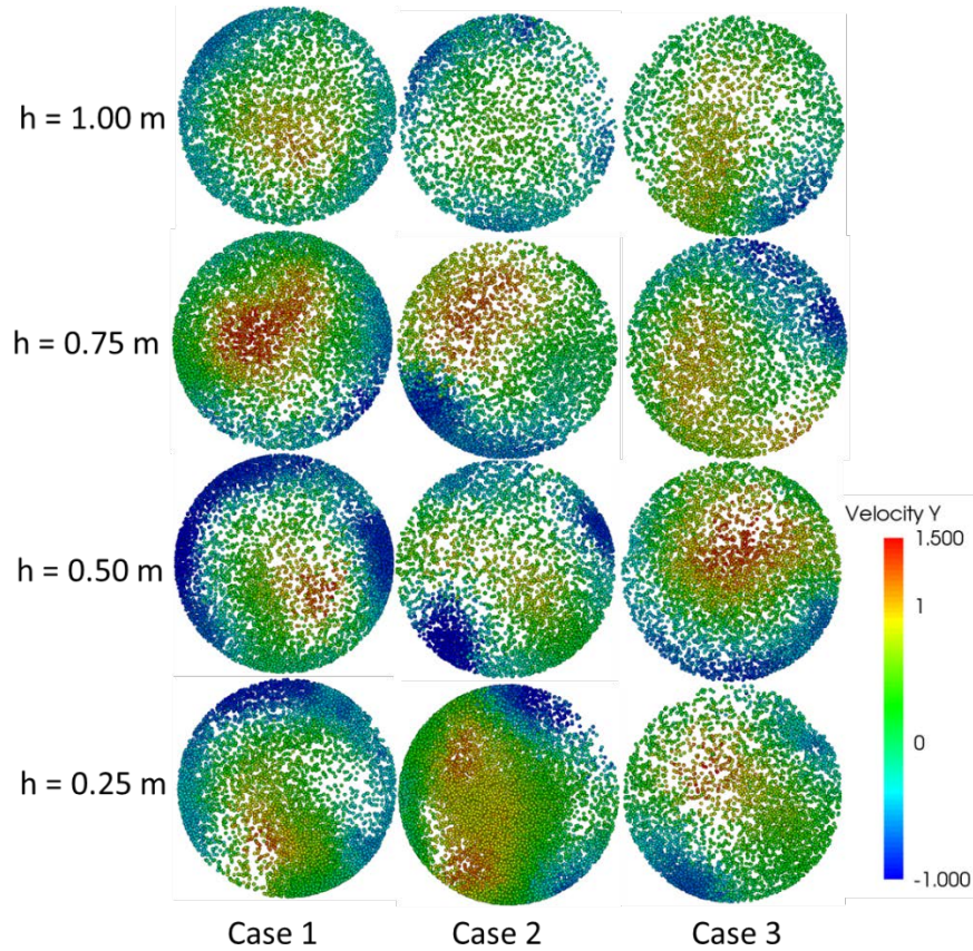
Figure 22: Influence of different operating conditions on instantaneous solid velocity. Shown are radial cross sections of the CFB riser at indicated heights (h) from the inlet
