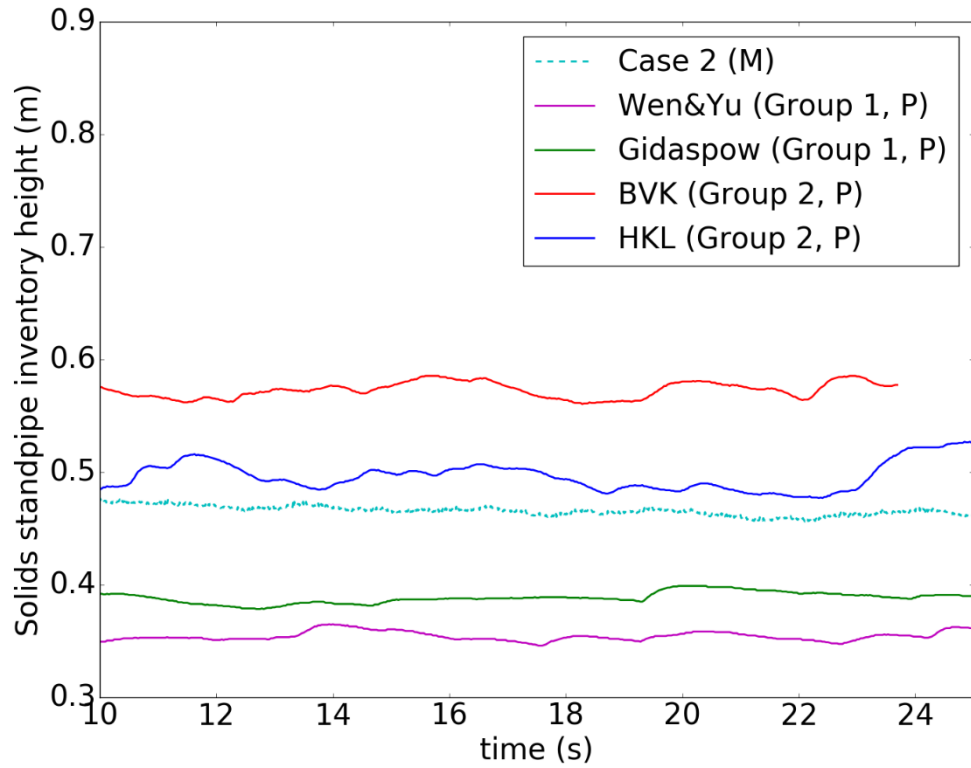
Figure 6: Instantaneous solids standpipe inventory height under different drag correlations (M: Measured, P: Predicted).
