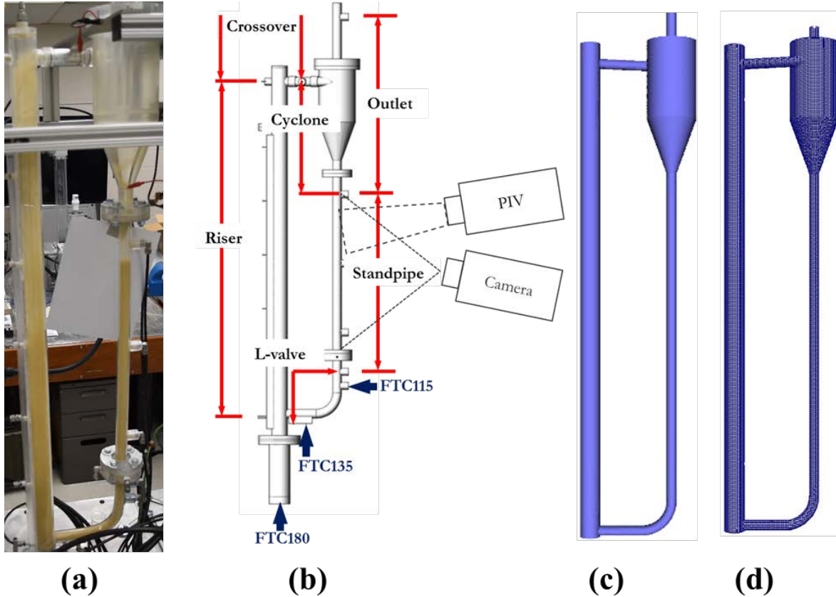
Figure 1: (a) Snapshot of experimental setup; (b) Schematic representation of the circulating fluidized bed; (c) Geometric configuration and (d) grid representation deployed in the simulations.
