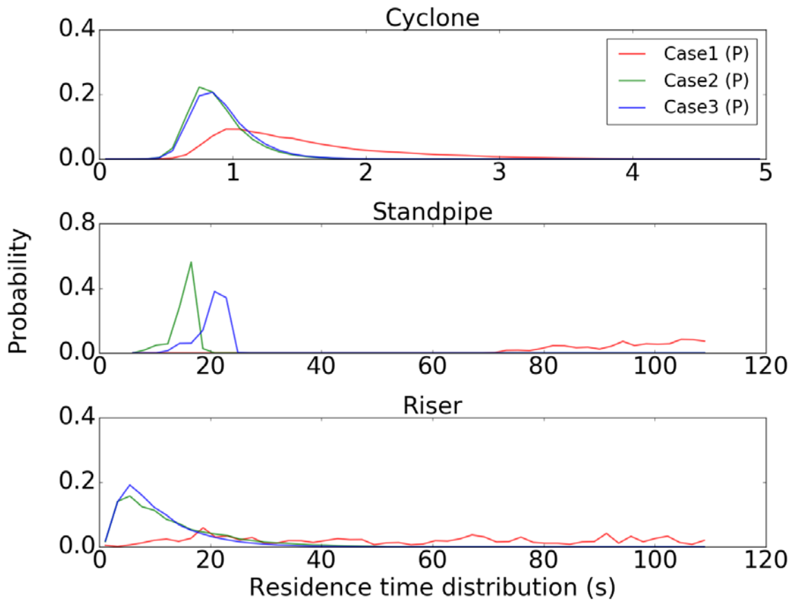
Figure 24: Residence time distribution through different components of the CFB under 3 different operating conditions.
