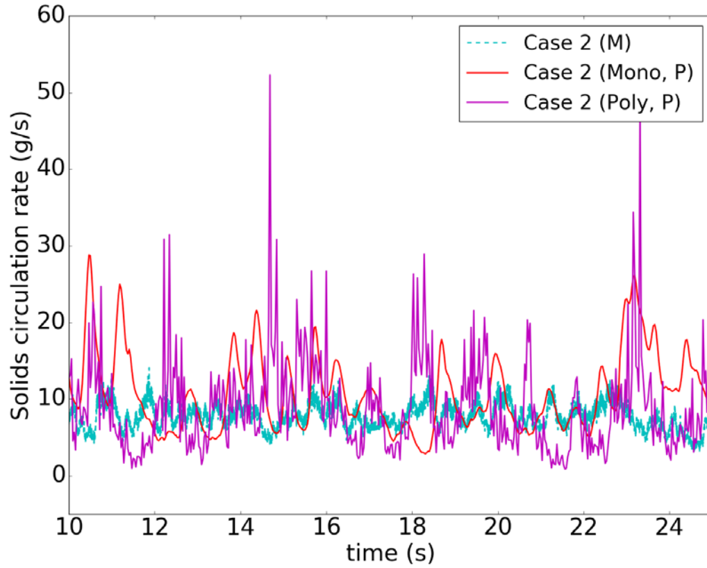
Figure 15: Solids circulation rate with and without particle size distribution (M: Measured, P: Predicted, Mono: Mono-disperse, Poly: Poly-disperse).
