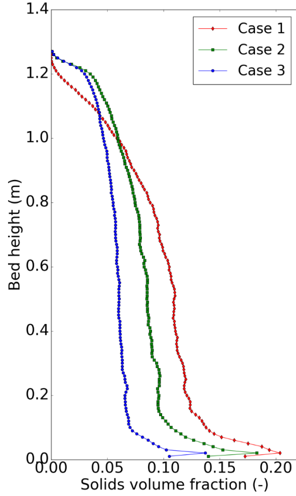
Figure 20: Average solid holdup along the riser under different operation conditions.
