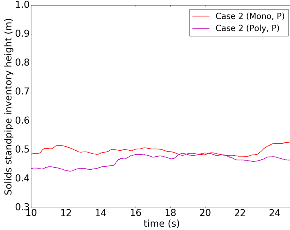
Figure 16: Solids standpipe inventory height (P: Predicted, Mono: Mono-disperse, Poly: Poly-disperse).
