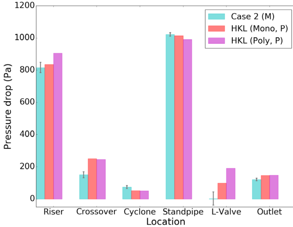
Figure 14: Comparison of measured and predicted time-averaged pressure drop across key system components (M: Measured, P: Predicted, Mono: Mono-disperse, Poly: Poly-disperse).
