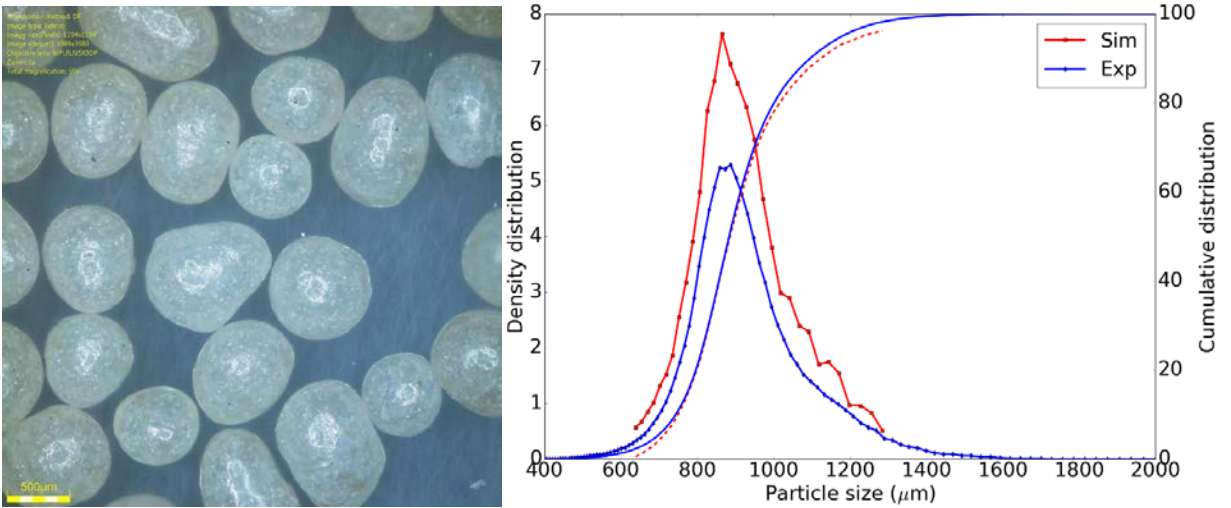
Figure 13: Particle size distribution. Sim = used in simulation; Exp = measured values
