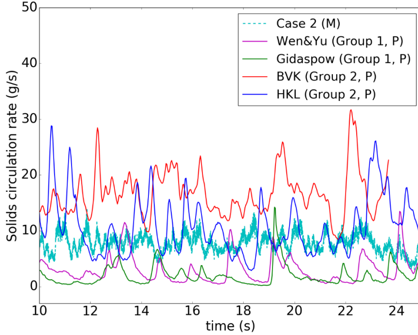
Figure 5: Solids circulation rate predicted by different drag correlations (M: Measured, P: Predicted).
