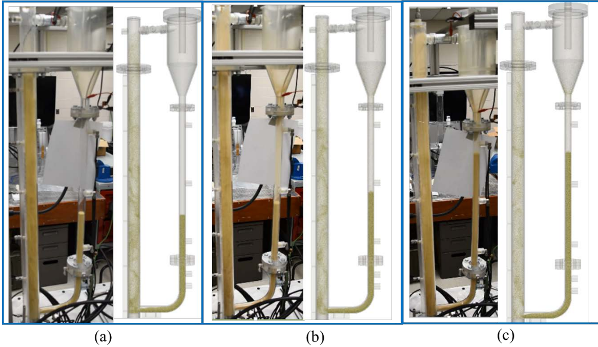
Figure 17: Direct comparison between experiments and simulations under different operating conditions (a): Case 1, (b): Case 2, (c): Case 3.
