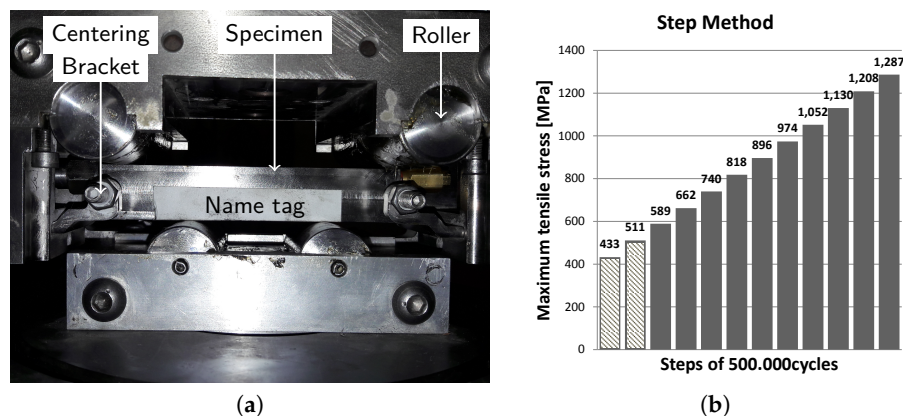
Figure 3. All specimens were subjected to four-point bending fatigue tests according to the step method. (a) specimen installed in the four-point bending test setup and (b) the maximum tensile stress levels in each load step.
