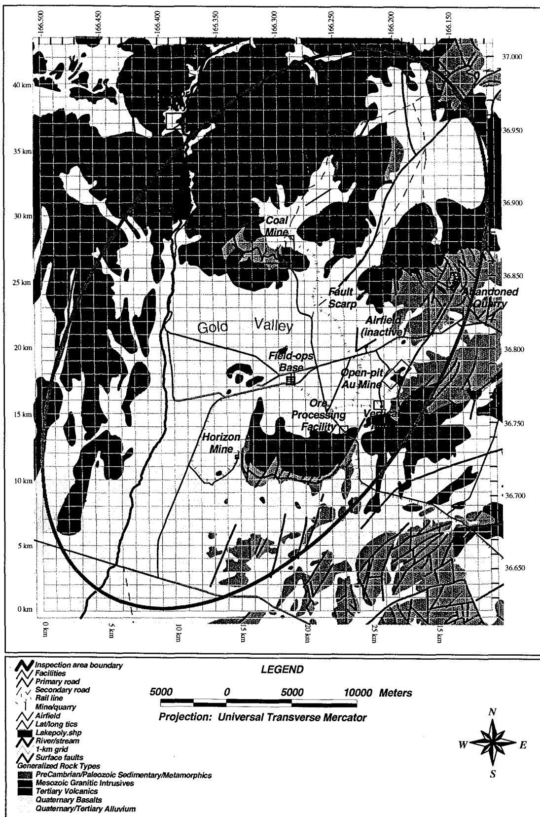
Generalized Geologic Map of the Gold Valley Area.
