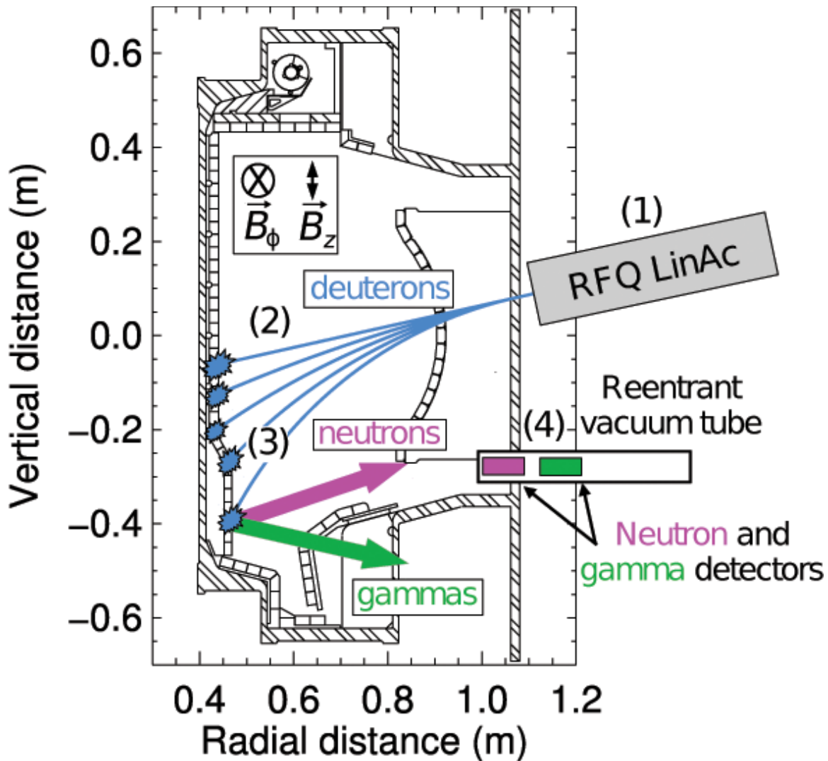
Figure II-9. Schematic representation of the AIMS diagnostic on Alcator C-Mod
