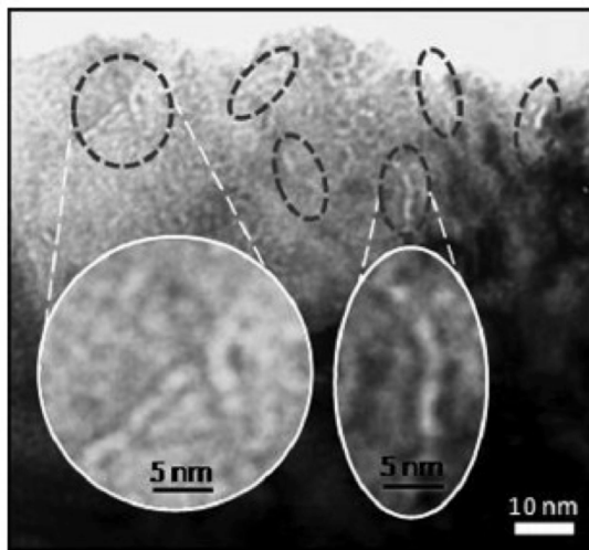
Figure II-10: Transmission electron microscope image showing the formation of helium induced nanobubbles in the surface of tungsten exposed to deuterium-helium mixture plasma 17
