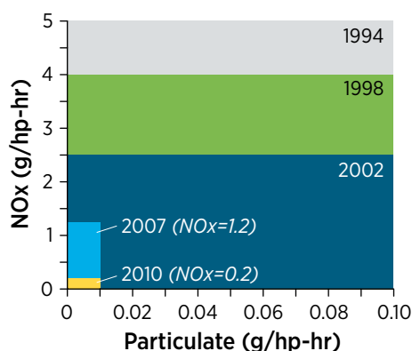
Figure 1: Emission Standards for Heavy-Duty Highway Engines. U.S. emissions limits for nitrogen oxides (NOx) and particulate matter (PM) have been reduced significantly over the last 20 years. Biodiesel's benefits are maximized in engines older than MY 2010.
