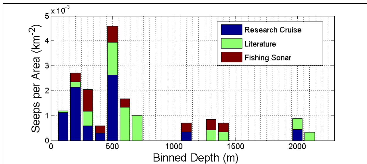
Figure 5. Histogram showing all methane emission sites on the Washington and Oregon segments of the Cascadia margin, with 300 meter clustering applied to the individual bubble streams and normalized by the area contained within each 100 meter depth bin. Color bar legend shows methane plume site data sources.
