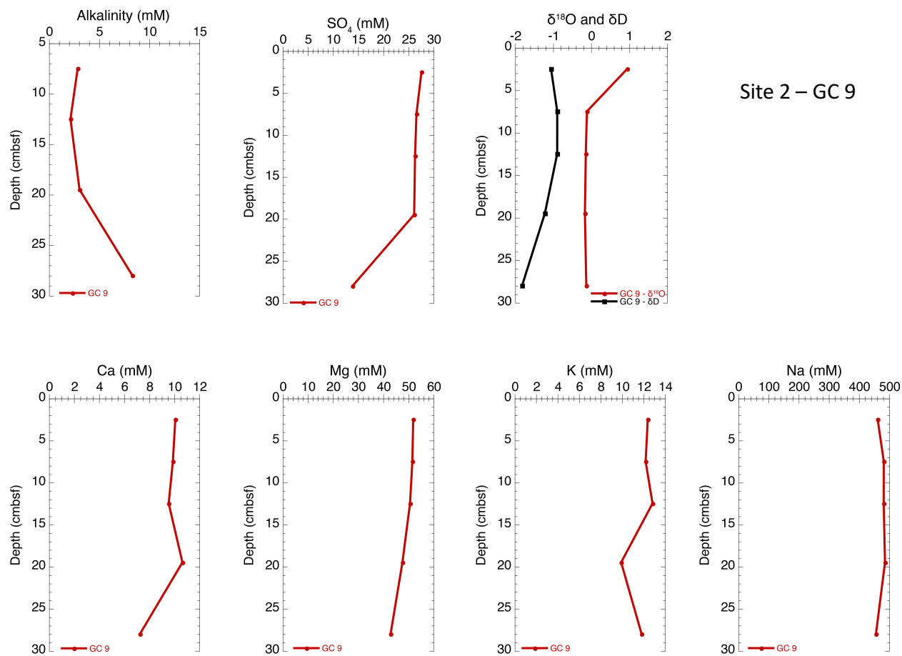
Figure 8. Pore water alkalinity, \text{SO}_4 , \delta^{18}\text{O} , \delta\text{D} , Ca, Mg, K, and Na from Gravity Core 9 at Site 2. For location of gravity cores at each site, refer to Appendix I.
