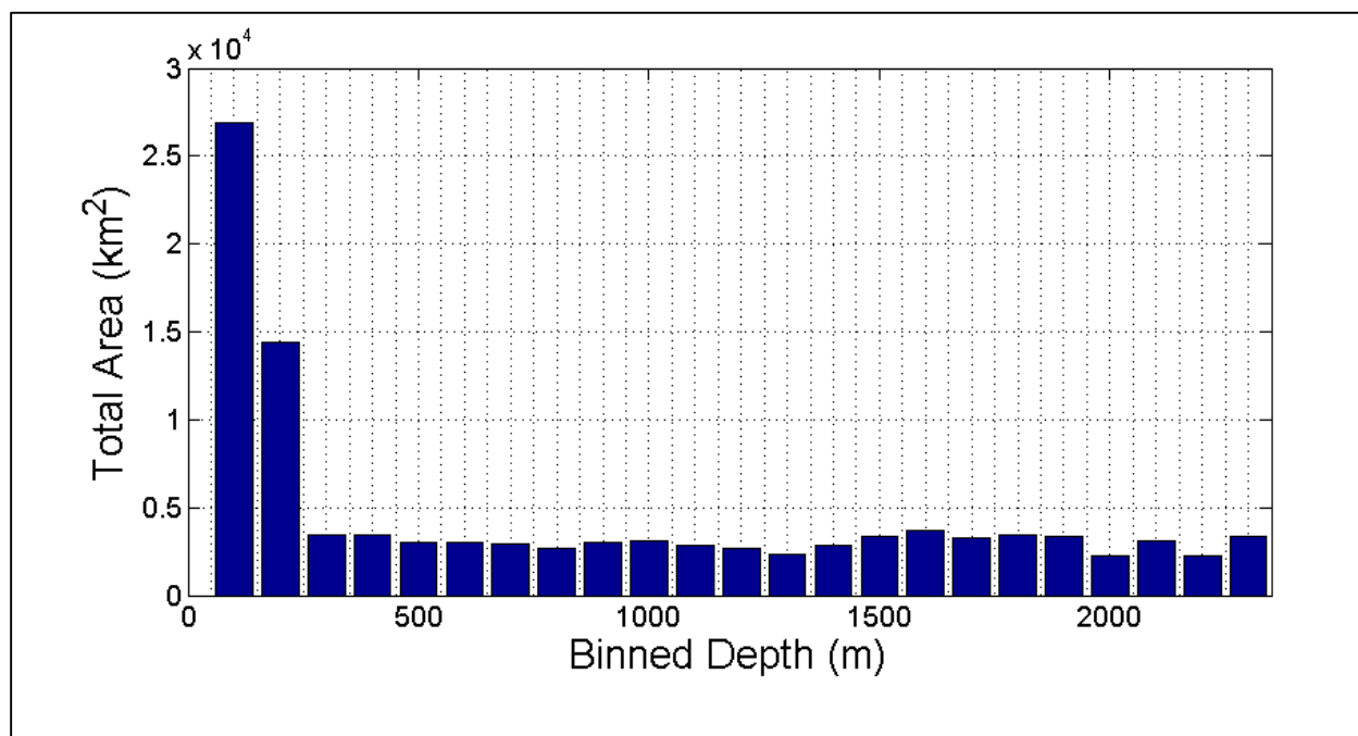
Supplemental Figure S2. Histogram showing the area of the individual depth bins for the Cascadia margin after partitioning into 100 meter depth intervals, beginning at 50 to 149 meters water depth. Note that the partition containing the shallow continental shelf between 50 and 149 meters has the largest area. Cascadia shelf break varies along-strike, but lies at approximately 180 to 200 meters water depth.
