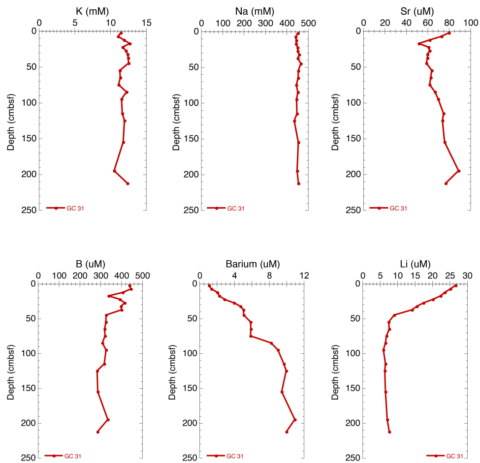
Figure 27. Pore water K, Na, Sr, B, Ba, and Li from Gravity Core 31 at Site 6. For location of gravity cores at each site, refer to Appendix I.
