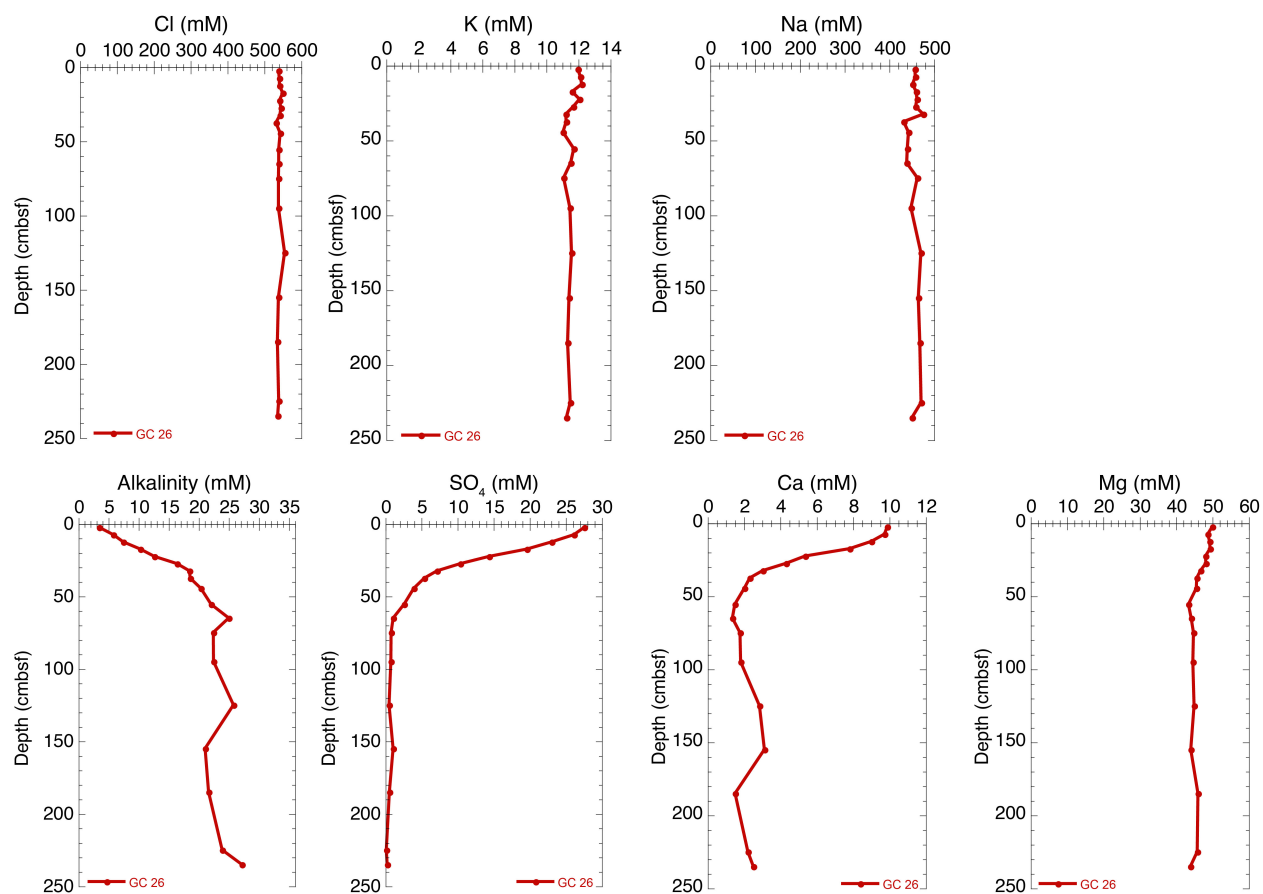
Figure 23. Pore water Cl, K, Na, alkalinity, sulfate, Ca, and Mg from Gravity Core 26 at Site 6. For location of gravity cores at each site, refer to Appendix I.
