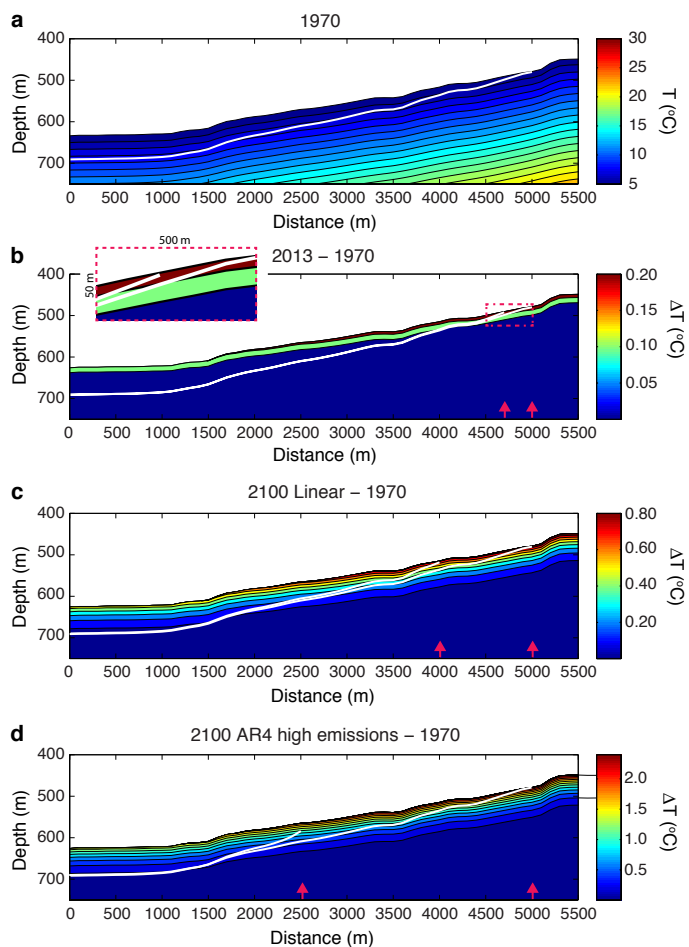
Supplementary Figure 2. Sediment thermal simulations for bathymetric transect P3. a. Initial subseafloor temperature distribution in 1970 based on the regression (see Methods) and a basal heat flow of 60 mW/m [Booth-Rea et al., 2008]. The white line is the base of the gas hydrate stability zone (BGHSZ) in the sediment column for Structure I gas hydrate and hydrostatic pressure following the methods outlined in Tischenko (2005). b. The simulated change in sediment temperature between 1970 and 2013 and corresponding shift in the BGHSZ. The BGHSZ shoals over a broad area in response to warming, accompanied by a retreat of its landward edge (indicated by red arrows). c. Simulated change in sediment temperature between 1970 and 2100 based on the linear extrapolation of seafloor temperature. The upper white line is the BGHSZ in 2100. d. Simulated change in sediment temperature between 1970 and 2100 based on the high-emissions AR4 extrapolation. The upper white line is the BGHSZ in 2100 and the lower white line is the BGHSZ in 1970.
