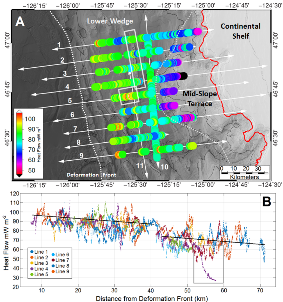
Figure 3: A) BSR heat flow measurements (circles) along the 11 MCS lines (white solid lines). Deformation front, lower and mid-slope defined by dashed grey lines. The 500 meter upper limit of hydrate stability is indicated by a solid red line. B) All heat flow profiles are indexed as distance from the deformation front. General heat flow trends are traced by black lines.
