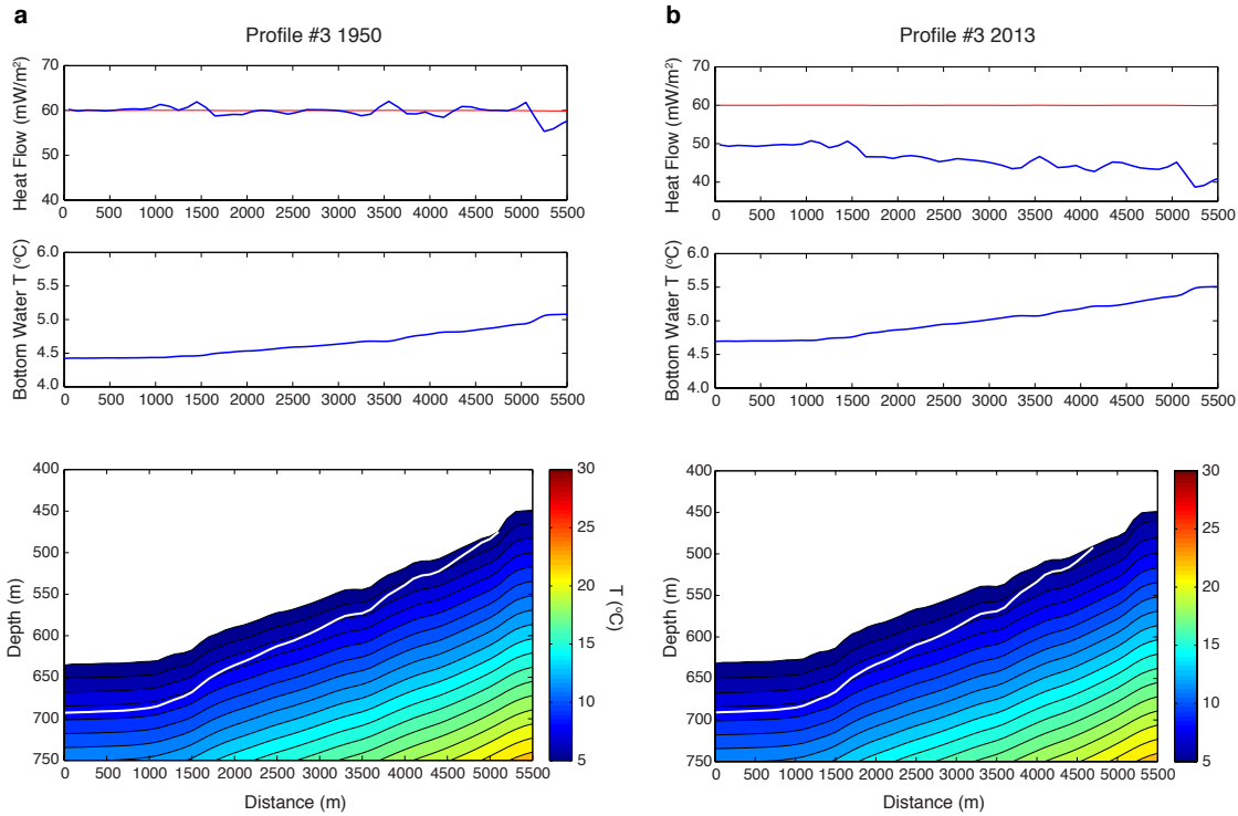
Supplementary Figure 4. Heat flow at the seafloor, estimated seafloor temperature, and subseafloor temperature distribution along transect P3 in a. 1950 and b. 2013. The white line represents the BGHSZ.
