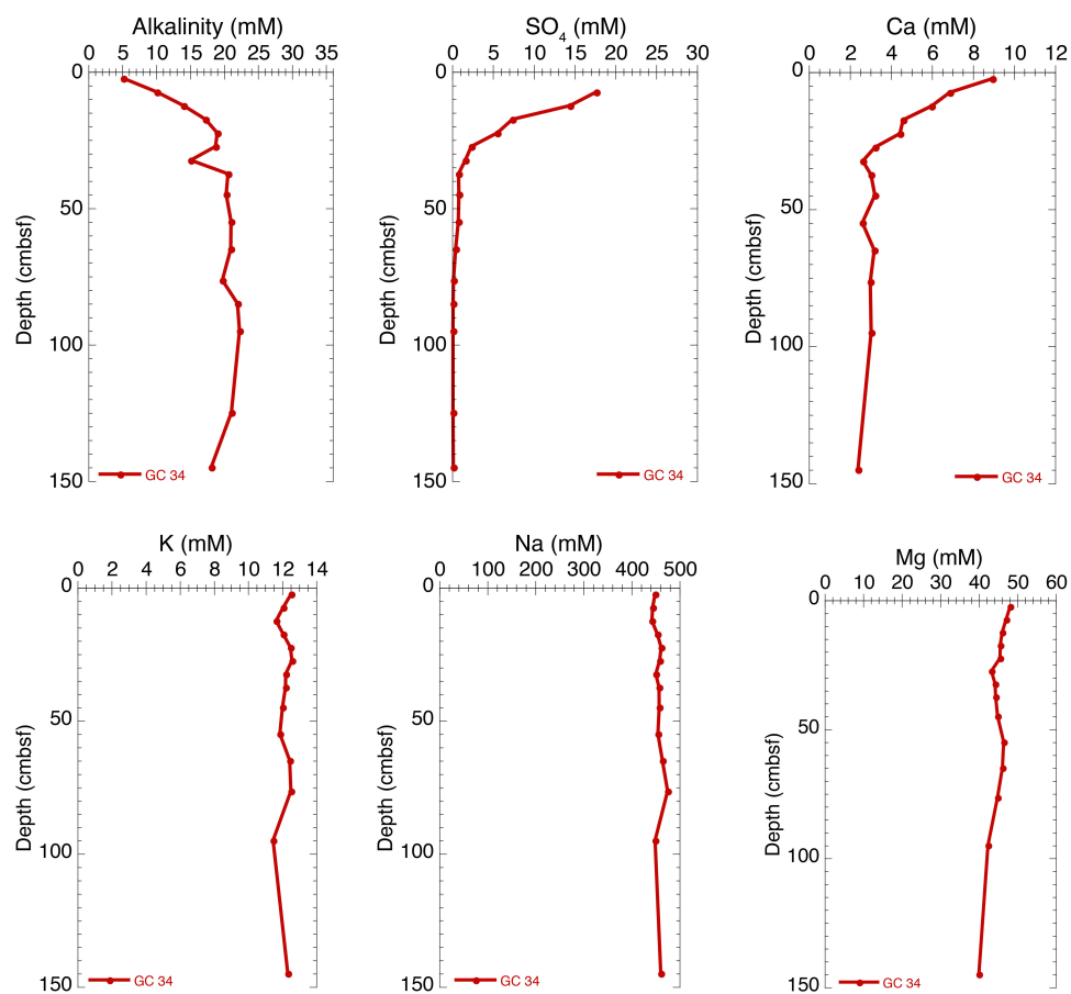
Figure 30. Pore water alkalinity, sulfate, Ca, Mg, K, and Na from Gravity Core 34 at Site 8. For location of gravity cores at each site, refer to Appendix I.
