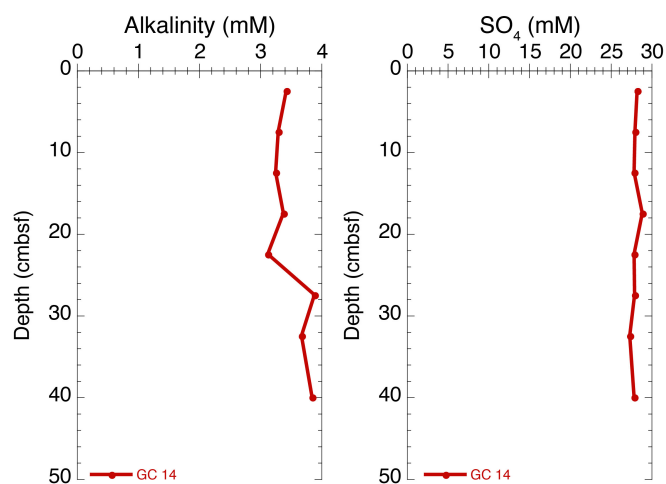
Figure 13. Pore water alkalinity and \text{SO}_4 from Gravity Core 14 at Site 4. For location of gravity cores at each site, refer to Appendix I.
