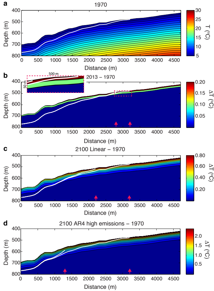
Supplementary Figure 1. Sediment thermal simulations for bathymetric transect P2. a. Initial subseafloor temperature distribution in 1970 based on the regression (see Methods) and a basal heat flow of 60 mW/m [Booth-Rea et al., 2008]. The white line is the base of the gas hydrate stability zone (BGHSZ) in the sediment column for Structure I gas hydrate and hydrostatic pressure following the methods outlined in Tischenko (2005). b. The simulated change in sediment temperature between 1970 and 2013 and corresponding shift in the BGHSZ. The BGHSZ shoals over a broad area in response to warming, accompanied by a retreat of its landward edge (indicated by red arrows). c. Simulated change in sediment temperature between 1970 and 2100 based on the linear extrapolation of seafloor temperature. The upper white line is the BGHSZ in 2100. d. Simulated change in sediment temperature between 1970 and 2100 based on the high-emissions AR4 extrapolation. The upper white line is the BGHSZ in 2100 and the lower white line is the BGHSZ in 1970.
