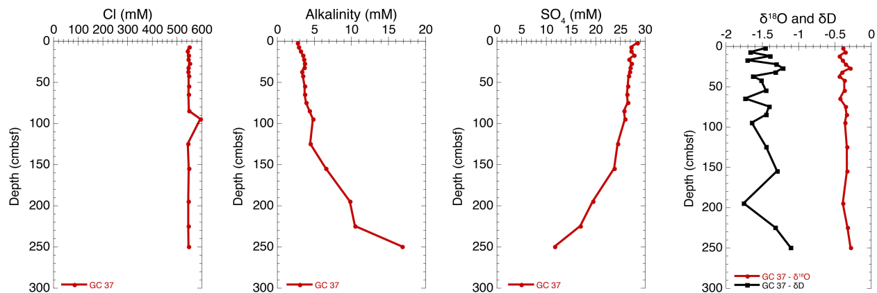
Figure 32. Pore water Cl, \delta^{18}\text{O} , \delta\text{D} , alkalinity, and sulfate from Gravity Core 37 at Site 9. For location of gravity cores at each site, refer to Appendix I.
