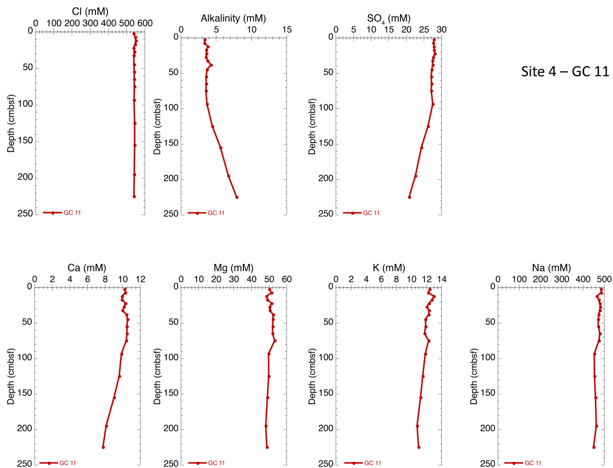
Figure 10. Pore water Cl, alkalinity, SO 4 , Ca, Mg, K, and Na from Gravity Core 11 at Site 4. For location of gravity cores at each site, refer to Appendix I.
