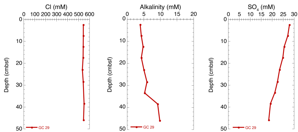
Figure 25. Pore water Cl, alkalinity, and sulfate from Gravity Core 29 at Site 6. For location of gravity cores at each site, refer to Appendix I.
