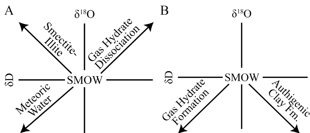
Figure 1. Schematic diagrams of expected pore water trends in \delta^{18}\text{O} and \delta\text{D} when chloride concentrations (A) increase and (B) decrease with respect to seawater.
