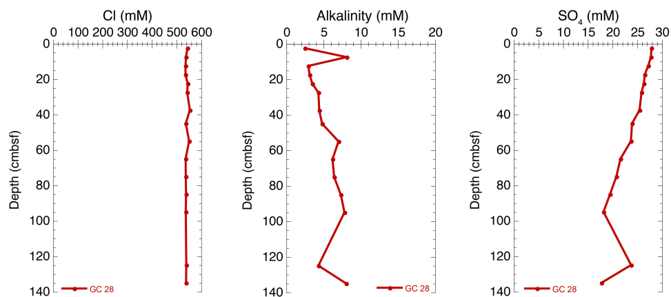
Figure 24. Pore water Cl, alkalinity, and sulfate from Gravity Core 28 at Site 6. For location of gravity cores at each site, refer to Appendix I.
