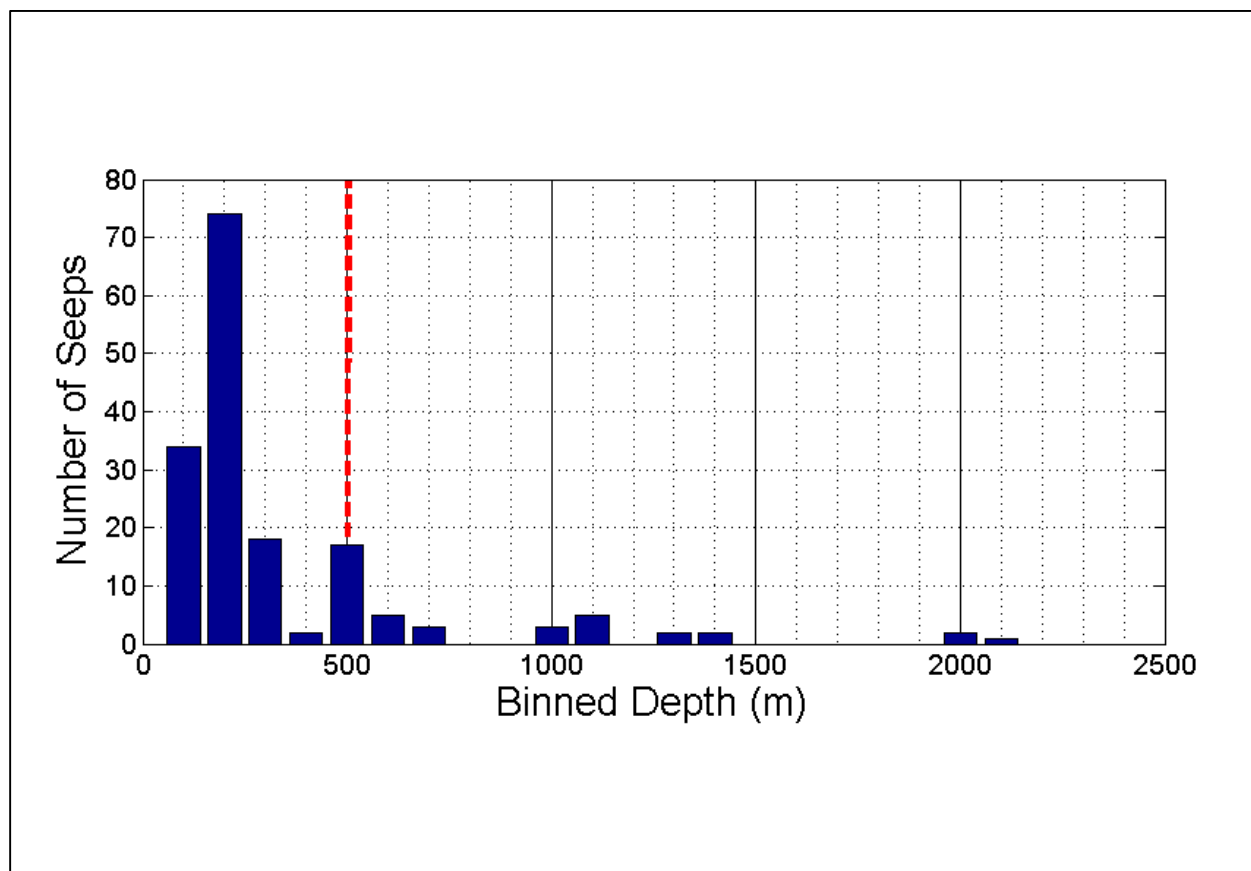
Figure 2. Histogram of all individual methane bubble streams observed in this study plotted as a function of site depth (meters), with no clustering or normalization by area applied. Depth bins are 100 meters wide, beginning at 50 meters water depth. Note the strong peak in the 150 to 249 meter depth bin where listric faults are present on the continental shelf edge between 150 and 249 meters water depth.
