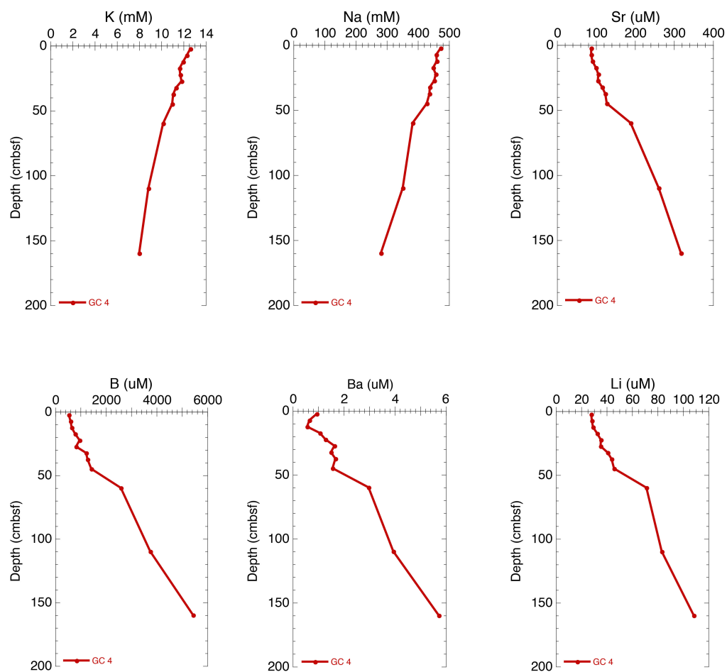
Figure 5. Pore water K, Na, Sr, B, Ba, and Li from Gravity Core 4 at Site 2. For location of gravity cores at each site, refer to Appendix I.
