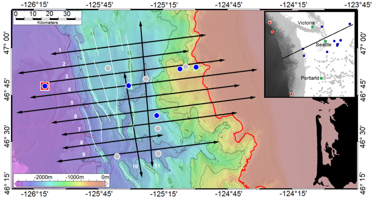
Figure 1: Location of COAST 2012 Multi-Channel Seismic profiles (black lines) with their corresponding line numbers (white text). White lines trace prominent anticlinal ridges visible in the MCS. LDEO OBSs (Blue circles) deployed during the 2012-2013 year within the Langseth survey area were equipped with thermistors. CTD cast location (red square) was used for BSR seafloor temperature calculations and sediment cores (grey circles) were used for BSR heat flow sedimentation correction. Inset displays IODP/ODP borehole (Red dots) and continental heat flow measurements (grey dots) including those used in the current study (blue dots). Green dots mark major metropolitan cities.
