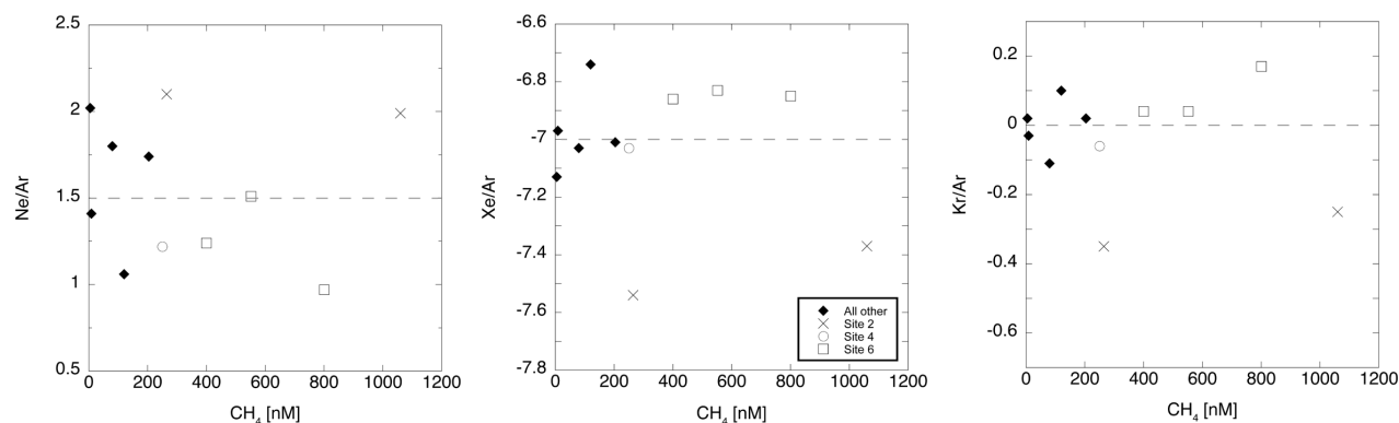
Figure 34. Plotted noble gas ratios represent the percent in situ saturation of Ne/Ar, Kr/Ar, and Xe/Ar. Site 2 samples are plotted as an “X”, open circles are Site 4, open squares are site 6, and filled diamonds are all other sampled sites.
