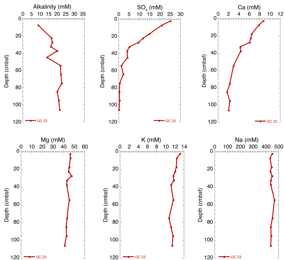
Figure 21. Pore water alkalinity, sulfate, Ca, Mg, K, and Na from Gravity Core 23 at Site 5. For location of gravity cores at each site, refer to Appendix I.
