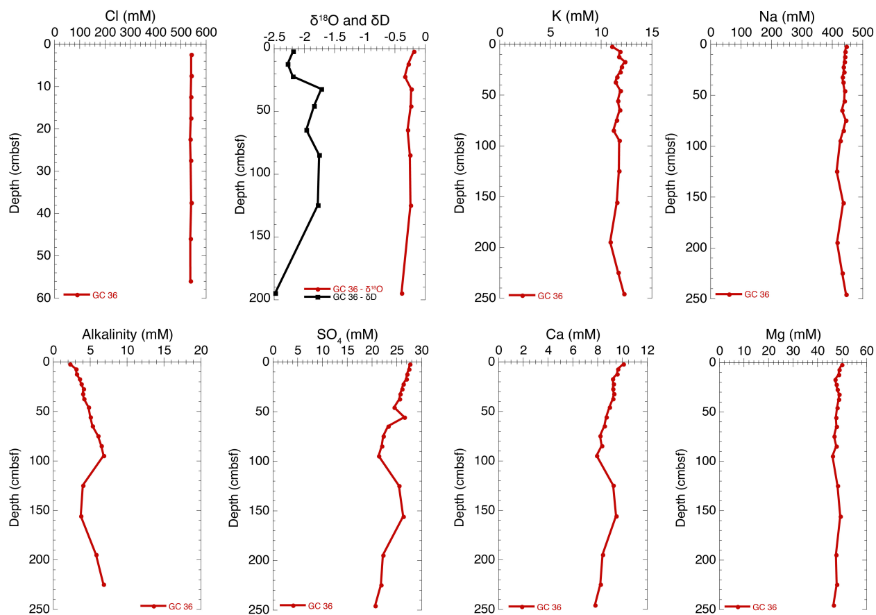
Figure 31. Pore water Cl, \delta^{18}\text{O} , \delta\text{D} , K, Na, alkalinity, sulfate, Ca, and Mg from Gravity Core 36 at Site 8. For location of gravity cores at each site, refer to Appendix I.
