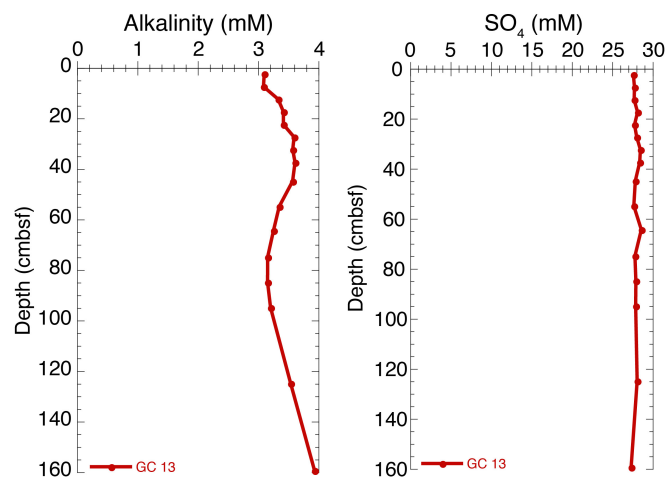
Figure 12. Pore water alkalinity and SO 4 from Gravity Core 13 at Site 4. For location of gravity cores at each site, refer to Appendix I.
