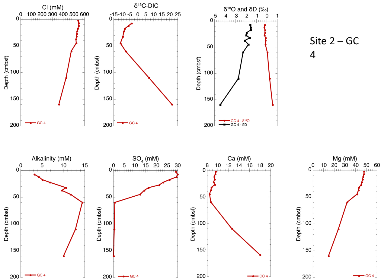
Figure 4. Pore water Cl, \delta^{13}\text{C-DIC} , \delta^{18}\text{O} , \delta\text{D} , alkalinity, \text{SO}_4 , Ca, and Mg from Gravity Core 4 at Site 2. For location of gravity cores at each site, refer to Appendix I.
