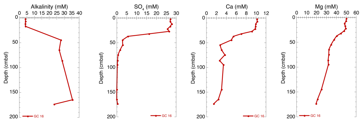
Figure 15. Pore water alkalinity, \text{SO}_4 , Ca, and Mg from Gravity Core 16 at Site 4. For location of gravity cores at each site, refer to Appendix I.
