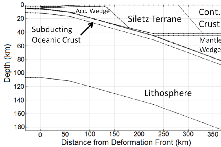
Figure 4: Thermo-physical units of the finite element model based on active and passive seismic profiles.
