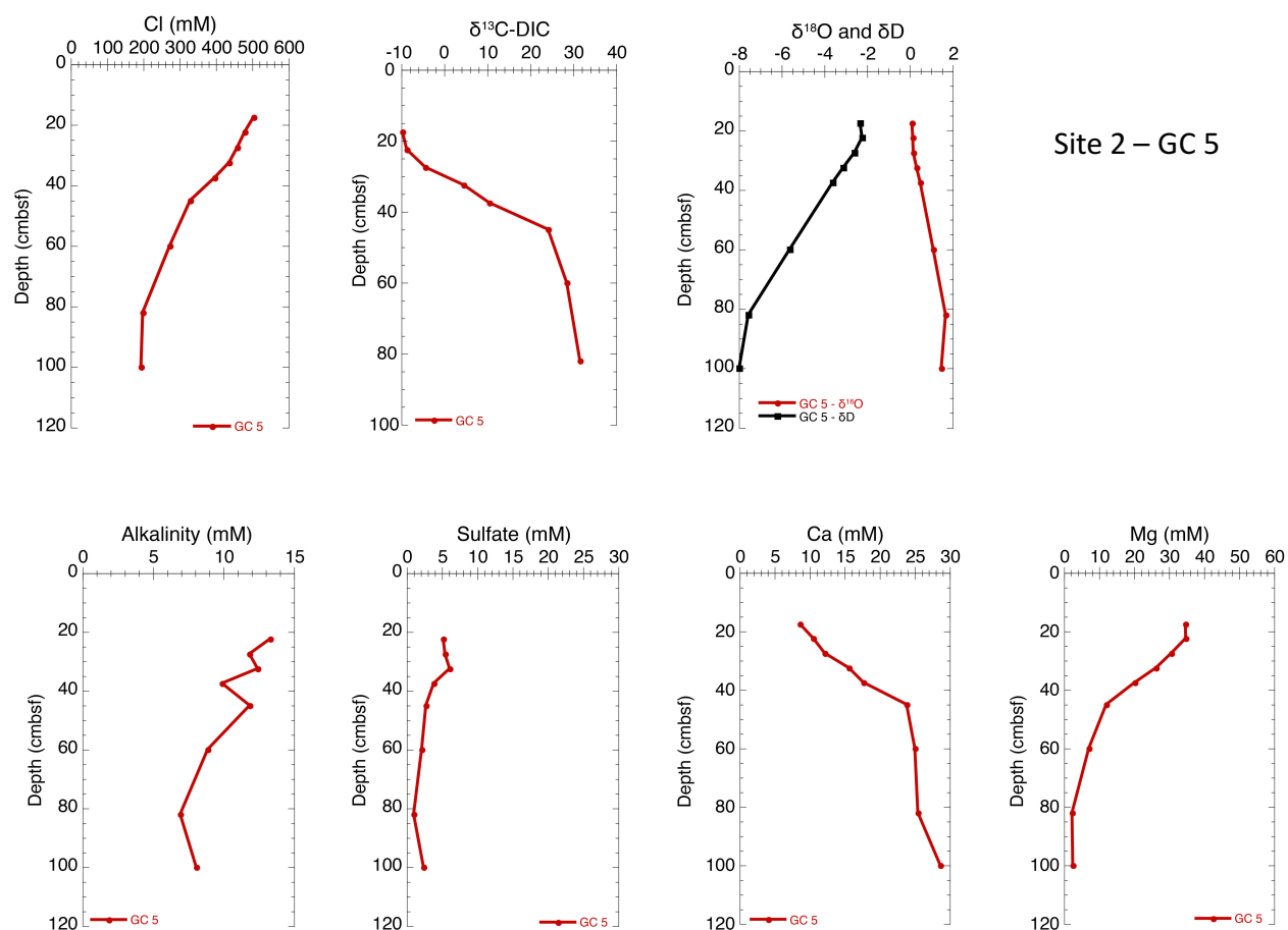
Figure 6. Pore water Cl, \delta^{13}\text{C-DIC} , \delta^{18}\text{O} , \delta\text{D} , alkalinity, \text{SO}_4 , Ca, and Mg from Gravity Core 5 at Site 2. For location of gravity cores at each site, refer to Appendix I.
