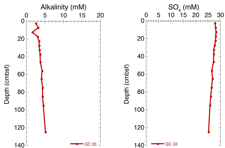
Figure 28. Pore water alkalinity and sulfate from Gravity Core 33 at Site 8. For location of gravity cores at each site, refer to Appendix I.
