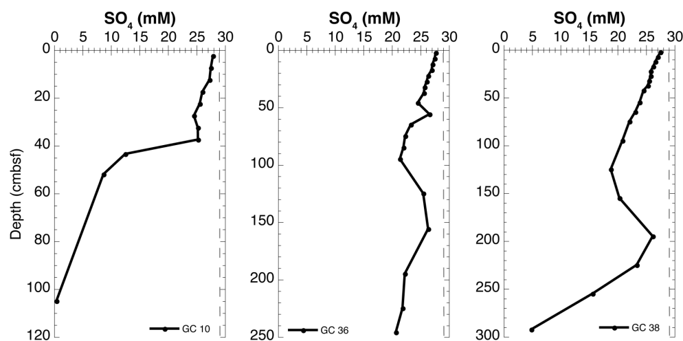
Figure 35. Examples of non-steady state pore water sulfate profiles. The profiles above are just a subset of those profiles that exhibit non-steady state conditions. GC 10 is from Site 2, GC 36 is from Site 8, and GC 38 is from Site 9. Gray dashed lines indicate seawater concentration.
