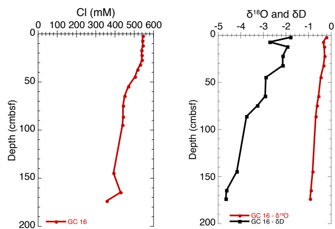
Figure 14. Pore water Cl, \delta^{18}\text{O} , and \delta\text{D} from Gravity Core 16 at Site 4. For location of gravity cores at each site, refer to Appendix I.
