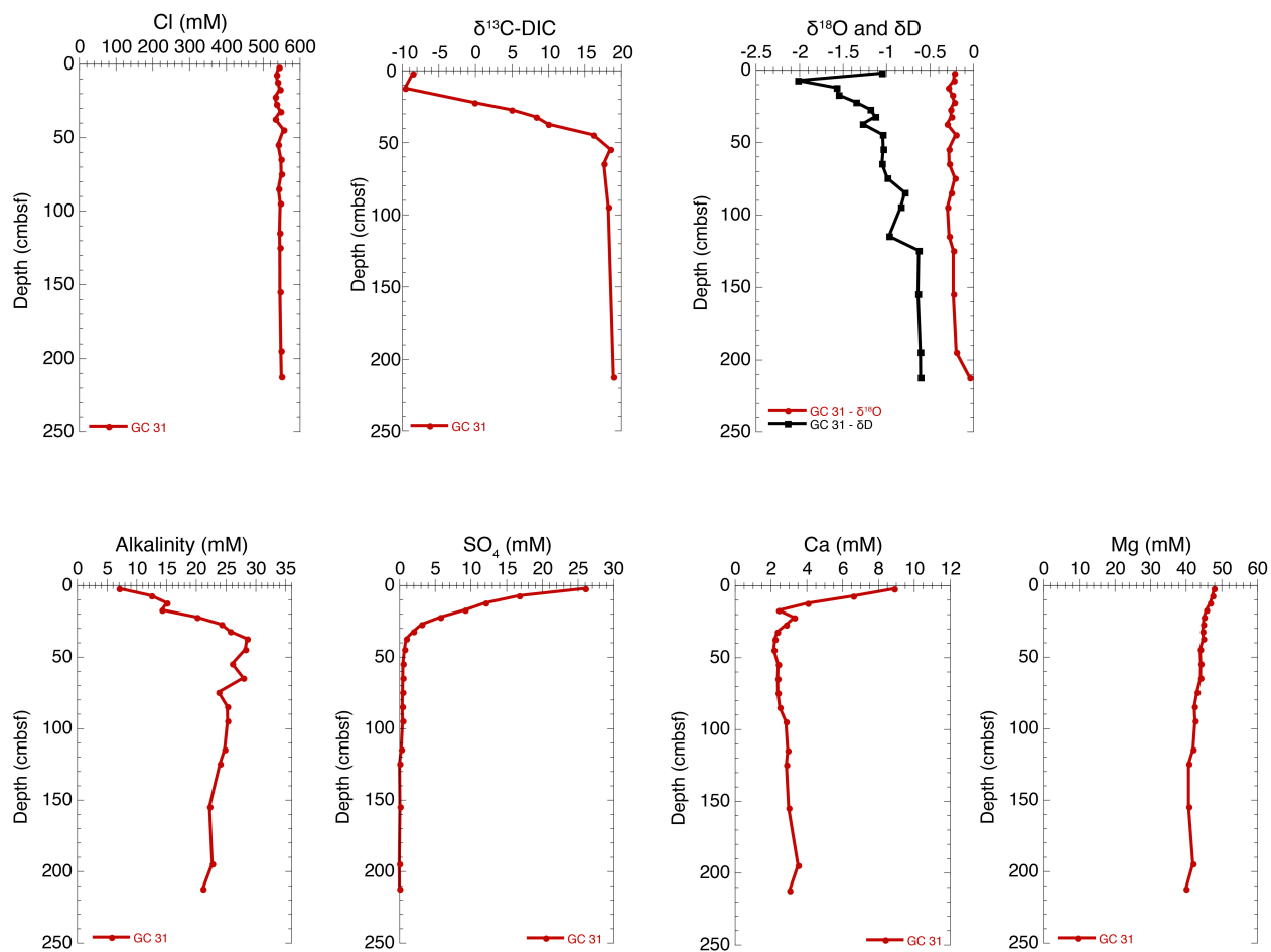
Figure 26. Pore water Cl, \delta^{18}\text{O} , \delta\text{D} , \delta^{13}\text{C-DIC} , alkalinity, sulfate, Ca, and Mg from Gravity Core 31 at Site 6. For location of gravity cores at each site, refer to Appendix I.
