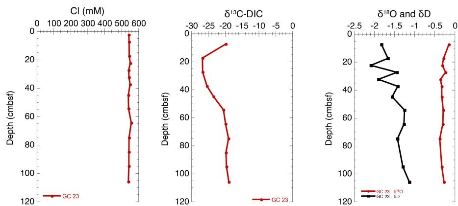
Figure 20. Pore water Cl, \delta^{18}\text{O} , \delta\text{D} , and \delta^{13}\text{C-DIC} from Gravity Core 23 at Site 5. For location of gravity cores at each site, refer to Appendix I.
