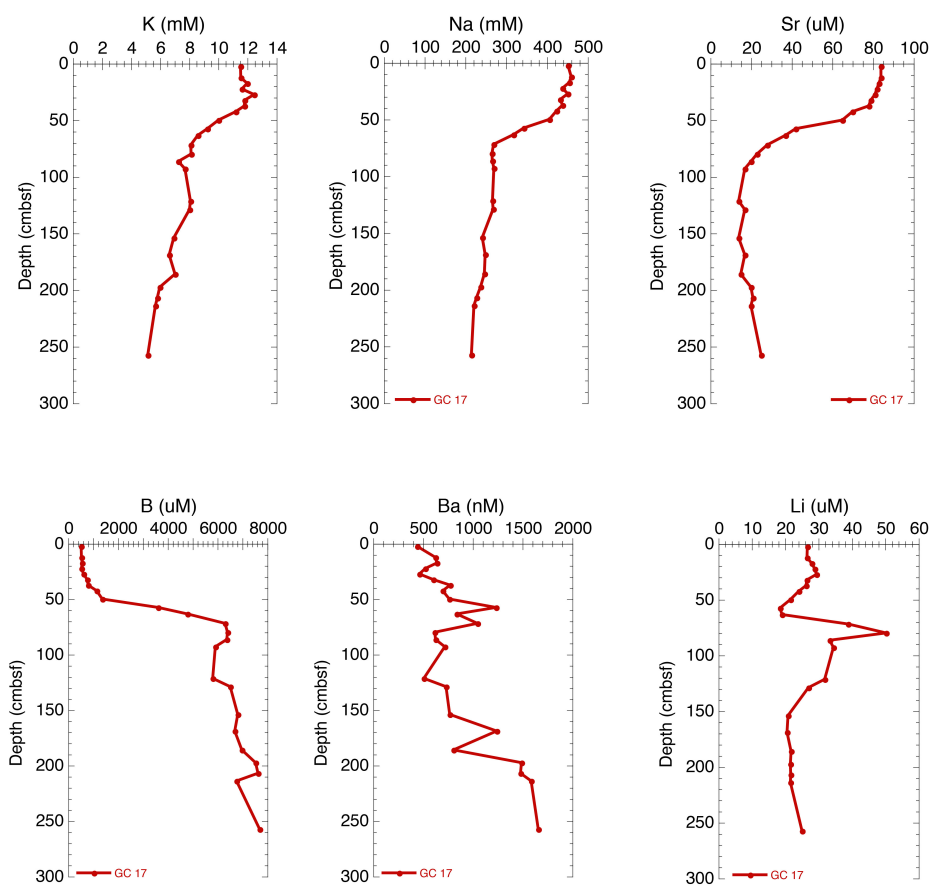
Figure 18. Pore water K, Na, Sr, B, Ba, and Li from Gravity Core 17 at Site 4. For location of gravity cores at each site, refer to Appendix I.
