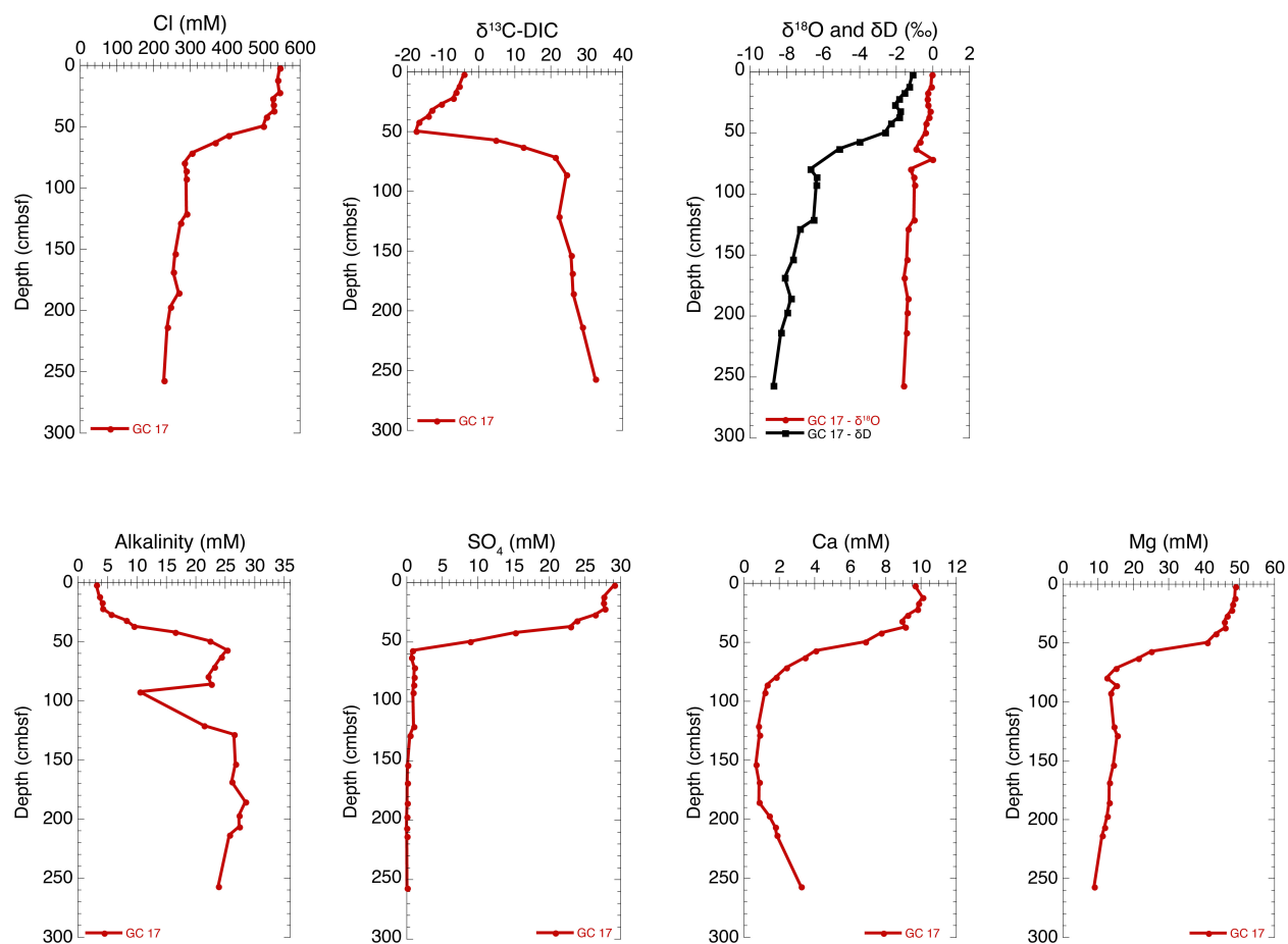
Figure 17. Pore water Cl, \delta^{18}\text{O} , \delta\text{D} , \delta^{13}\text{C-DIC} , alkalinity, \text{SO}_4 , Ca, and Mg from Gravity Core 17 at Site 4. For location of gravity cores at each site, refer to Appendix I.
