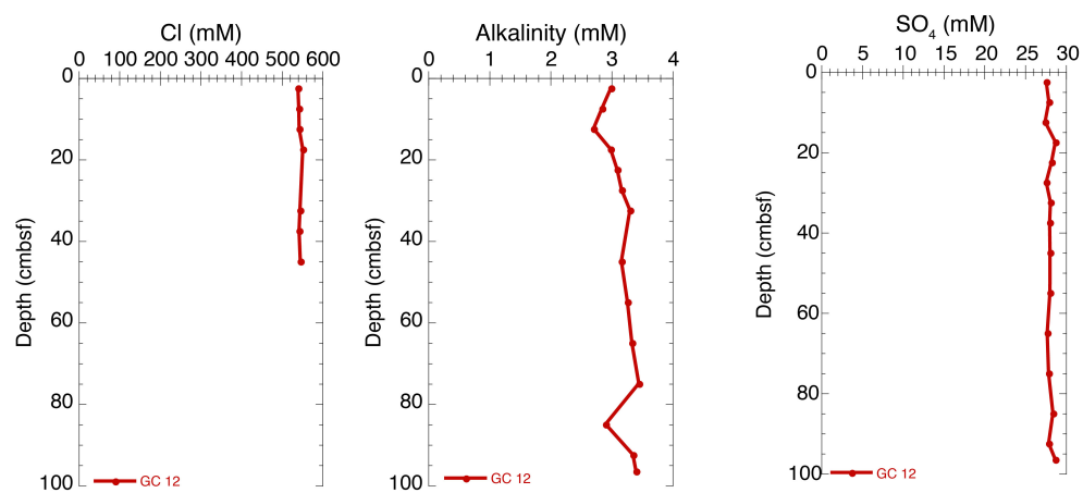
Figure 11. Pore water Cl, alkalinity, and SO 4 from Gravity Core 12 at Site 4. For location of gravity cores at each site, refer to Appendix I.
