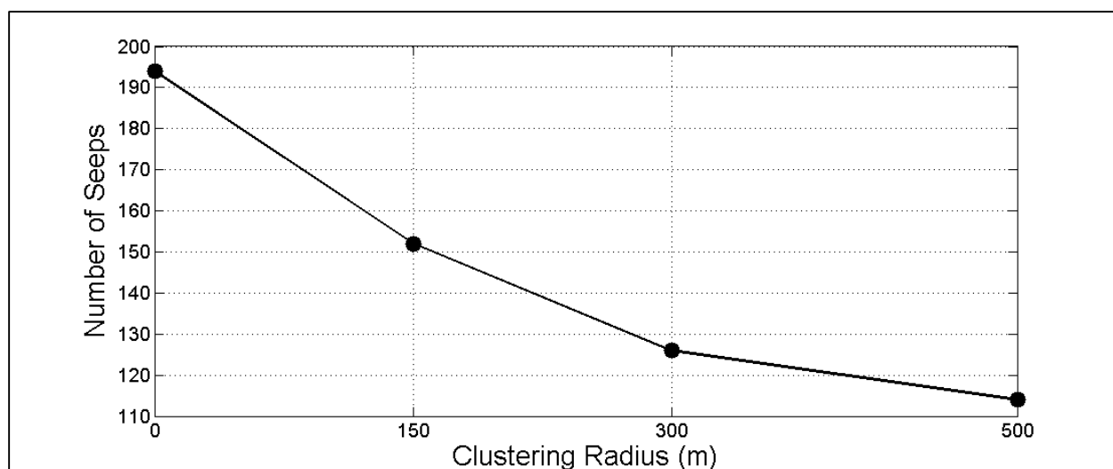
Supplemental Figure S3: Summary count of the total number of emission sites on the Washington and Oregon segments of the Cascadia margin after applying bubble stream clustering radii of 0, 150, 300 and 500 meters. A clustering radius of 0 meters would count every distinct individual bubble stream as an emission site. A clustering radius of 300 meters rather than 500 meters was used in Figures 3,4 and 5 since some sites on the continental shelf are associated with quasi-linear faults and do not show a characteristic clustering parameter (see Figure 1 in text)
