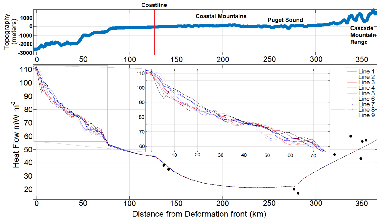
Figure 5: Large scale view of model derived surface heat flow profiles from the incoming Juan de Fuca plate to east of the Cascade Mountains. Topographic profile (top) indicates major geographical locations. Co-located black dots mark continental heat flow measurements [Blackwell et al., 1990].
