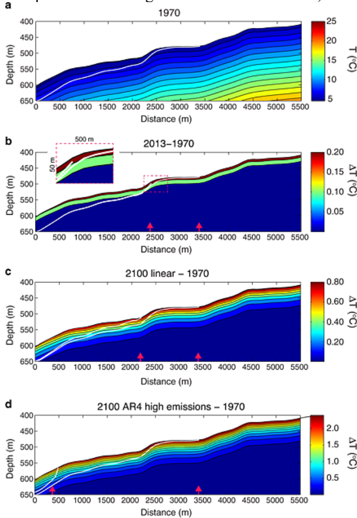
Figure 3. Sediment thermal simulations for bathymetric transect P1. (a) Initial subseafloor temperature distribution in 1970 based on the regression (see Methods) and a basal heat flow of 60 mW/m 2 [Booth-Rea et al., ]. The white line is the base of the gas hydrate stability zone (BGHSZ) in the sediment column for Structure I gas hydrate and hydrostatic pressure following the methods outlined in Tishchenko et al. [2005]. (b) The simulated change in sediment temperature between 1970 and 2013 and the corresponding shift in the BGHSZ. The BGHSZ shoals over a broad area in response to warming, accompanied by a retreat of its landward edge (indicated by red arrows). (c) Simulated change in sediment temperature between 1970 and 2100 based on the linear extrapolation of seafloor temperature. The upper white line is the BGHSZ in 2100. (d) Simulated change in sediment temperature between 1970 and 2100 based on the high-emission AR4 projection. The upper white line is the BGHSZ in 2100, and the lower white line is the BGHSZ in 1970.
