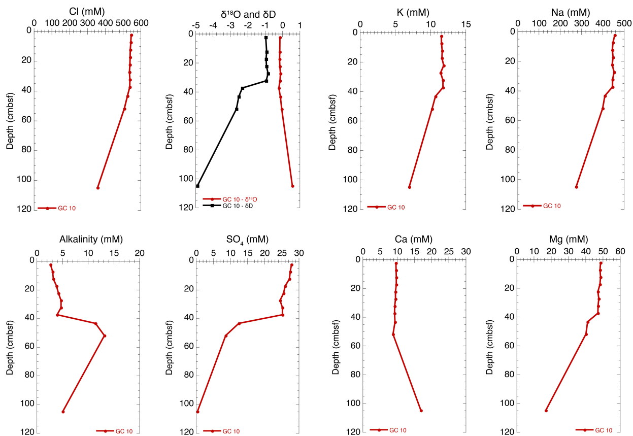
Figure 9. Pore water Cl, \delta^{18}\text{O} , \delta\text{D} , K, Na, alkalinity, \text{SO}_4 , Ca, and Mg from Gravity Core 10 at Site 2. For location of gravity cores at each site, refer to Appendix I.
