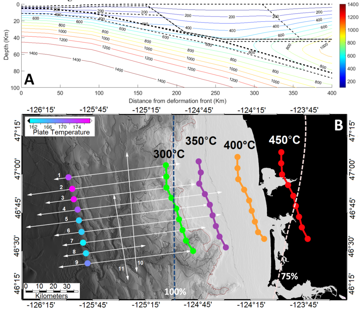
Figure 6: A) Modeled isotherm profile for MCS Line 5. B) Temperature of Juan de Fuca plate sediment interface at the deformation front (circles) for all 9 profile lines, see color bar for scale. The 300°, 350°, 400°, and 450°C isotherms are shown, along with 100% and 75% locking zones.
