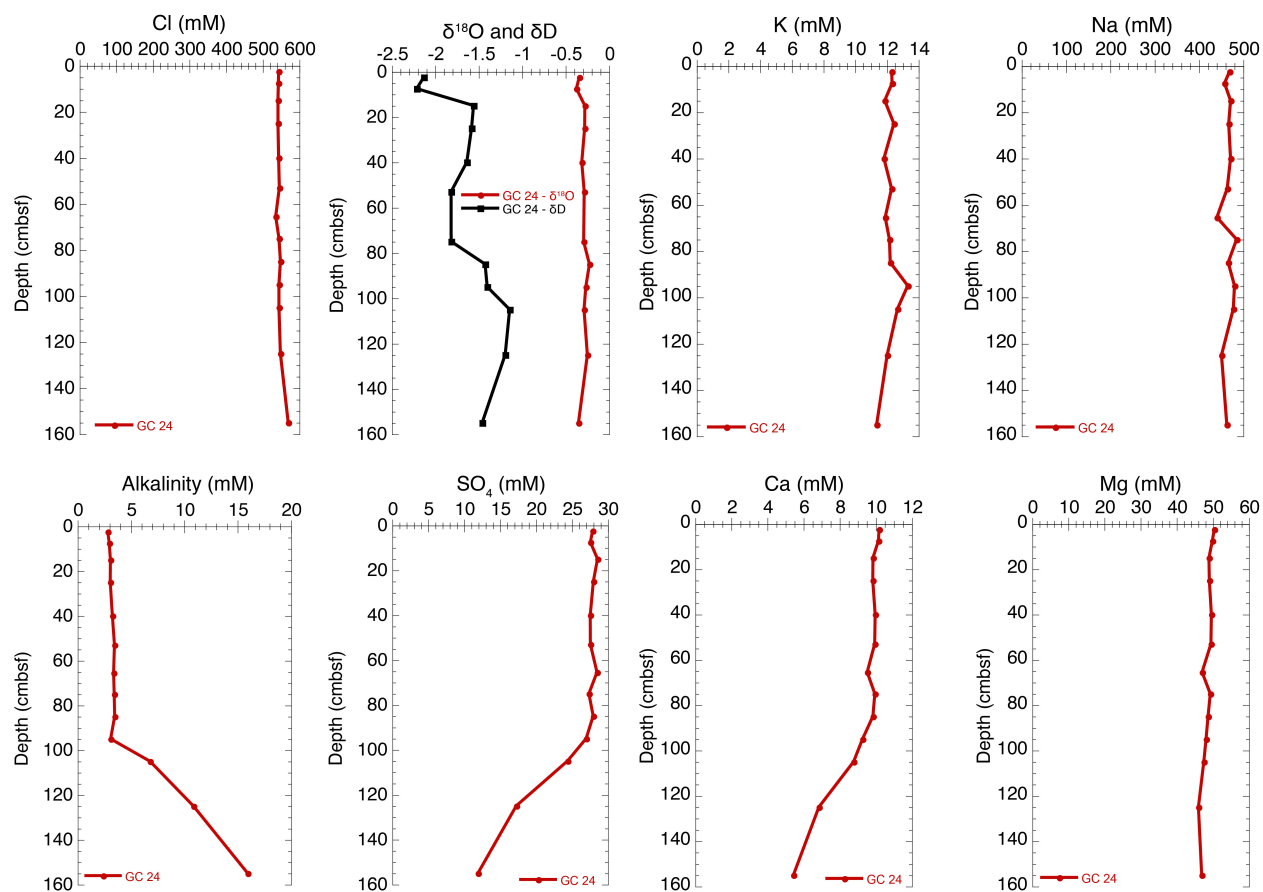
Figure 22. Pore water Cl, \delta^{18}\text{O} , \delta\text{D} , K, Na, alkalinity, sulfate, Ca, and Mg from Gravity Core 24 at Site 5. For location of gravity cores at each site, refer to Appendix I.
