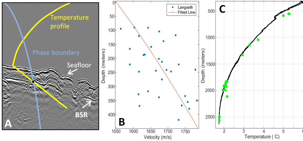
Figure 2: Method and parameters used to calculate BSR heat flow. A) BSR temperature is calculated knowing the depth of the seafloor and BSR using the methane hydrate phase stability curve (blue line). B) Seismic velocity ( V_p ) to meters below seafloor relationship from the Langseth pre-stack time migrated velocity profiles. Data points represent velocity picks over anticlinal ridges within the lower accretionary margin. Orange line is the best fit of the data. See text for equation. C) Temperature profile determined by CTD cast (Figure 1). Green dots are seafloor temperatures, measured 5 centimeters above the seafloor derived from Thermal Blankets
