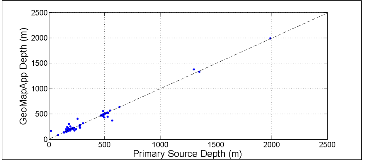
Supplemental Figure S4: Comparison of all primary source depths (fishing sonar, research sites, literature) with their equivalent depths obtained using the GeoMapApp database (multibeam bathymetry overlay data only). The R^2 value for a linear fit of a 1:1 slope is 0.9823. The strong linear correlation implies that most depths used are consistent with independent swath bathymetry depth sources and therefore likely to be reliable for this compilation.
