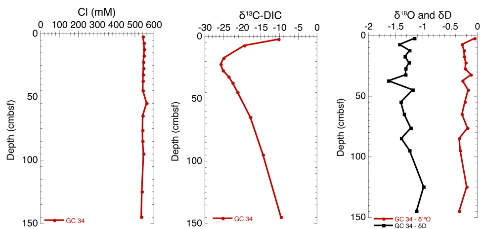
Figure 29. Pore water Cl, \delta^{18}\text{O} , \delta\text{D} , and \delta^{13}\text{C} -DIC from Gravity Core 34 at Site 8. For location of gravity cores at each site, refer to Appendix I.
