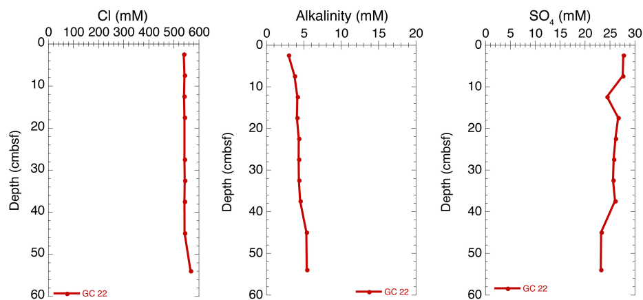
Figure 19. Pore water Cl, alkalinity, and SO 4 from Gravity Core 22 at Site 5. For location of gravity cores at each site, refer to Appendix I.
