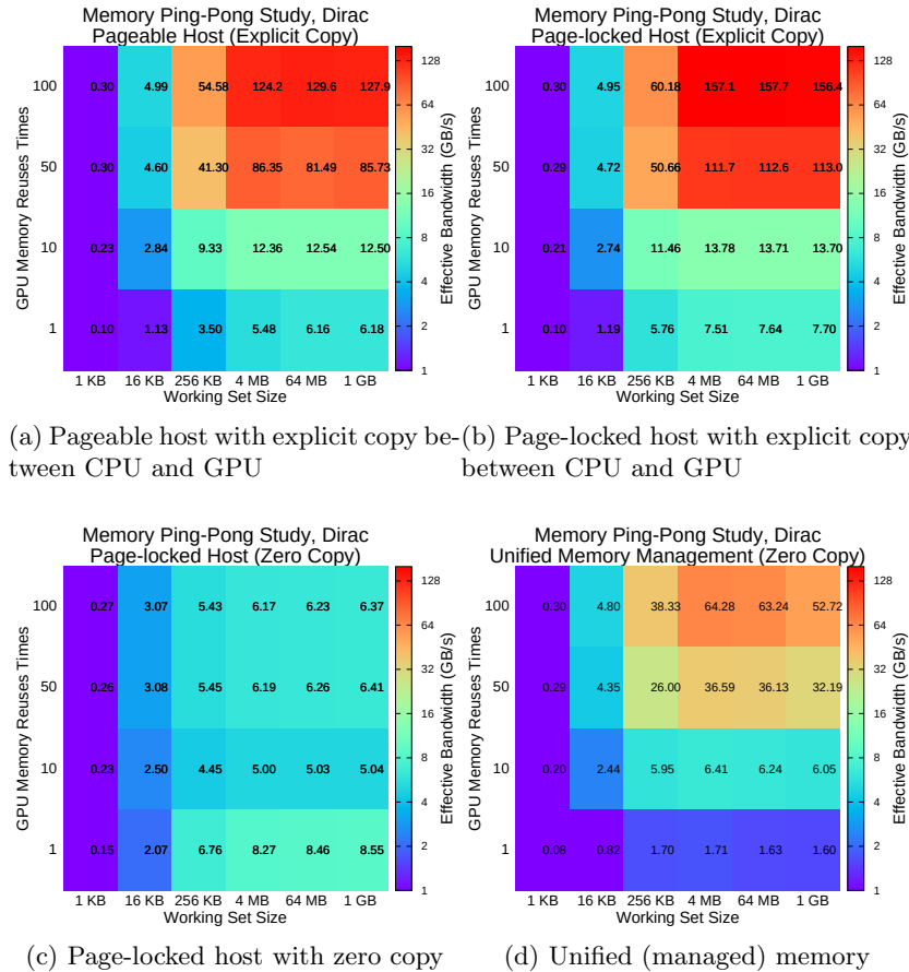
Fig. 7. Effective bandwidth as a function of GPU temporal locality (reuse) and working set size for four different GPU device memory management mechanisms.
