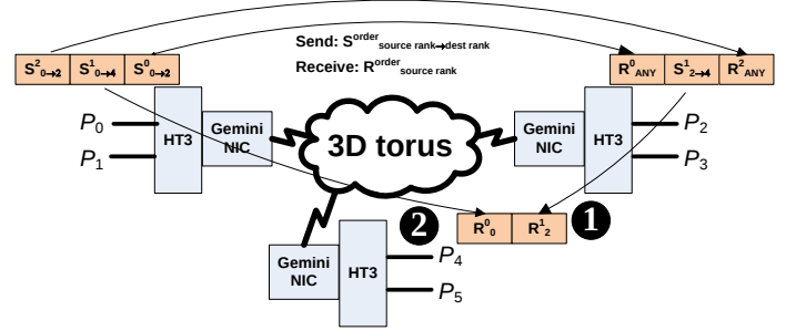
Figure 10. MPI message ordering constraints for deterministic execution.
