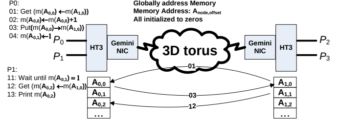
Figure 7. A UPC ordering challenge on relaxed ordering interconnect. Can the interconnect reorder operations 03 and 12?
