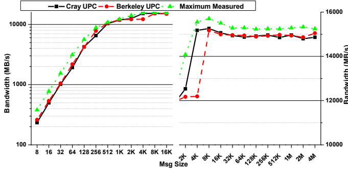
Figure 8. Cray and Berkeley UPC performance implemented on DMAPP and GNI interfaces respectively. Performance is compared with best observed performance on each message size.
