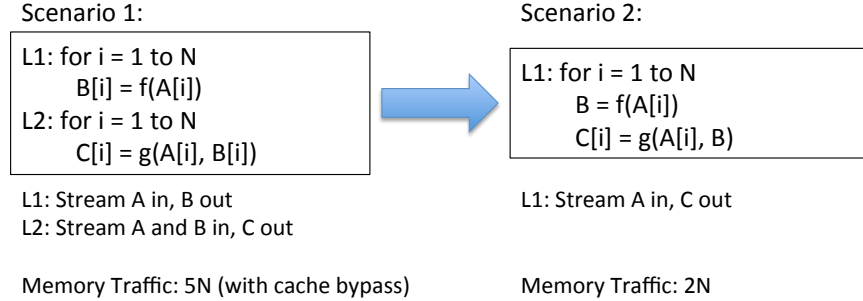
Fig. 4: Example of loop fusion code optimization.
