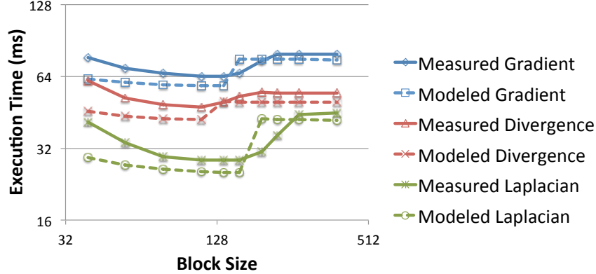
Fig. 9: Measured and modeled execution times for various blocking sizes for three benchmark finite difference kernels.
