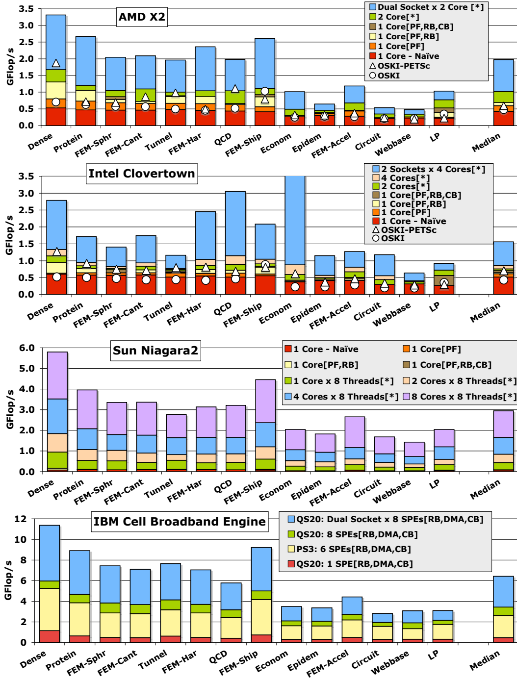
Figure 4: Effective SpMV performance (not raw flop rate) on (from top to bottom) AMD X2, Clovertown, Niagara, and Cell, showing increasing degrees of single-core optimizations — prefetching (PF), register blocking (RB) and cache-blocking (CB) (denoted as *) — as well as performance on increasing numbers of cores, and multiple-socket (full system) optimized results. OSKI and OSKI-PETSc results are denoted with circles and triangles. Note: Bars show the best performance for the current subset of optimizations/parallelism. The LP matrix could not be run on the PS3; the 6 SPE QS20 data is shown instead.
