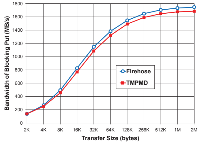
Figure 5. Firehose vs. TMPMD for Blocking Put
