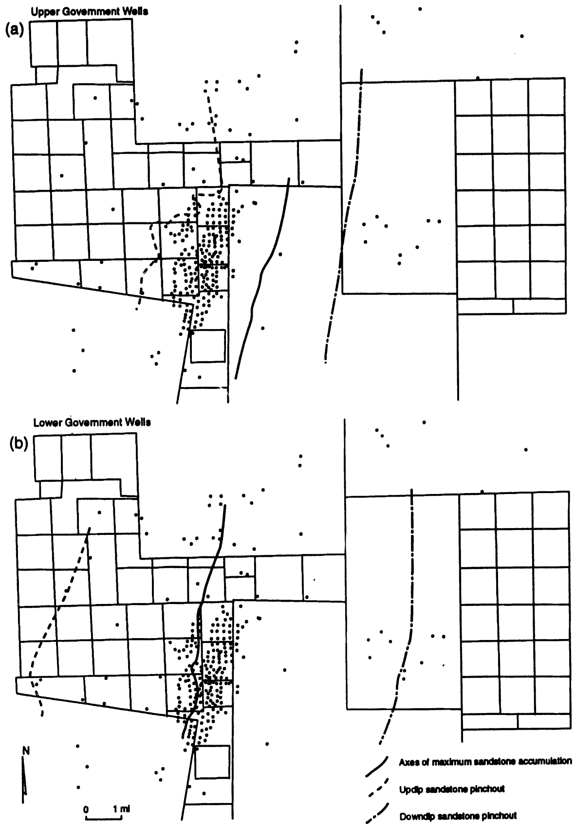
Figure 14. Map of axis of maximum sandstone accumulation and updip and downdip lines marking sandstone pinch-outs.
