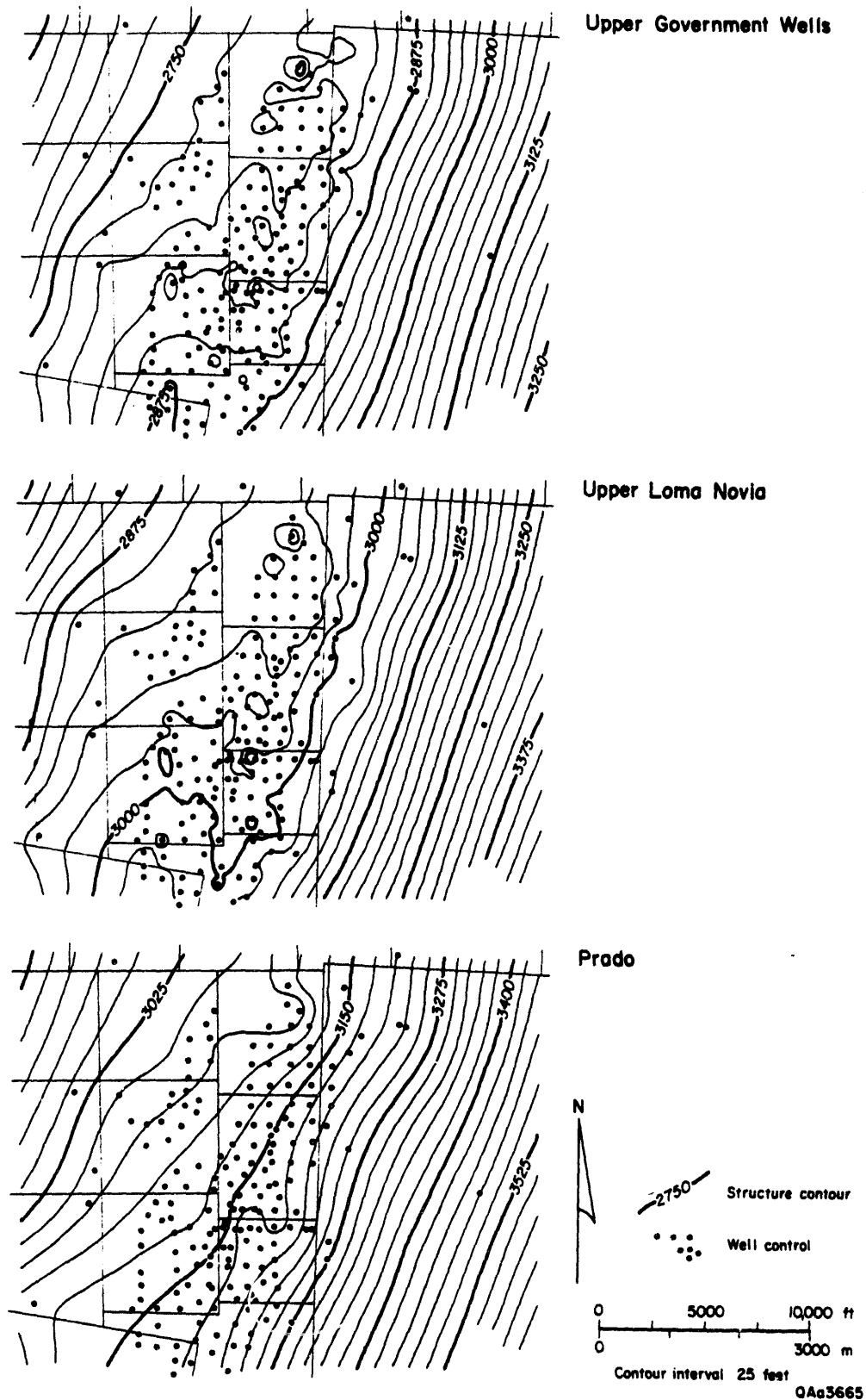
Figure 6. Structure-contour maps of Upper Government Wells, Upper Loma Novia, and Prado reservoirs, Prado field. Development of structural nose in field area is a result of drape compaction over thick, sand-rich Middle Loma Novia reservoirs.
