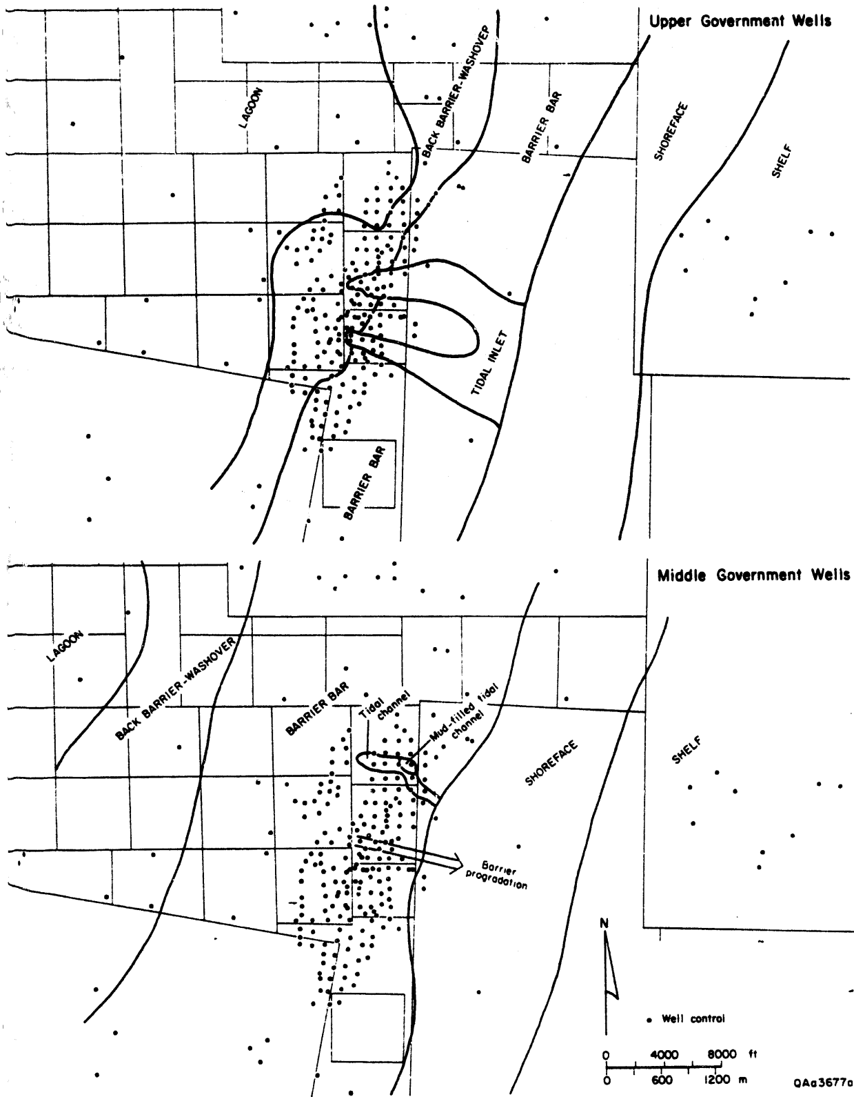
Figure 18. Depositional facies of Upper Government Wells, Middle Government Wells, Upper Loma Novia, and Middle Loma Novia reservoir sandstones, Prado field.
