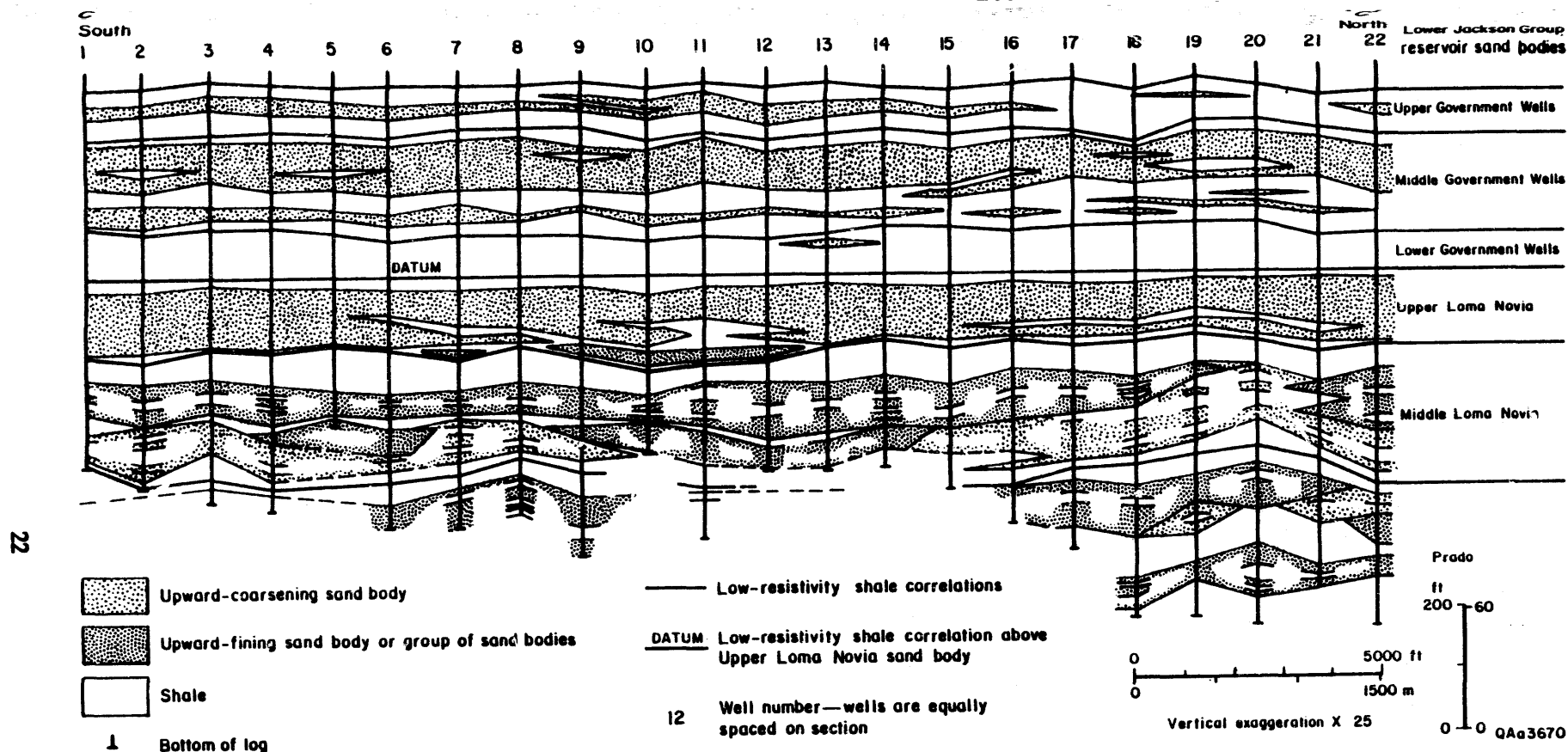
Figure 11. Strike-oriented cross section, Prado field, showing correlation of mapping units and distribution and character of reservoir sandstones. Upper Government Wells, Middle Government, and Upper Loma Novia reservoir sandstones are characteristically upward-coarsening continuous sand bodies. In contrast, Middle Loma Novia and Prado reservoir sandstones are characteristically complex packages of upward-fining as well as upward-coarsening sand bodies.
