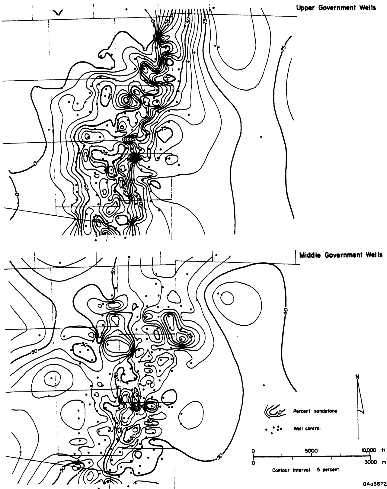
Figure 13. Percentage-sandstone maps for Upper Government Wells, Middle Government Wells, Upper Loma Novia, and Middle Loma Novia reservoir sandstones, Prado field. Maximum percentage sandstone for all intervals trends north-northeast. The area of greater than 75 percent sandstone prograded downdip from the Middle Loma Novia to the Upper Government Wells.
