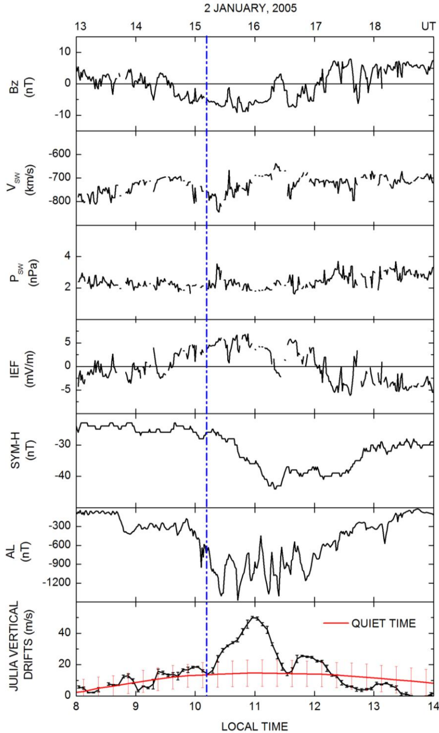
Figure 1. Variations of Jicamarca vertical plasma drifts as a response to changes in solarwind and geophysical parameters on 2 January 2005. From top panel are shown IMF Bz, V_x , P_{sw} , IEF_y , SYM-H, AL and JULIA vertical plasma drifts respectively. The red line on the bottom panel shows the empirical bimonthly climatological quiet time vertical plasma drifts for non-SSW January-February period from Hui and Fejer [2015] along with their standard deviations. The vertical dashed line indicates the commencement time of substorm.
