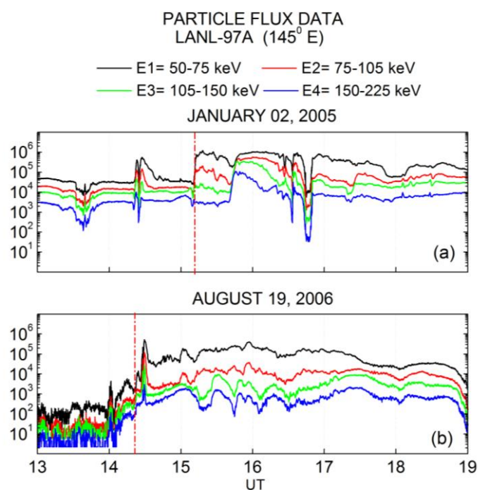
Figure 3. Electron flux data at geosynchronous orbit from LANL-97A satellite in different energy bins for both events. The red lines marks the onset time of the substorms.
