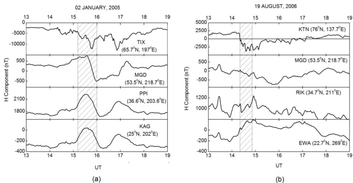
Figure 4. -Variations in the H-component of earth's geomagnetic field to confirm the onset of substorms during the two events.
