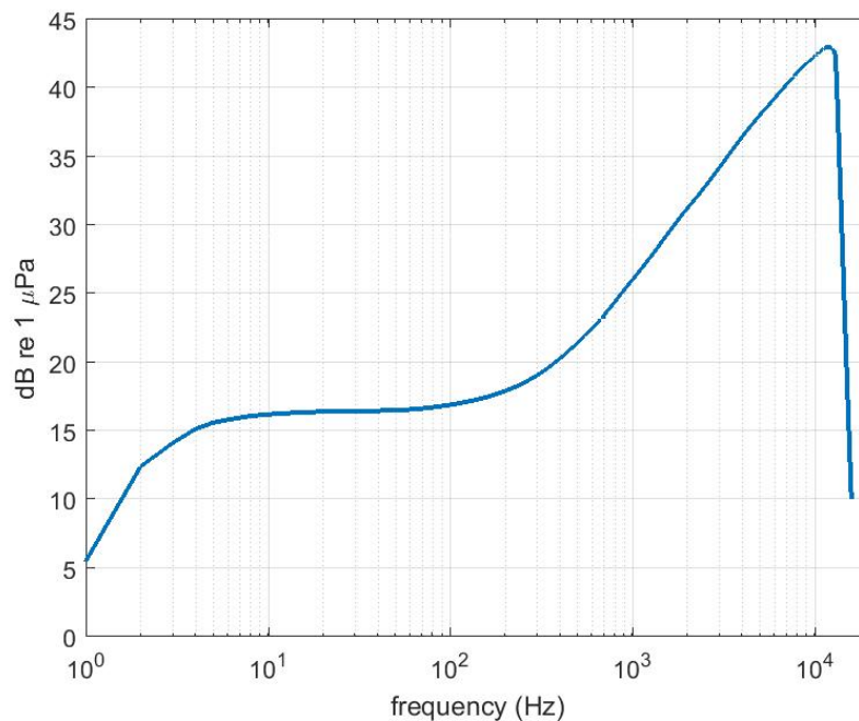
Figure 3. The instrument response curve for the hydrophone preamplifier.
