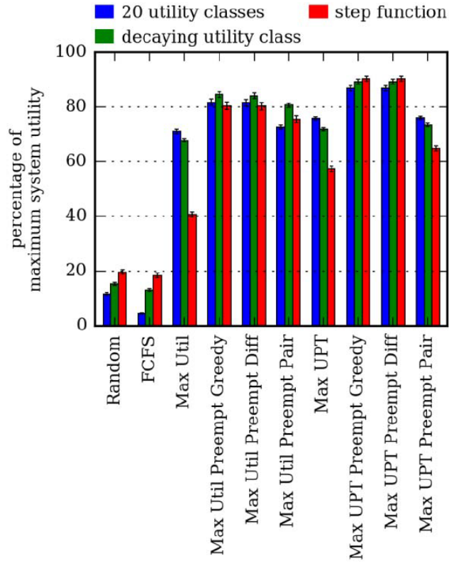
Figure 3. The percentage of maximum system utility is shown for workloads where the utility class used to determine utility functions is varied from step functions, a single decaying utility class, and 20 utility classes as described in Subsection IV.C. The results are shown with 95% mean confidence intervals.
