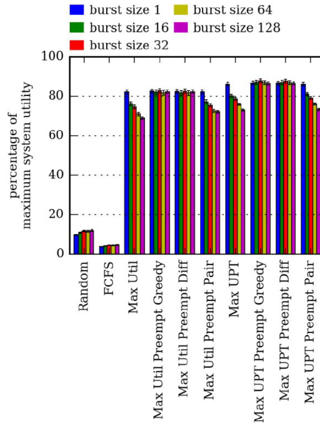
Figure 4. The percentage of maximum system utility earned by each of the heuristics for five different workloads where the burst sizes of tasks arriving are 1, 16, 32, 64, and 128. The results are shown with 95% mean confidence intervals.
