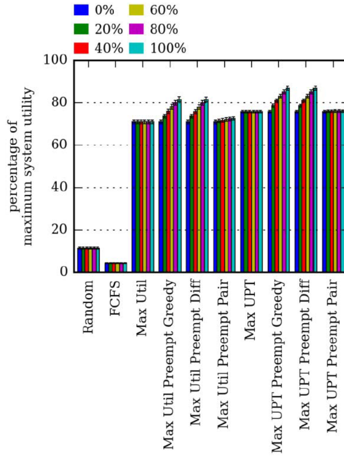
Figure 5. The percentage of maximum system utility earned by each of the heuristics for six different workloads where the percentage of tasks that can preempt and the percentage of tasks that can be preempted are varied over 0%, 20%, 40%, 60%, 80%, and 100%. The results are shown with 95% mean confidence intervals.
