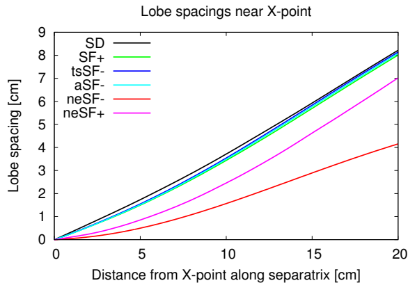
FIG. 6. Lobe spacings near the X-point, measured by the distance between two crossing points between the perturbed and unperturbed separatrix as sketched in figure 1.
