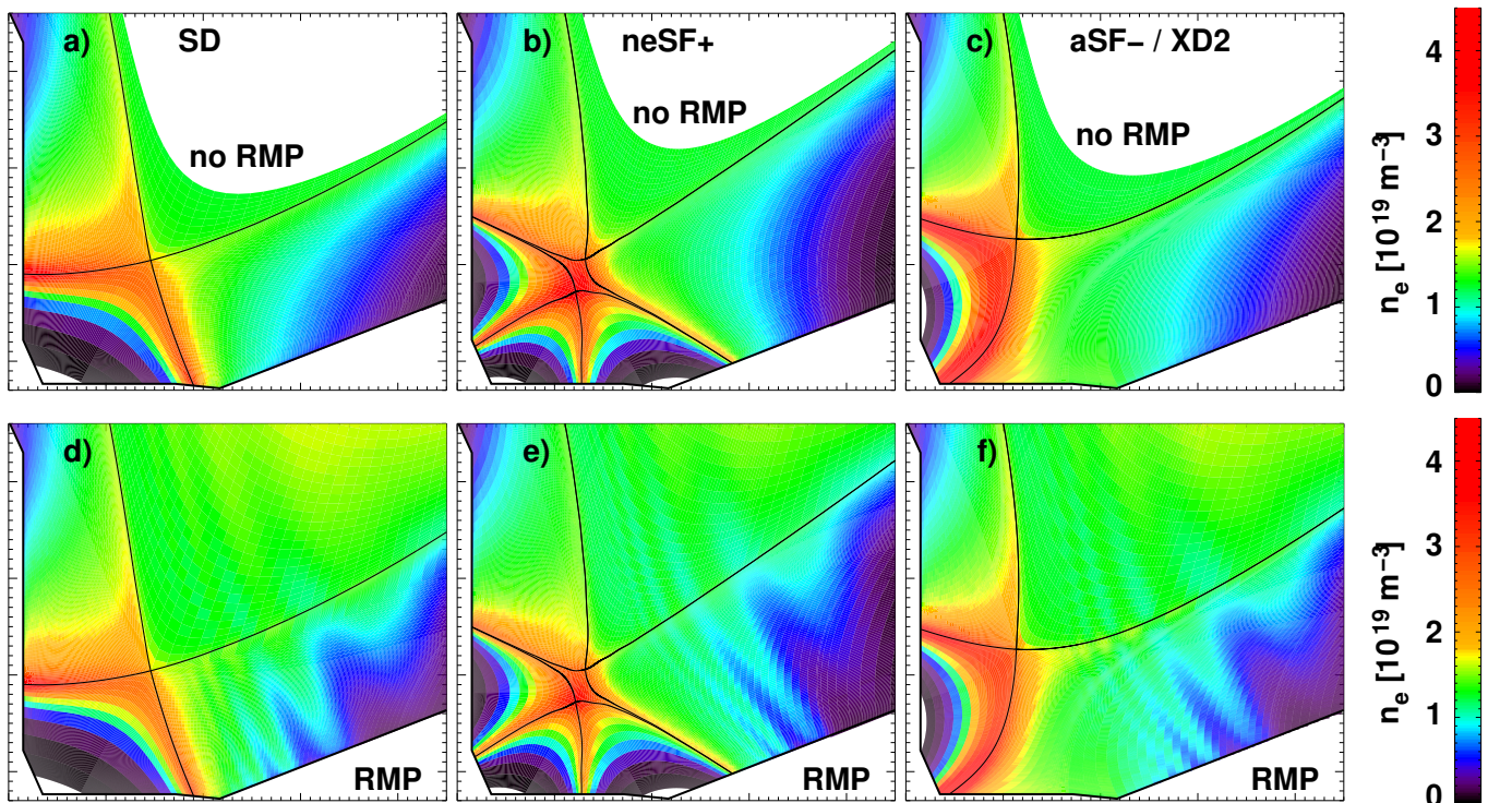
FIG. 8. Comparison of the edge plasma density with and without magnetic perturbations: (a,d) standard divertor configuration, (b,e) near exact snowflake configuration and (c,f) asymmetric snowflake minus / X-divertor configuration. The position of the unperturbed separatrix is marked in black for reference.
