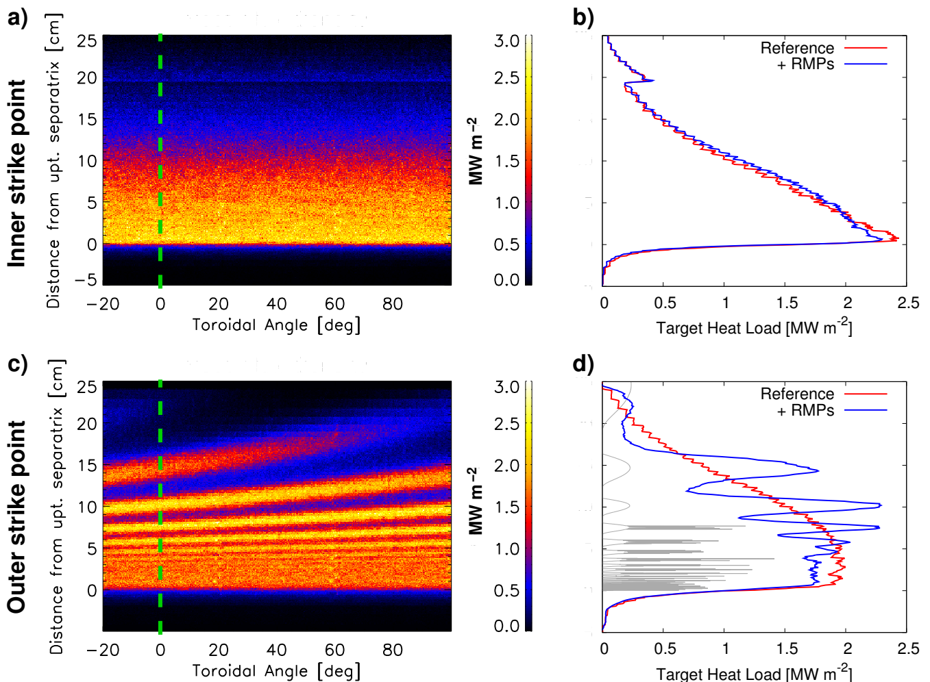
FIG. 9. Divertor heat loads at the inner and outer strike point for the SF+ case, the 1D profiles are extracted at \varphi = 0 deg.
