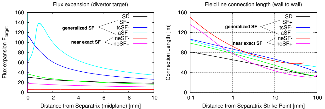
FIG. 3. (a) Flux expansion and (b) field line connection length at the outer divertor target.
