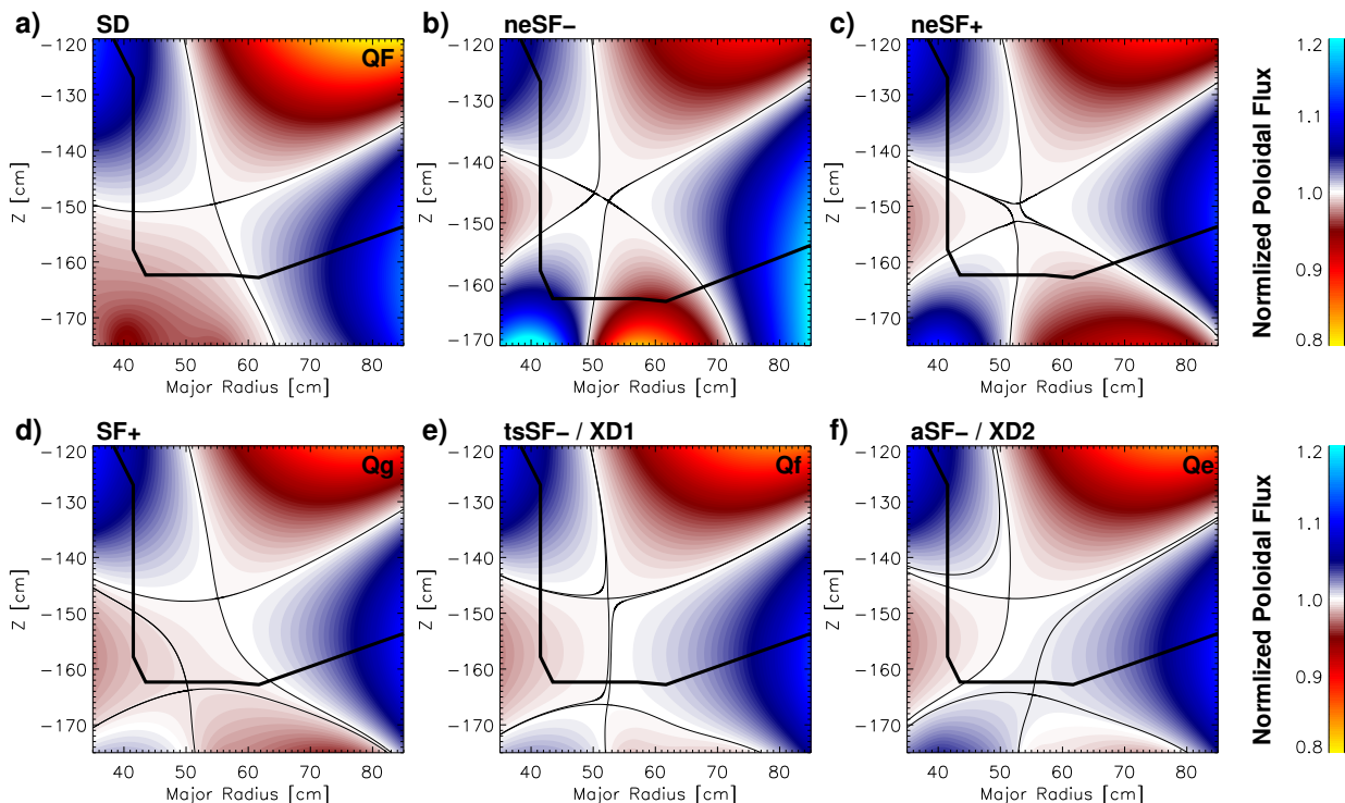
FIG. 2. The standard divertor (SD) reference configuration (a) and an overview of different near exact and generalized 'snowflake' configurations in NSTX-U: (b,c) near exact SF (neSF) configurations approximated as SF- and SF+ respectively, (d) a 'snowflake plus' (SF+) configuration, (e) a 'tilted symmetric snowflake minus' (tsSF-) configuration and (f) an 'asymmetric snowflake minus' (aSF-) configuration. These equilibrium configurations are taken from the 116313/NfHz0+Q series, except for neSF- which is 135111/Nwj_08.
